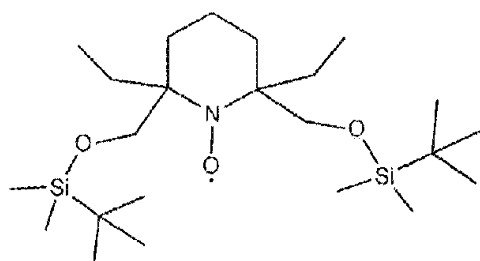
G5, LogP=8.2
