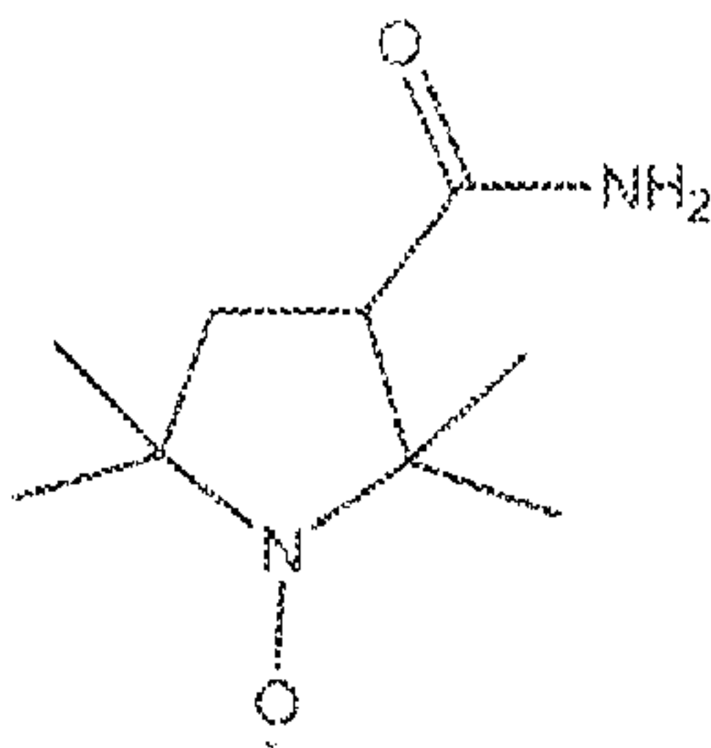
3-Carbamoyl-PROXYL, LogP=0.9
