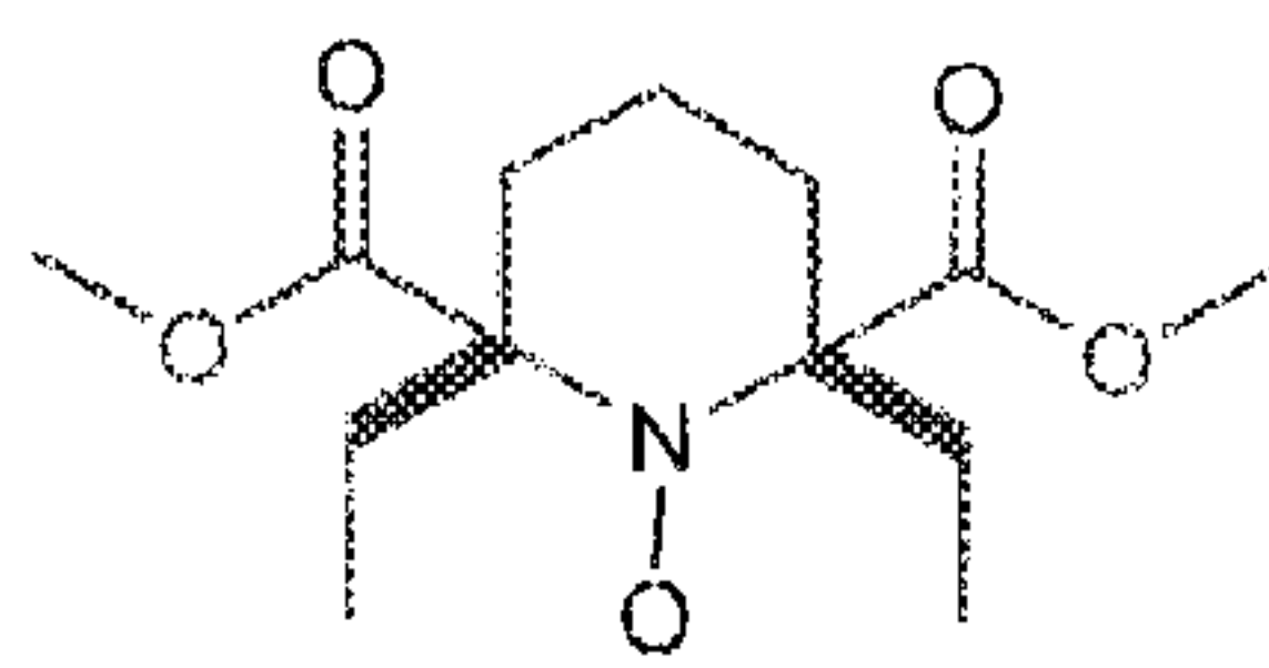
G2, LogP=2.5
