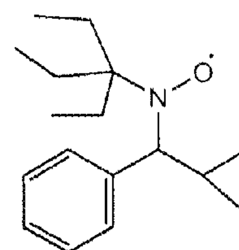
G4, LogP=5.4
