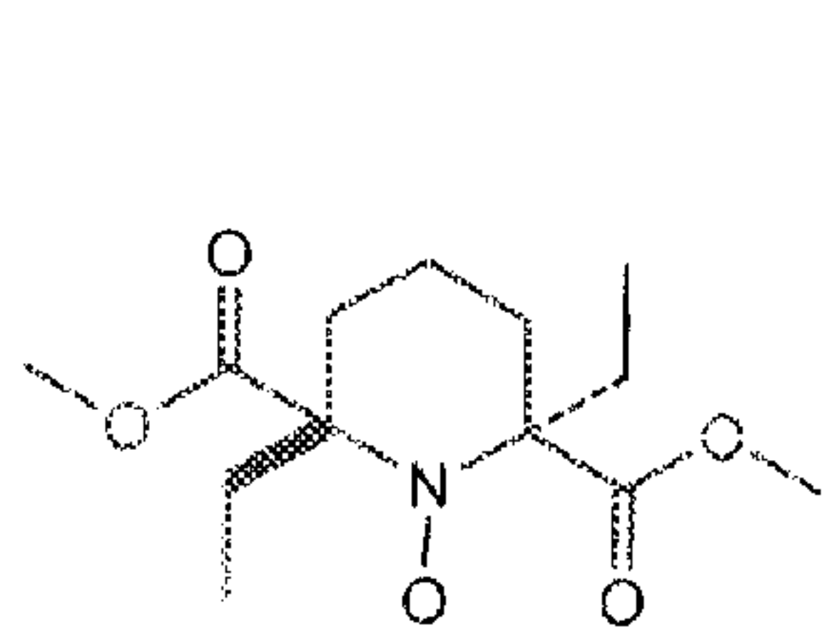
G1, LogP=2.0
