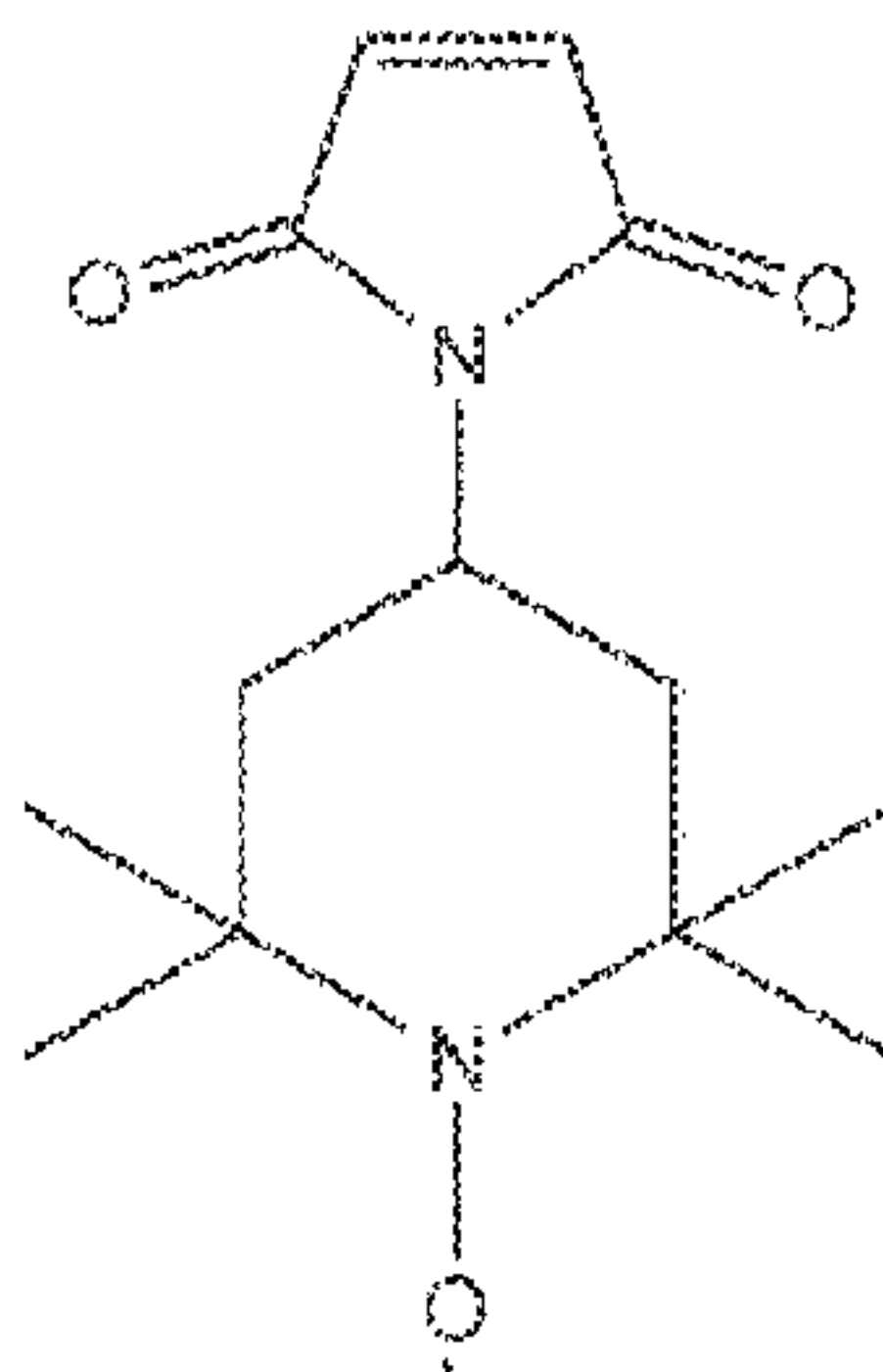
4-Maleimido-TEMPO, LogP=2.9
