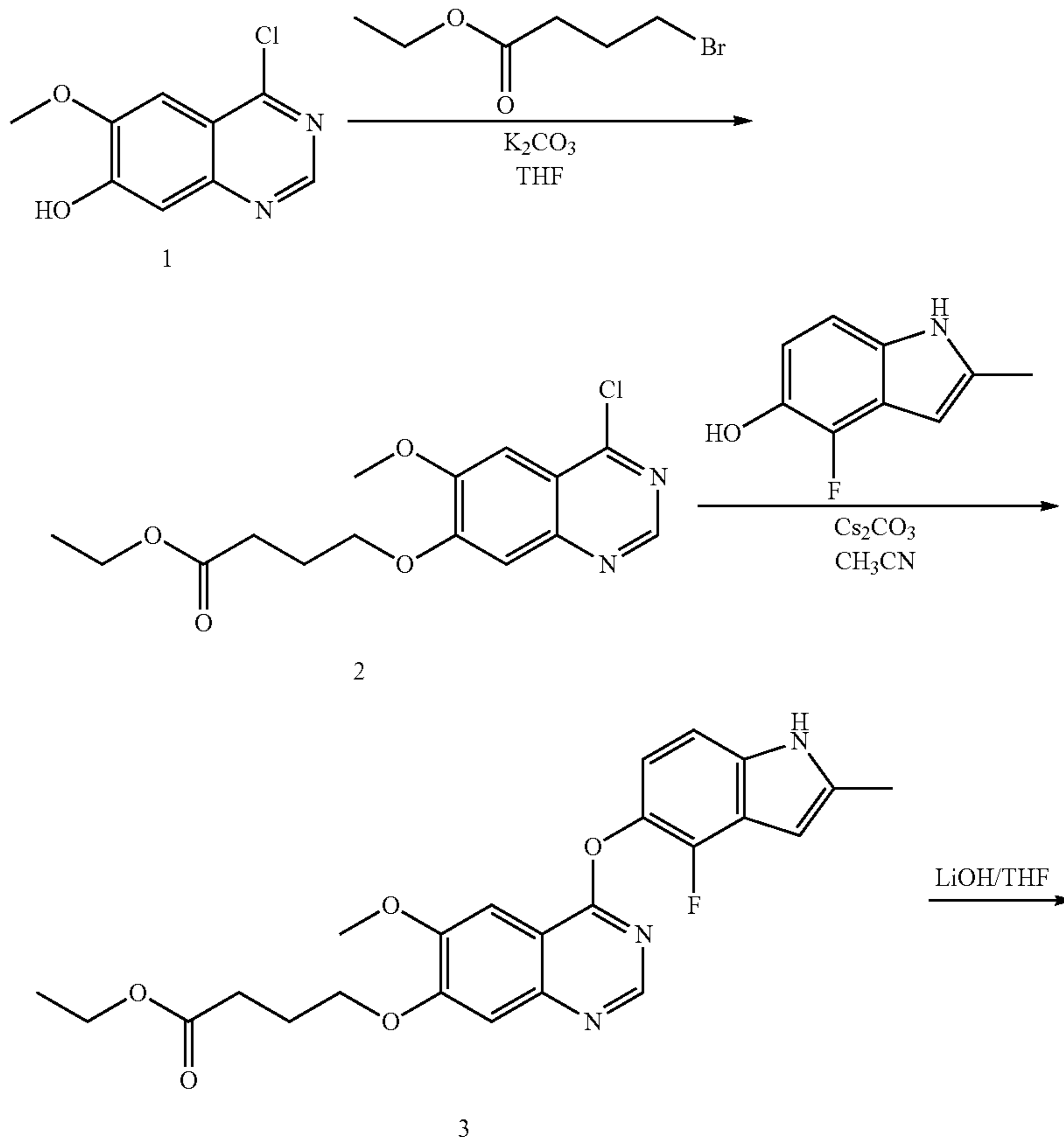
Scheme 1: Method of synthesizing Compound 5.
