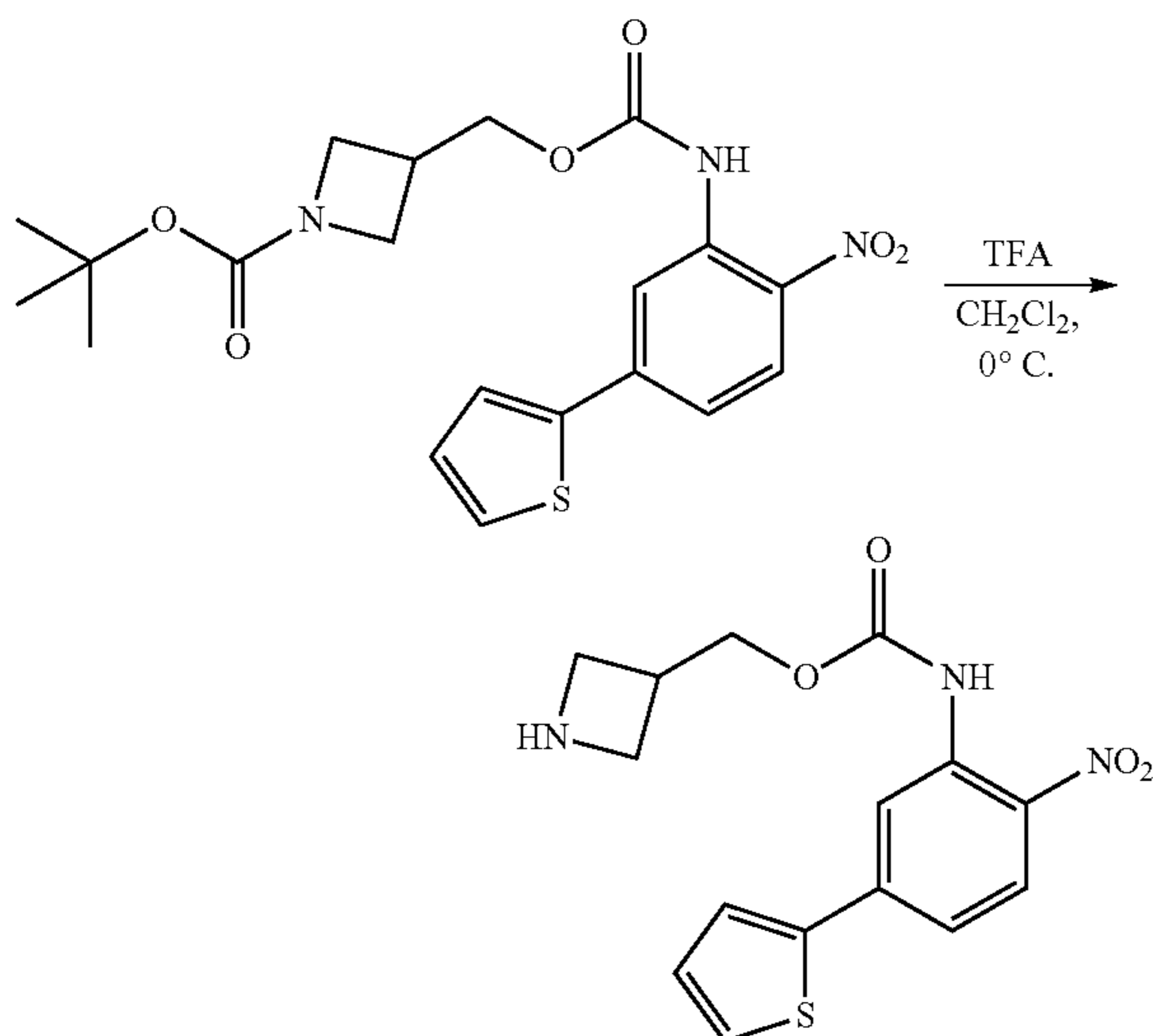
Scheme 18
