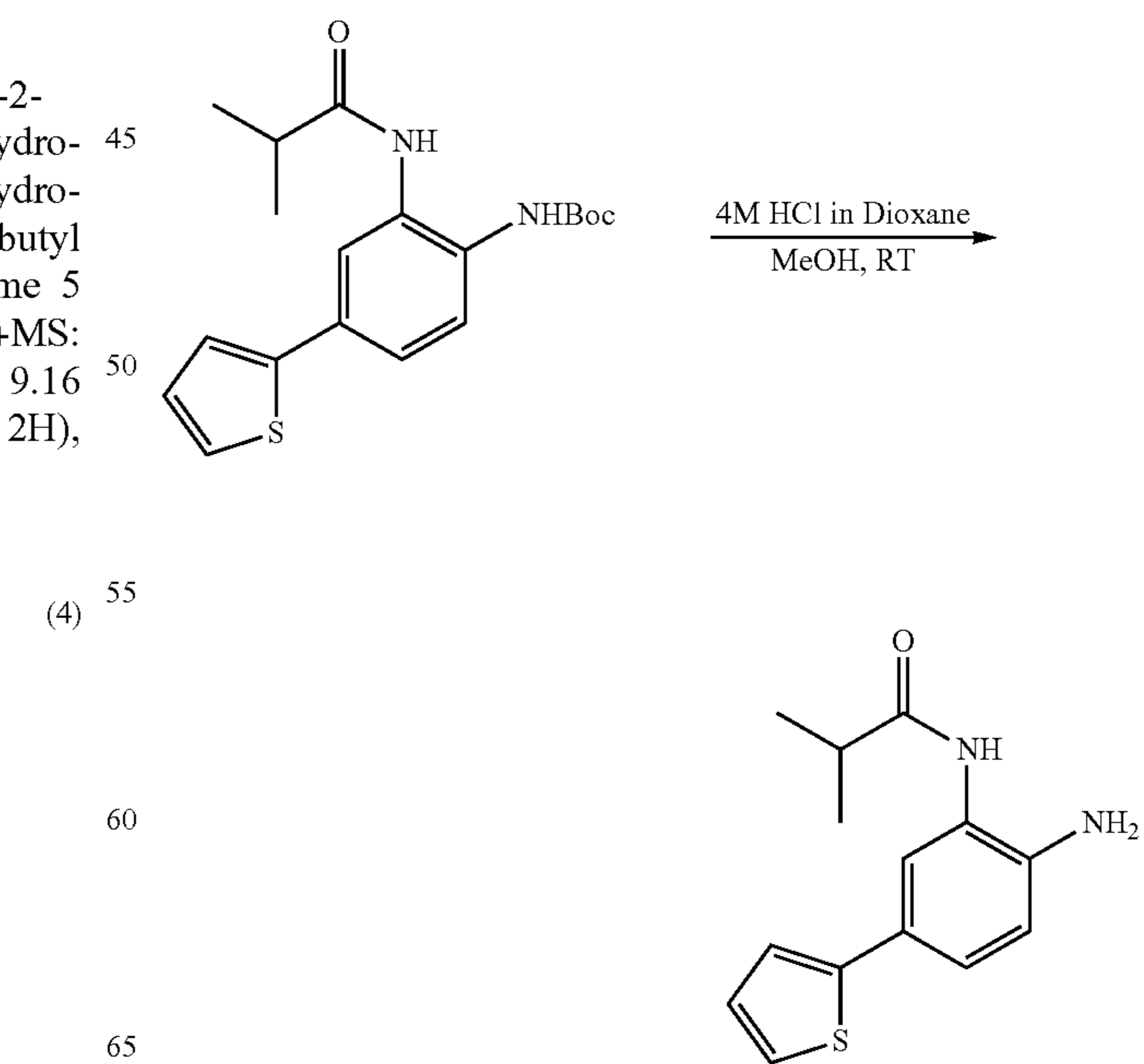
Scheme 7A
