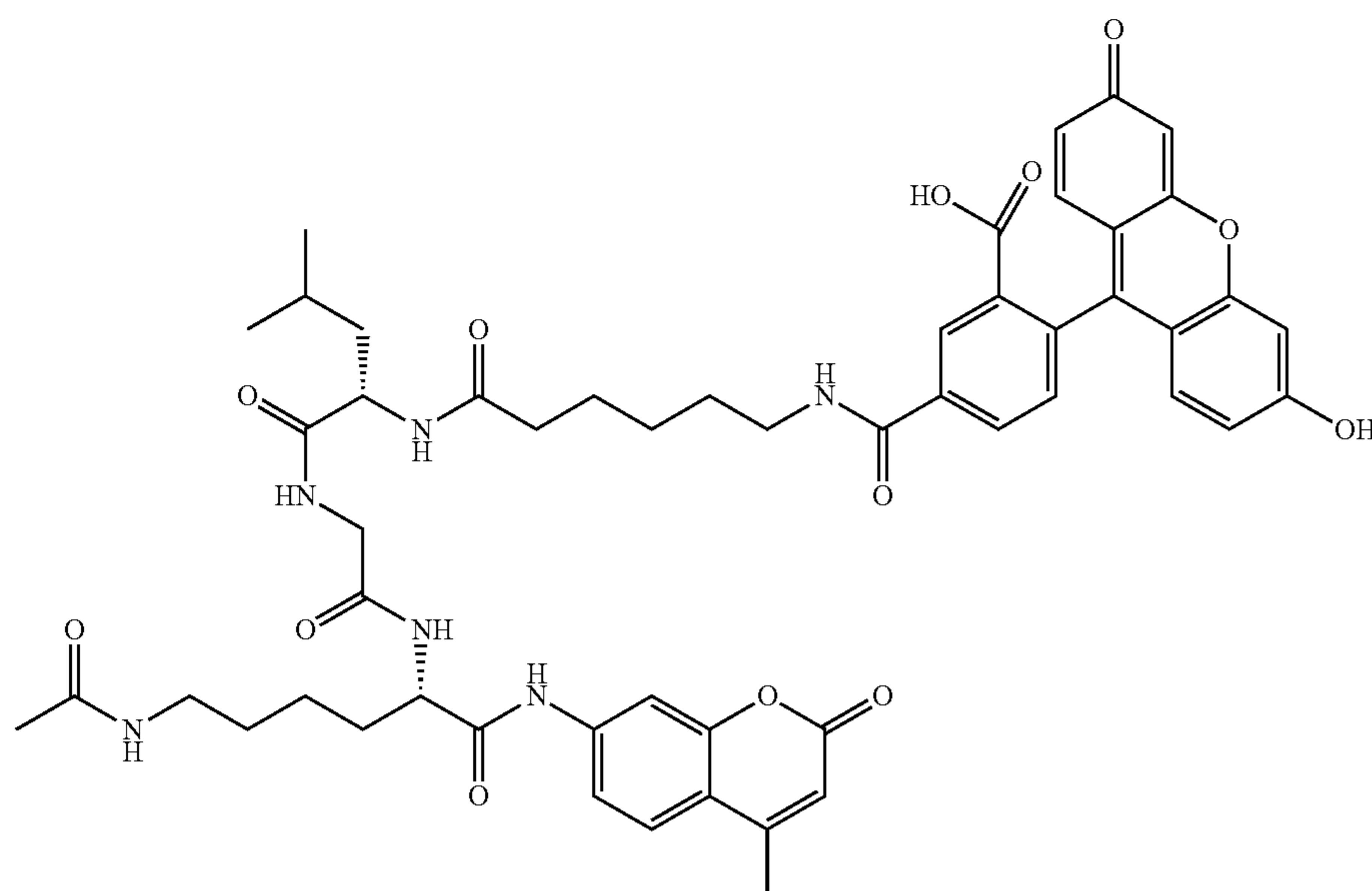
Substrate A
