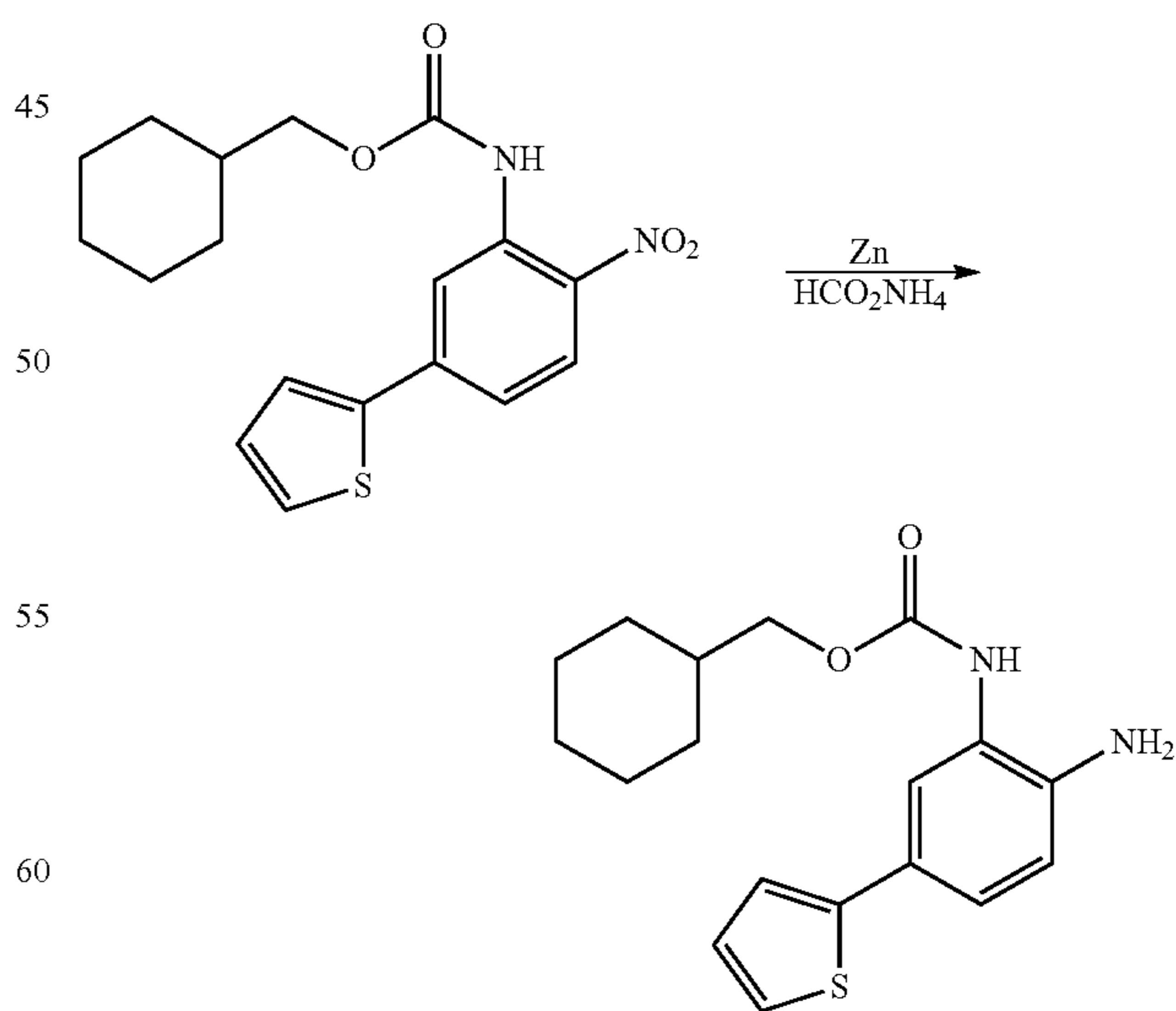
Scheme 11
