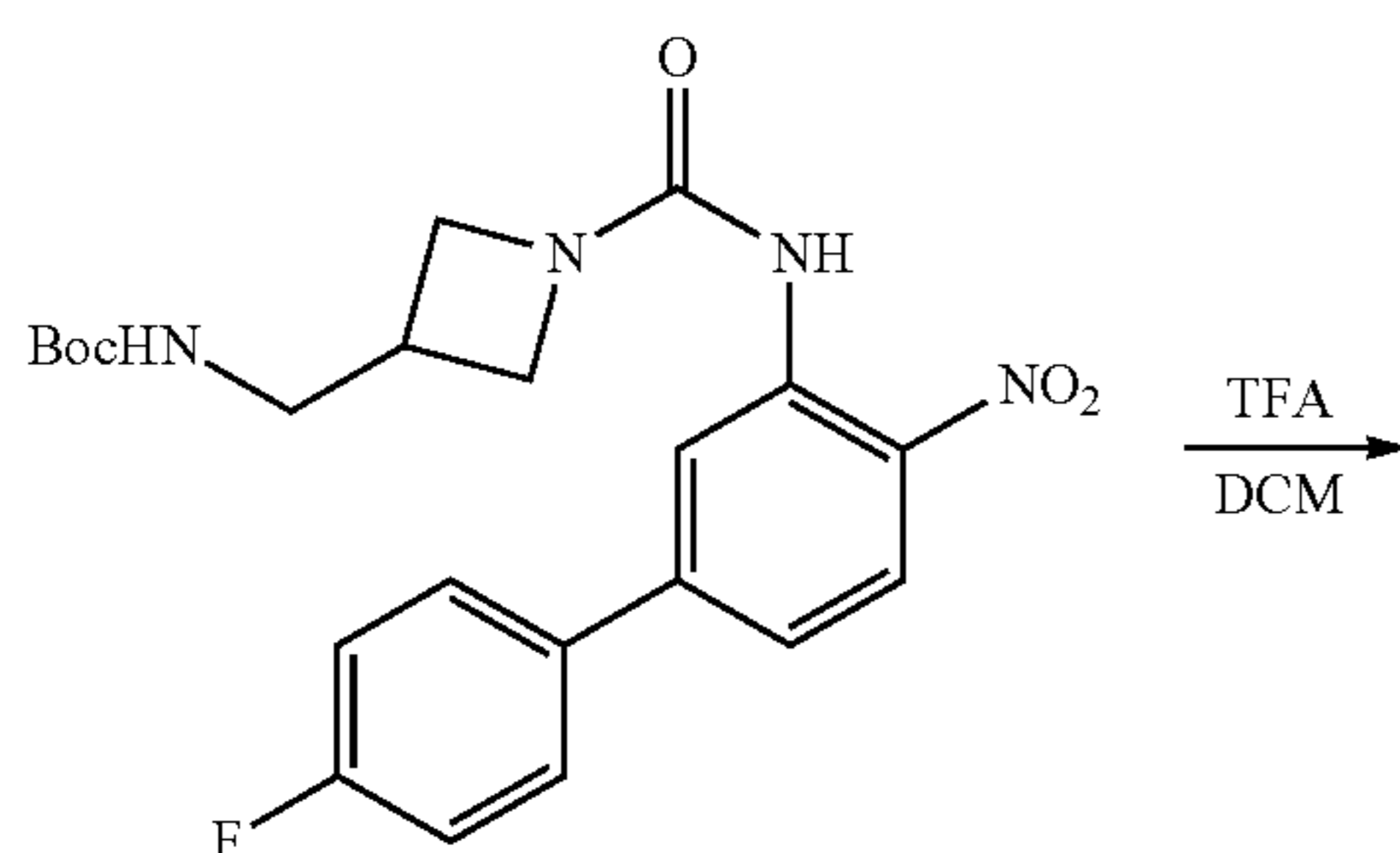
Scheme 46
