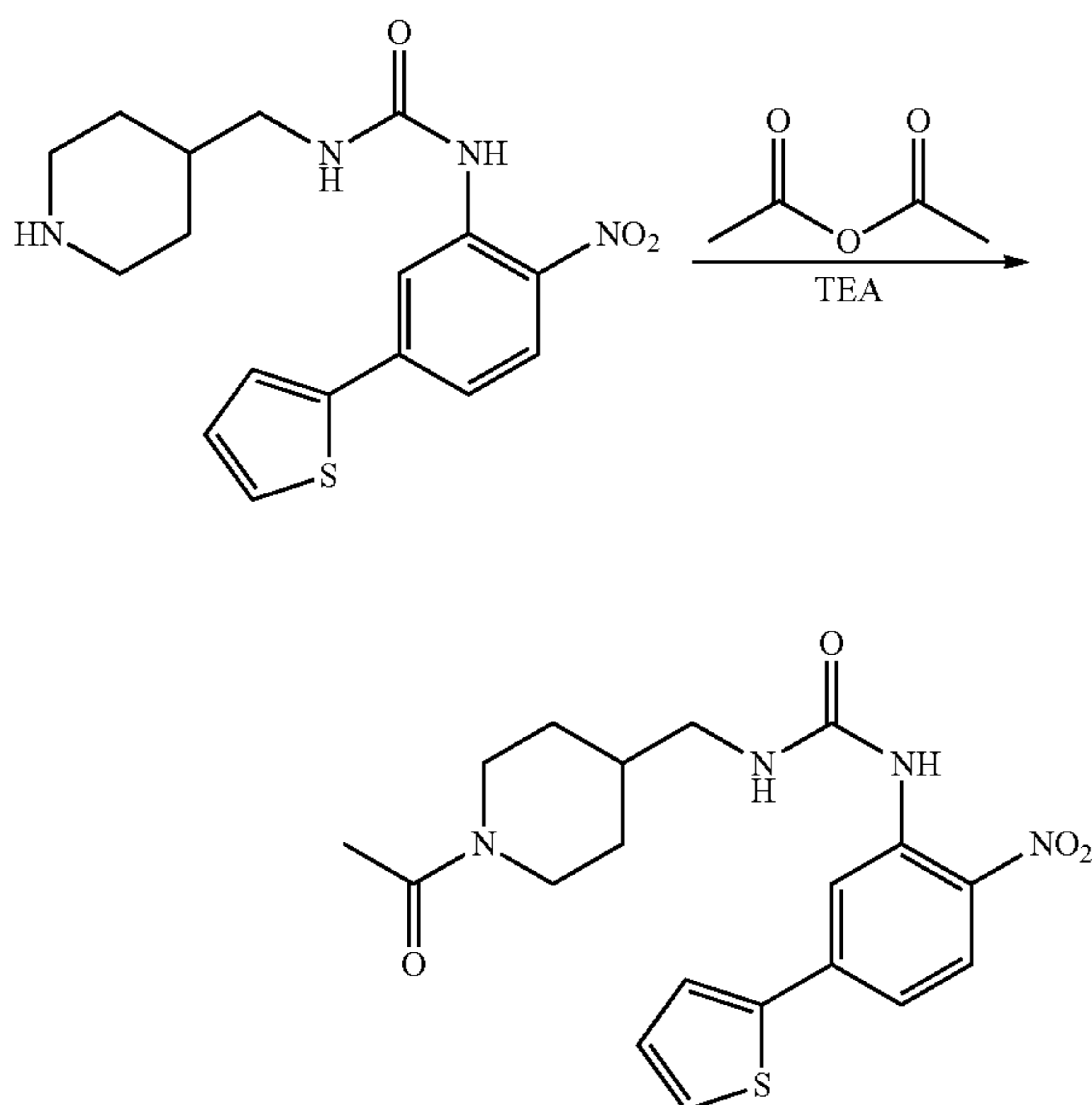
Scheme 29
