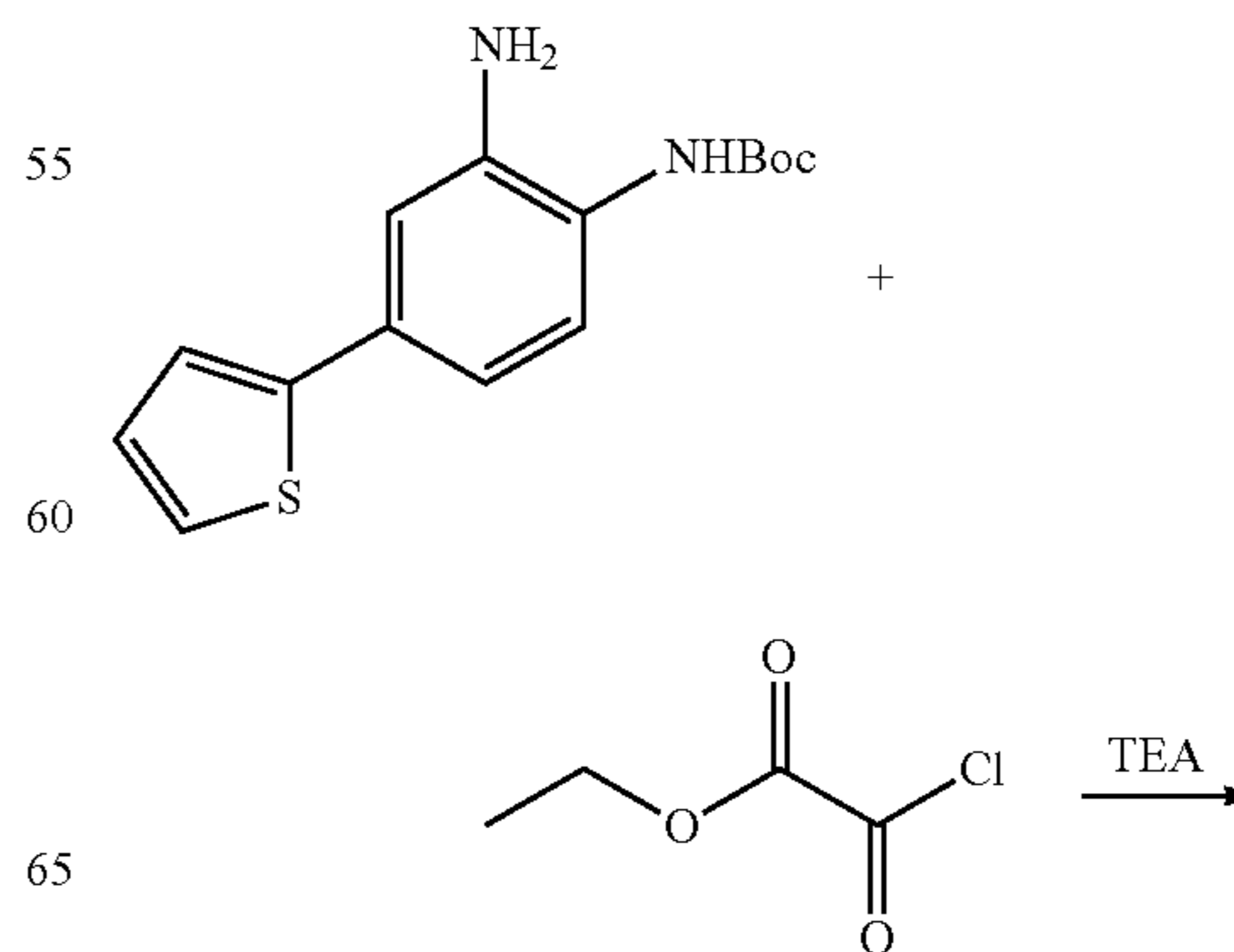
Scheme 42
