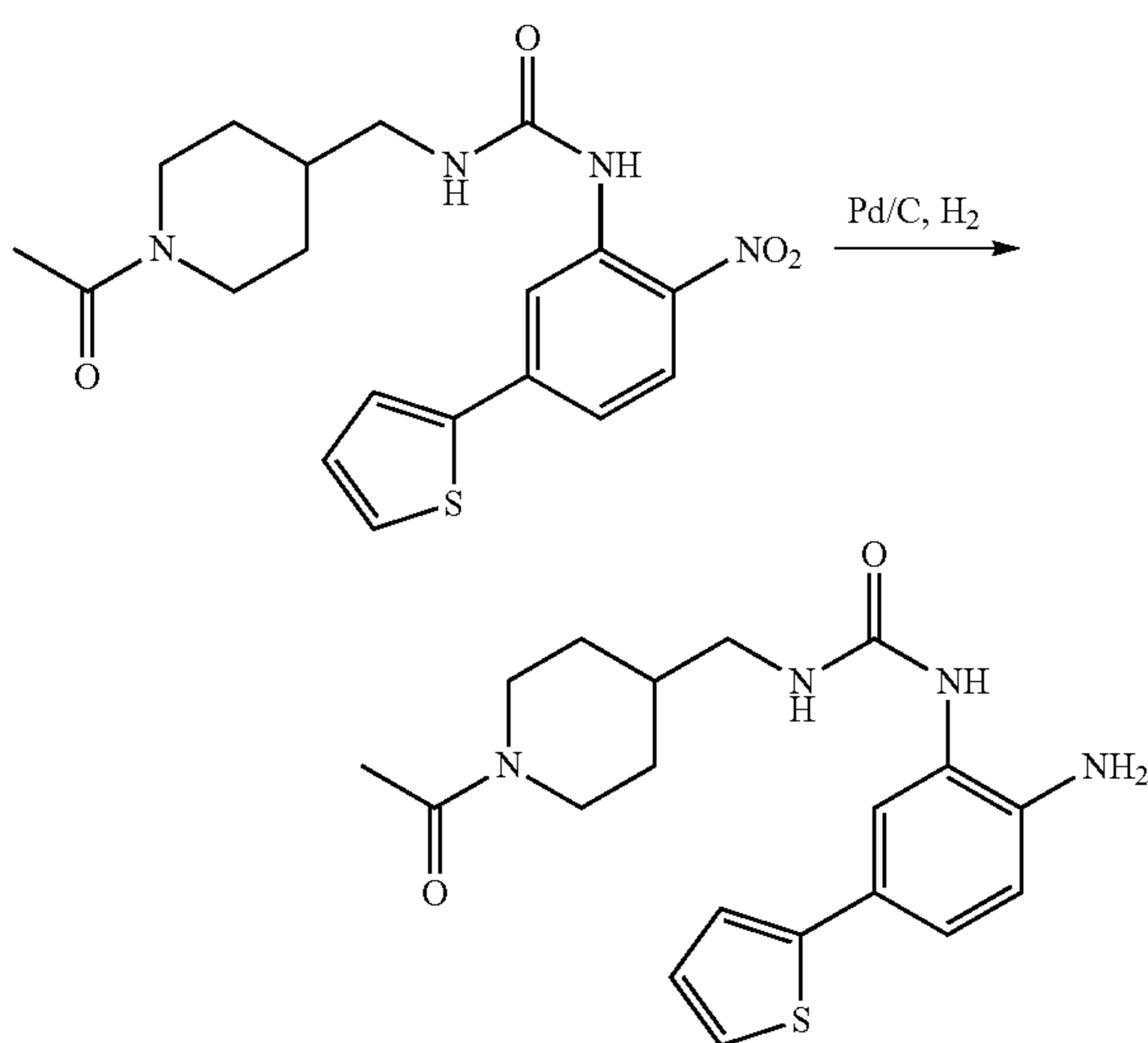
Scheme 30
