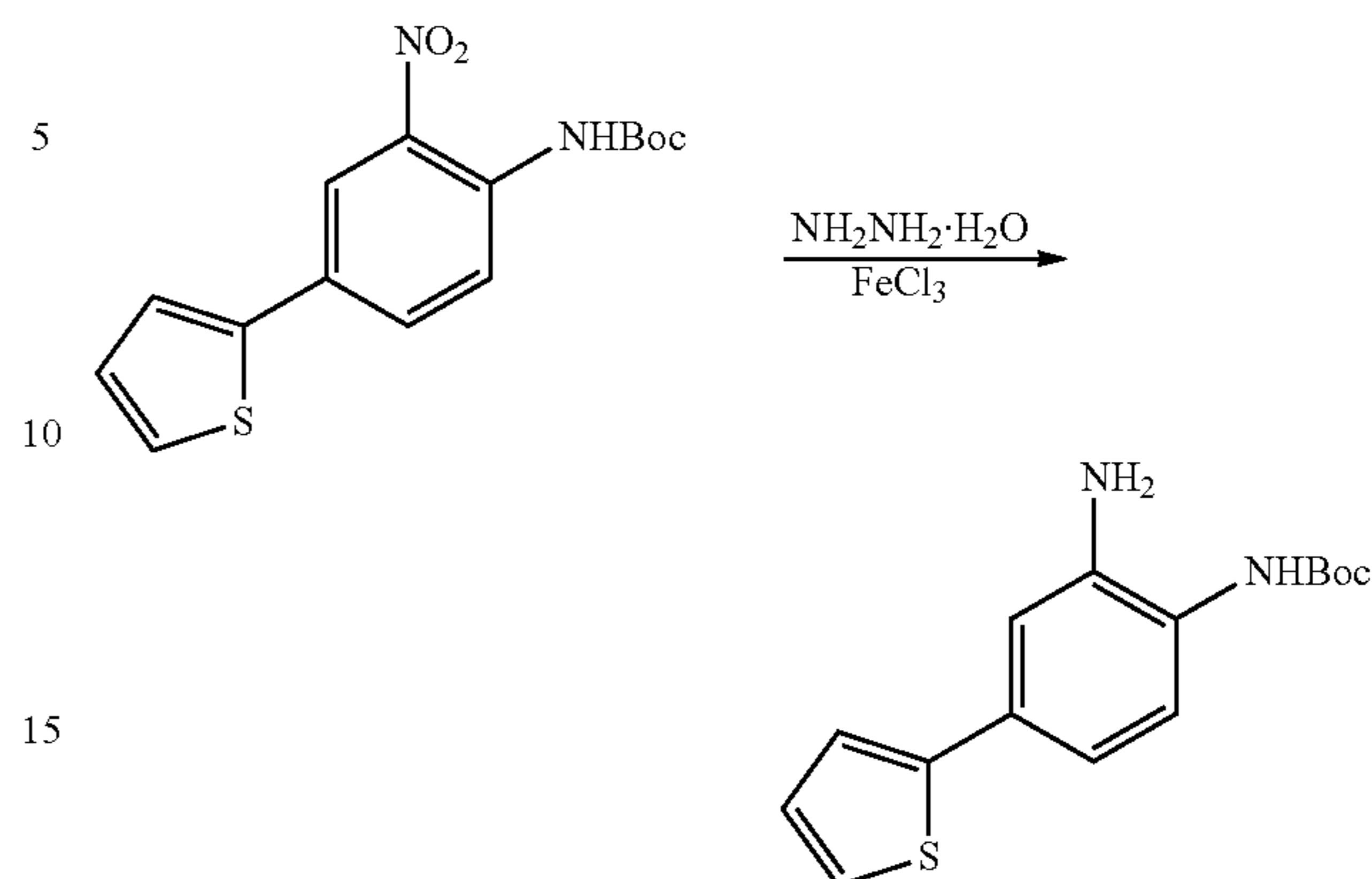
Scheme 4:
