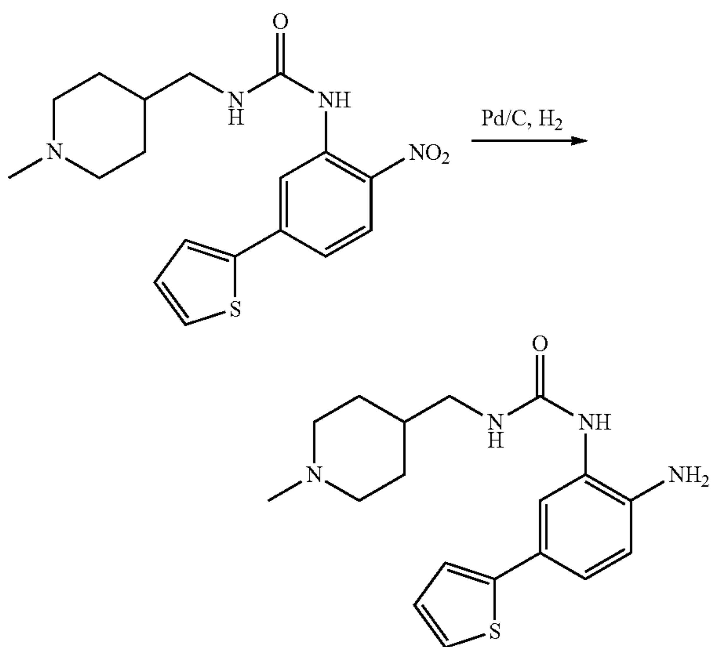
Scheme 32
