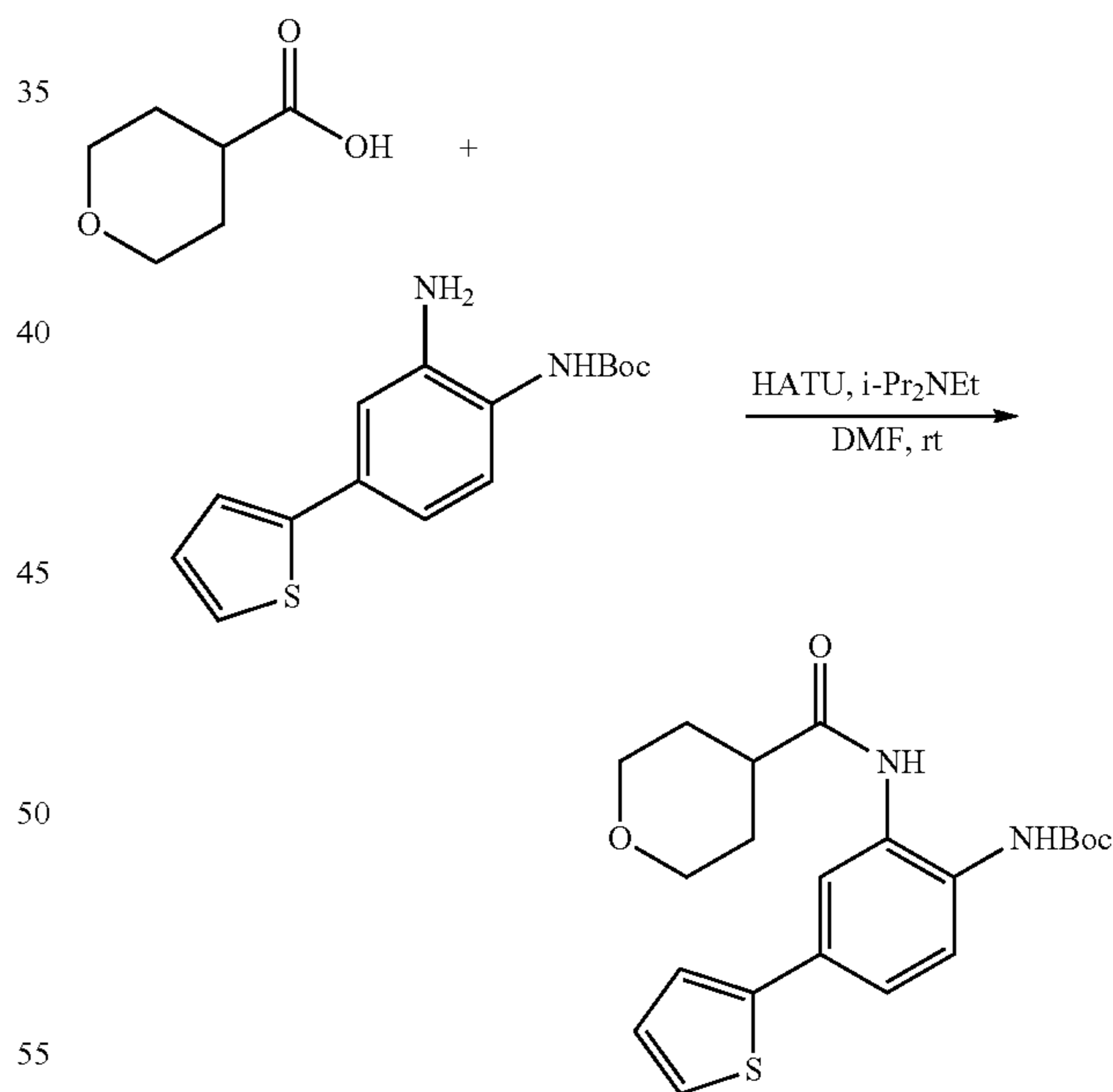
Scheme 5:
