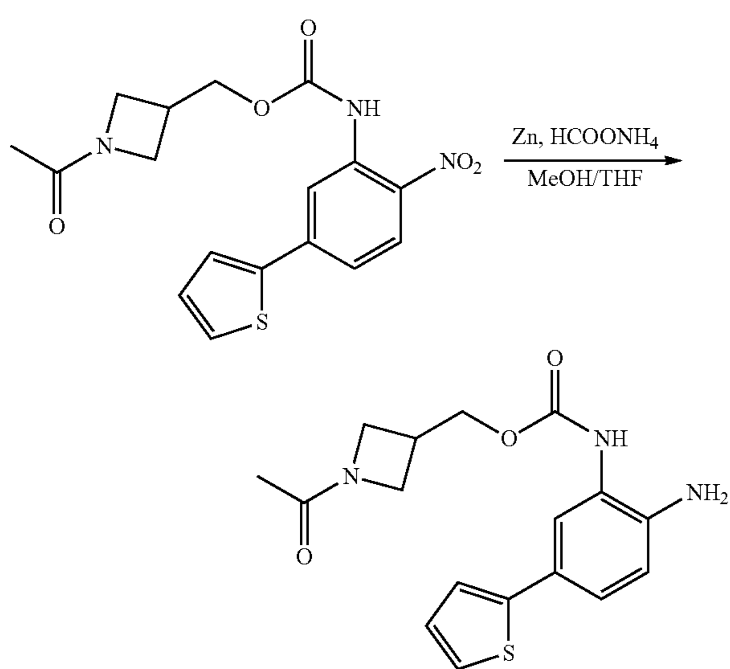
Scheme 22
