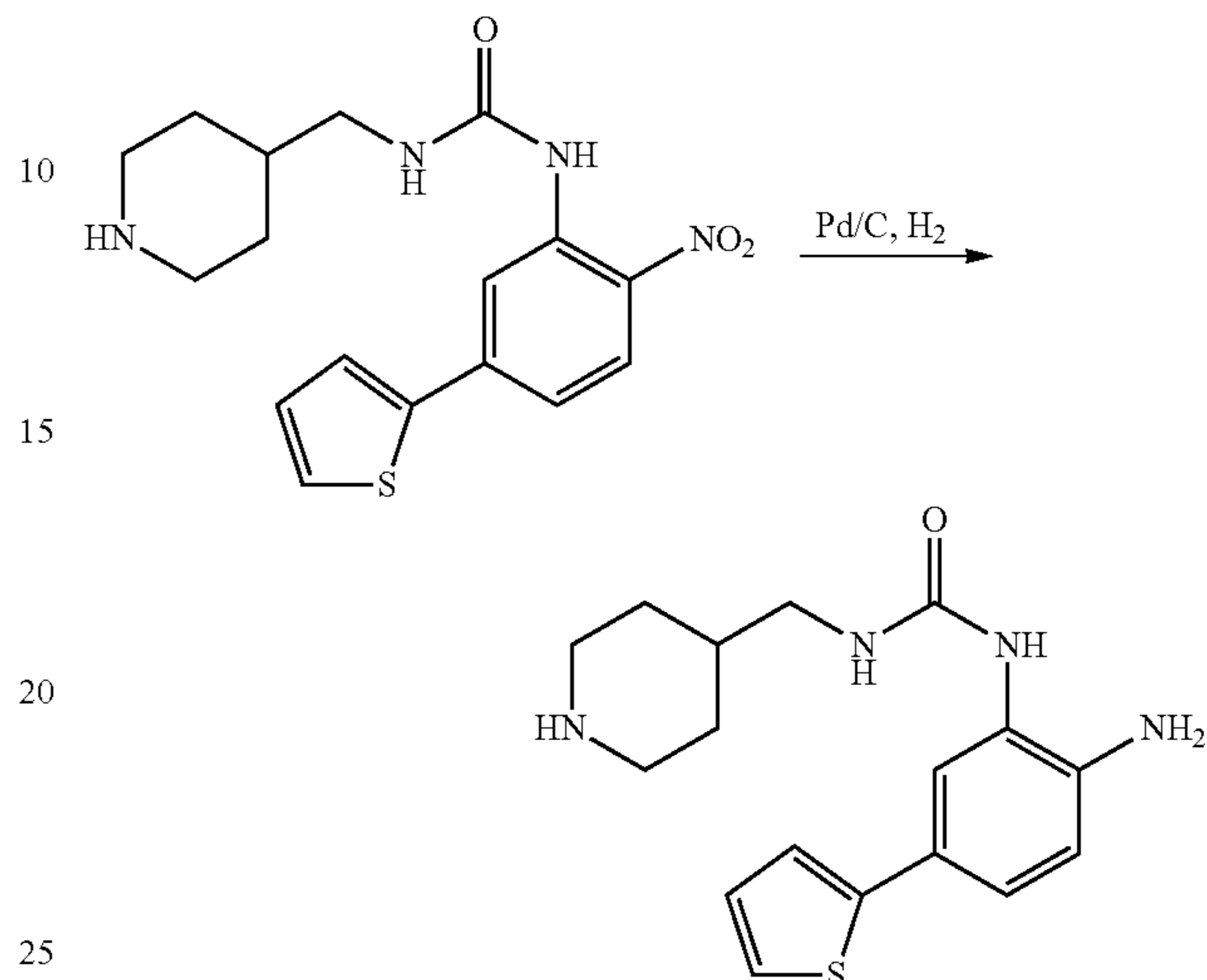
Scheme 33
