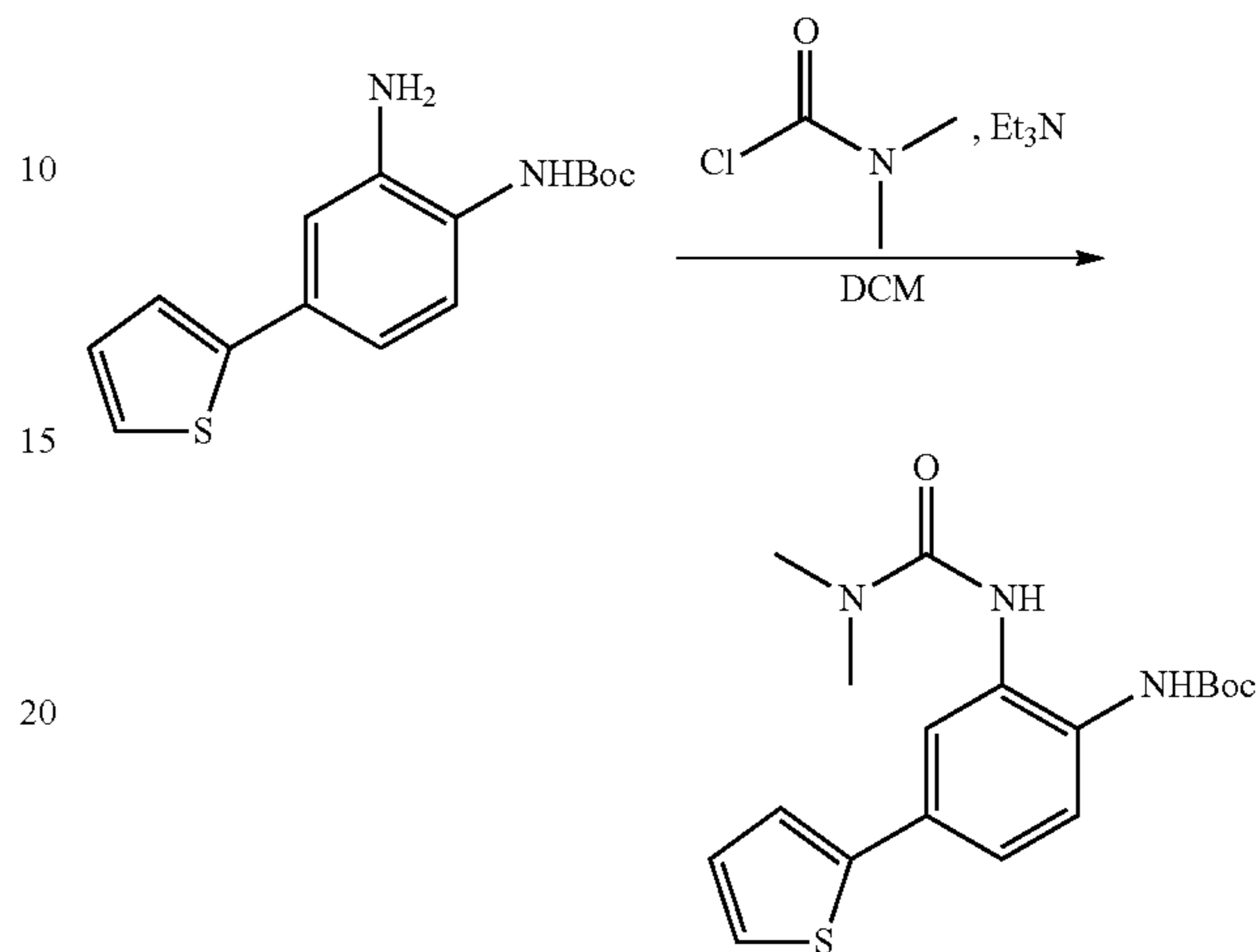
Scheme 34
