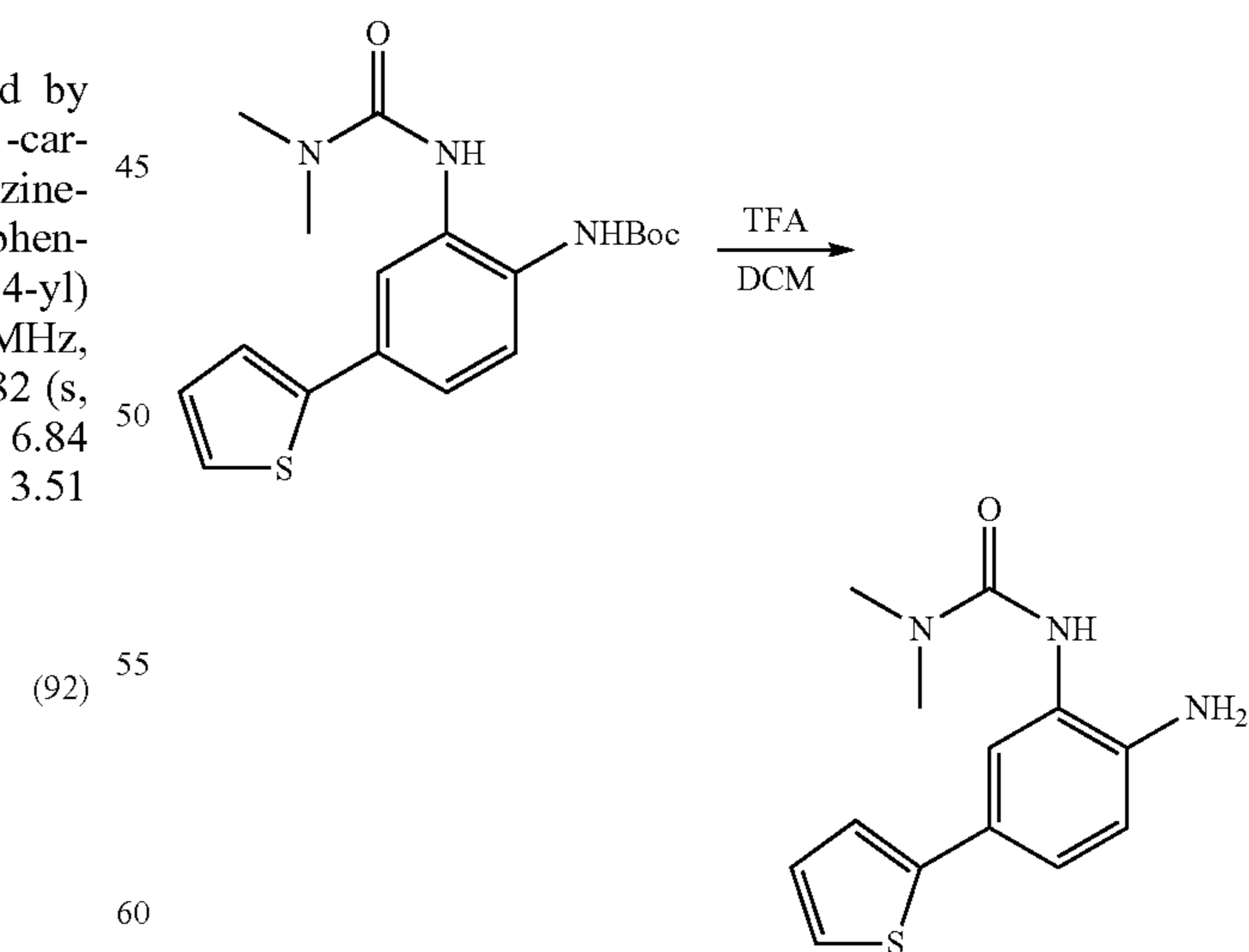
Scheme 35
