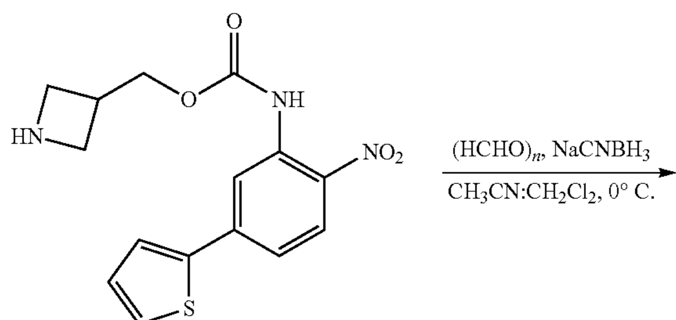
Scheme 19
