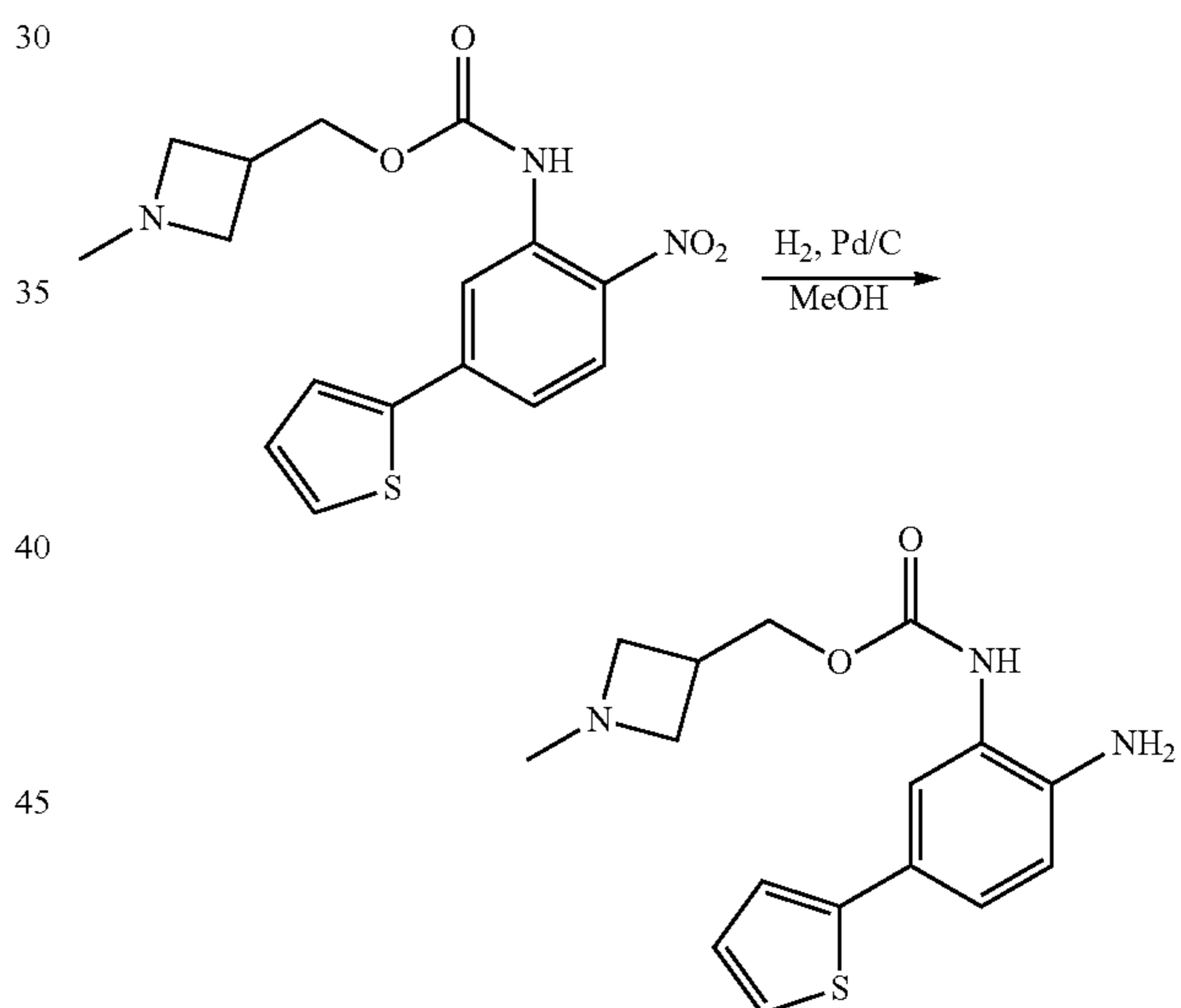
Scheme 20
