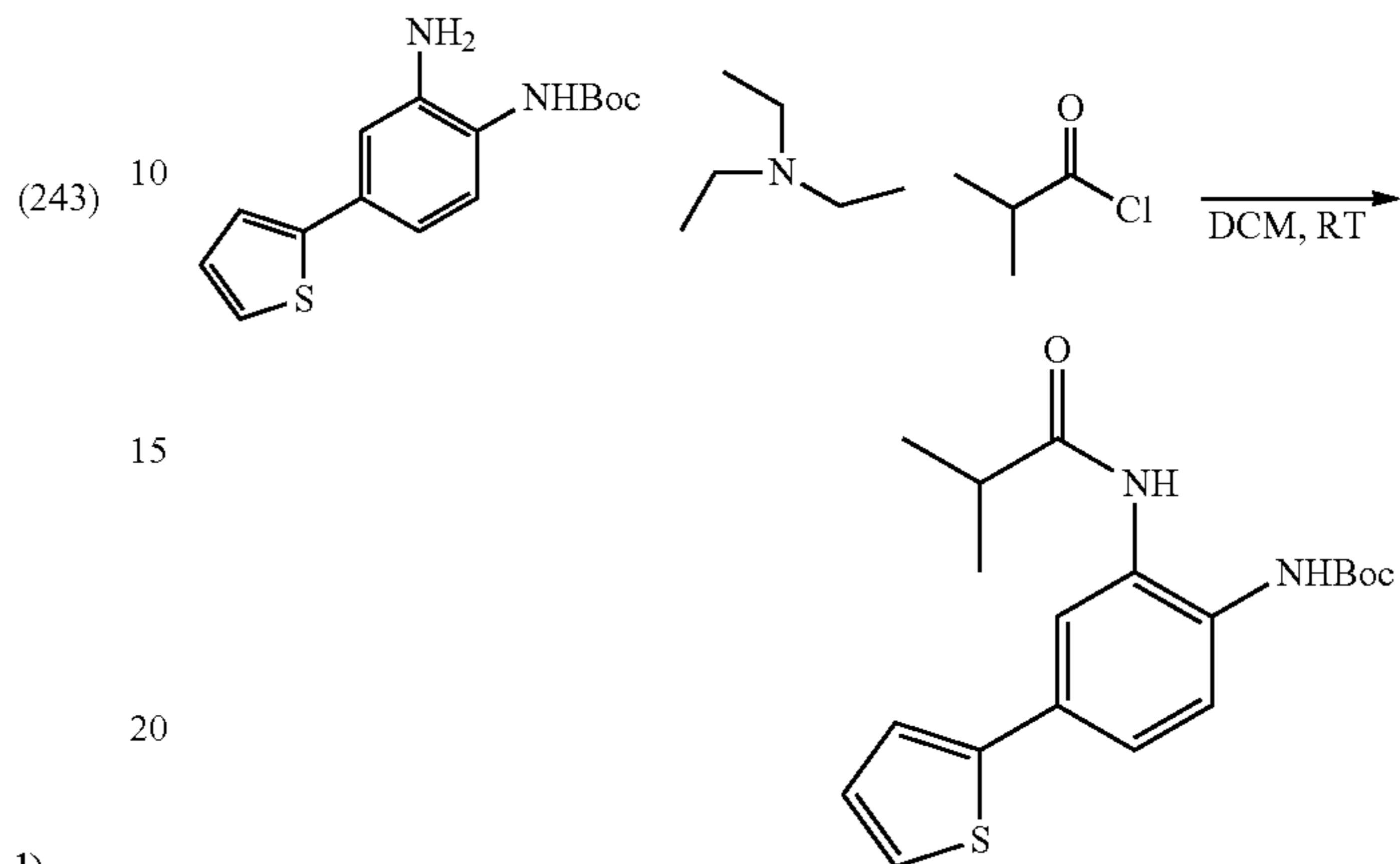
Scheme 6A
