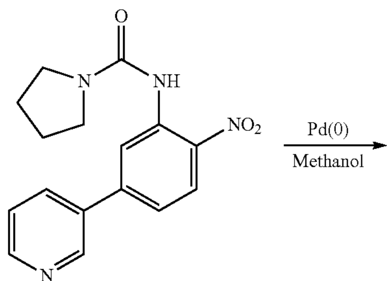
Scheme 38
