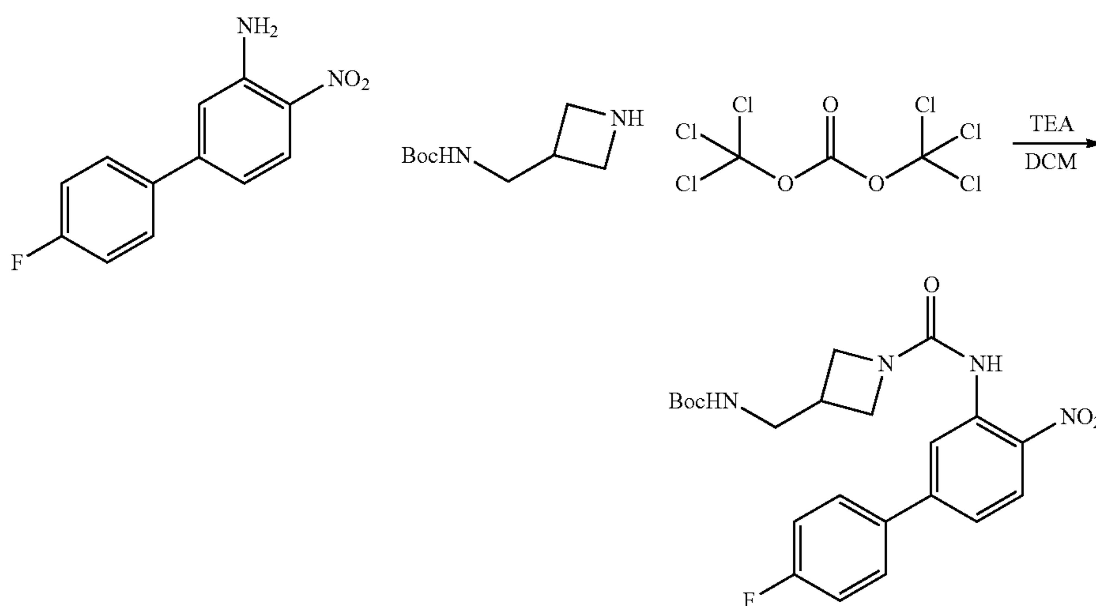
Scheme 45
