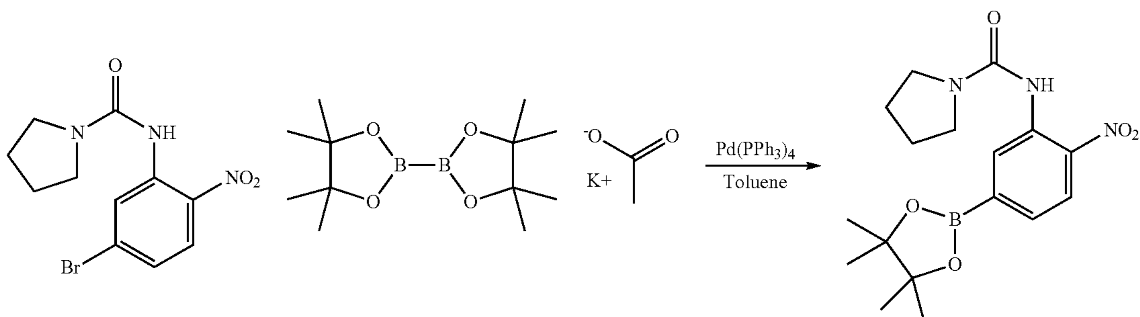
Scheme 39
