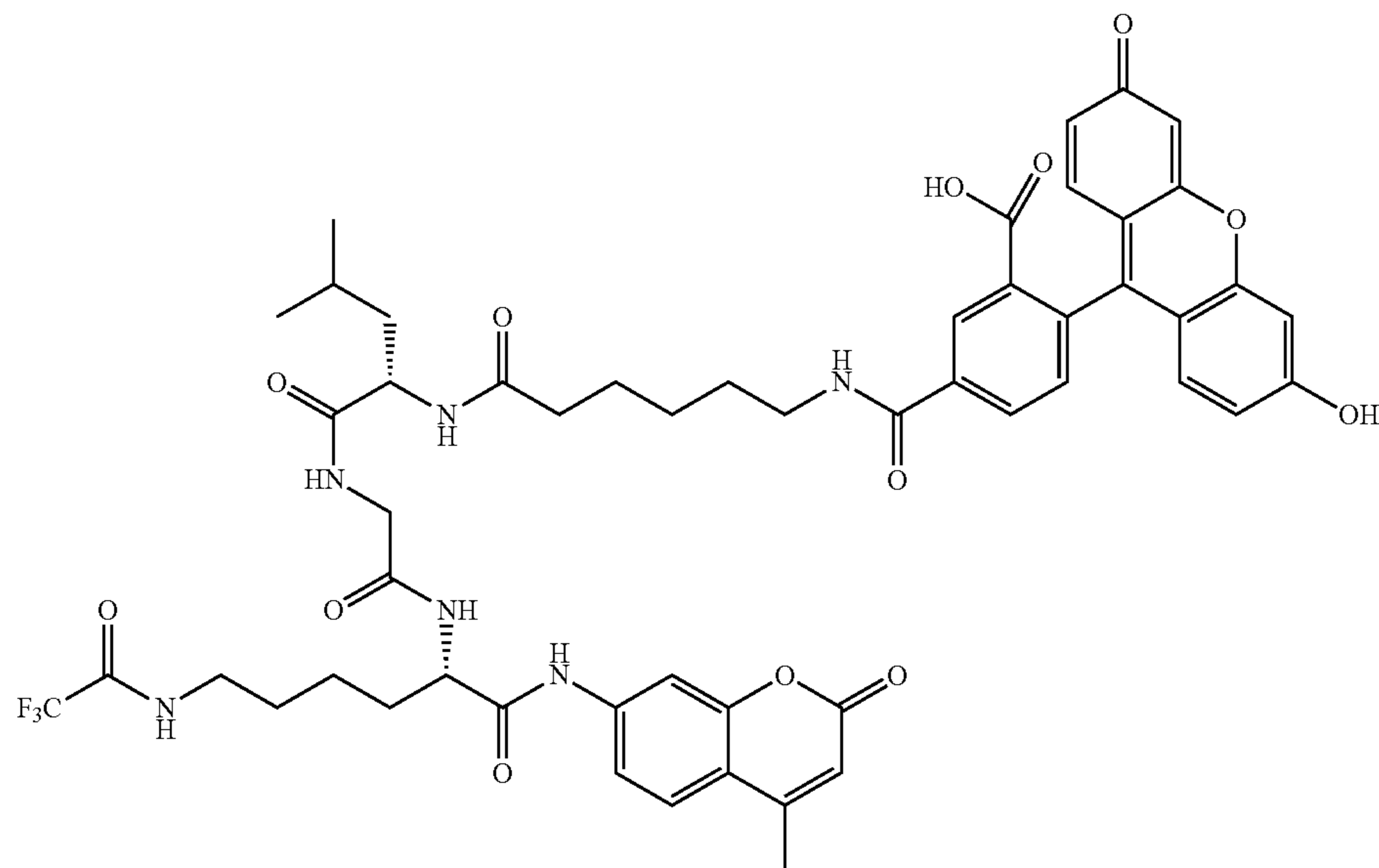
Substrate B
