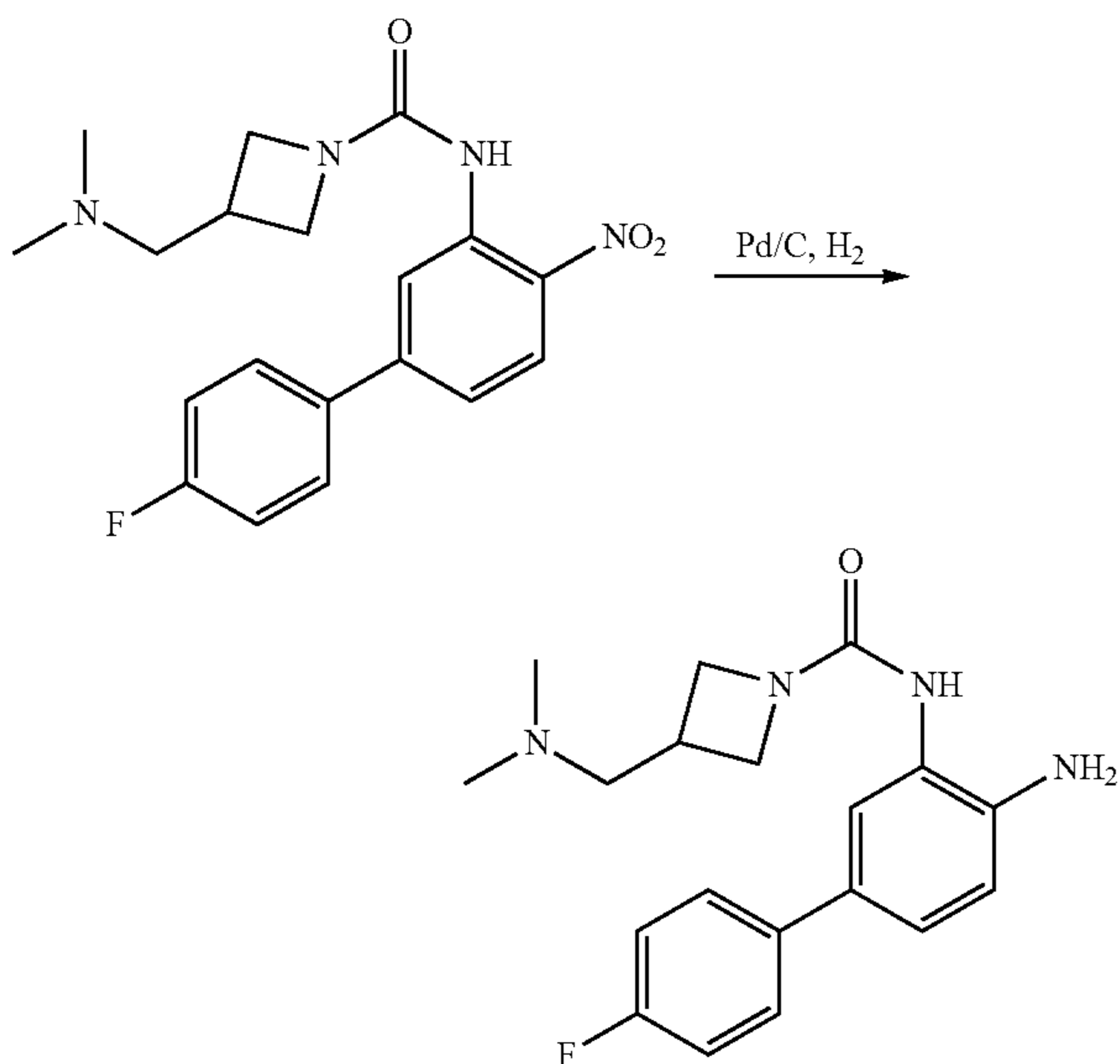
Scheme 48
