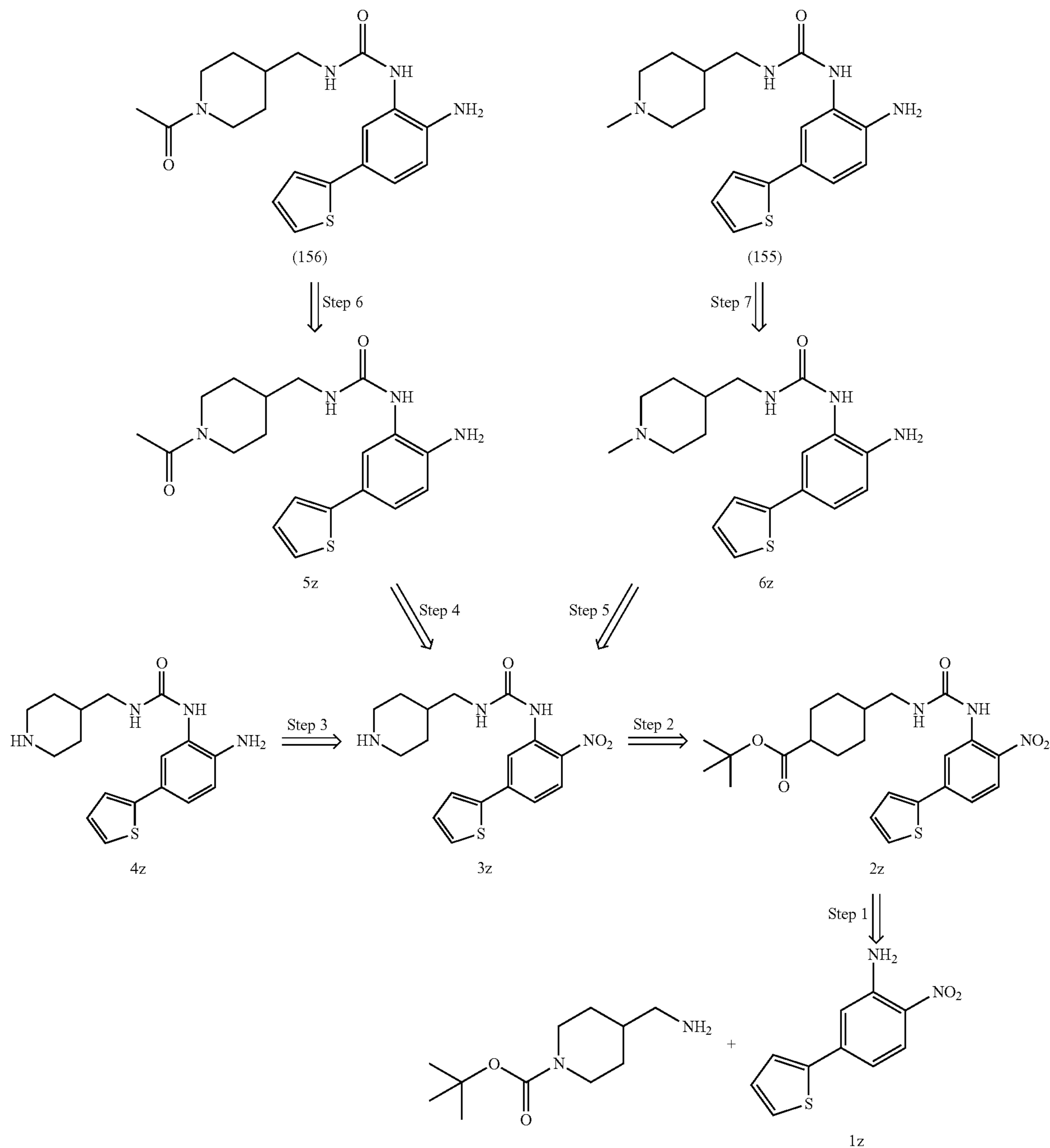
Scheme 3A
