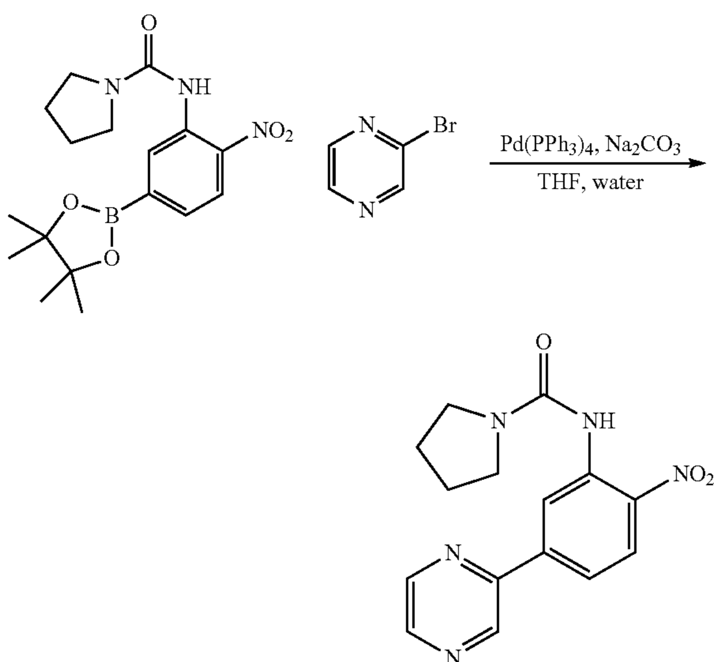
Scheme 40
