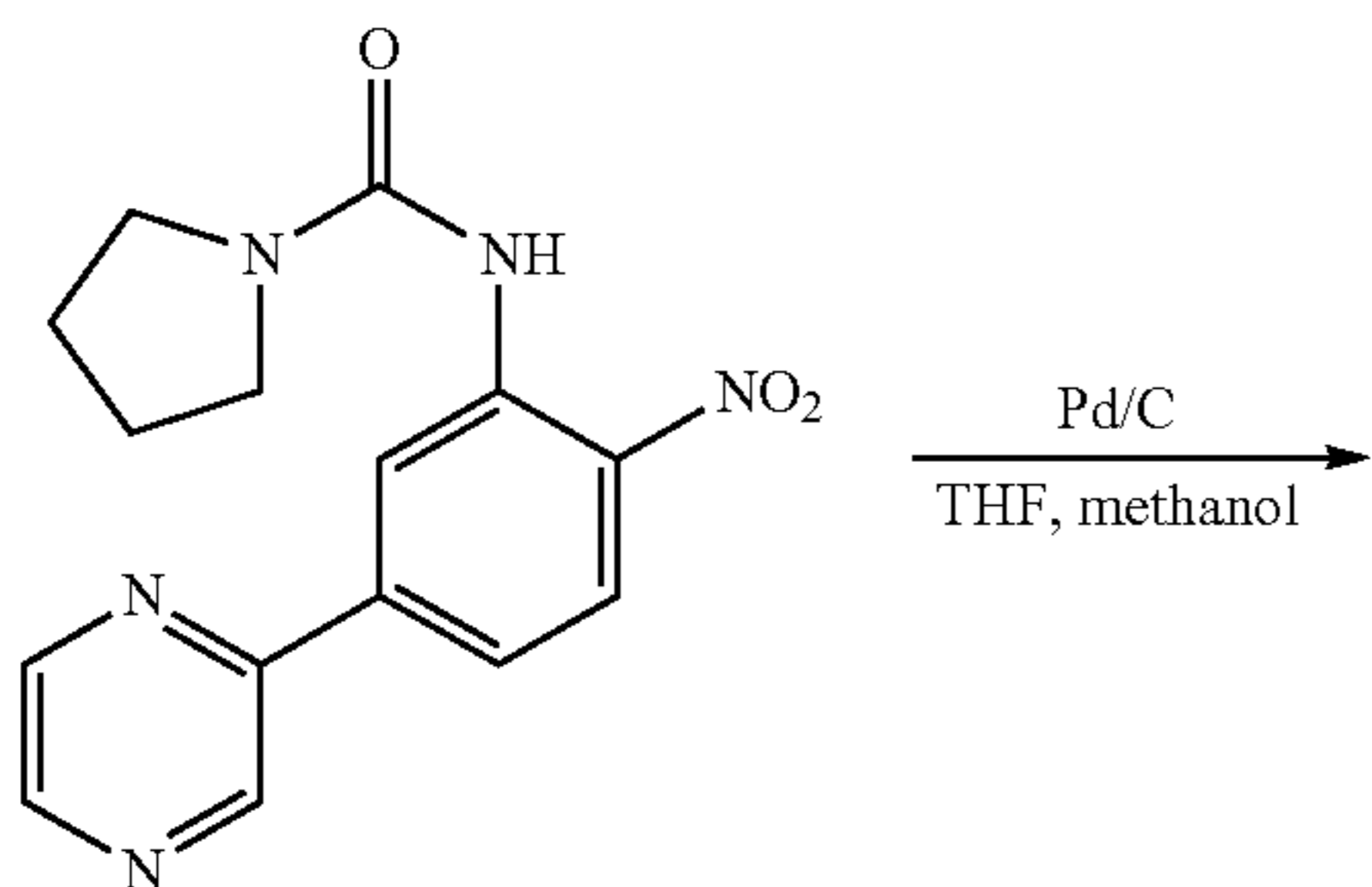
Scheme 41
