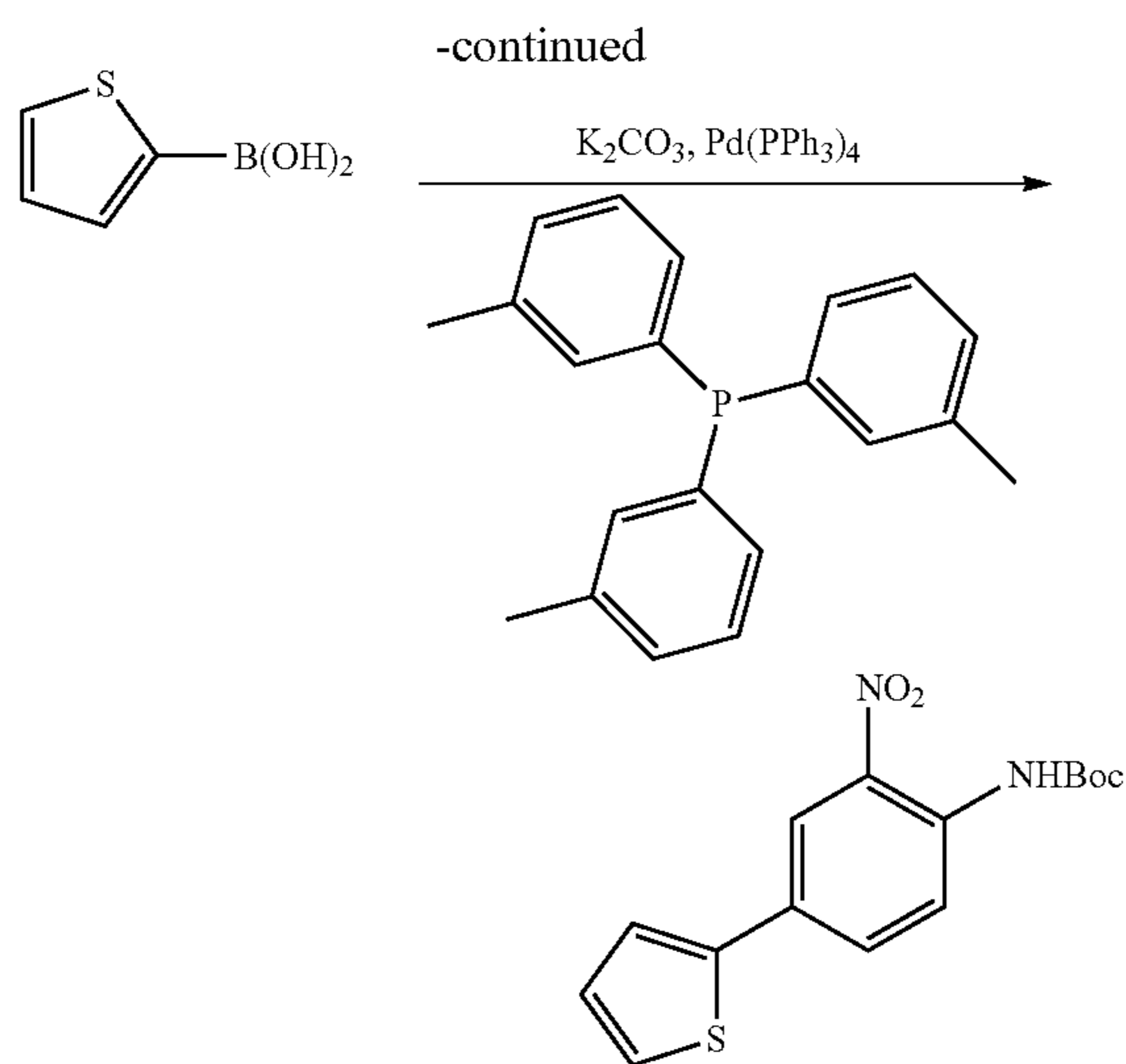
Scheme 4:
