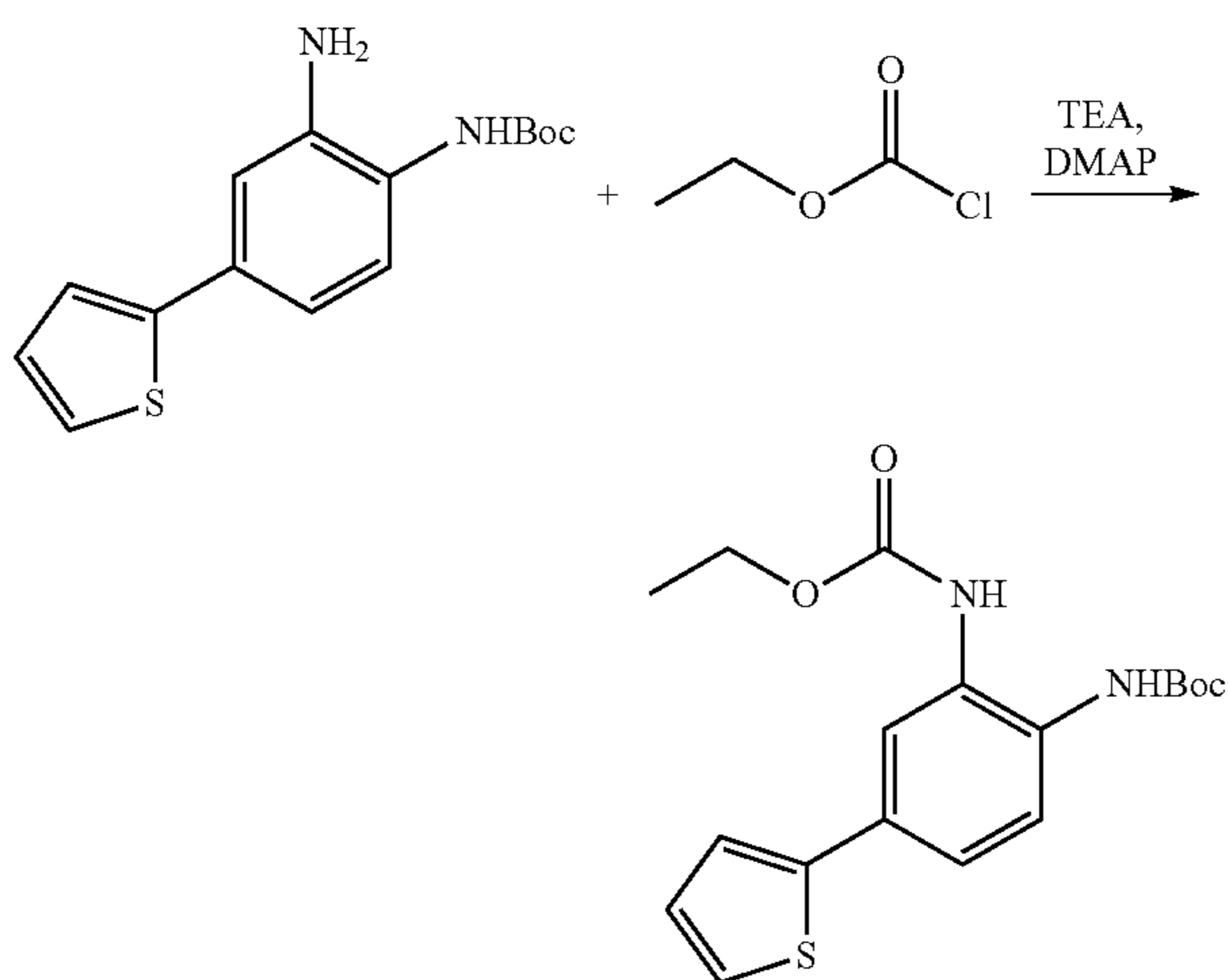
Scheme 16
