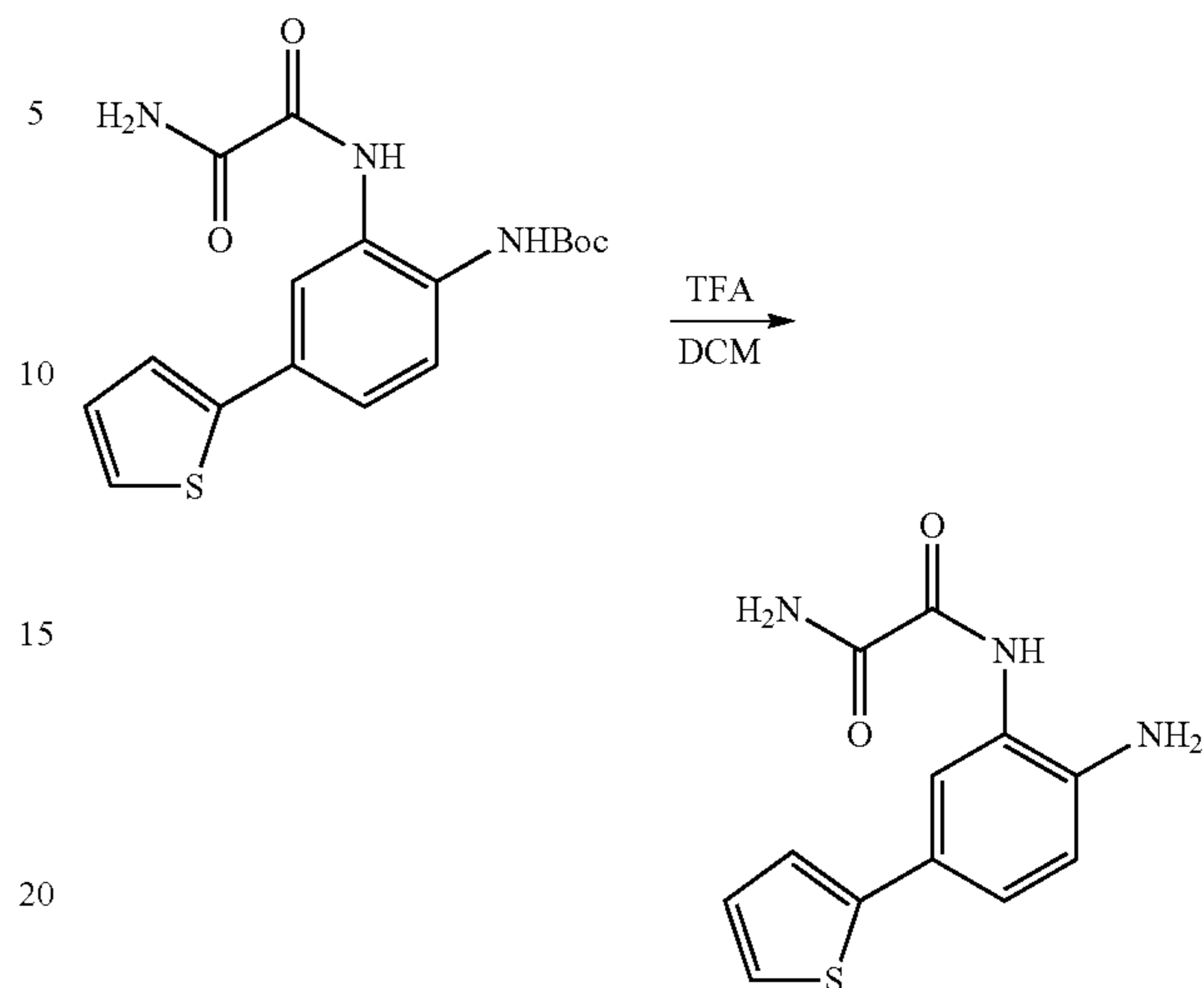
Scheme 44
