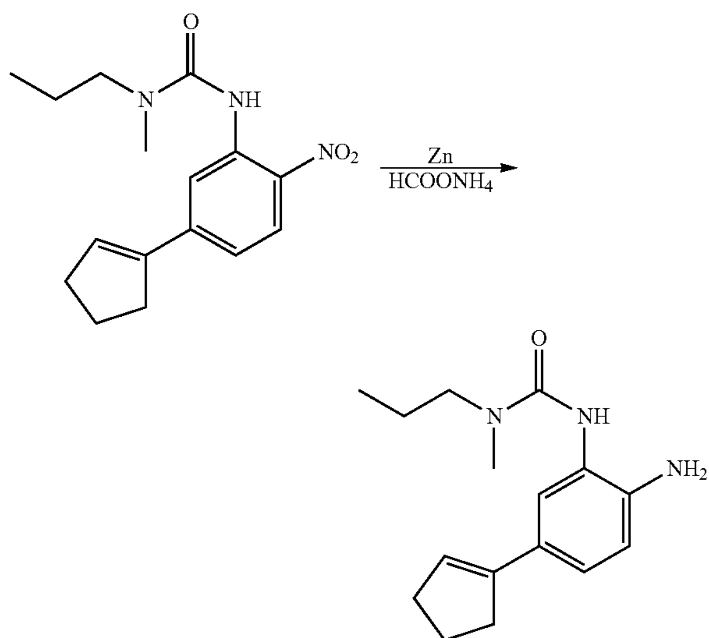
Scheme 26
