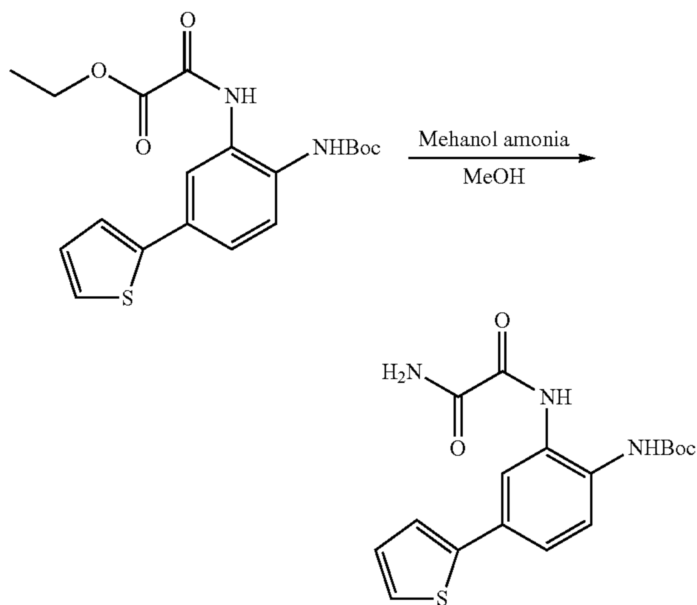
Scheme 43
