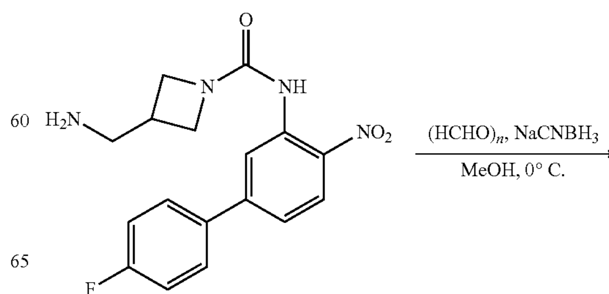
Scheme 47
