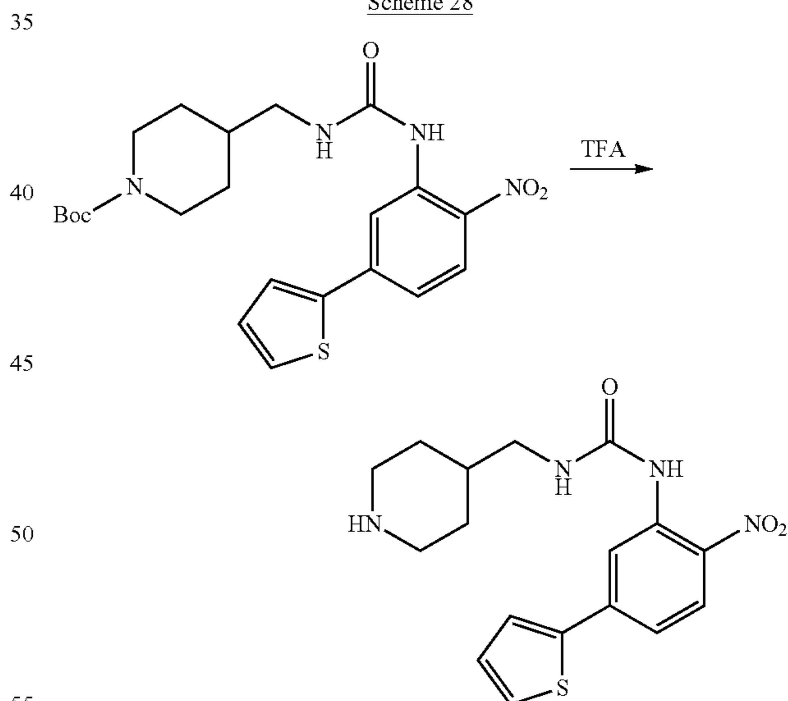
Scheme 28
