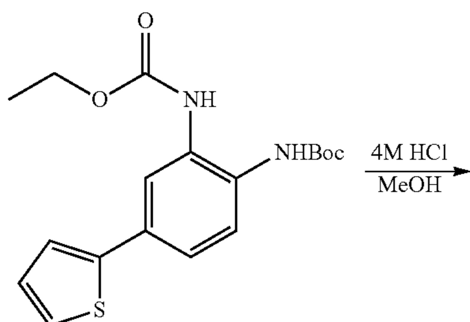
Scheme 17
