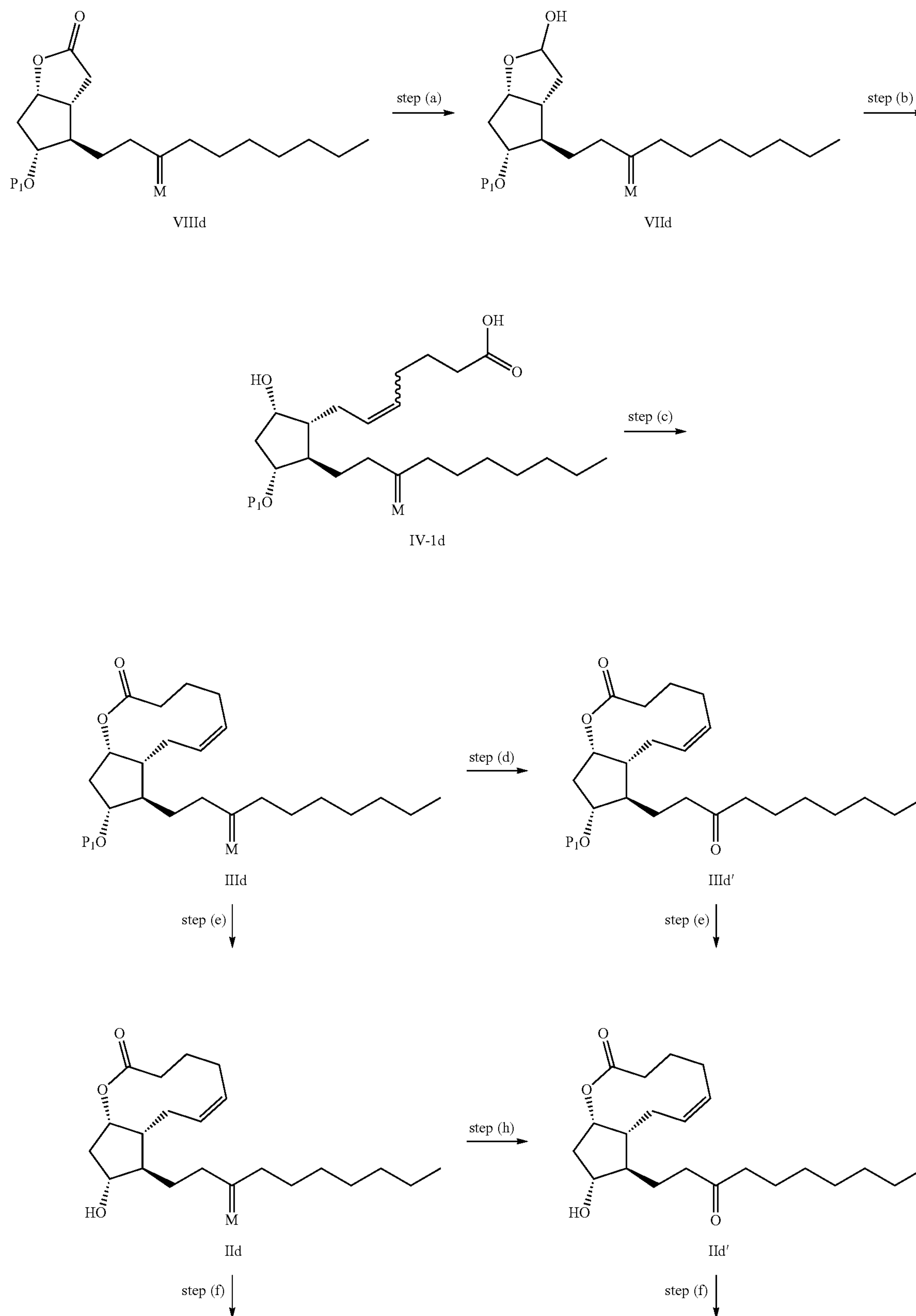
Scheme 7
