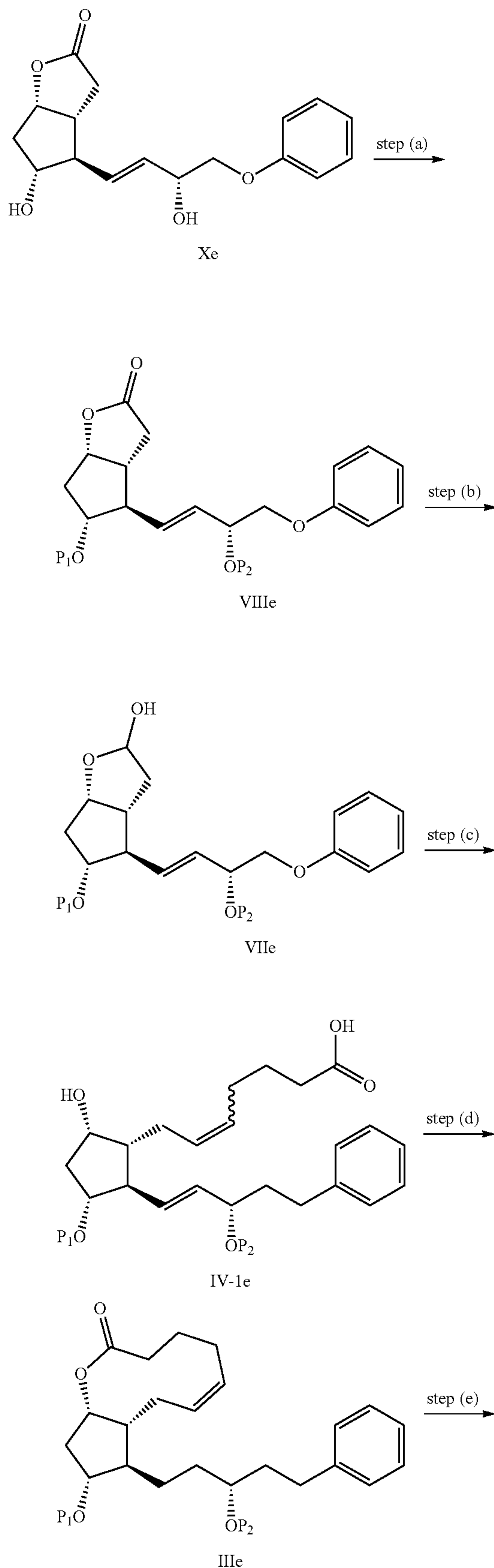
Scheme 9
