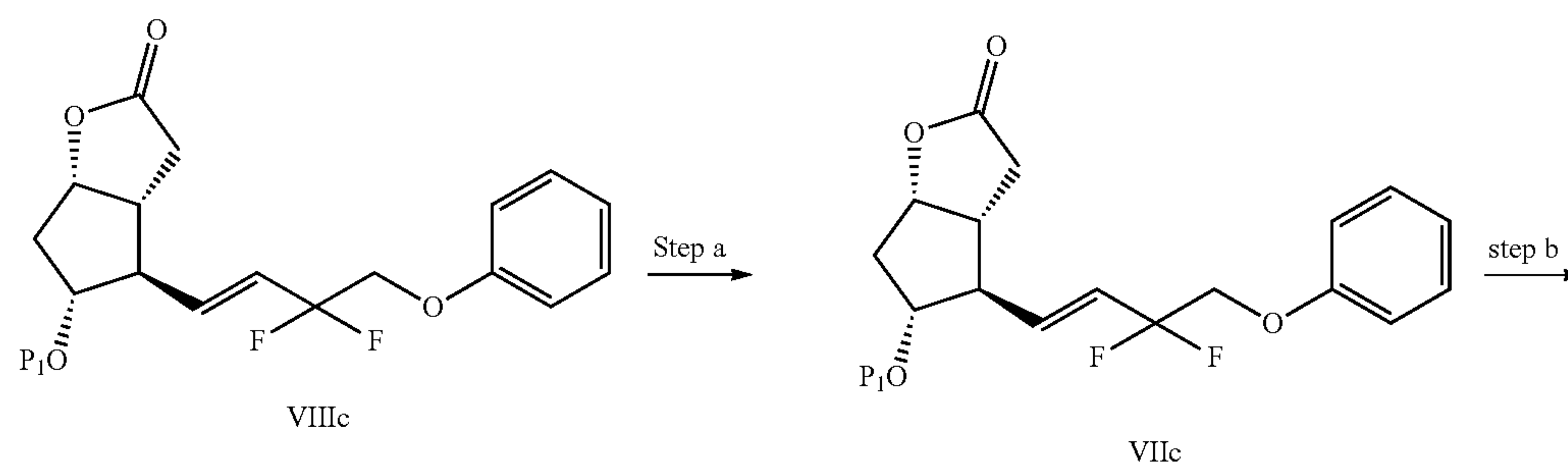
Scheme 6
