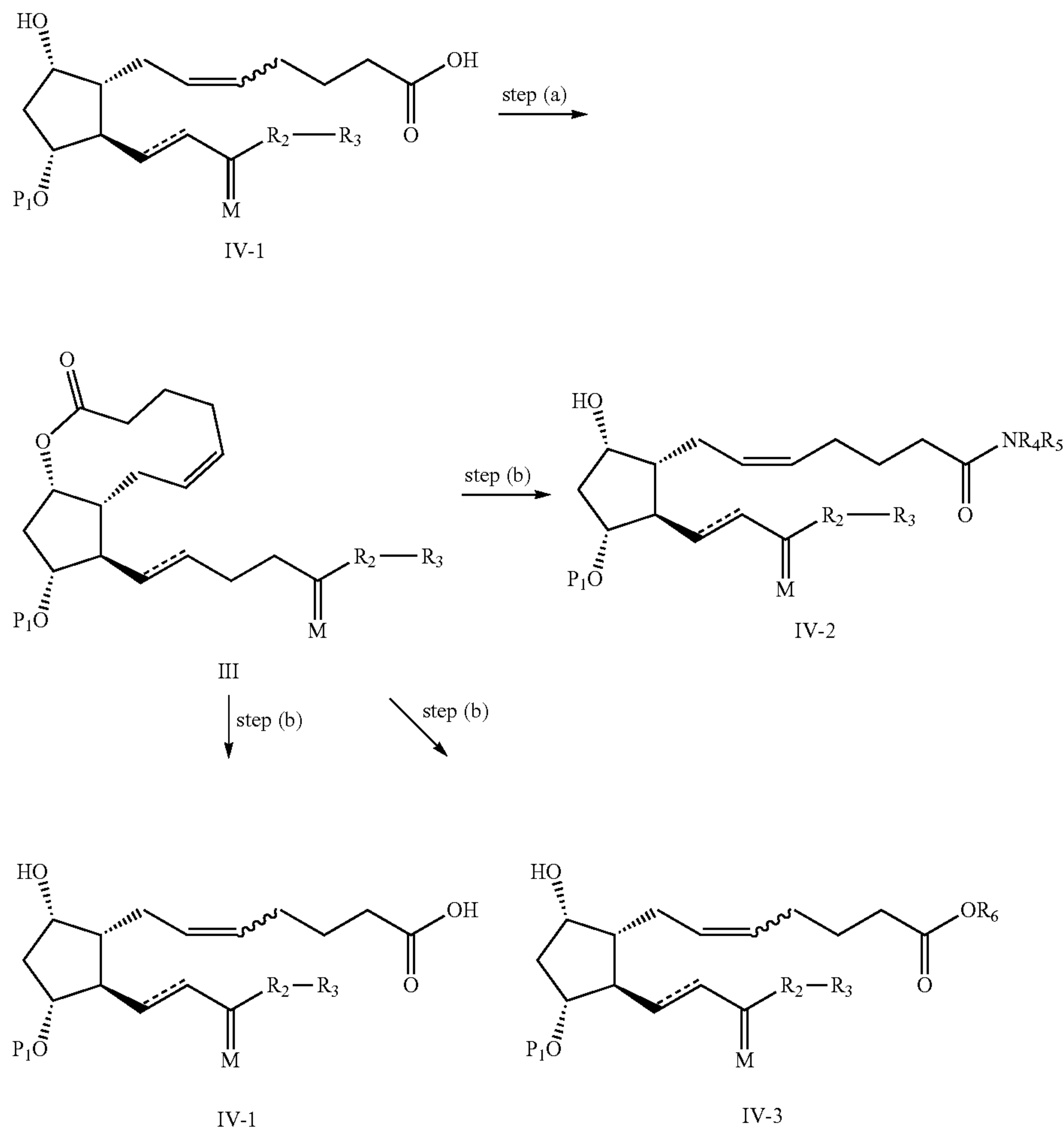
Scheme 8
