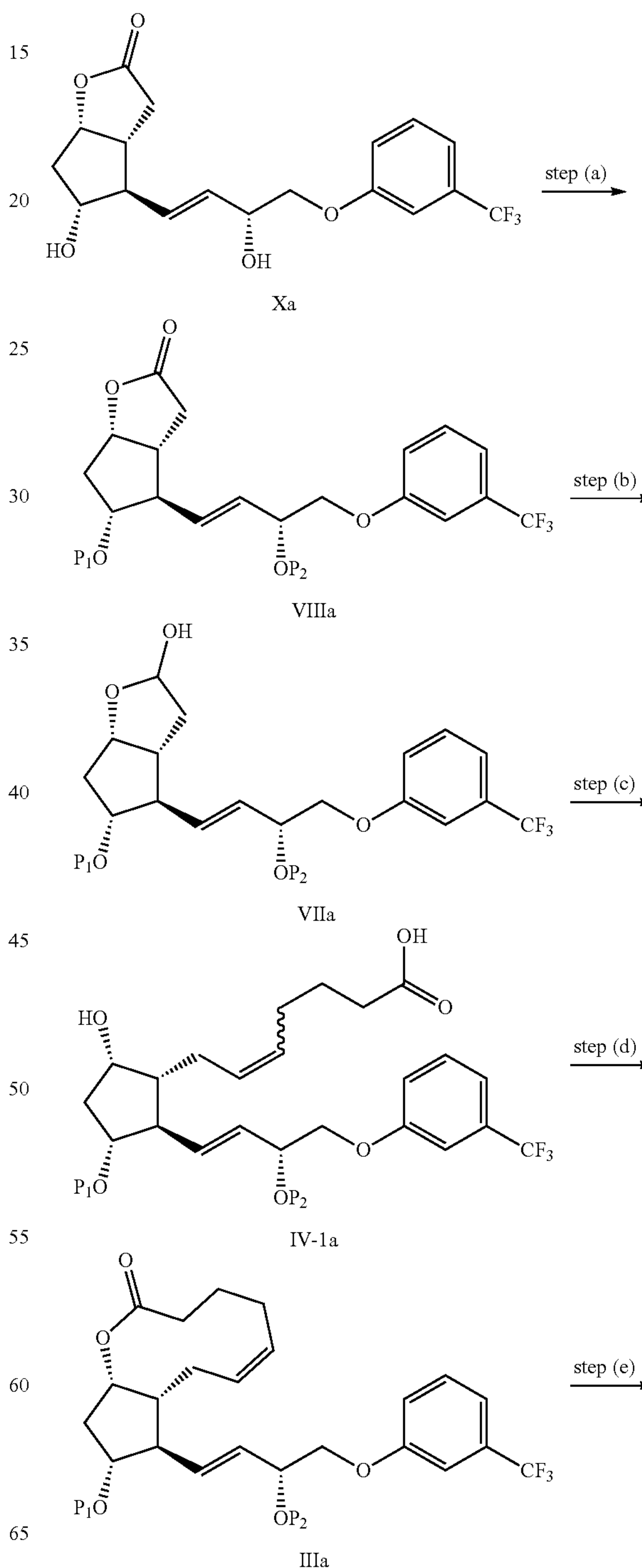
Scheme 4
