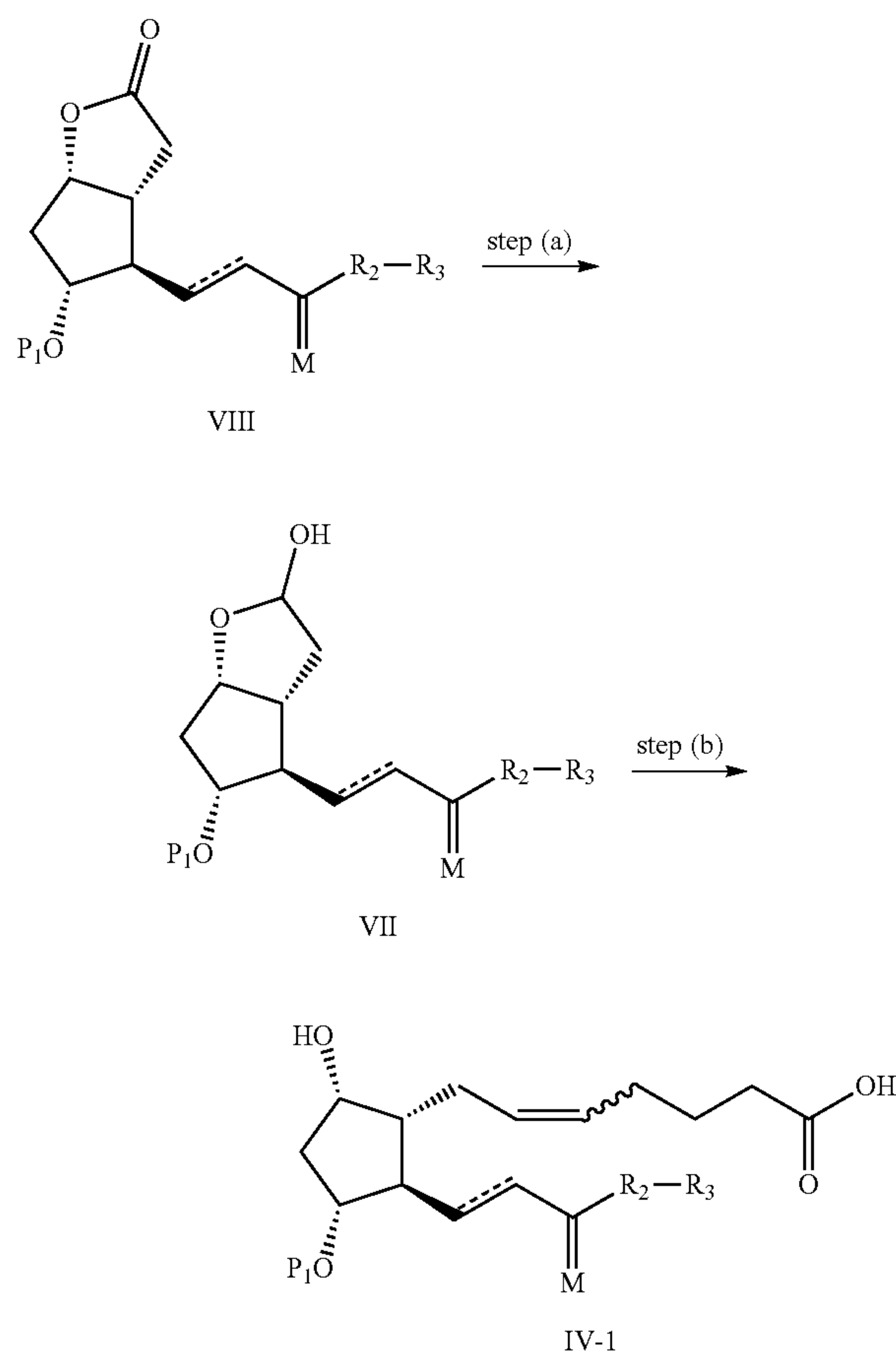
Scheme 1
