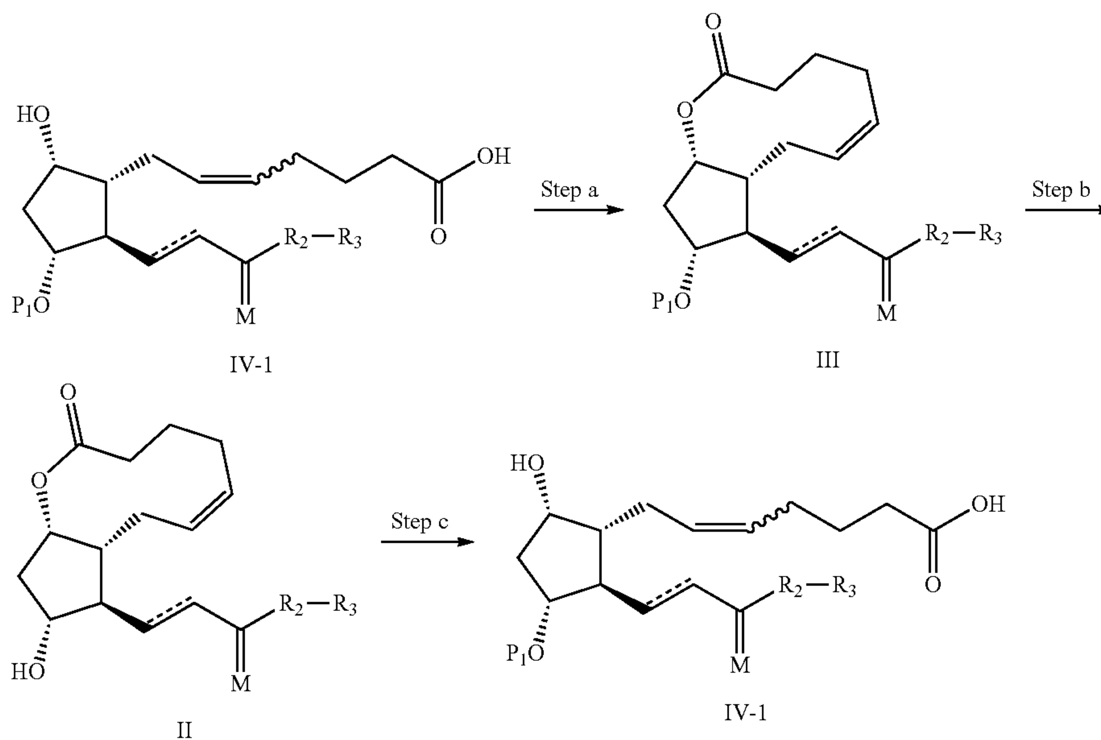
Scheme 3
