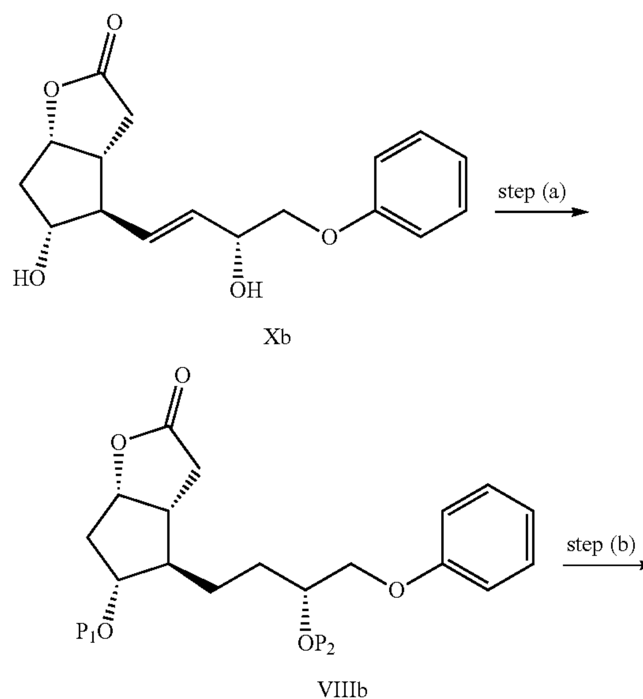
Scheme 5
