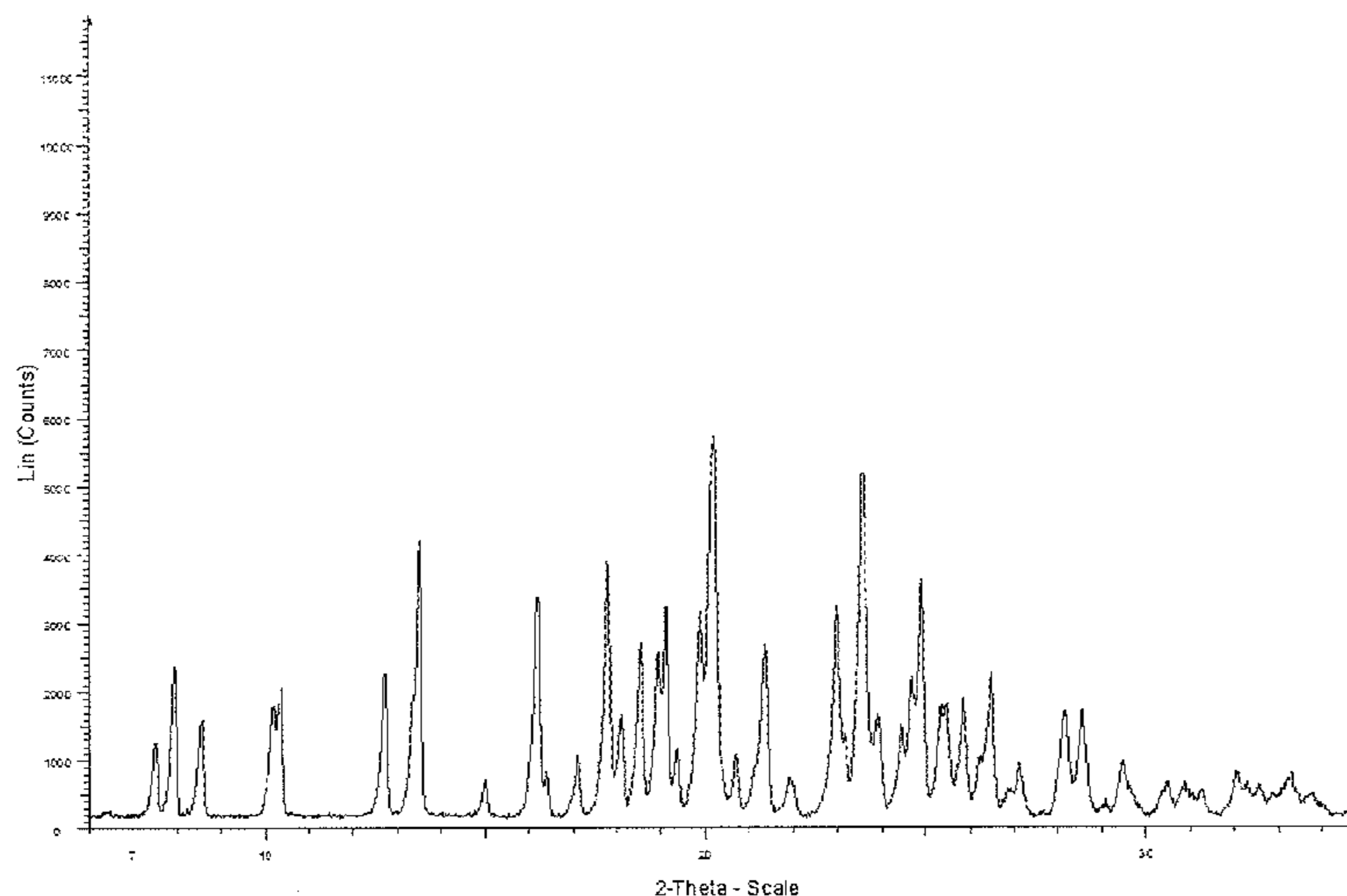
XRPD spectrum of Compound (I), n=1 Form A from ethyl acetate/n-heptane
