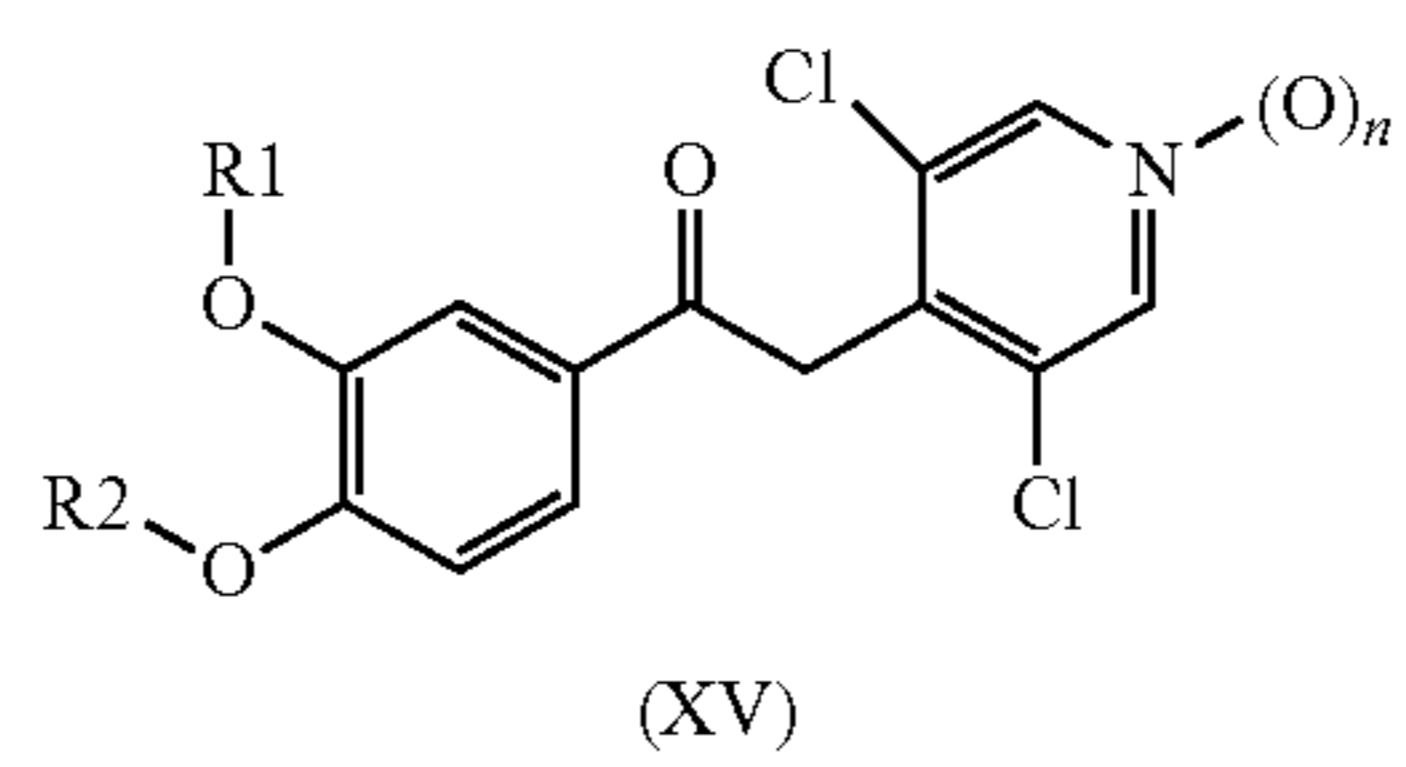
Scheme 4
