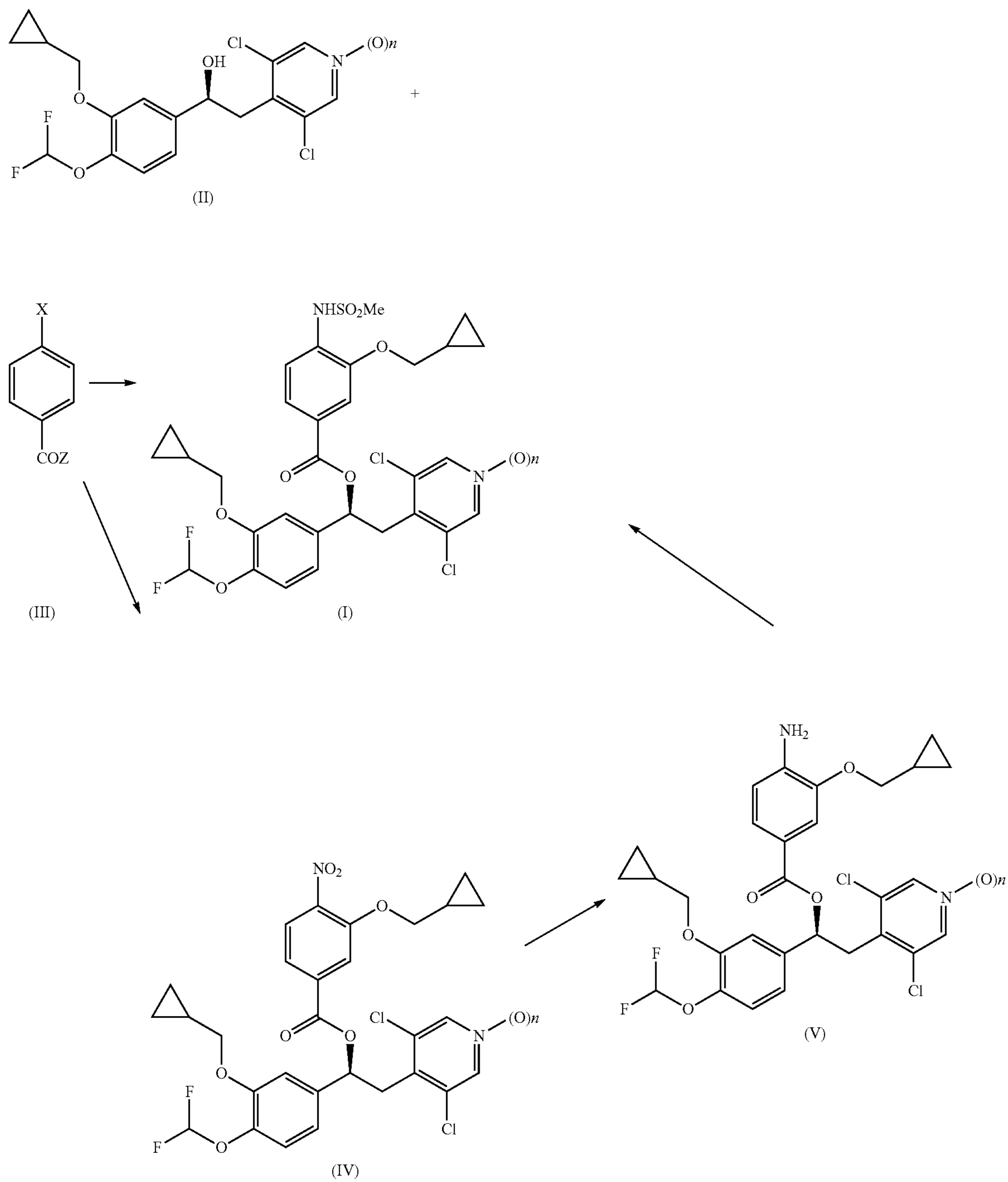
Scheme 3
