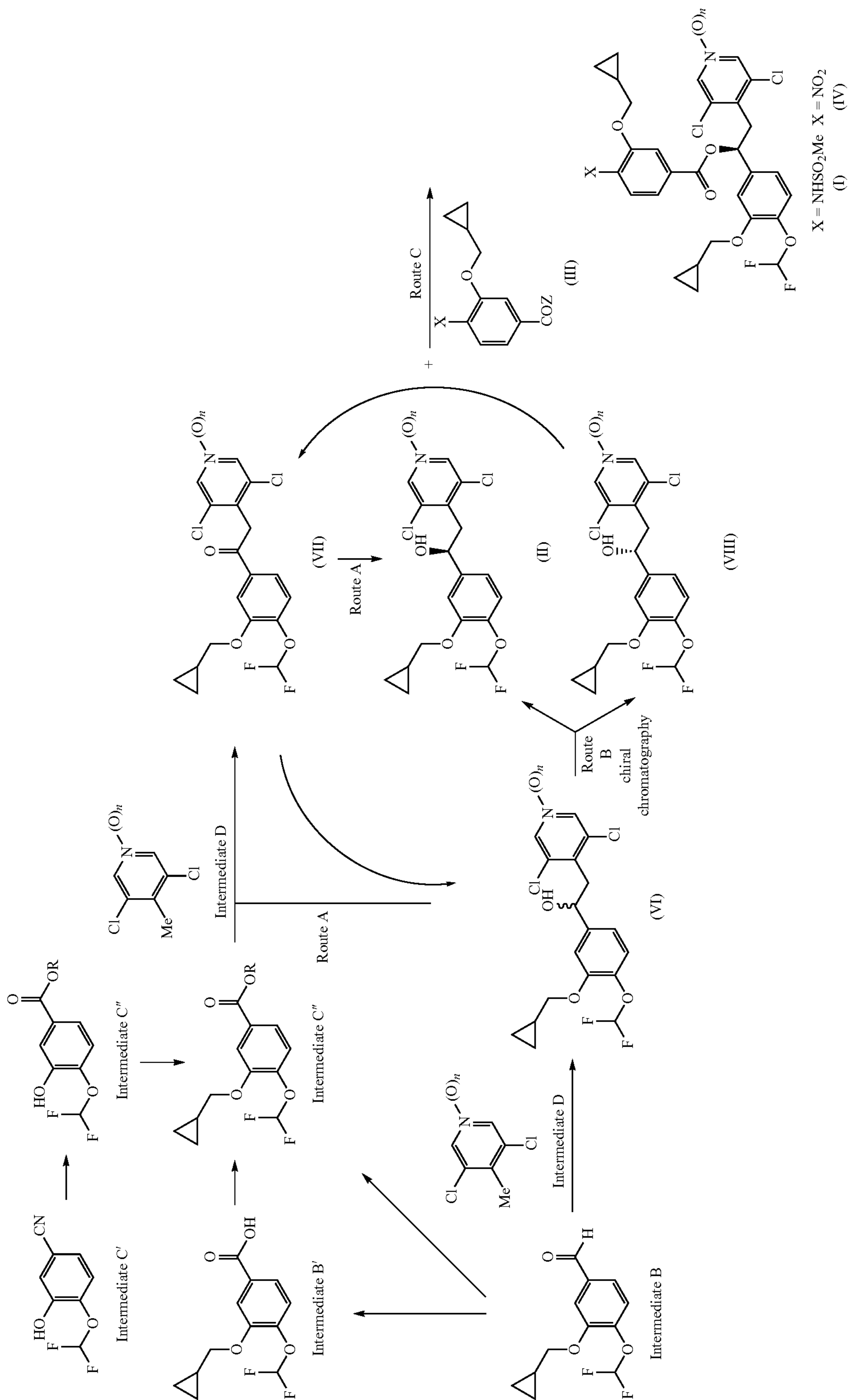
Scheme 1
