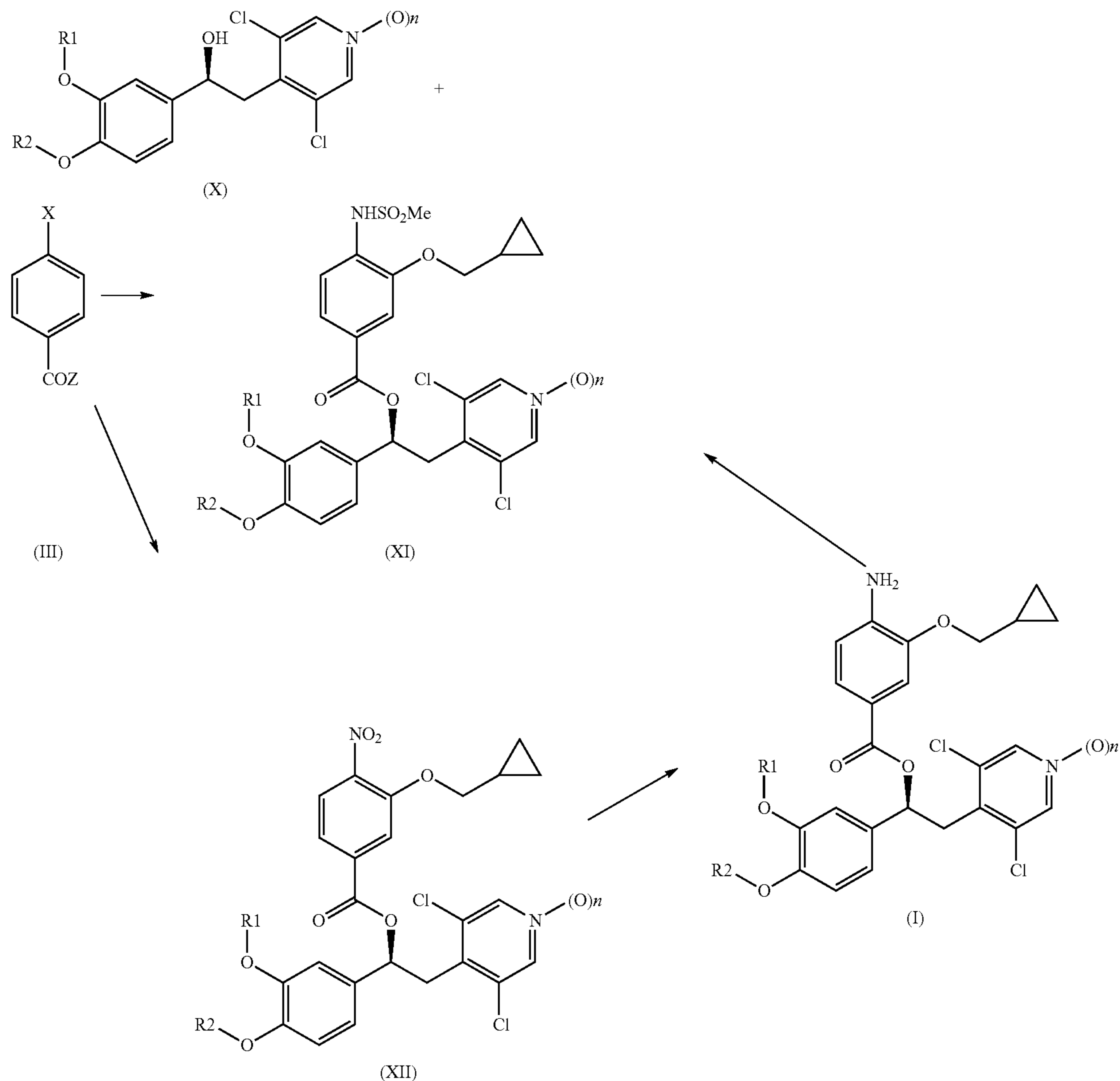
Scheme 6
