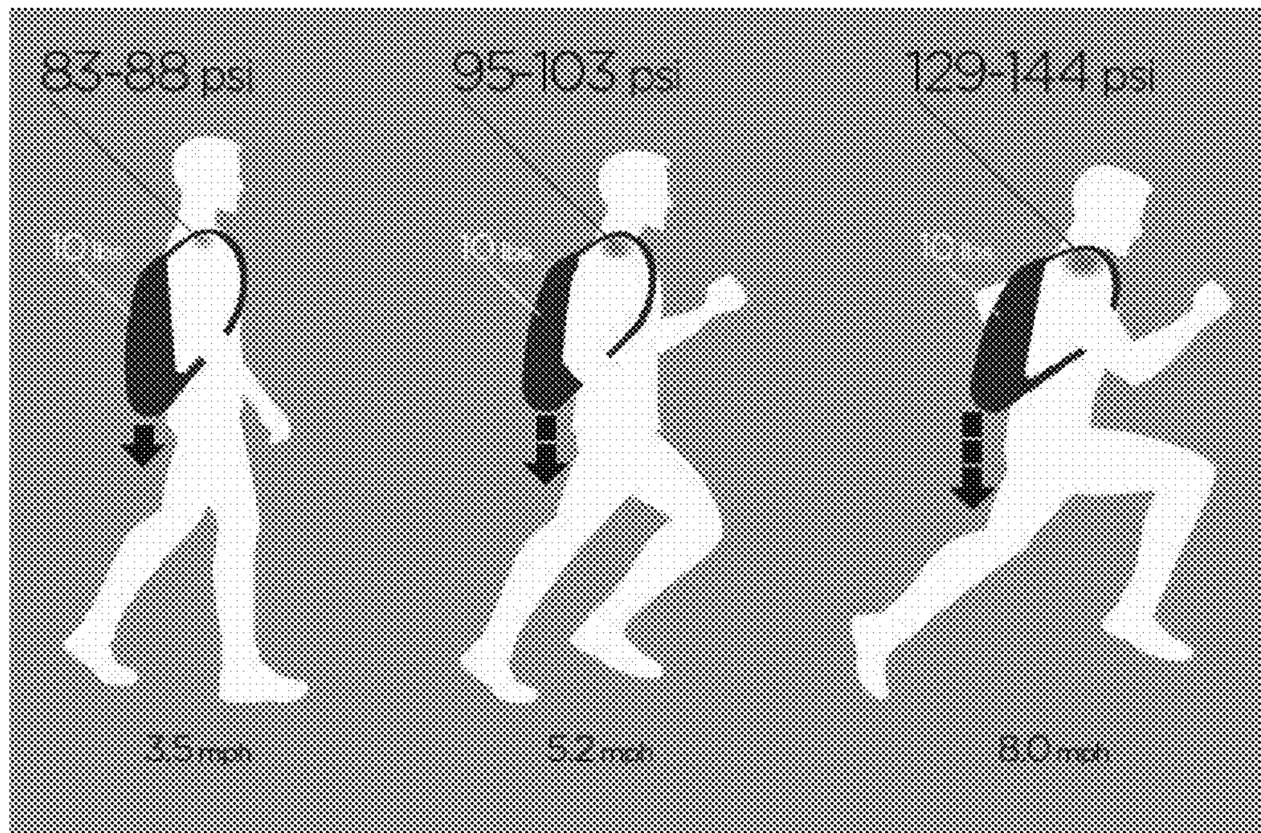
FIG. 22 (Prior Art)
