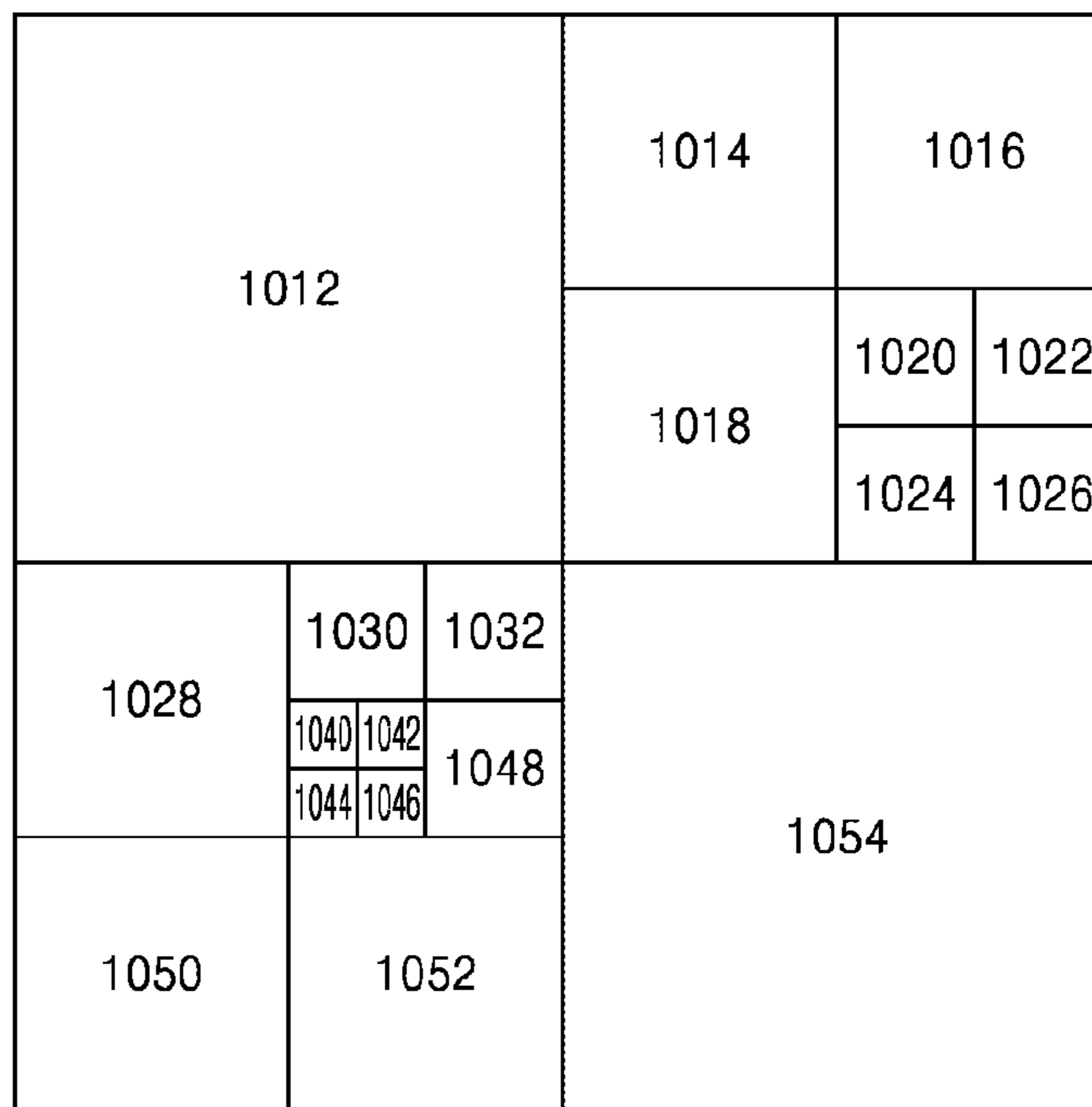
CODING UNIT (1010)
