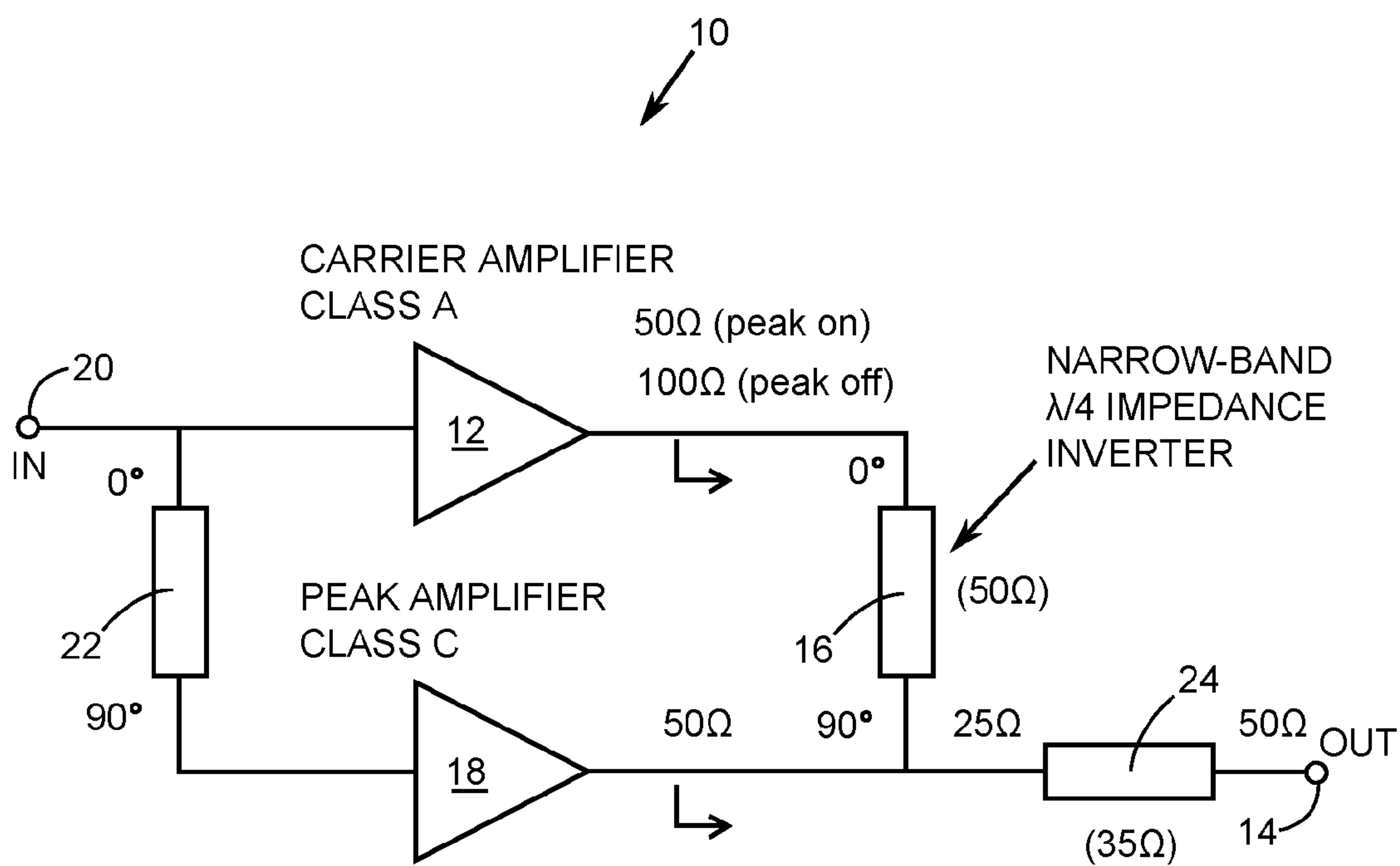
FIG. 1 (RELATED ART)
