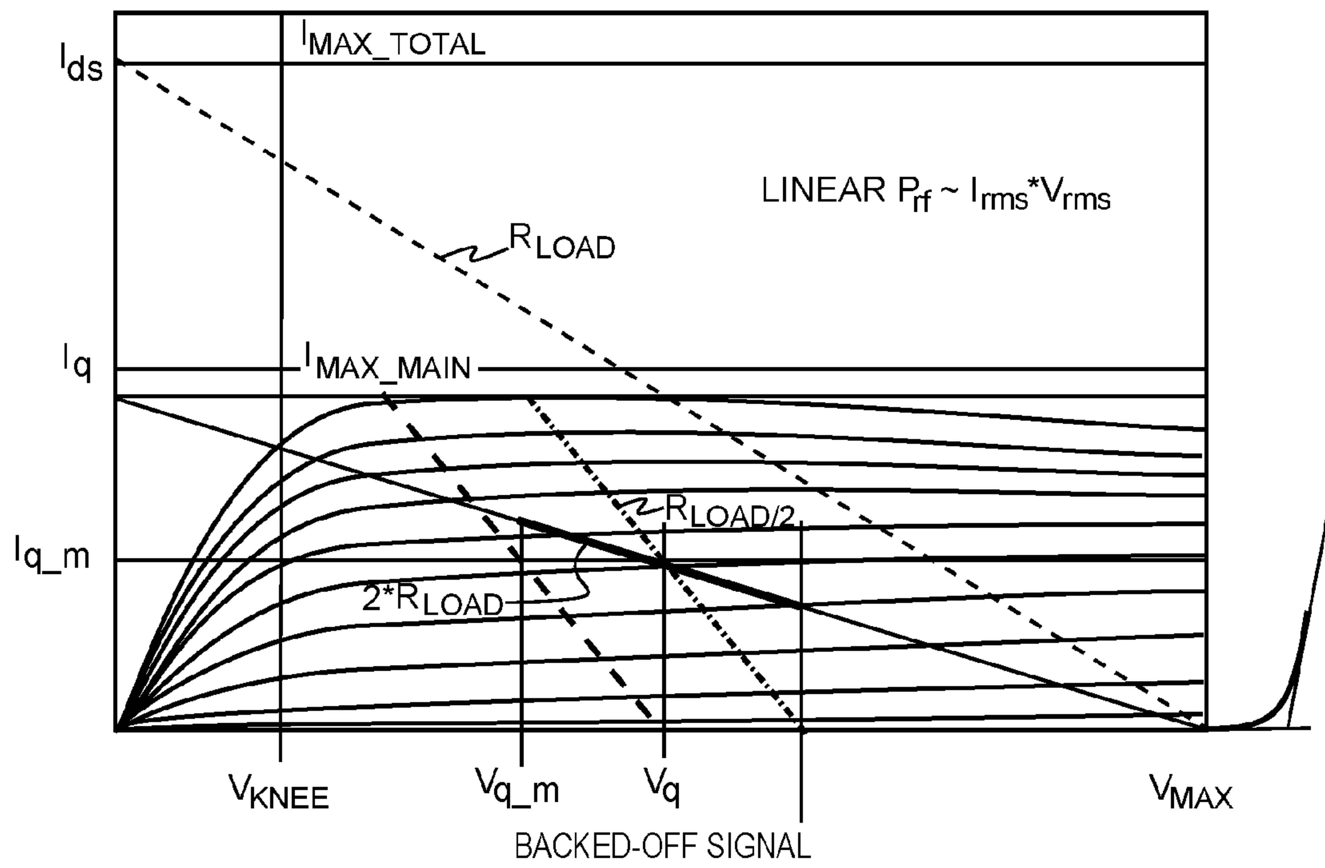
FIG. 32 (RELATED ART)
