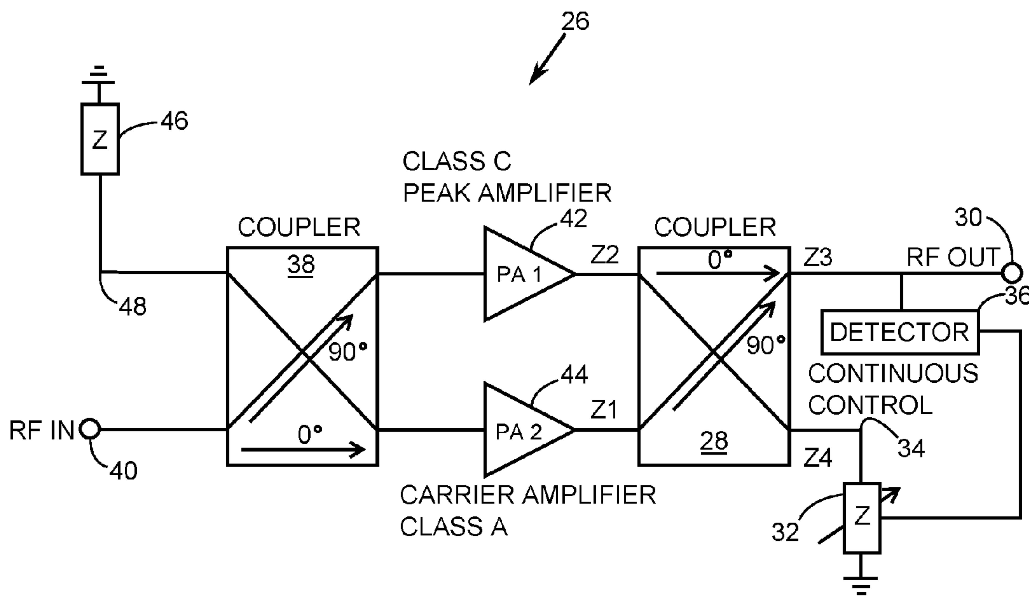
FIG. 2 (RELATED ART)
