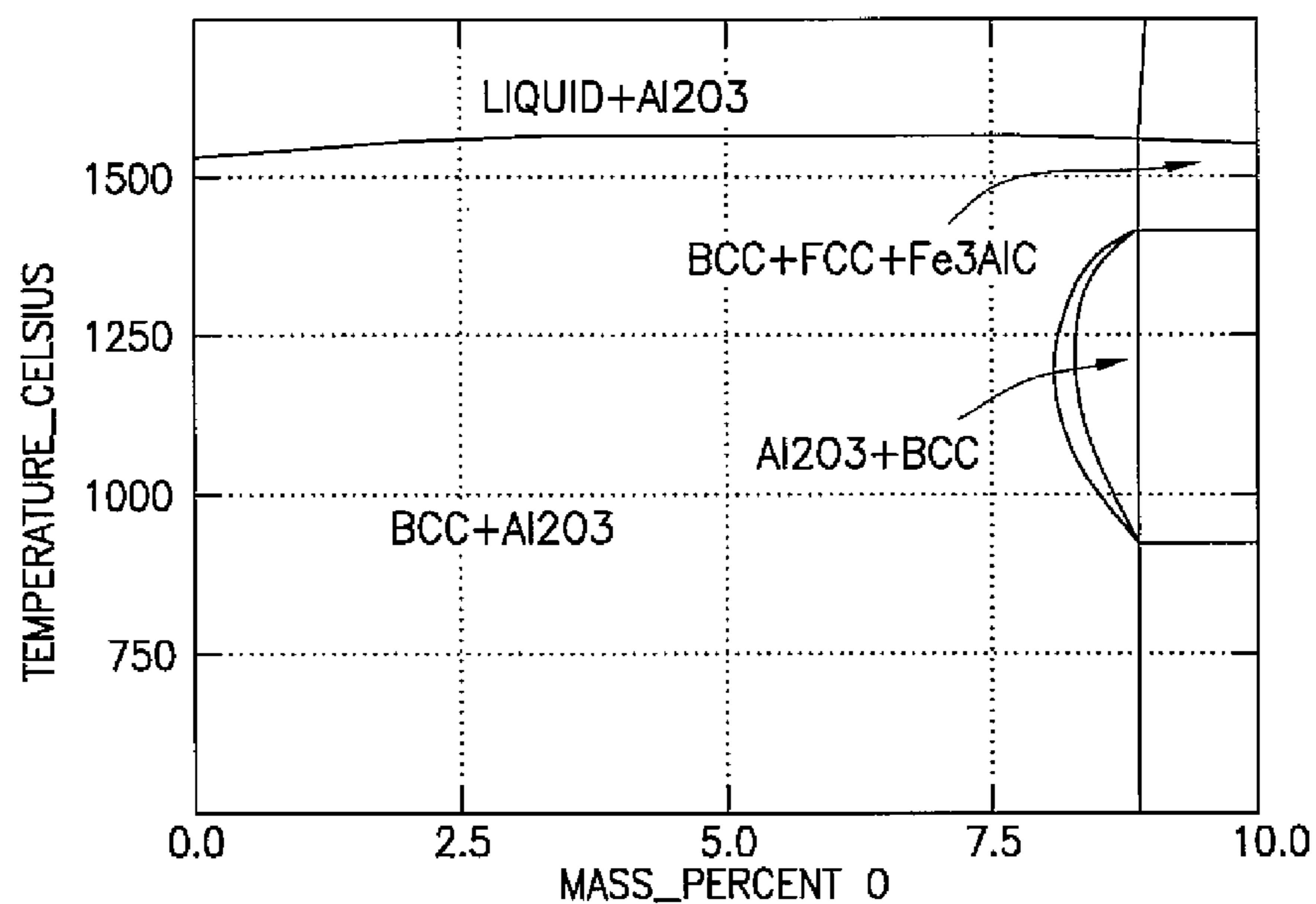
PHASE DIAGRAMS OF Fe-10%Al ALLOY, (a) ISOPLETH OF Fe-10%Al-C SHOWING BCC STRUCTURE UP TO 1000C, (b) ISOPLETH OF Fe-10%Al-O SHOWING PREFERENCE FOR FORMATION OF Al 2 O 3
