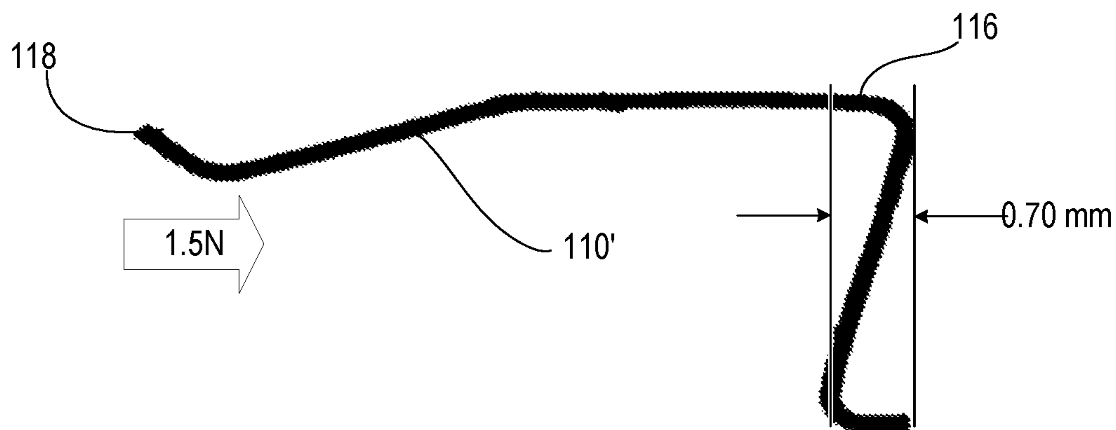
FIG. 3 (Prior Art)
