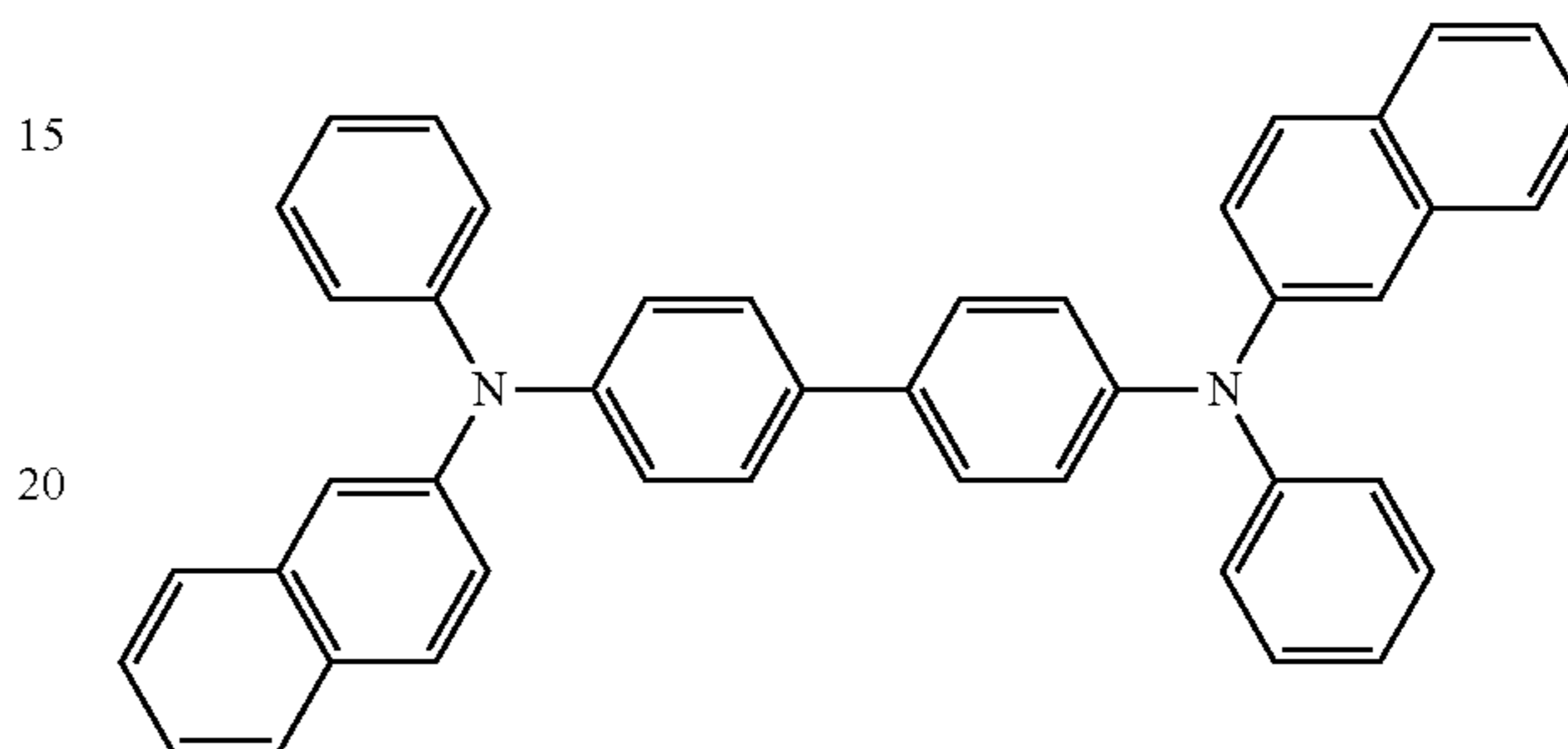
\beta -NPB
