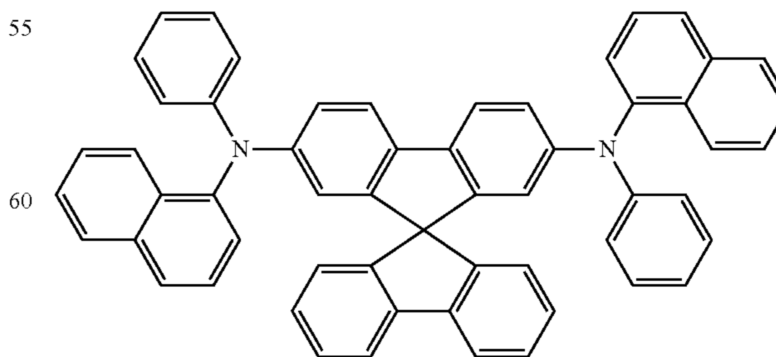
Spiro-NPB
