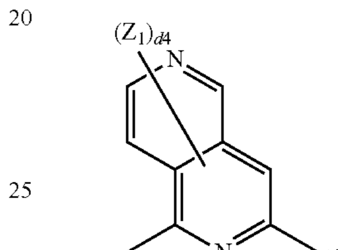
Formula 3-59
