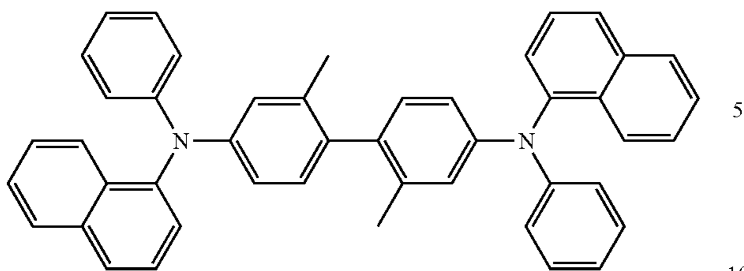
mthylated NPB
