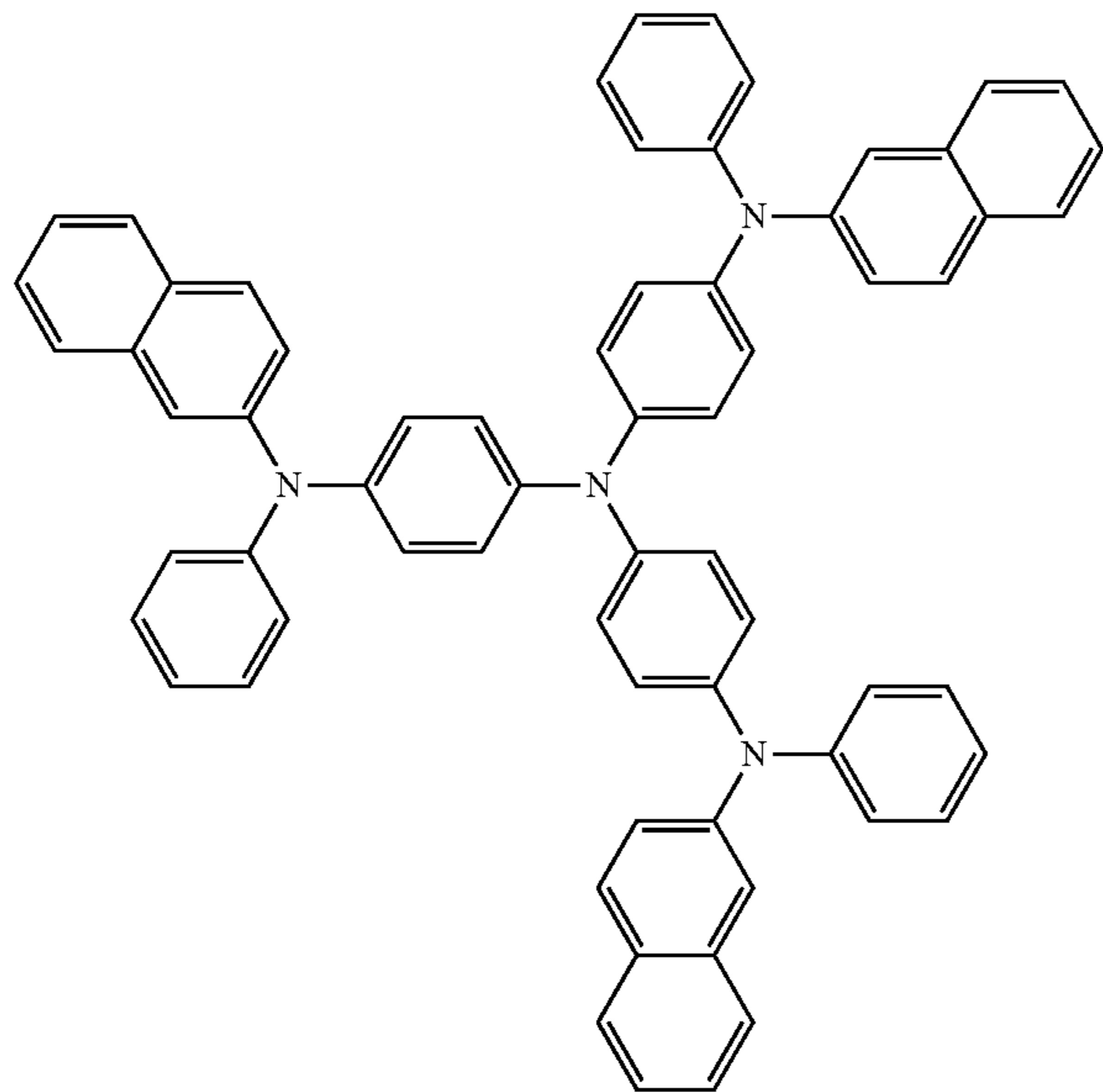
2-TNATA
