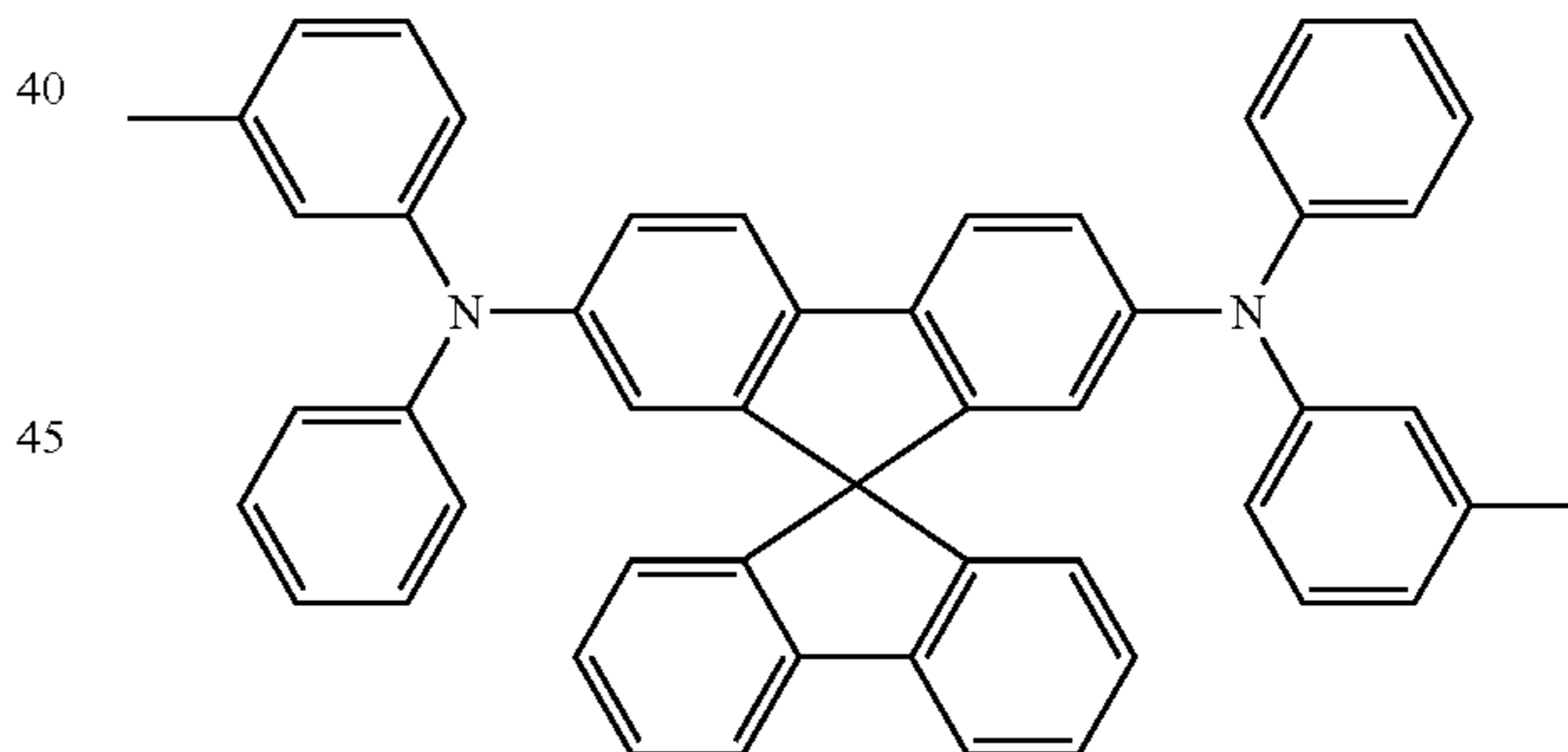
Spiro-TPD
