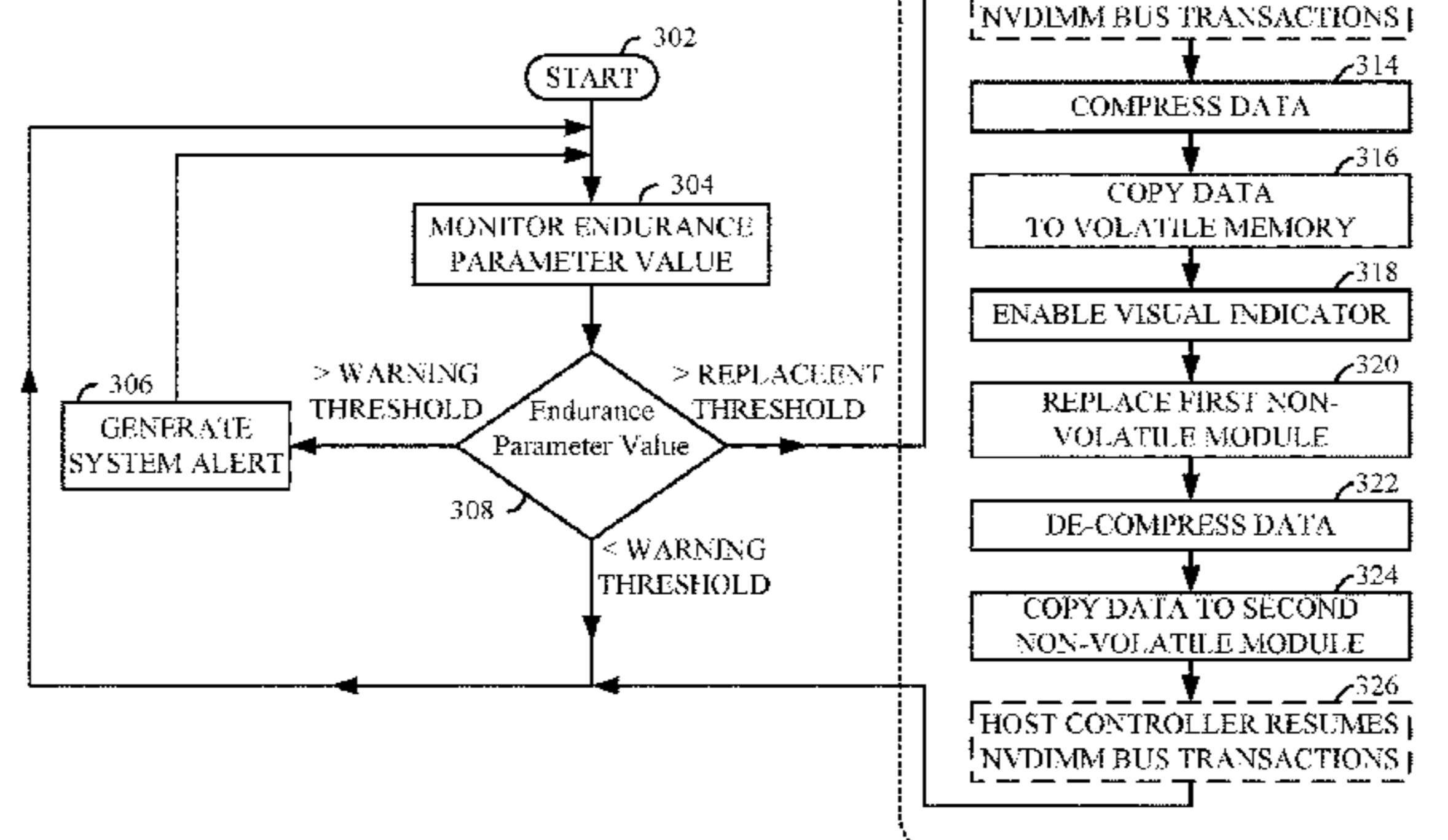
300 Method for Replacing NVDIMM Non-Volatile Memory
