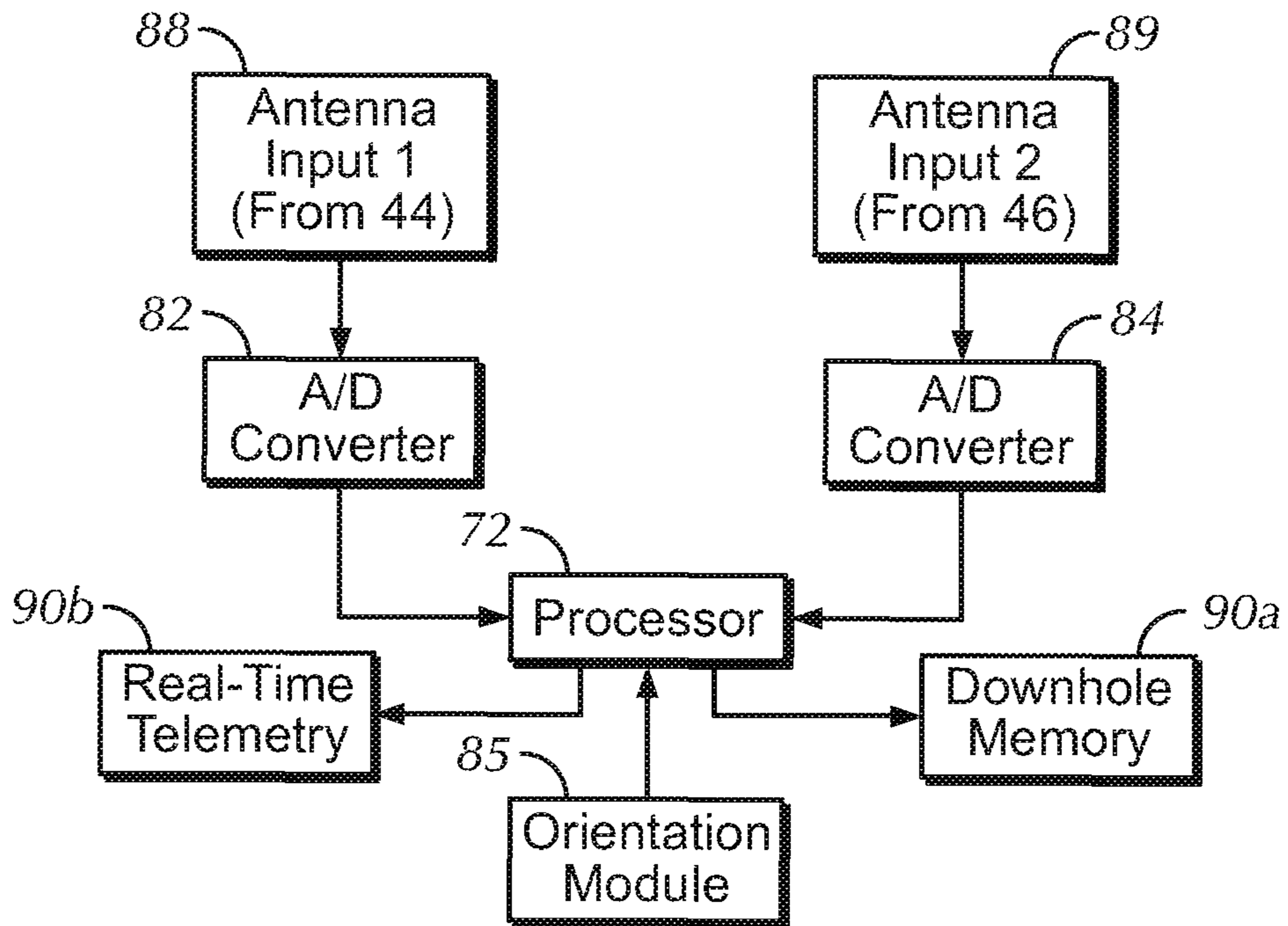
Receiver
