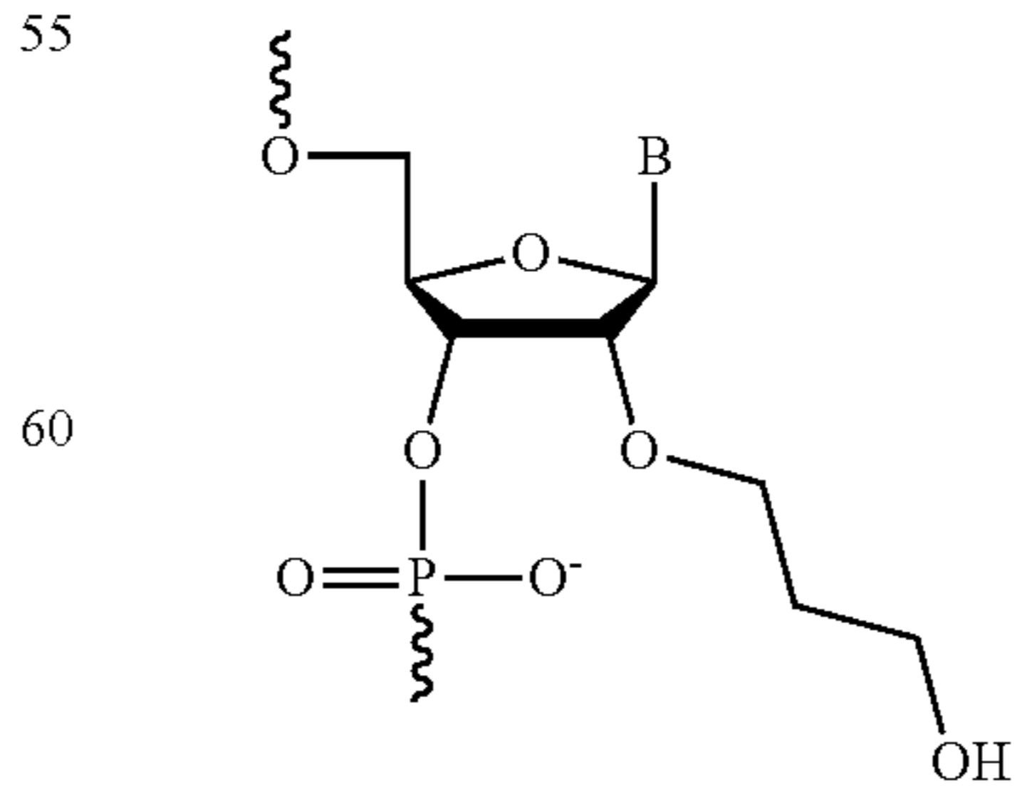
2'-(3-hydroxy)propyl
