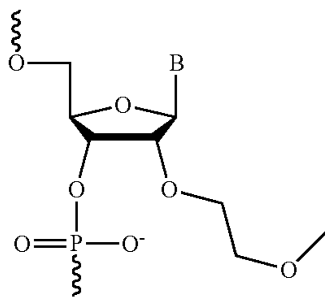
2'-MOE
