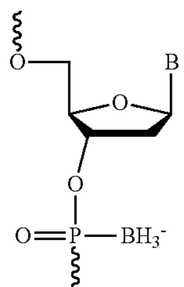
Boranophosphates
