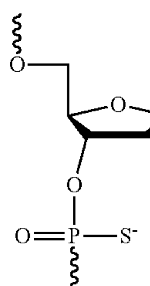
Phosphorothioate
