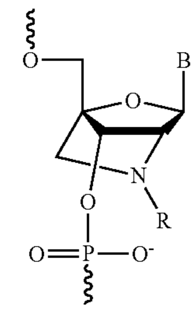
Amino-LNA
