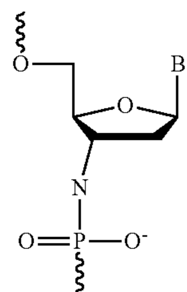
3'-Phosphoramidate
