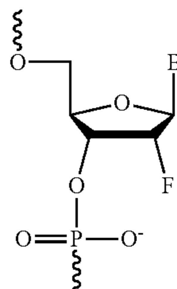
2'-Fluoro
