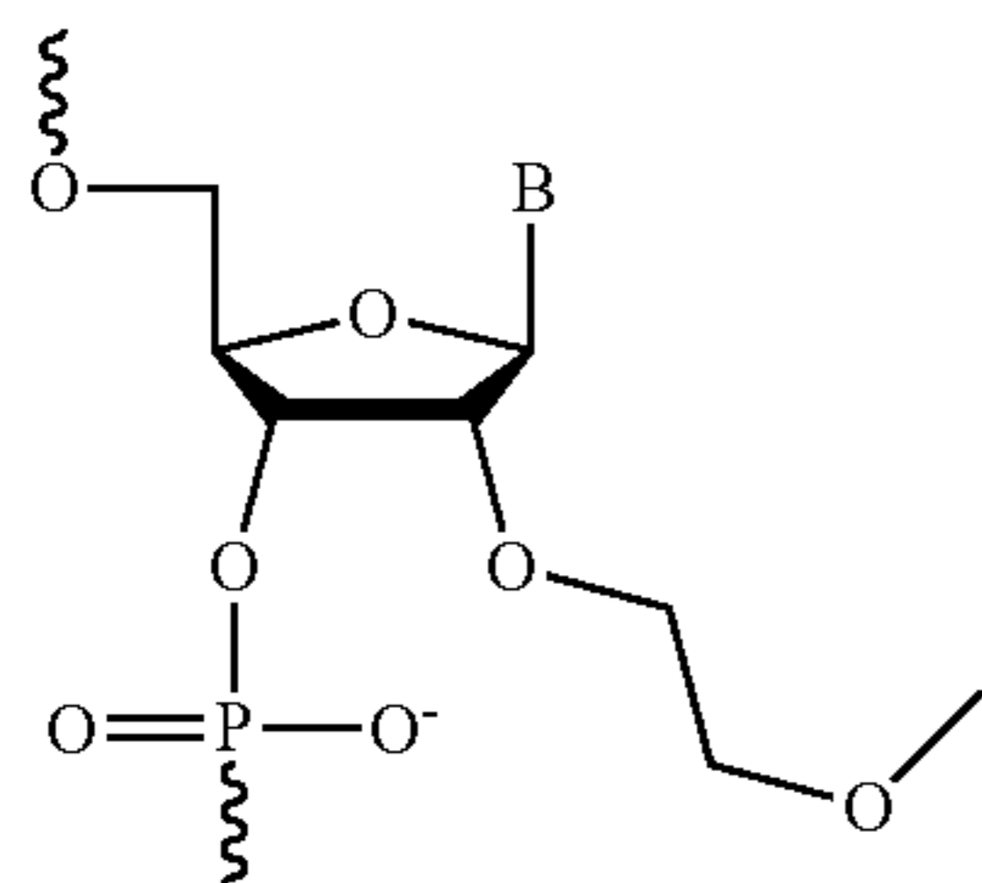
2'-MOE
