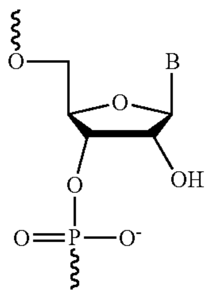
RNA
