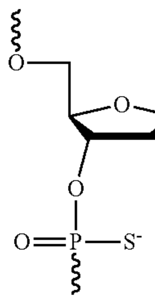
Phosphorothioate
