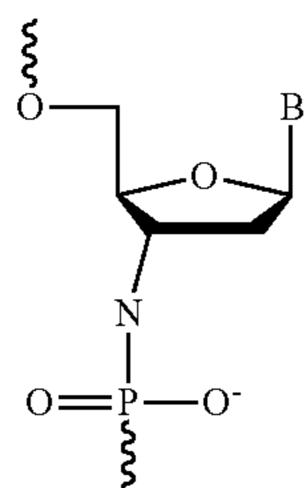
3'-Phosphoramidate
