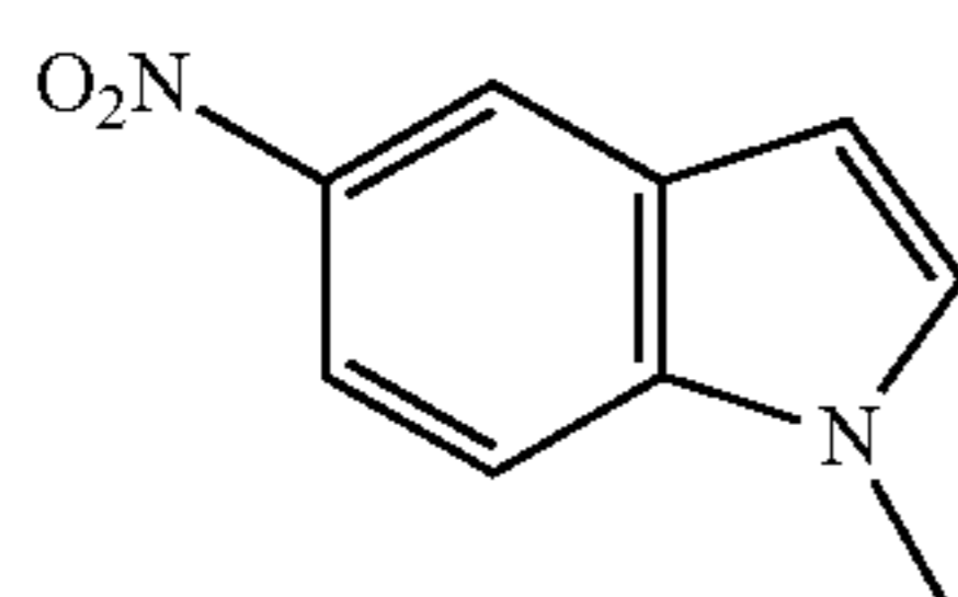
5-Nitroindole
