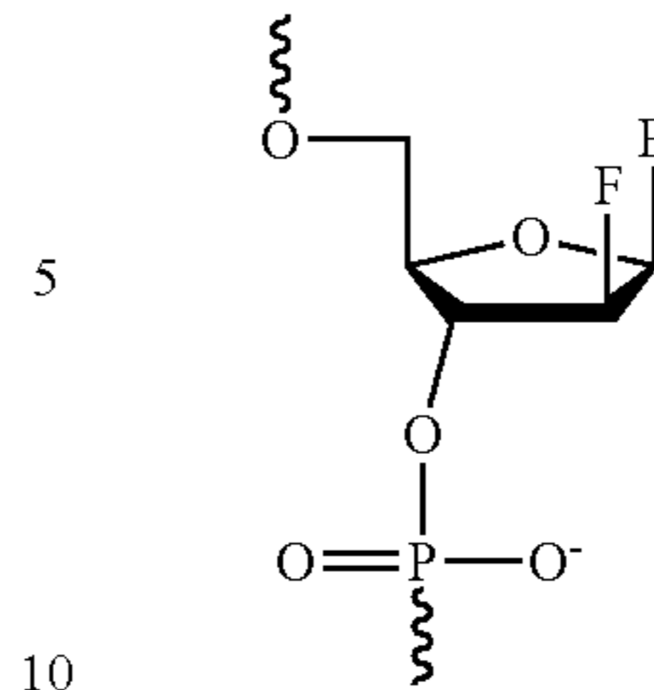
2'-F-ANA
