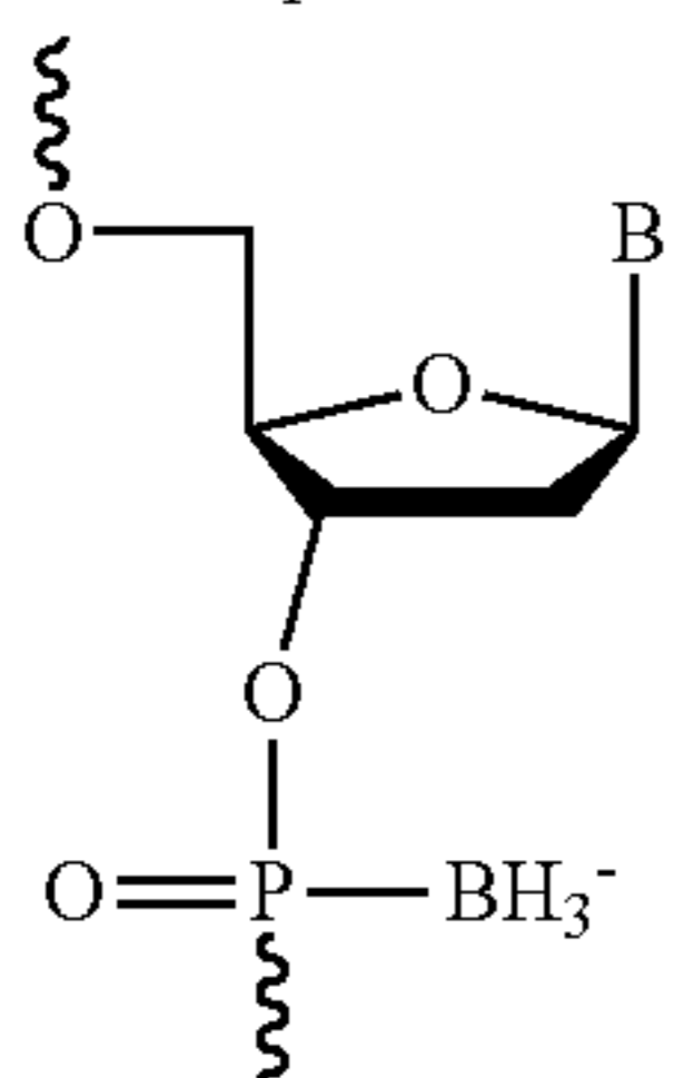
Boranophosphates
