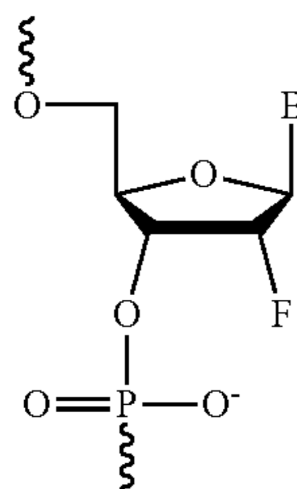
2'-Fluoro
