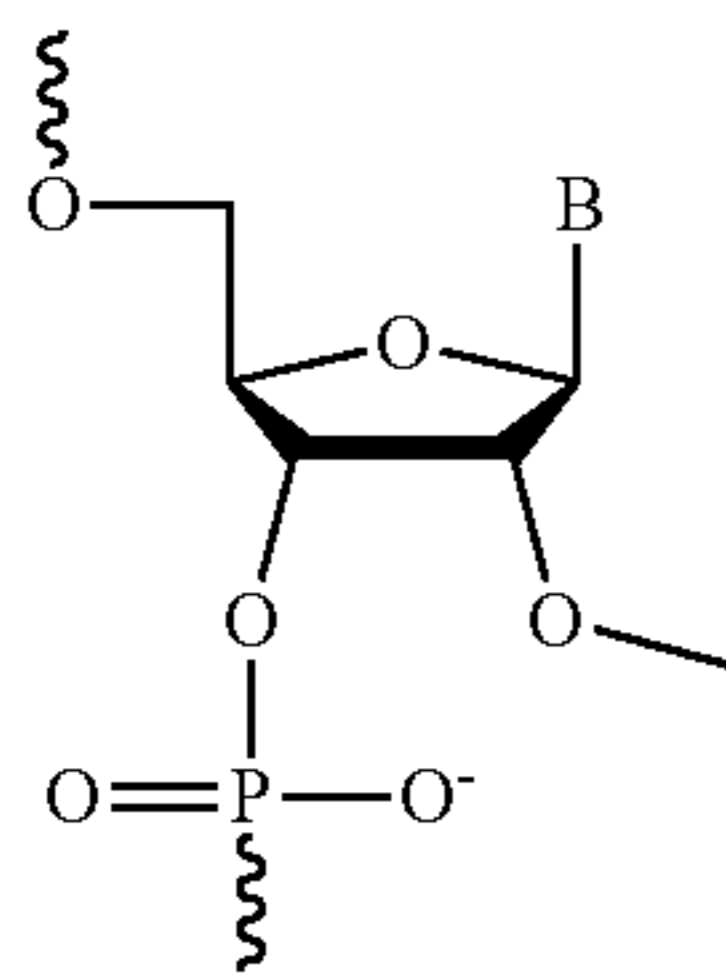
2'-O-Methyl
