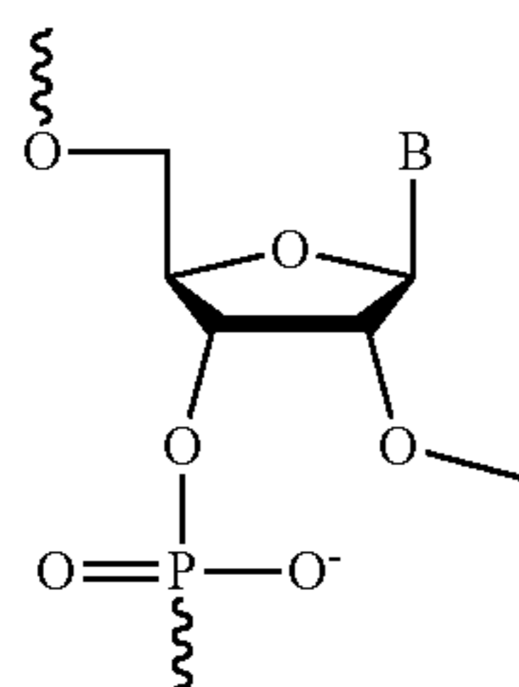
2'-O-Methyl
