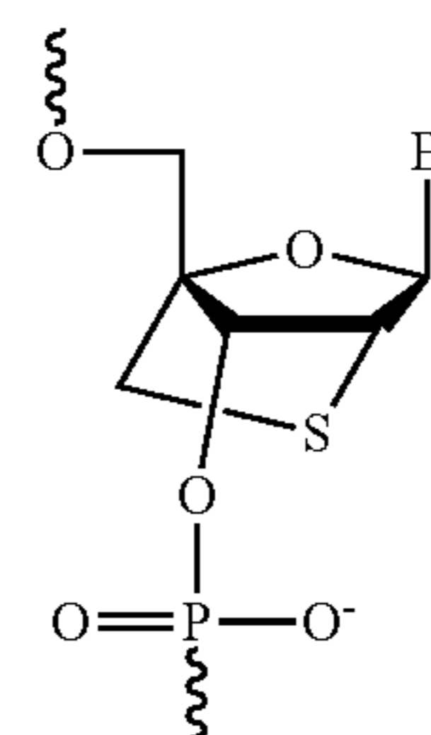
Thio-LNA
