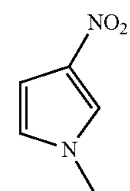
3-Nitropyrrole
