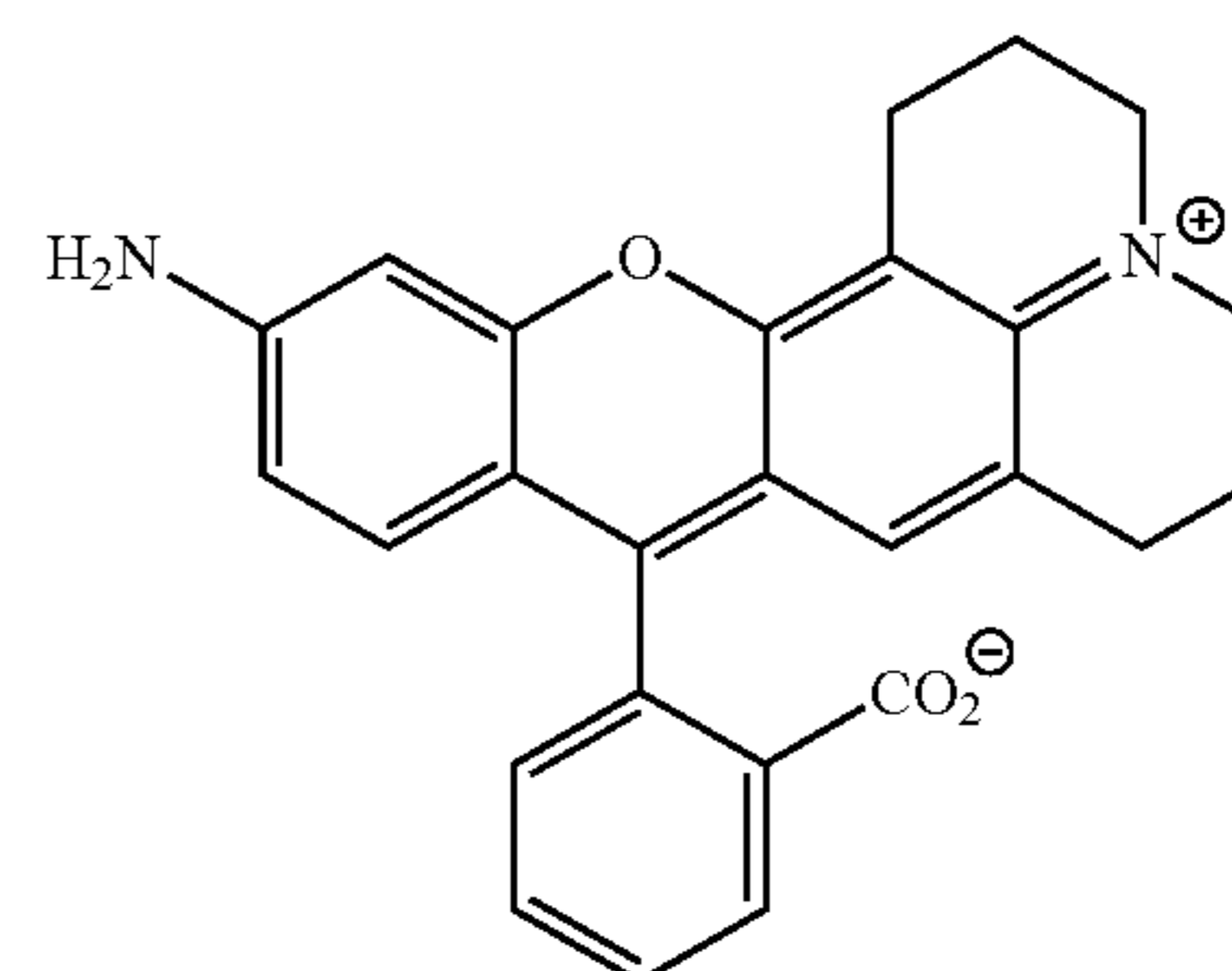
Scheme III
