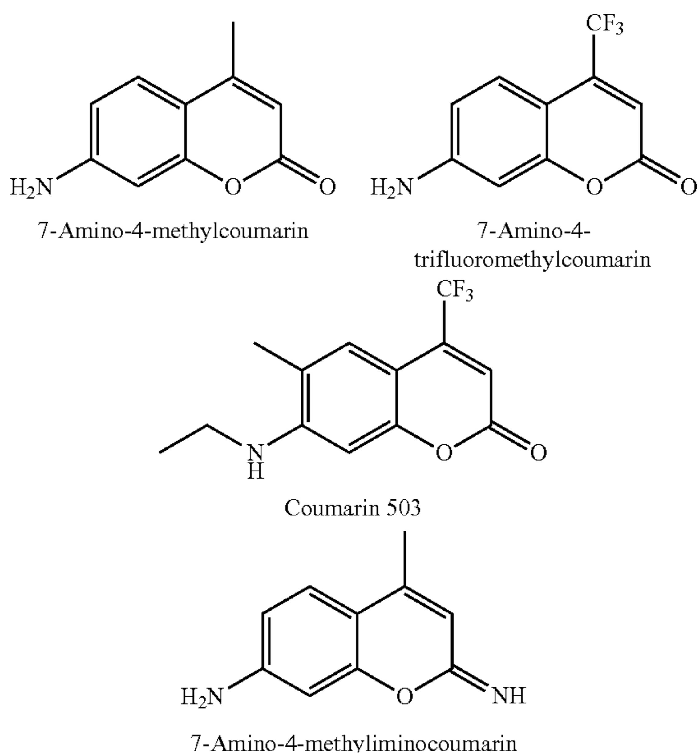
Scheme V
