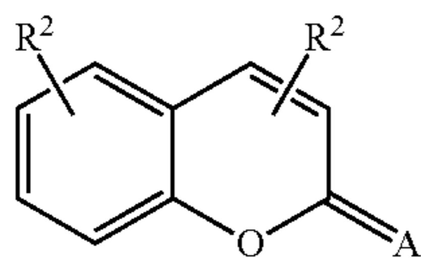
Scheme IV
