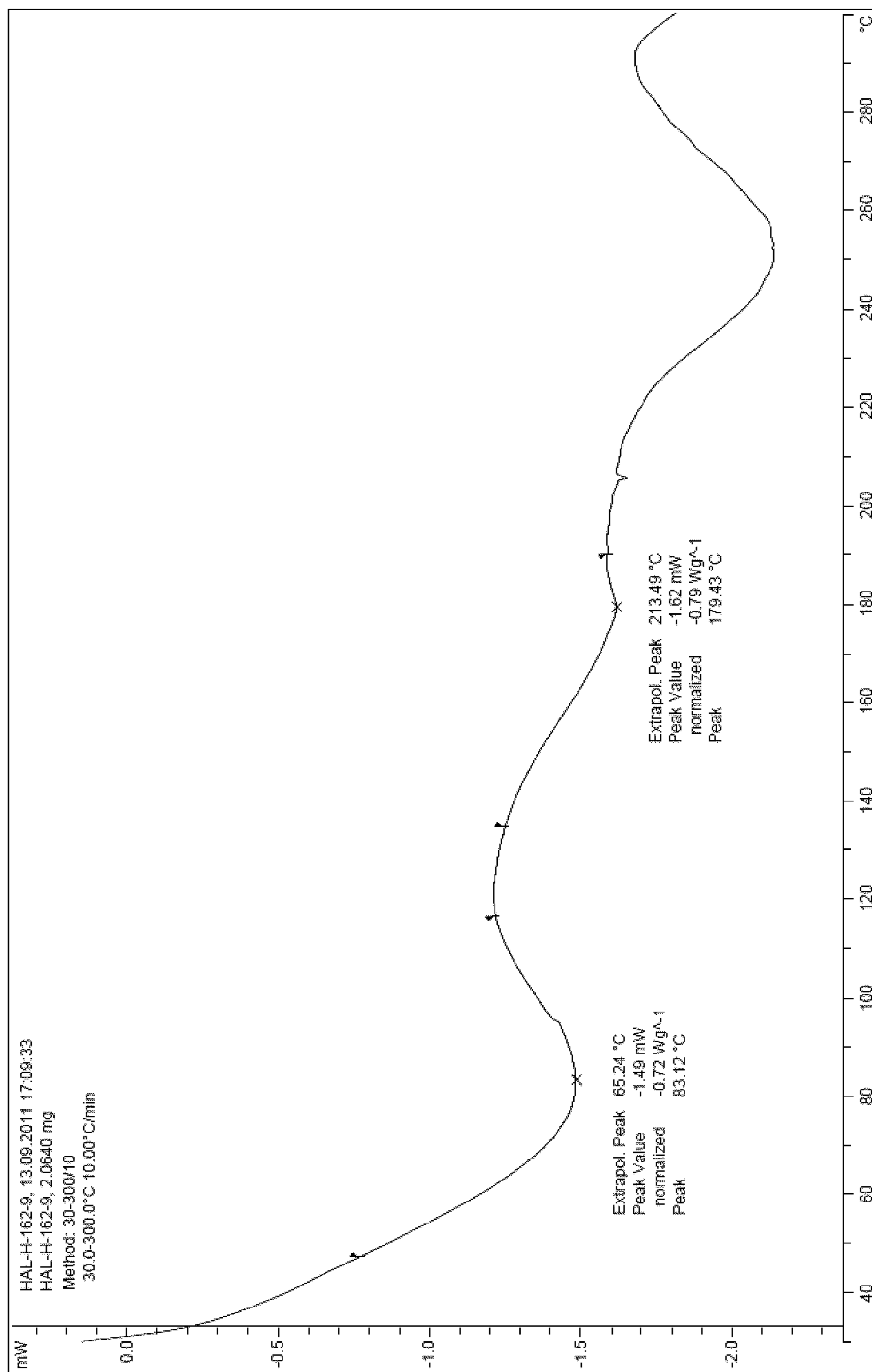
Figure 6. DSC thermogram of (1R,2S)-(E)-2-(3-(4-((cis-2,6-dimethylmorpholino)methyl)styryl)-1H-indazol-6-yl)-5'-methoxyspiro[cyclopropane-1,3'-indolin]-2'-one phosphate
