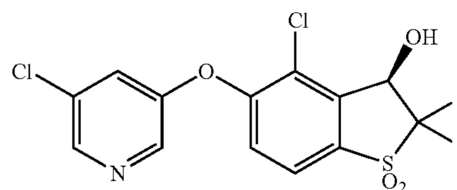
(R)-4-Chloro-5-((5-chloropyridin-3-yl)oxy)-2,2-difluoro-3-hydroxy-2,3-dihydrobenzo[b]thiophene 1,1-dioxide (Compound 86)
