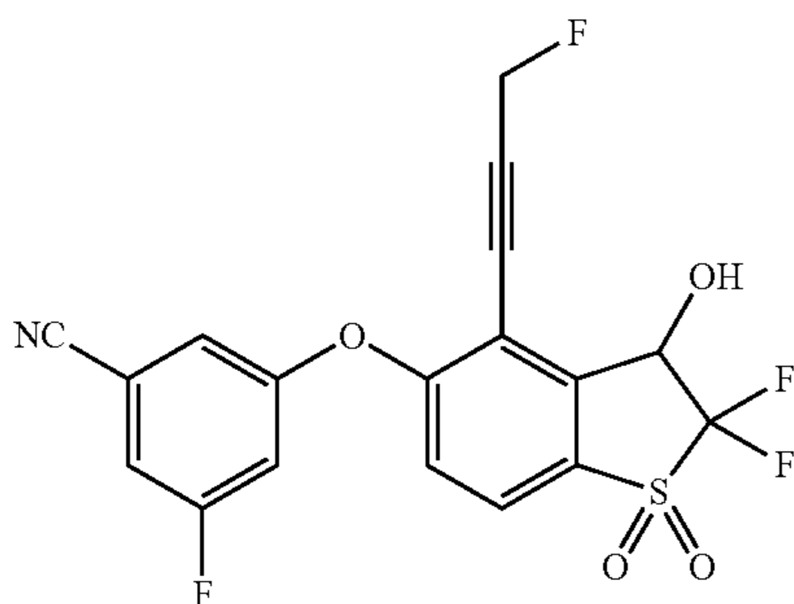
3-[[2,2-Difluoro-4-(3-fluoroprop-1-ynyl)-3-hydroxy-1,1-dioxo-3H-benzothiophen-5-yl]oxy]-5-fluorobenzonitrile (Compound 64)
