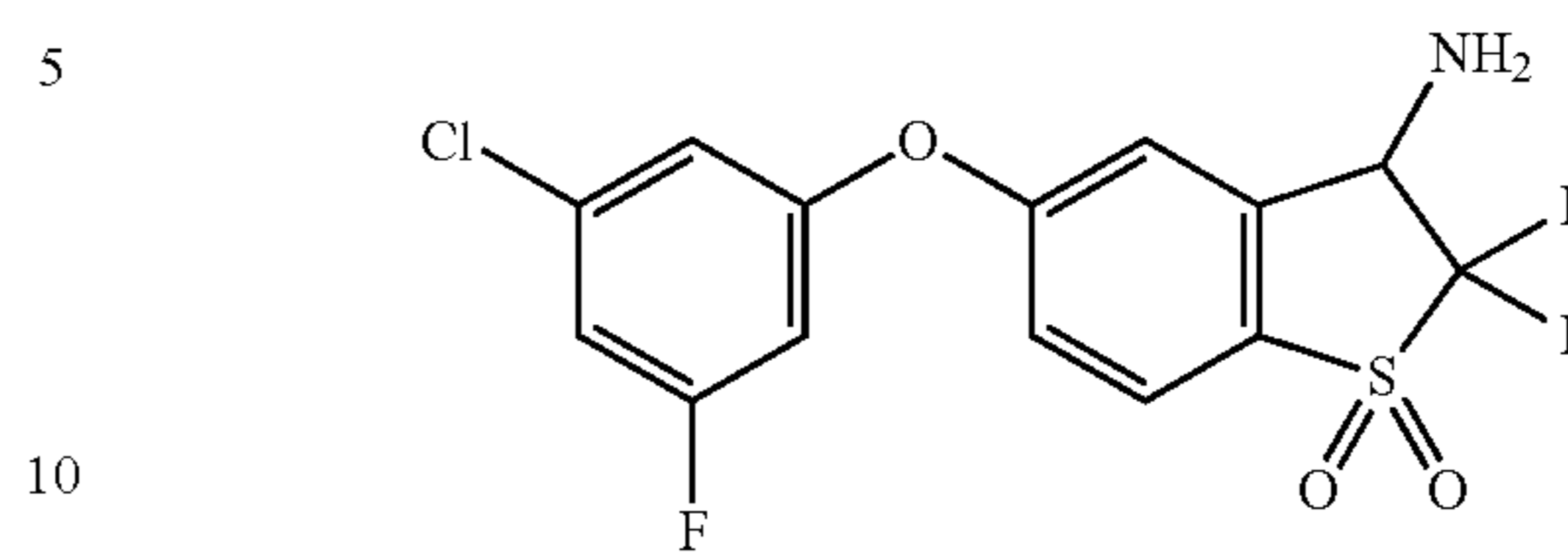
3-Amino-5-(3-chloro-5-fluorophenoxy)-2,2-difluoro-2,3-dihydrobenzo[b]thiophene 1,1-dioxide (Compound 12)
