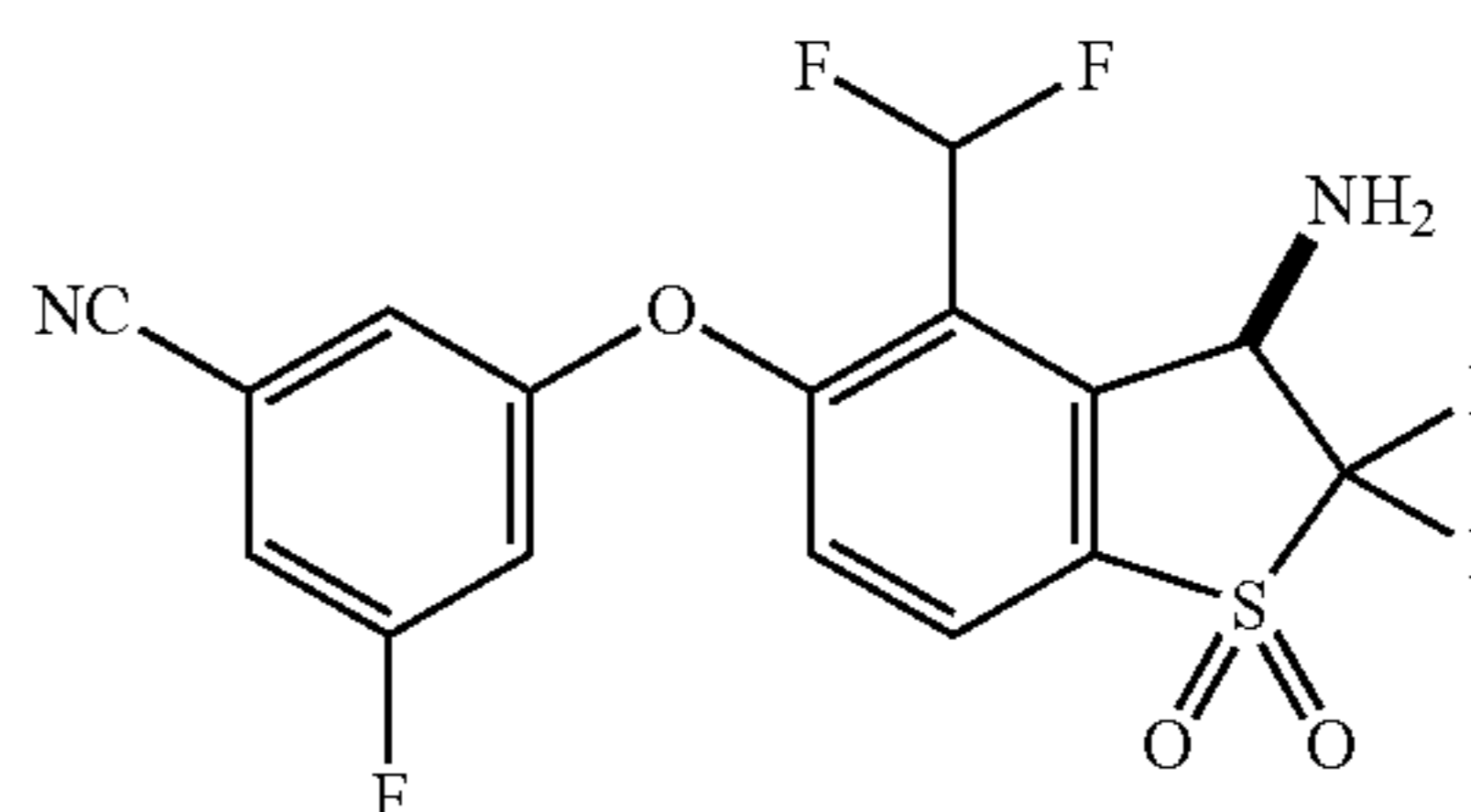
(R)-3-((3-Amino-4-(difluoromethyl)-2,2-difluoro-1,1-dioxido-2,3-dihydrobenzo[b]thiophen-5-yl)oxy)-5-fluorobenzonitrile (Compound 41)
