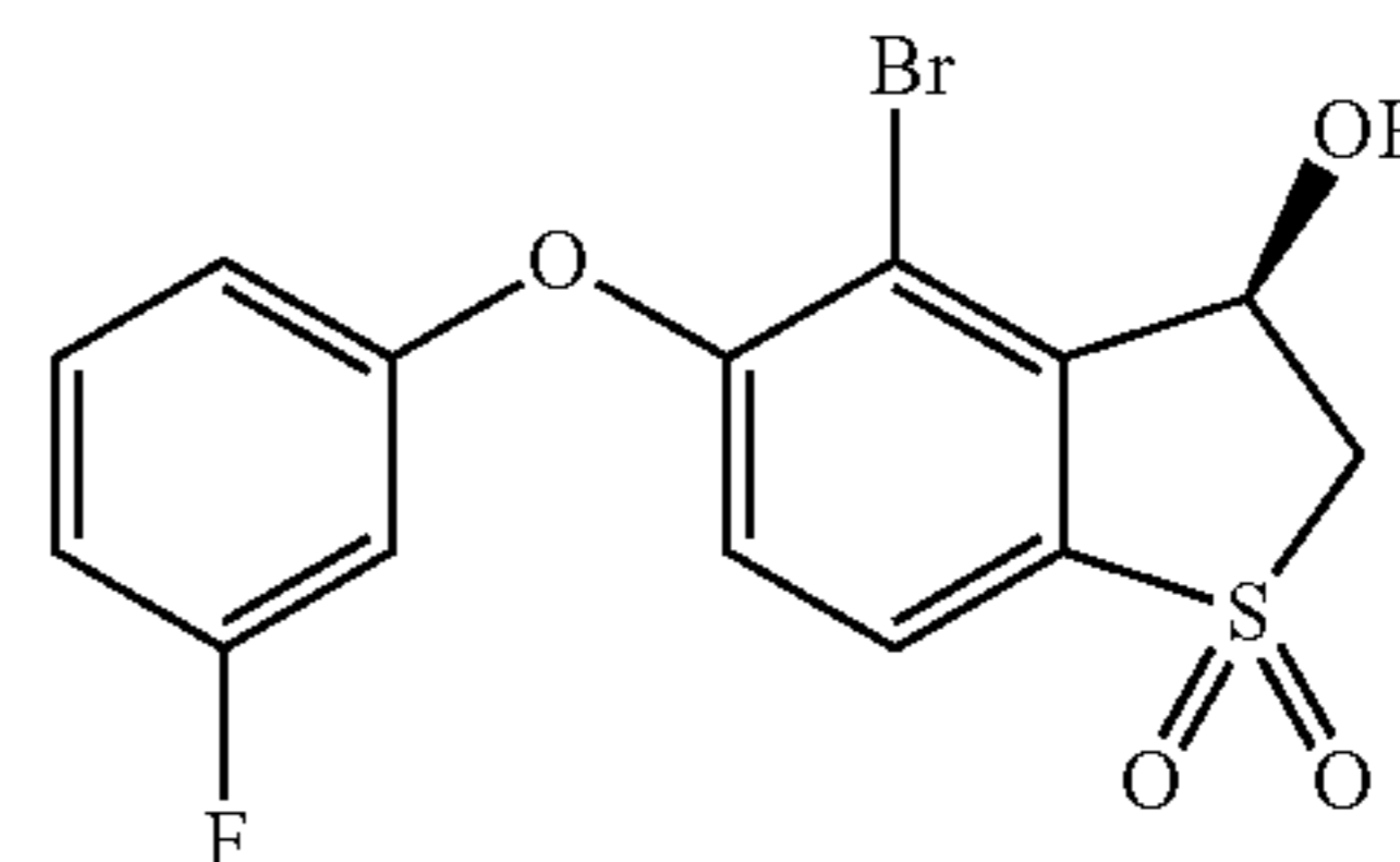
(R)-4-bromo-5-(3-fluorophenoxy)-3-hydroxy-2,3-dihydrobenzo[b]thiophene 1,1-dioxide (Compound 73)
