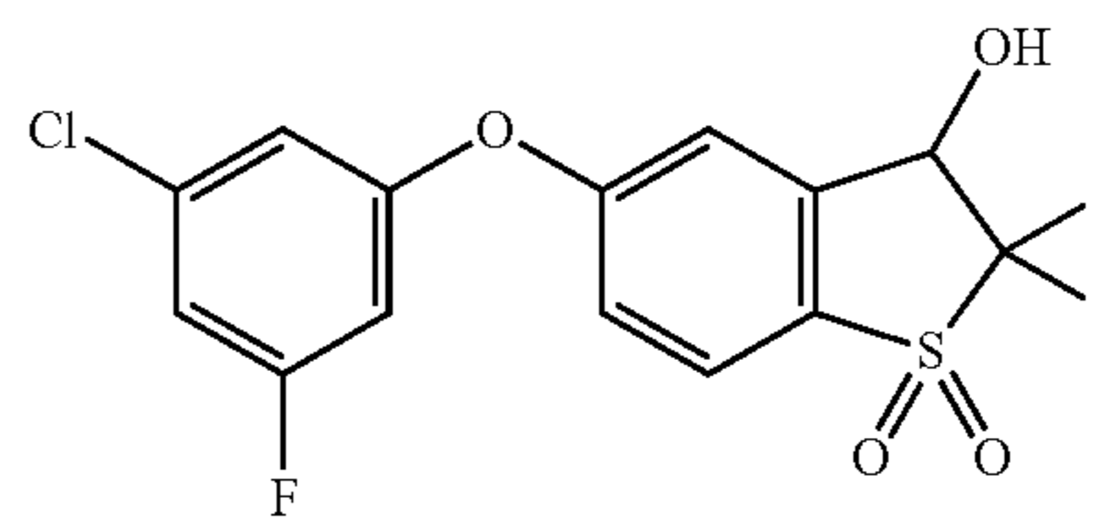
5-(3-Chloro-5-fluorophenoxy)-2,2-difluoro-3-hydroxy-2,3-dihydrobenzo[b]thiophene 1,1-dioxide (Compound 16)
