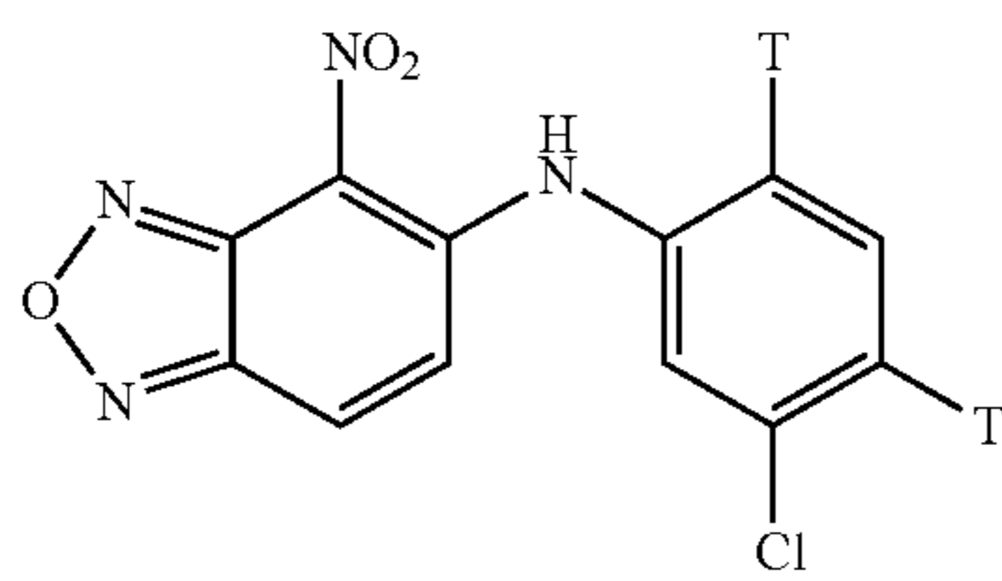
N-(3-Chlorophenyl-4,6-t 2 )-4-nitrobenzo[c][1,2,5]oxadiazol-5-amine (Compound 120)
