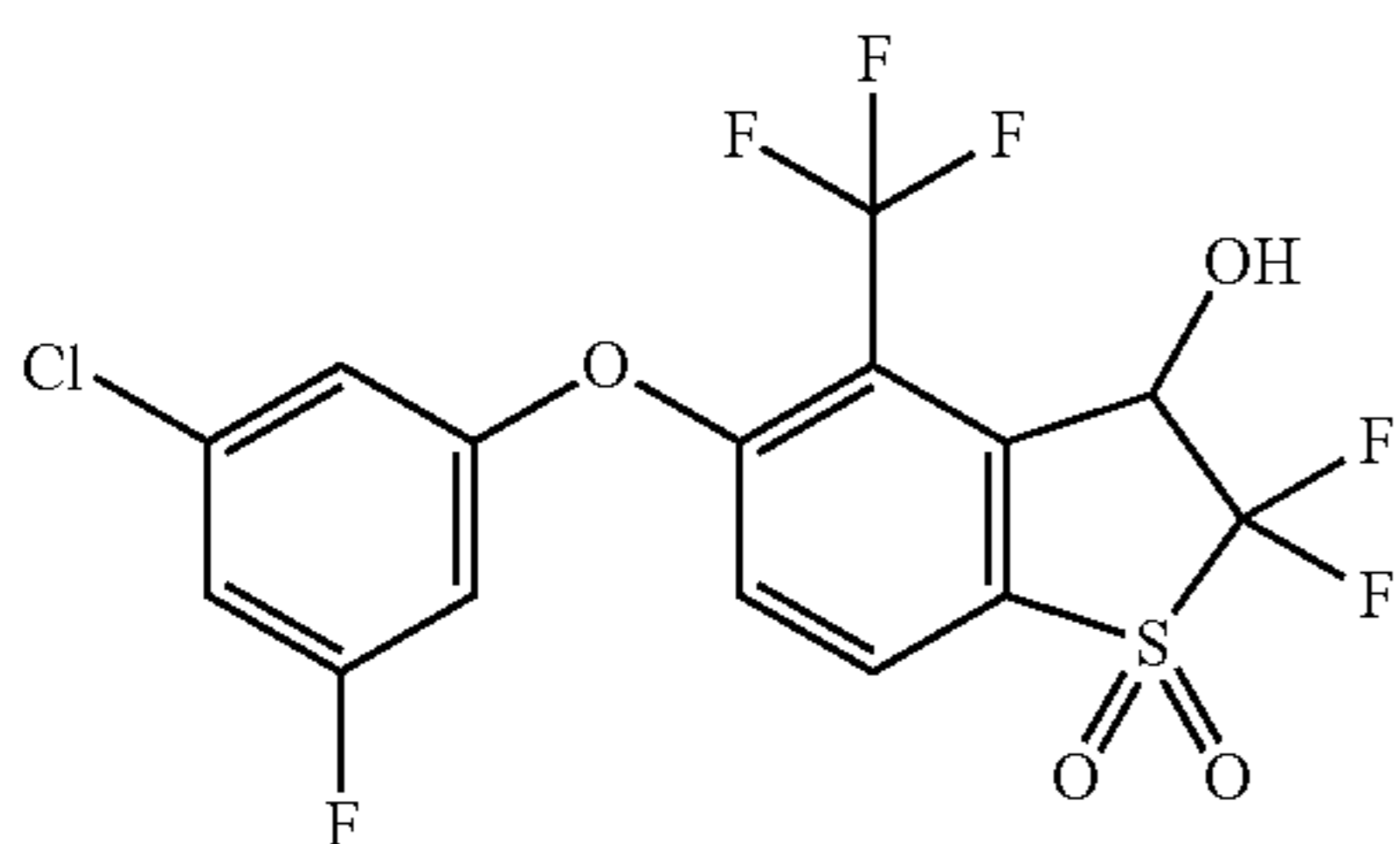
5-(3-Chloro-5-fluorophenoxy)-2,2-difluoro-3-hydroxy-4-(trifluoromethyl)-2,3-dihydrobenzo[b]thiophene 1,1-dioxide (Compound 14)
