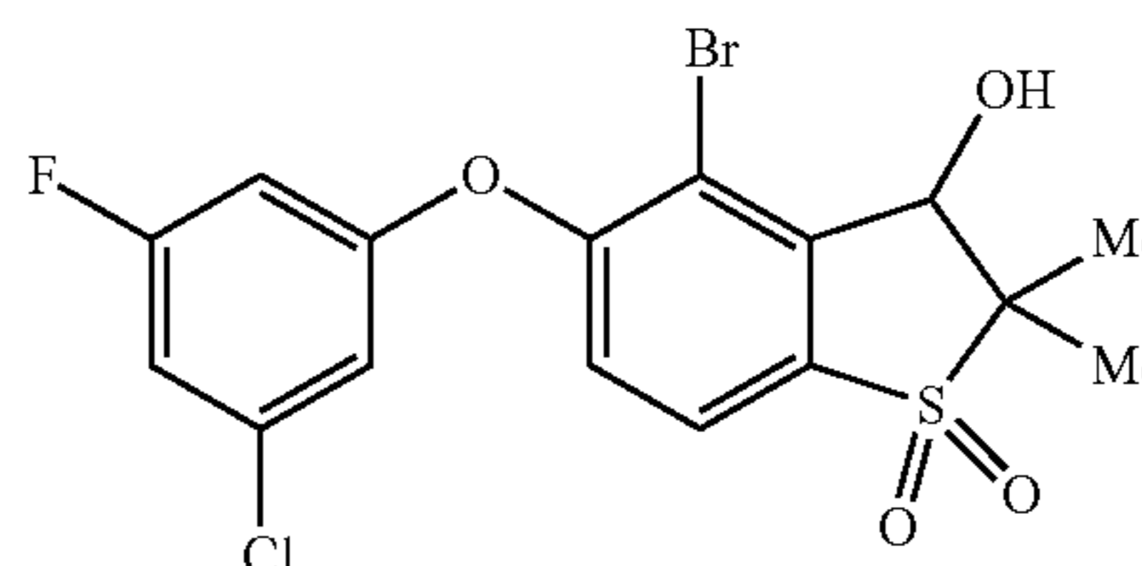
4-Bromo-5-(3-chloro-5-fluoro-phenoxy)-2,2-dimethyl-1,1-dioxo-3H-benzothiophen-3-ol (Compound 60)
