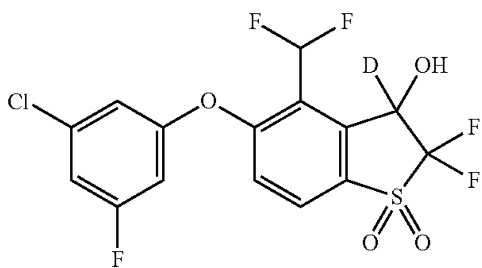
5-(3-Chloro-5-fluorophenoxy)-4-(difluoromethyl)-2,2-difluoro-3-hydroxy-2,3-dihydrobenzo[b]thiophene 1,1-dioxide-3-d (Compound 25)
