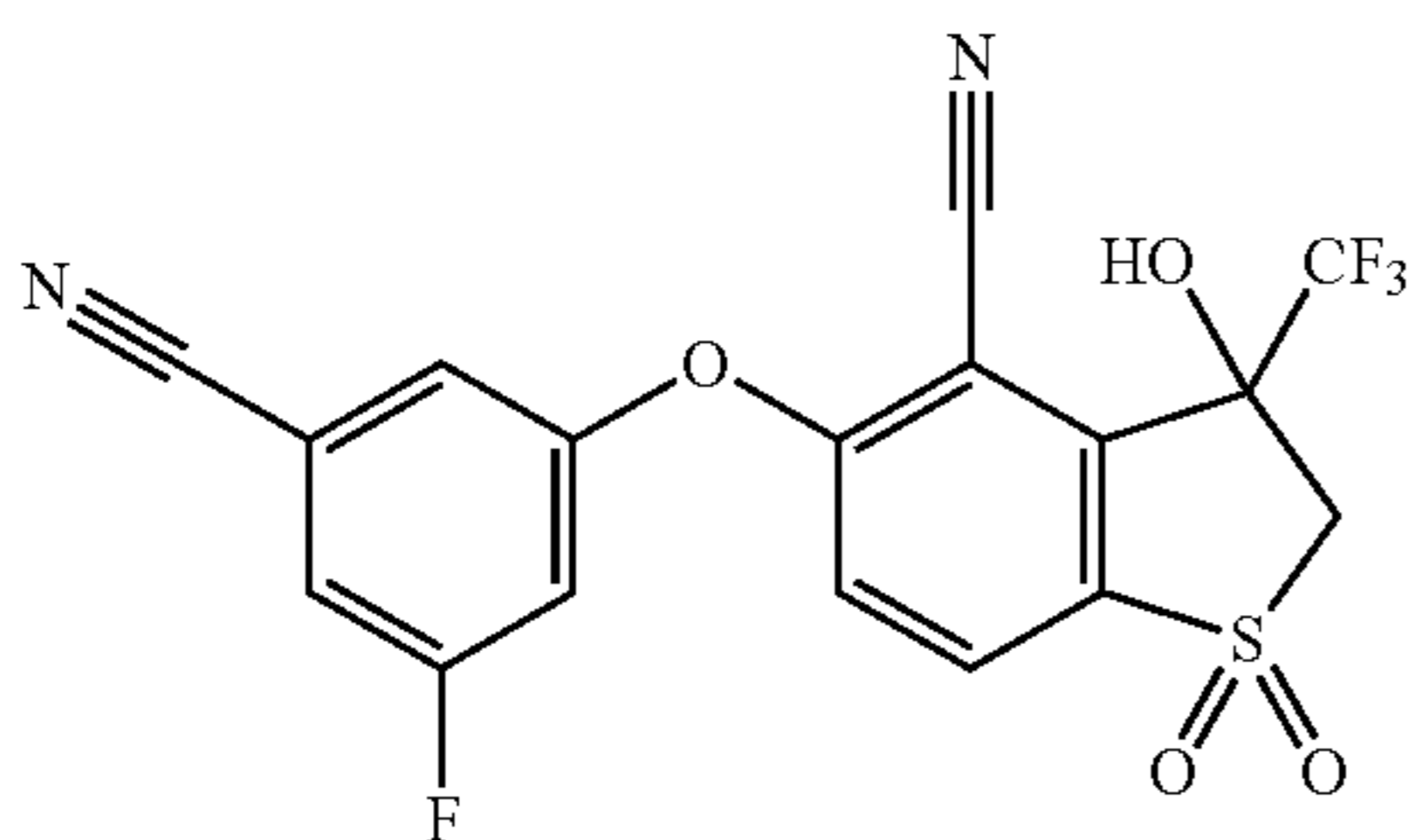
5-(3-Cyano-5-fluorophenoxy)-3-hydroxy-3-(trifluoromethyl)-2,3-dihydrobenzo[b]thiophene-4-carbonitrile 1,1-dioxide (Compound 104)
