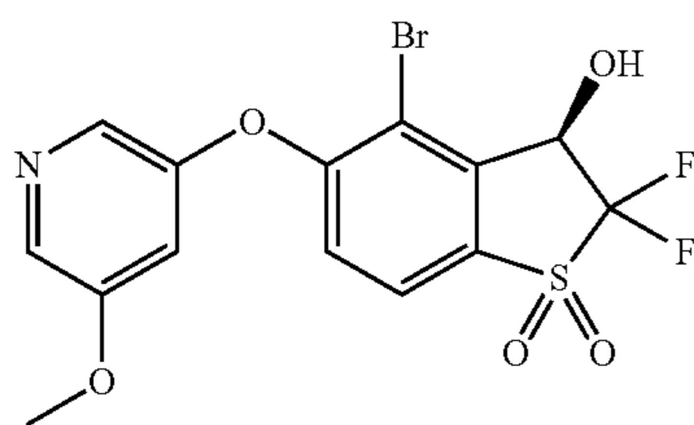
(R)-4-bromo-2,2-difluoro-3-hydroxy-5-((5-methoxy- pyridin-3-yl)oxy)-2,3-dihydrobenzo[b]thiophene 1,1-dioxide (Compound 83)
