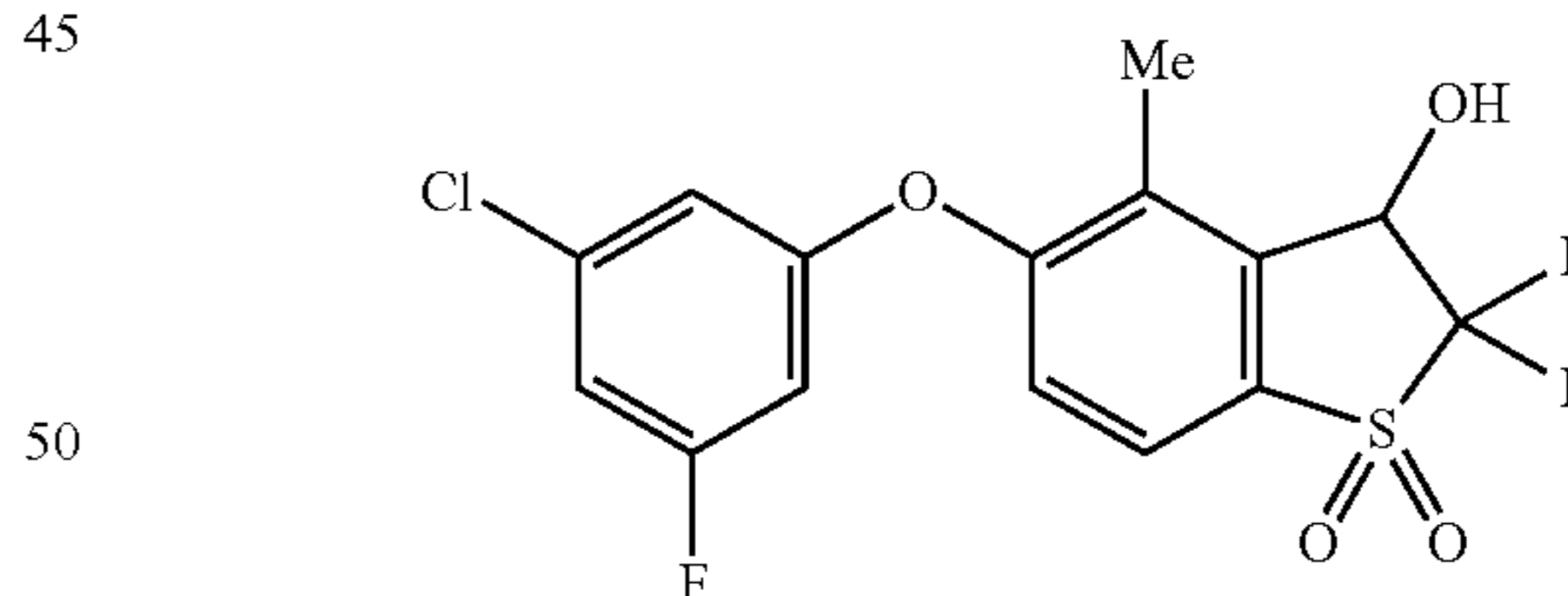
5-(3-Chloro-5-fluorophenoxy)-2,2-difluoro-3-hydroxy-4-methyl-2,3-dihydrobenzo[b]thiophene 1,1-dioxide (Compound 13)
