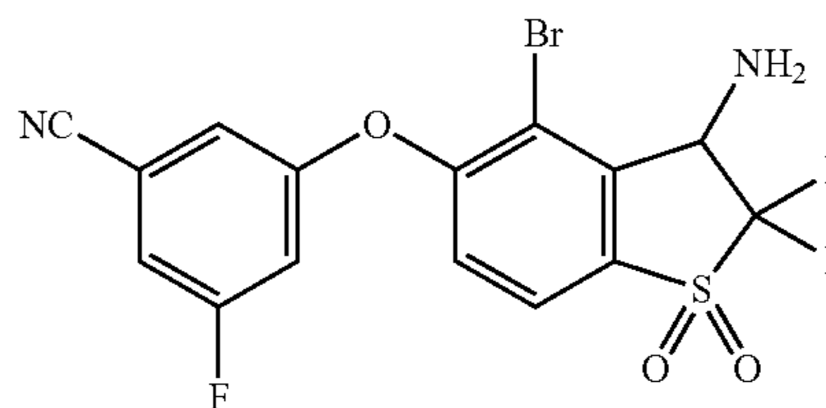
3-Amino-4-bromo-5-(3,5-difluorophenoxy)-2,2-difluoro-2,3-dihydrobenzo[b]thiophene 1,1-dioxide (Compound 30)
