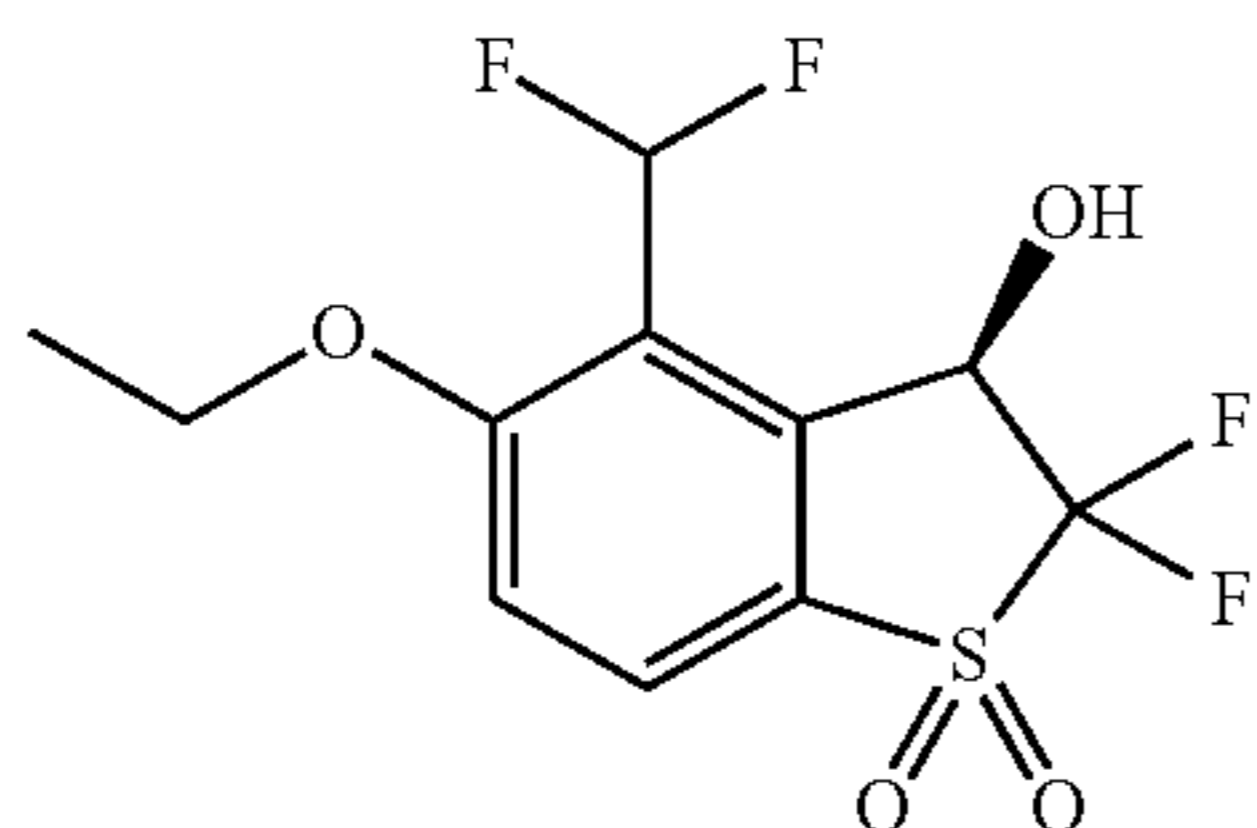
(R)-4-(Difluoromethyl)-5-ethoxy-2,2-difluoro-3-hydroxy-2,3-dihydrobenzo[b]thiophene 1,1-dioxide (Compound 92)
