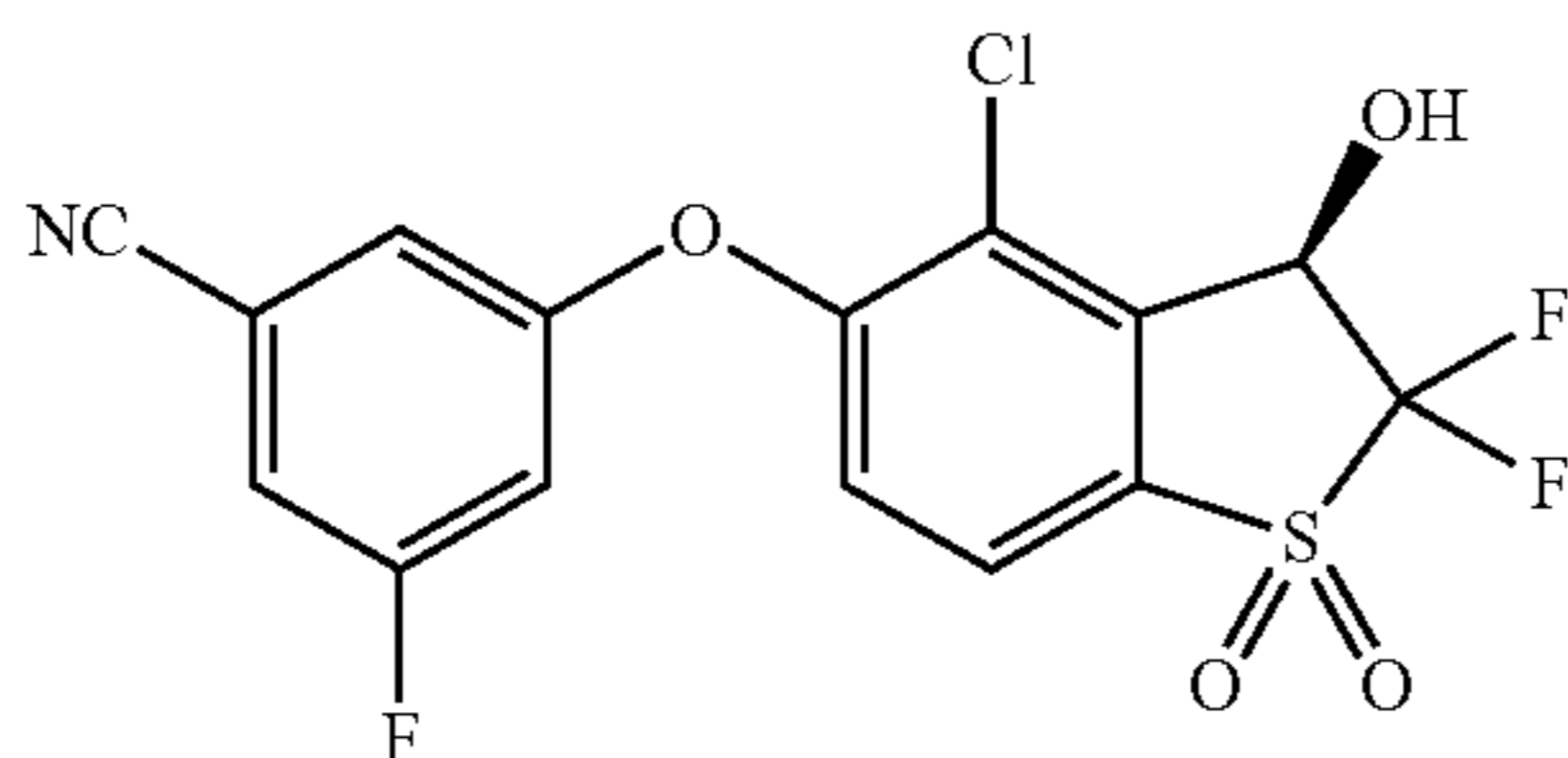
(R)-3-((4-chloro-2,2-difluoro-3-hydroxy-1,1-di- oxido-2,3-dihydrobenzo[b]thiophen-5-yl)oxy)-5- fluorobenzonitrile (Compound 85)
