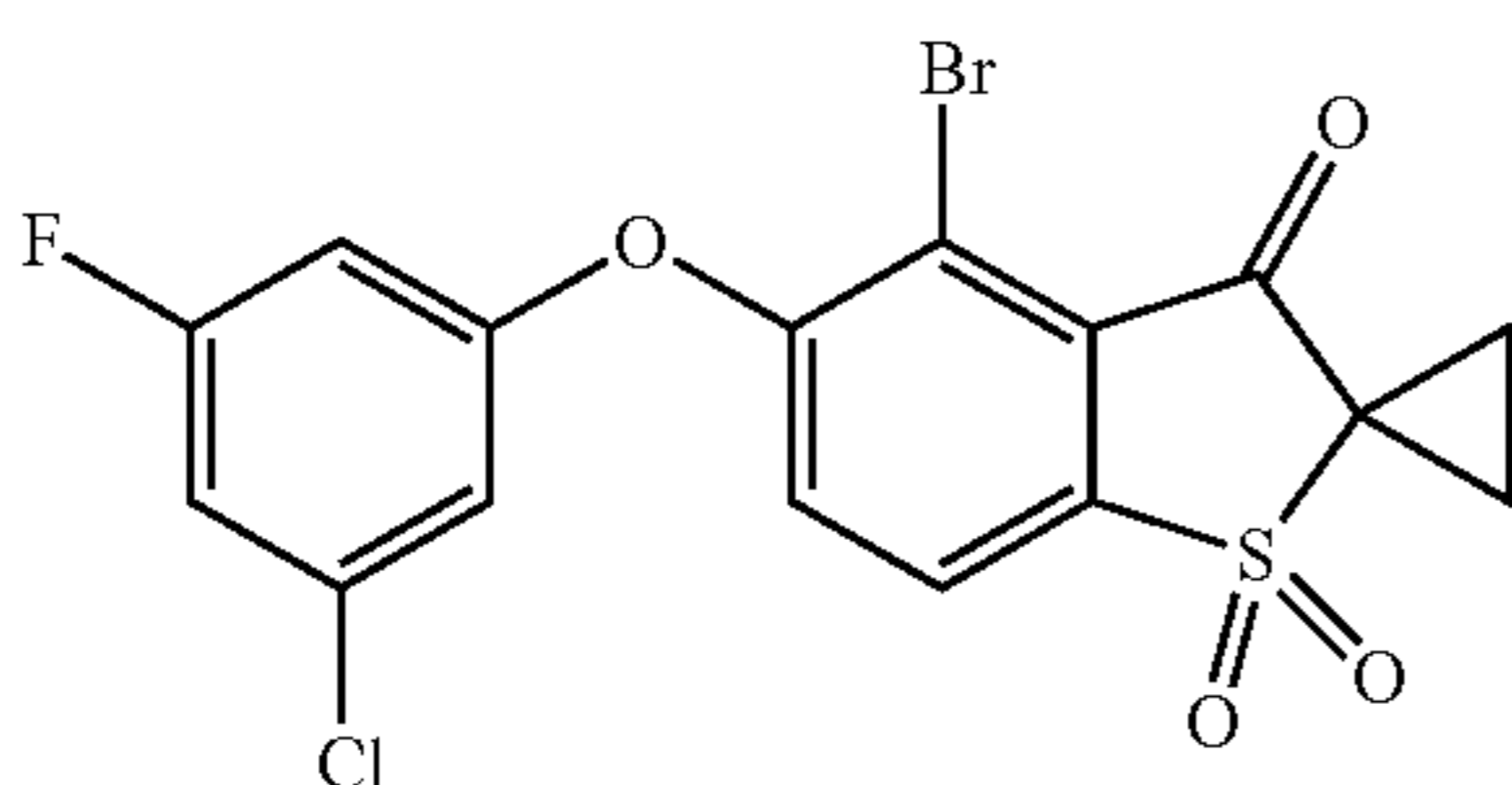
4-Bromo-5-(3-chloro-5-fluoro-phenoxy)-1,1-dioxo-spiro[benzothiophene-2,1'-cyclopropane]-3-one (Compound 58)
