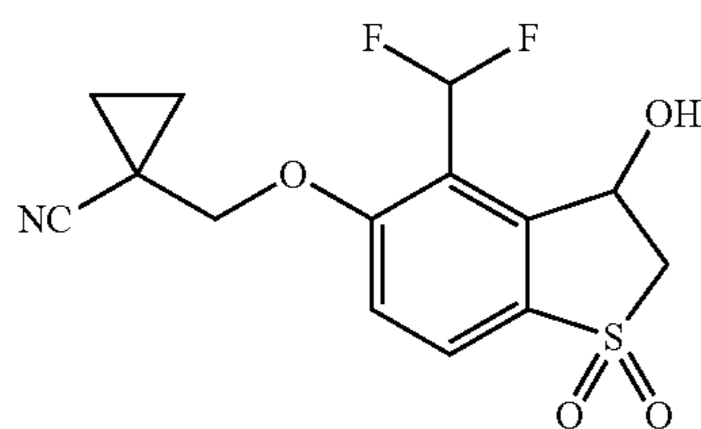
1-[[4-(difluoromethyl)-3-hydroxy-1,1-dioxo-2,3-dihydrobenzothiophen-5-yl]oxymethyl]cyclopropanecarbonitrile (Compound 108)
