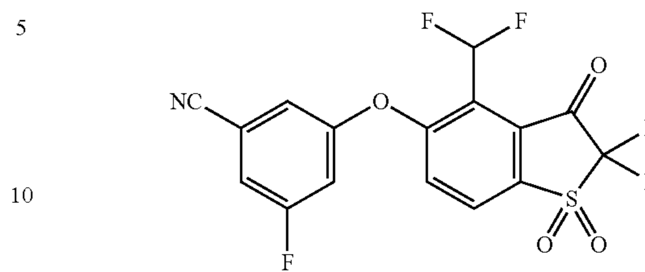
3-((4-(Difluoromethyl)-2,2-difluoro-1,1-dioxido-3-oxo-2,3-dihydrobenzo[b]thiophen-5-yl)oxy)-5-fluorobenzonitrile (Compound 39)
