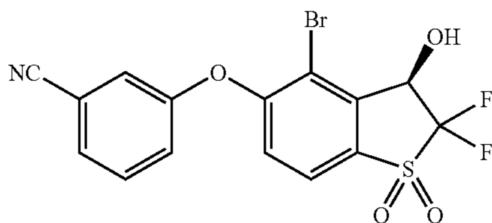
(R)-3-((4-bromo-2,2-difluoro-3-hydroxy-1,1-di- oxido-2,3-dihydrobenzo[b]thiophen-5-yl)oxy)benzo- nitrile (Compound 84)
