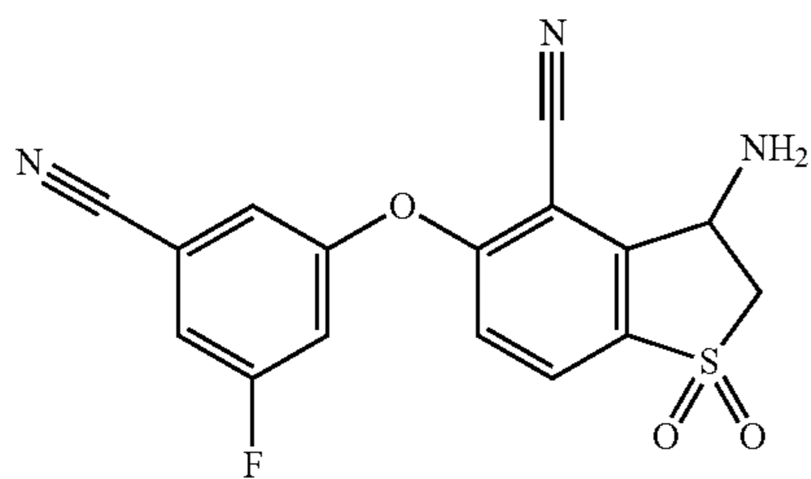
3-Amino-5-(3-cyano-5-fluorophenoxy)-2,3-dihydrobenzo[b]thiophene-4-carbonitrile 1,1-dioxide (Compound 117)
