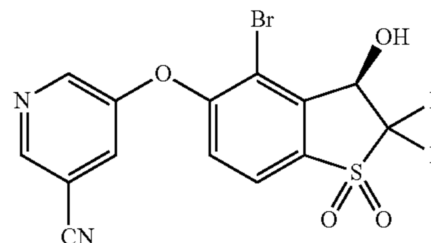
(R)-5-((4-bromo-2,2-difluoro-3-hydroxy-1,1-dioxido-2,3-dihydrobenzo[b]thiophen-5-yl)oxy)nicotinonitrile (Compound 78)
