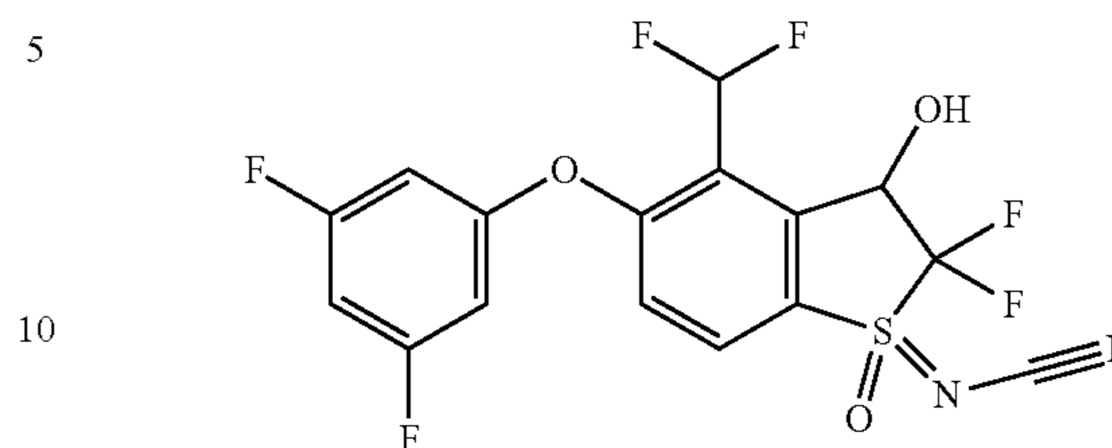
N-(4-(Difluoromethyl)-5-(3,5-difluorophenoxy)-2,2-difluoro-3-hydroxy-1-oxido-2,3-dihydro-1 \lambda^4 -benzo[b]thiophen-1-ylidene)cyanamide (Compound 51)
