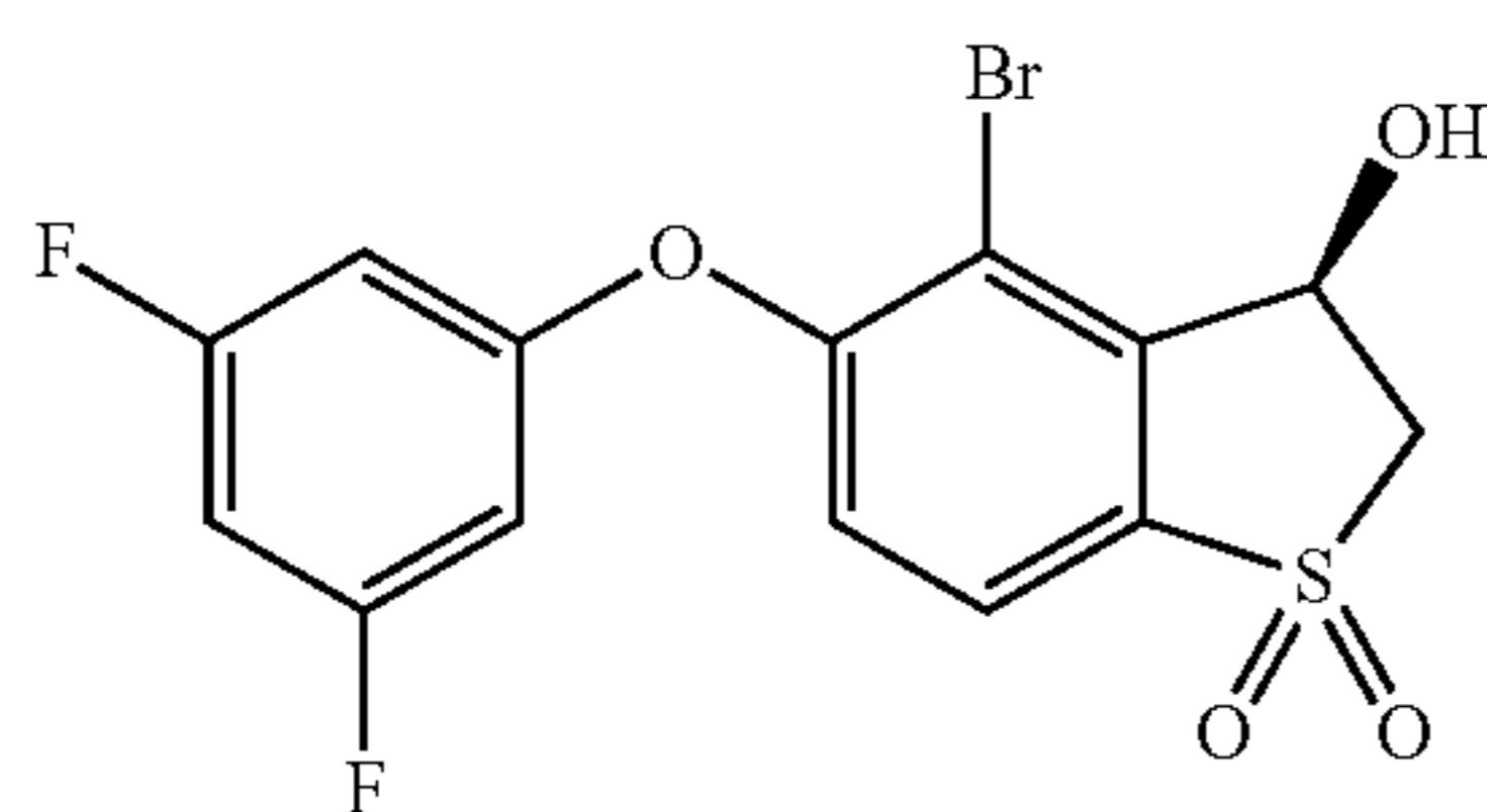
(R)-4-Bromo-5-(3,5-difluorophenoxy)-3-hydroxy-2,3-dihydrobenzo[b]thiophene 1,1-dioxide (Compound 67)
