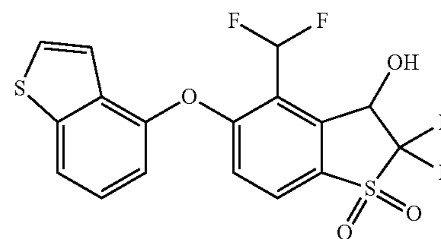
5-(Benzo[b]thiophen-4-yloxy)-4-(difluoromethyl)-2,2-difluoro-3-hydroxy-2,3-dihydrobenzo[b]thiophene 1,1-dioxide (Compound 94)
