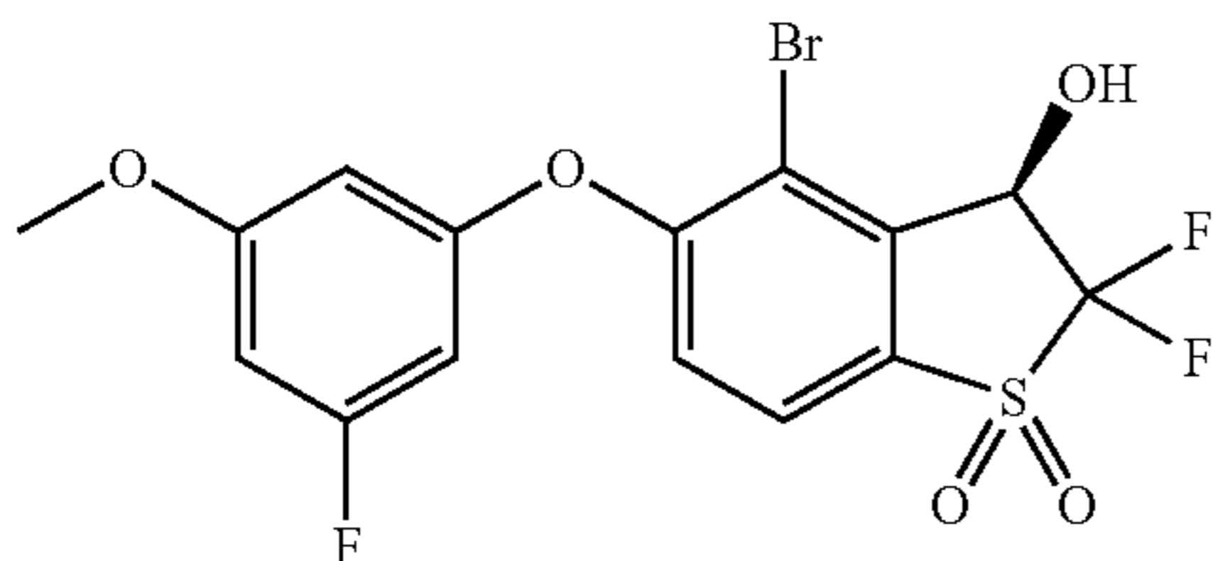
(R)-4-Bromo-2,2-difluoro-5-(3-fluoro-5-methoxyphenoxy)-3-hydroxy-2,3-dihydrobenzo[b]thiophene 1,1-dioxide (Compound 80)
