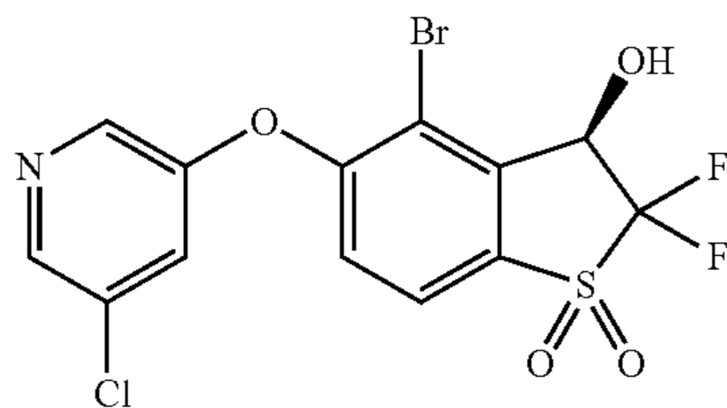
(R)-4-bromo-5-((5-chloropyridin-3-yl)oxy)-2,2-difluoro-3-hydroxy-2,3-dihydrobenzo[b]thiophene 1,1-dioxide (Compound 75)
