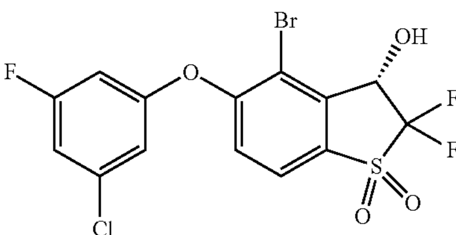
(3S)-4-Bromo-5-(3-chloro-5-fluoro-phenoxy)-2,2-difluoro-1,1-dioxo-3H-benzothiophen-3-ol (Compound 59)
