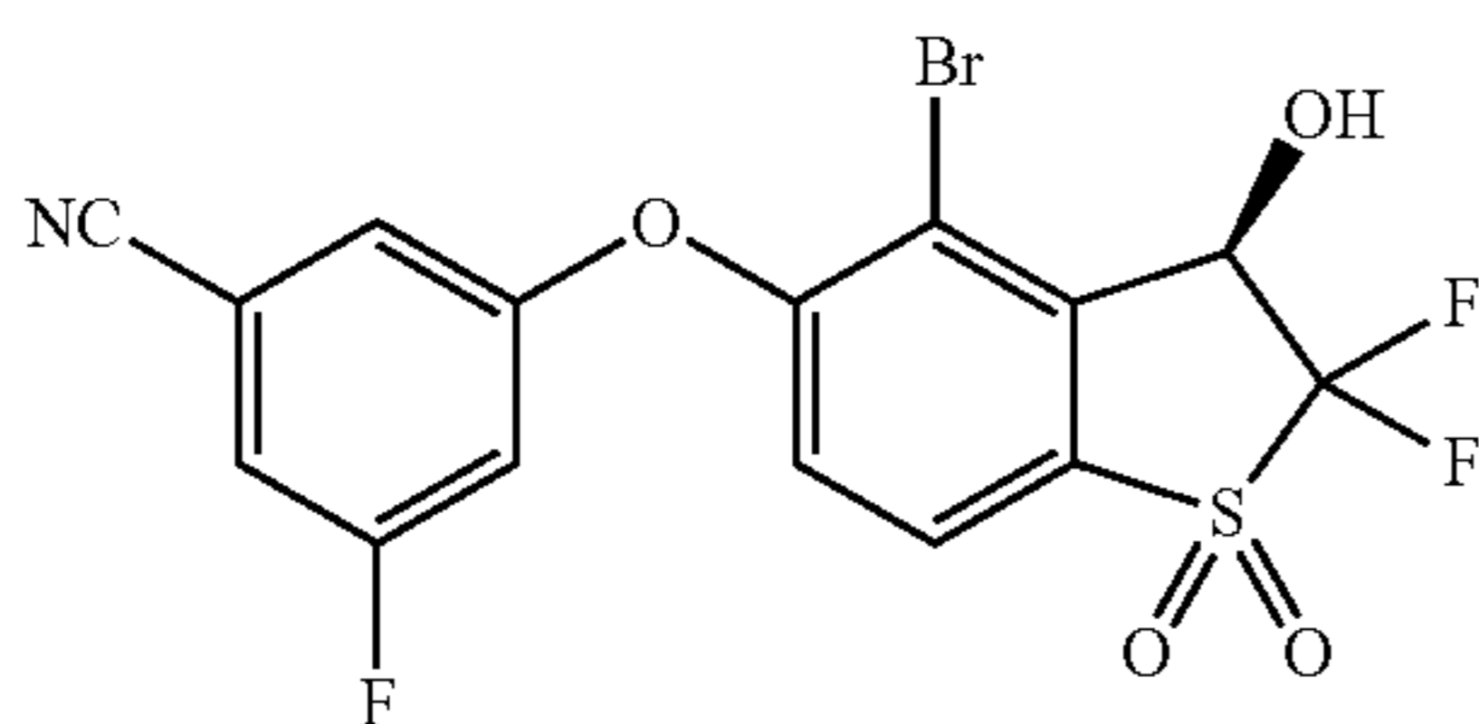
(R)-3-((4-bromo-2,2-difluoro-3-hydroxy-1,1-dioxido-2,3-dihydrobenzo[b]thiophen-5-yl)oxy)-5-fluorobenzonitrile (Compound 1)
