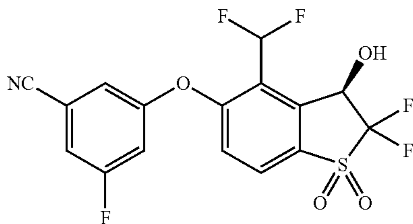
(R)-3-((4-(Difluoromethyl)-2,2-difluoro-3-hydroxy-1,1-dioxido-2,3-dihydrobenzo[b]thiophen-5-yl)oxy)-5-fluorobenzonitrile (Compound 3)
