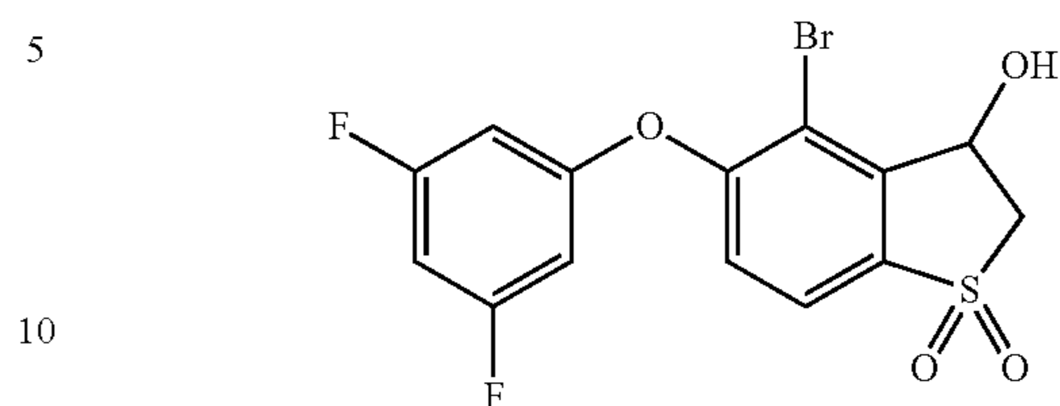
4-Bromo-5-(3,5-difluorophenoxy)-3-hydroxy-2,3-dihydrobenzo[b]thiophene 1,1-dioxide (Compound 72)
