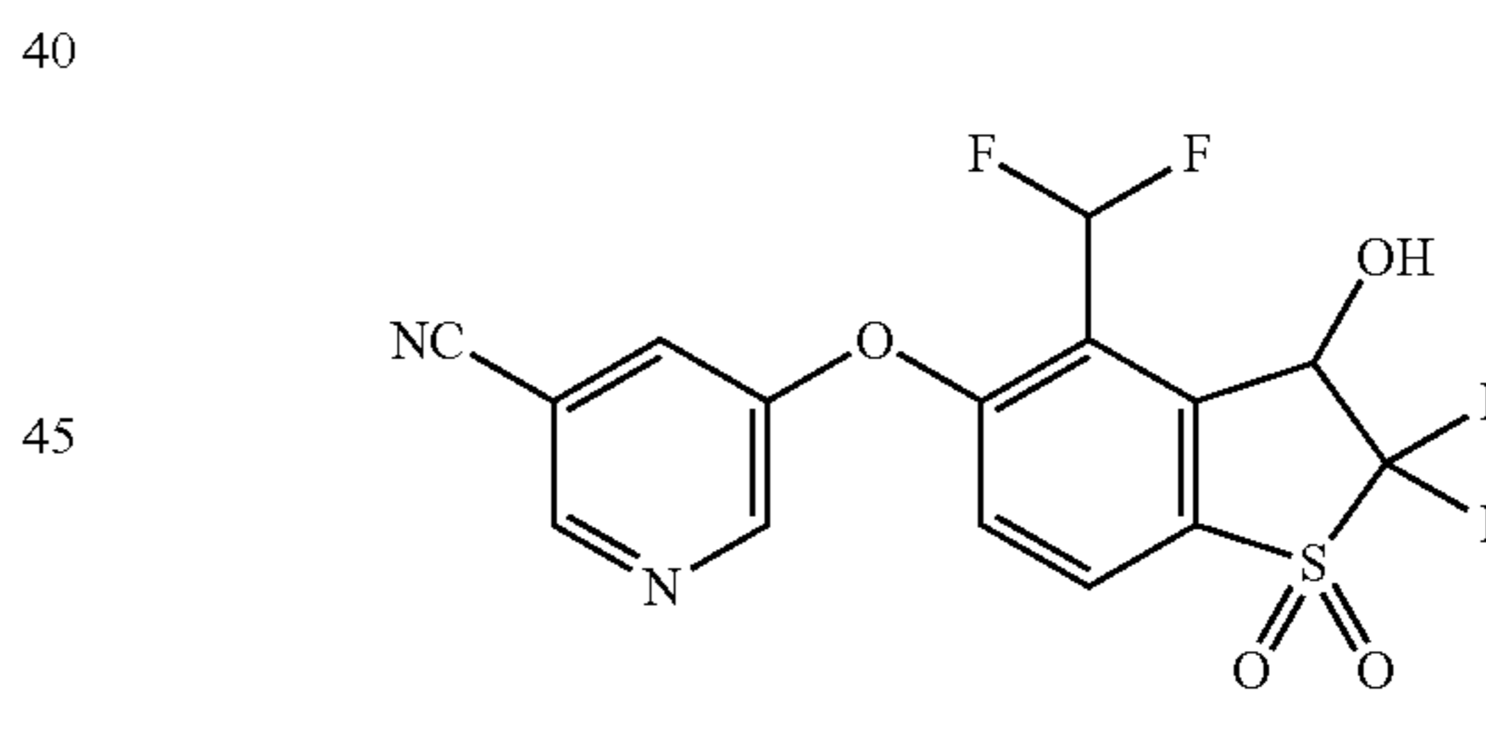
5-((4-(Difluoromethyl)-2,2-difluoro-3-hydroxy-1,1-dioxido-2,3-dihydrobenzo[b]thiophen-5-yl)oxy)nicotinonitrile (Compound 37)
