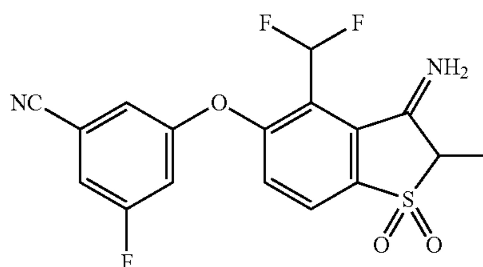
3-((3-Amino-4-(difluoromethyl)-2,2-difluoro-1,1-dioxido-2,3-dihydrobenzo[b]thiophen-5-yl)oxy)-5-fluorobenzonitrile (Compound 26) and 3-((4-(difluoromethyl)-2-fluoro-3-imino-1,1-dioxido-2,3-dihydrobenzo[b]thiophen-5-yl)oxy)-5-fluorobenzonitrile (Compound 27)
