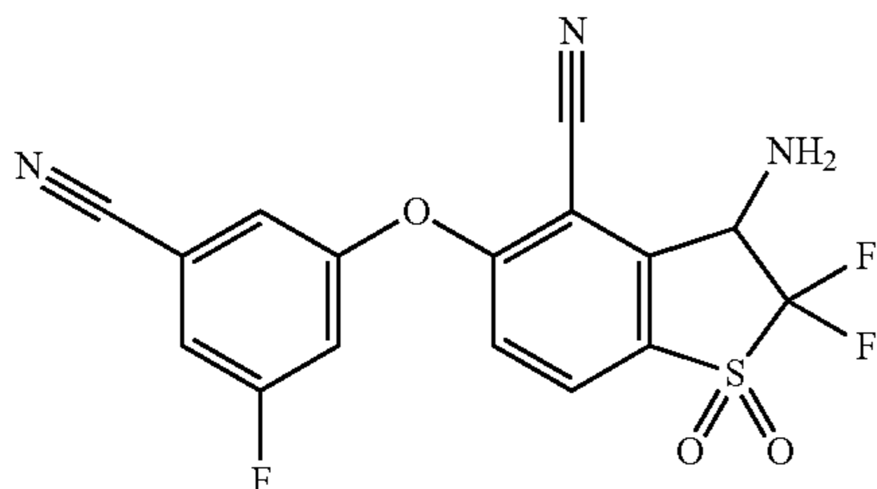
3-Amino-5-(3-cyano-5-fluorophenoxy)-2,2-difluoro-2,3-dihydrobenzo[b]thiophene-4-carbonitrile 1,1-dioxide (Compound 118)
