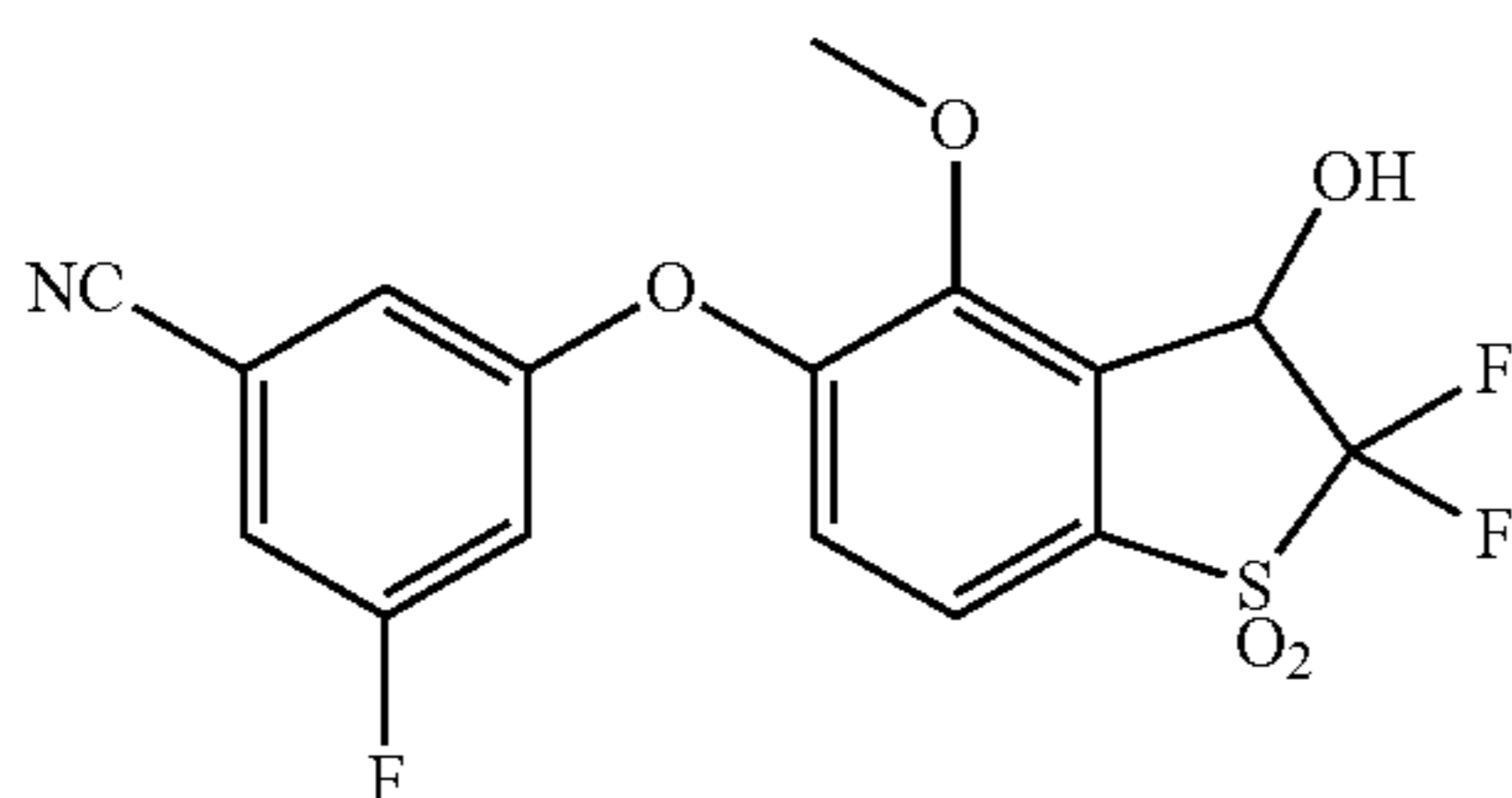
3-((2,2-Difluoro-3-hydroxy-4-methoxy-1,1-dioxido-2,3-dihydrobenzo[b]thiophen-5-yl)oxy)-5-fluorobenzonitrile (Compound 87)
