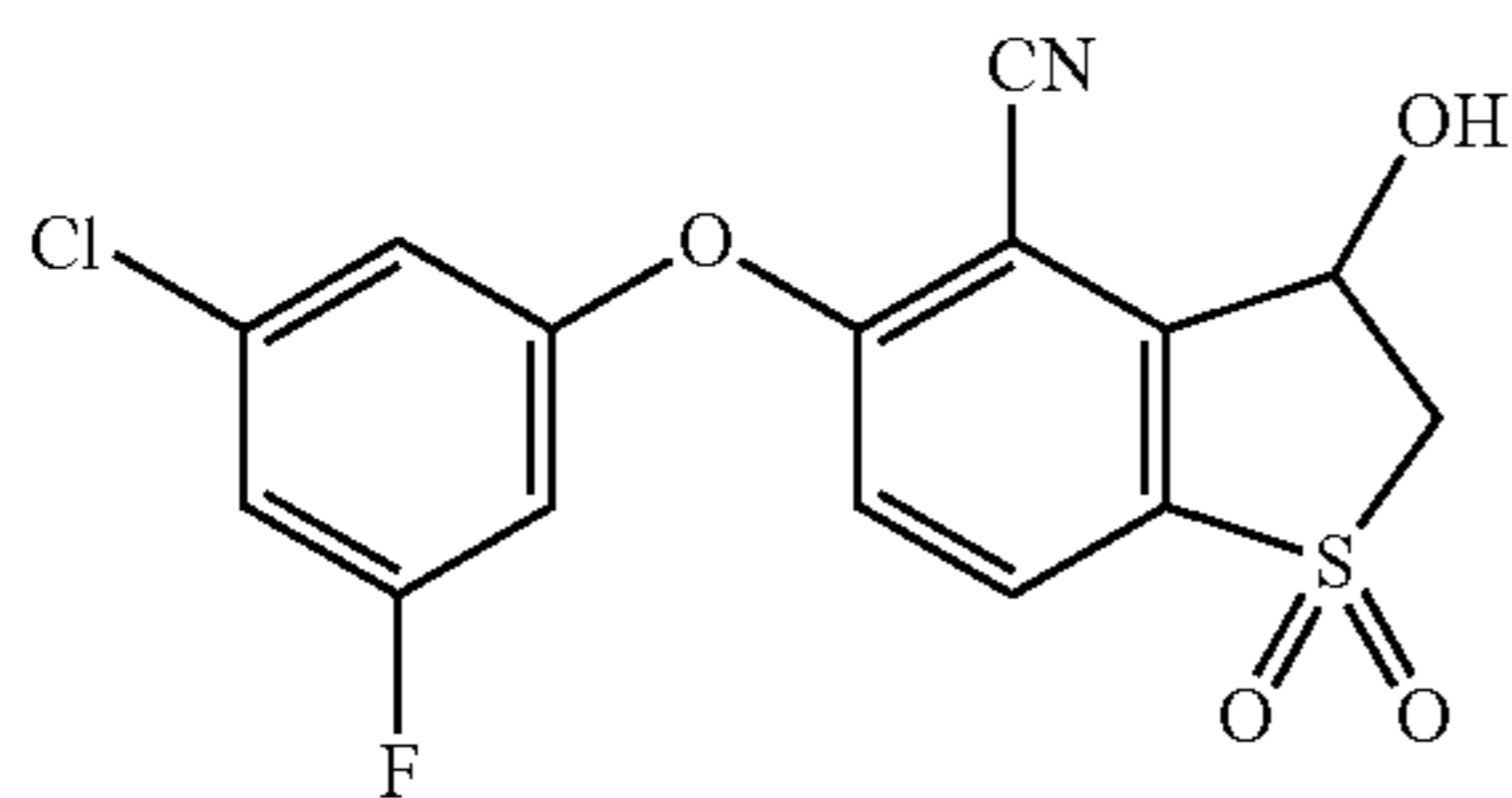
5-(3-chloro-5-fluorophenoxy)-3-hydroxy-2,3-dihydrobenzo[b]thiophene-4-carbonitrile 1,1-dioxide (Compound 7)
