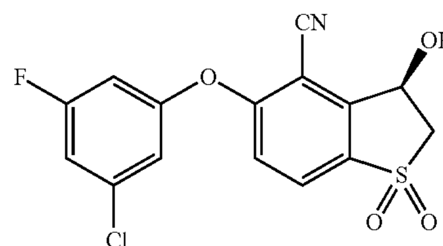
(3R)-5-(3-Chloro-5-fluoro-phenoxy)-3-hydroxy-1,1-dioxo-2,3-dihydrobenzothiophene-4-carbonitrile (Compound 2)
