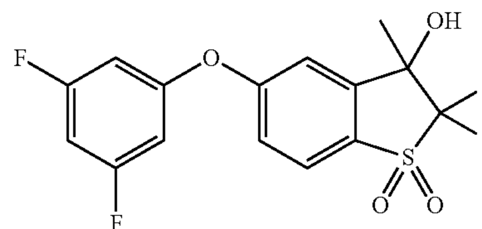
5-(3,5-Di fluorophenoxy)-2,2-difluoro-3-hydroxy-3-methyl-2,3-dihydrobenzo[b]thiophene 1,1-dioxide (Compound 79)
