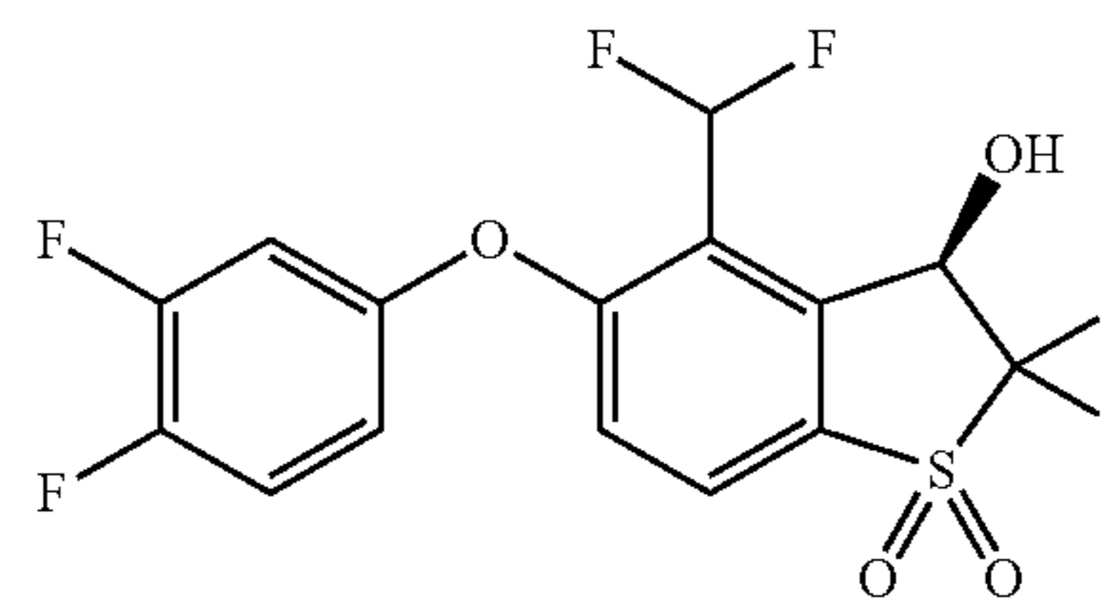
(R)-4-(Difluoromethyl)-5-(3,4-difluorophenoxy)-2,2-difluoro-3-hydroxy-2,3-dihydrobenzo[b]thiophene 1,1-dioxide (Compound 90)
