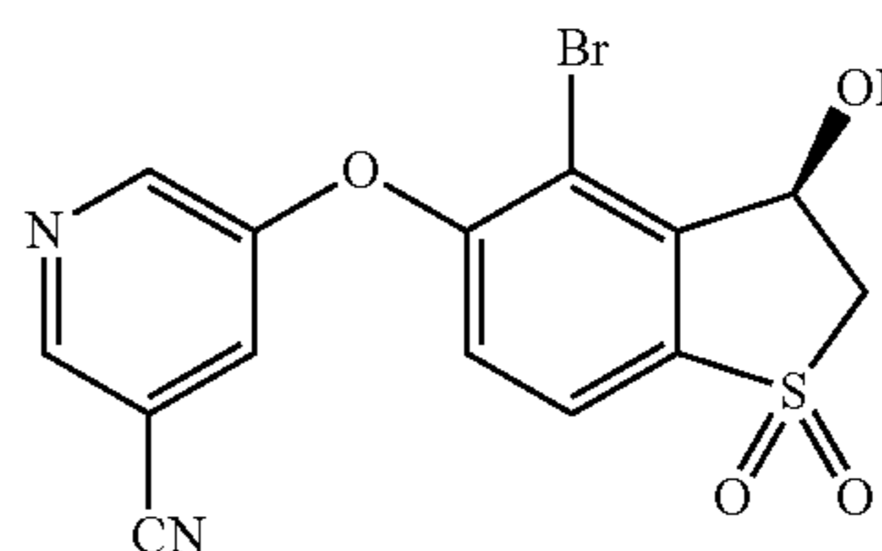
(R)-5-((4-bromo-3-hydroxy-1,1-dioxido-2,3-dihydrobenzo[b]thiophen-5-yl)oxy)nicotinonitrile (Compound 74)
