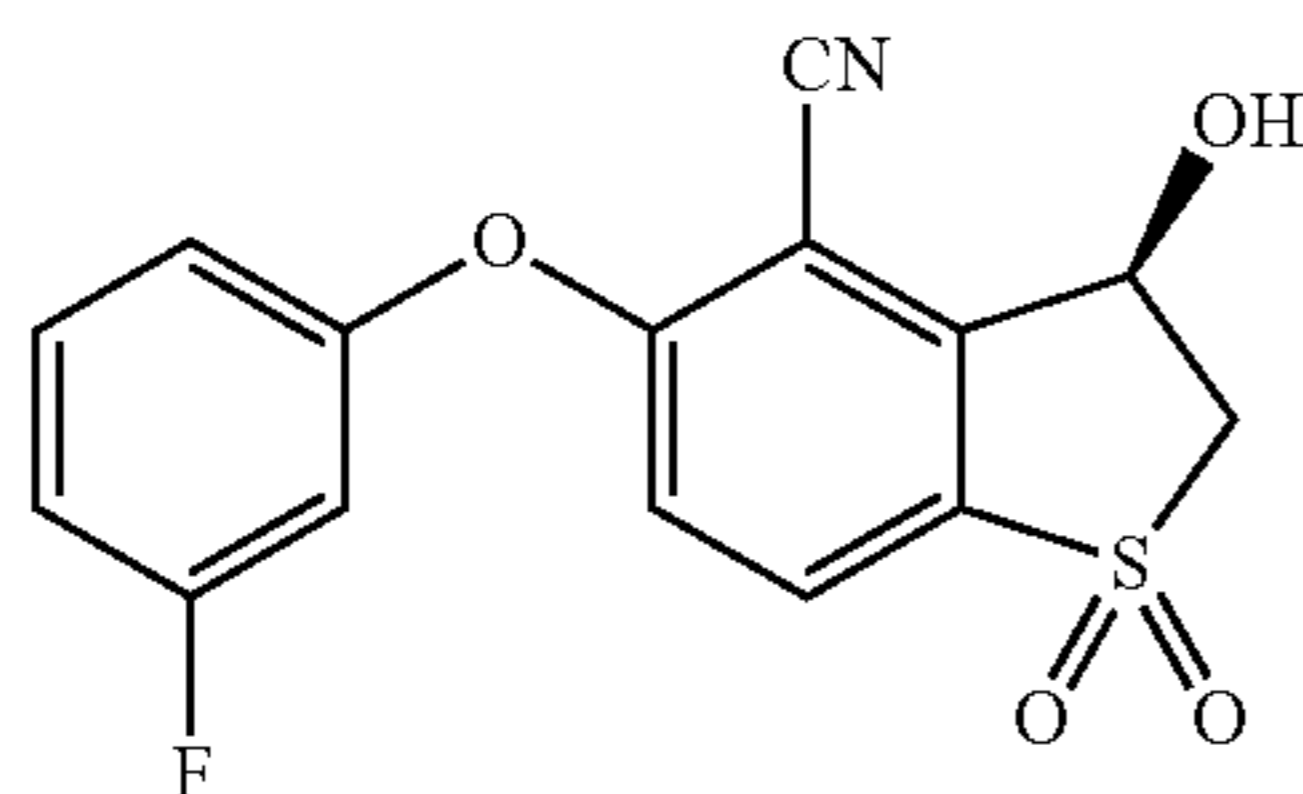
(R)-5-(3-fluorophenoxy)-3-hydroxy-2,3-dihydrobenzo[b]thiophene-4-carbonitrile 1,1-dioxide (Compound 76)
