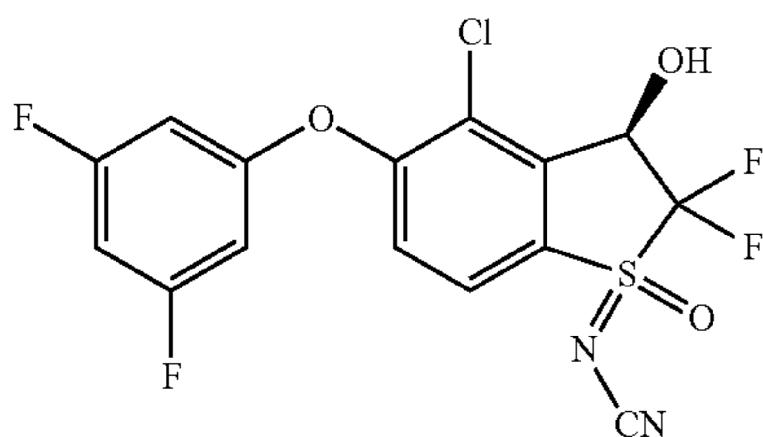
N-((3R)-4-Chloro-5-(3,5-difluorophenoxy)-2,2-difluoro-3-hydroxy-1-oxido-2,3-dihydro-1λ 4 -benzo[b]thiophen-1-ylidene)cyanamide (Compound 66)
