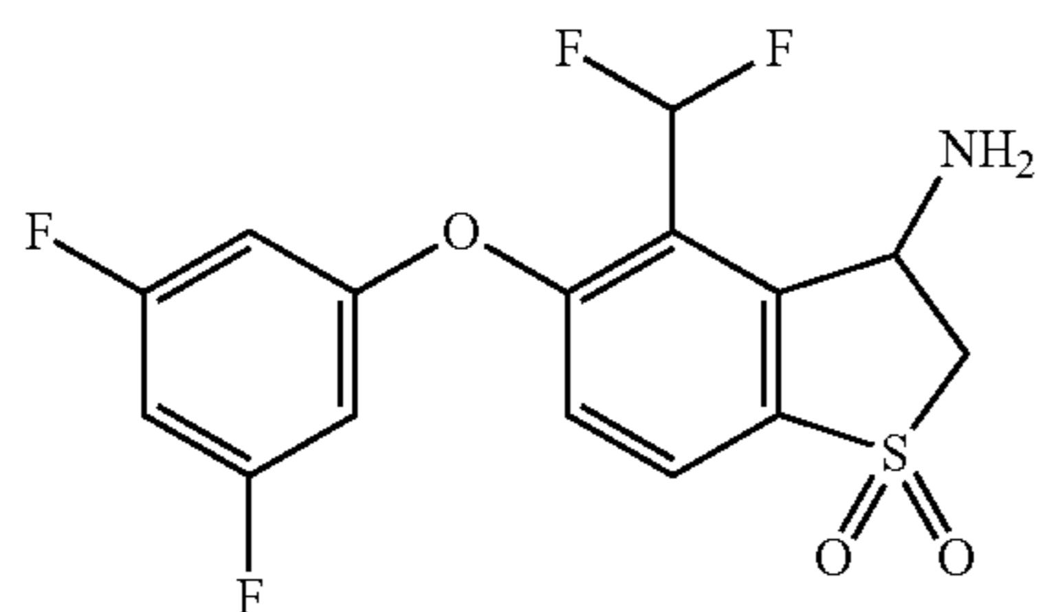
3-Amino-4-(difluoromethyl)-5-(3,5-difluorophenoxy)-2-fluoro-2,3-dihydrobenzo[b]thiophene 1,1-dioxide (Compound 21)
