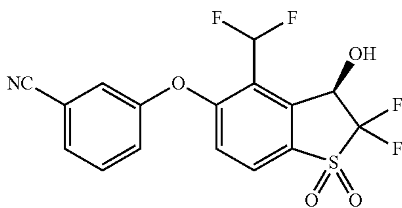
(R)-3-((4-(difluoromethyl)-2,2-difluoro-3-hydroxy-1,1-dioxido-2,3-dihydrobenzo[b]thiophen-5-yl)oxy)benzonitrile (Compound 89)
