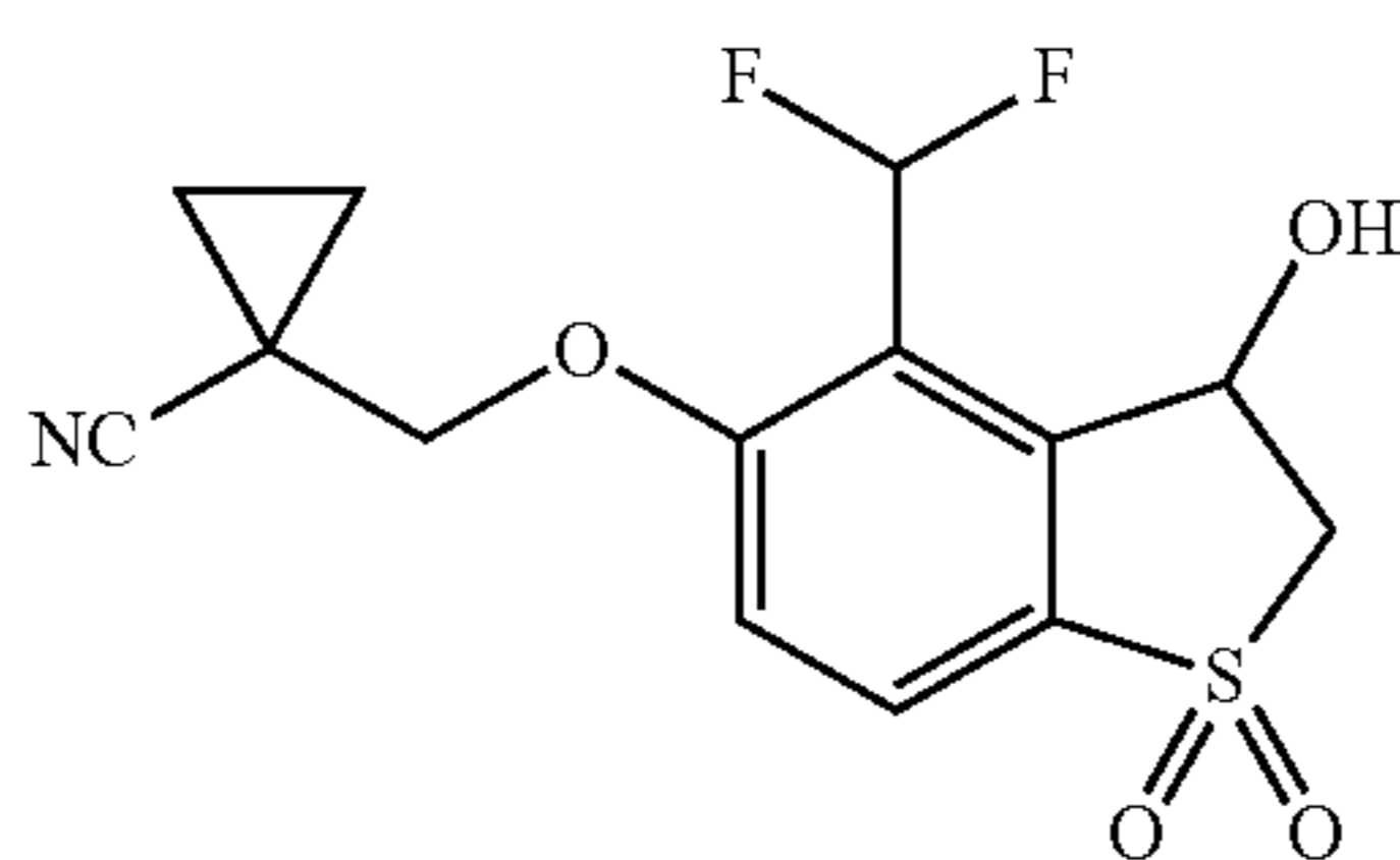
1-[[4-(difluoromethyl)-3-hydroxy-1,1-dioxo-2,3-dihydrobenzothiophen-5-yl]oxymethyl]cyclopropanecarbonitrile (Compound 108)
