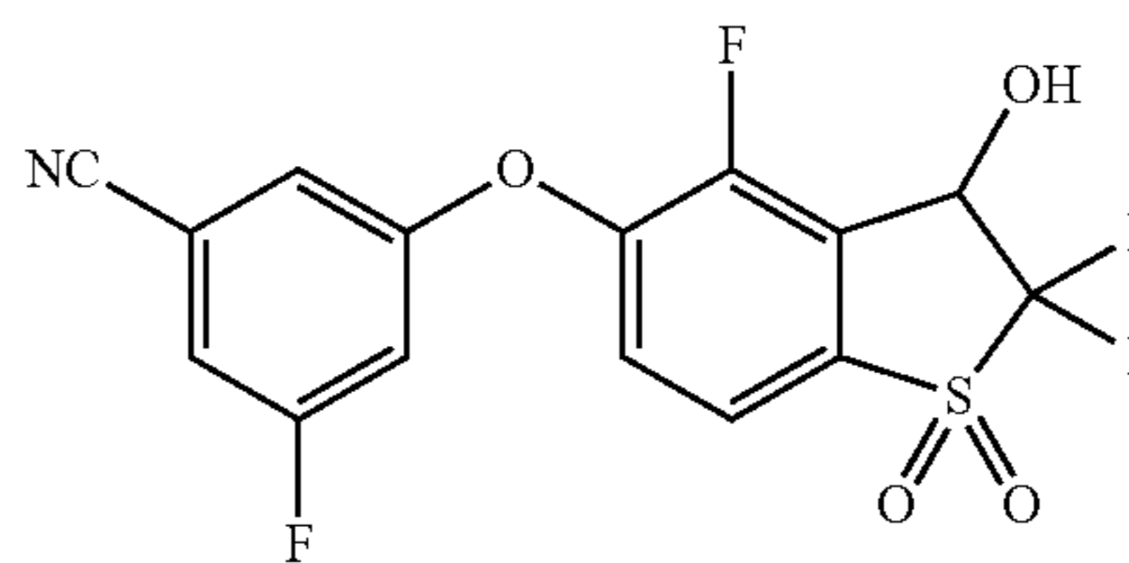
3-Fluoro-5-((2,2,4-trifluoro-3-hydroxy-1,1-dioxido-2,3-dihydrobenzo[b]thiophen-5-yl)oxy)benzonitrile (Compound 88)
