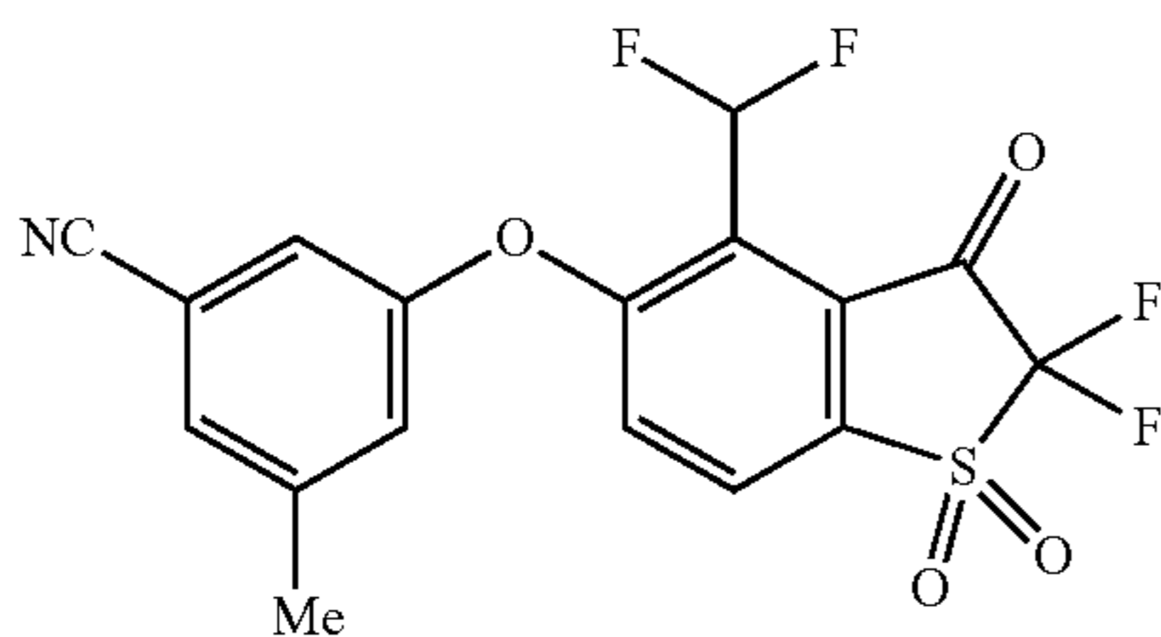
3-((4-(Difluoromethyl)-2,2-difluoro-1,1-dioxido-3-oxo-2,3-dihydrobenzo[b]thiophen-5-yl)oxy)-5-methylbenzonitrile (Compound 45)
