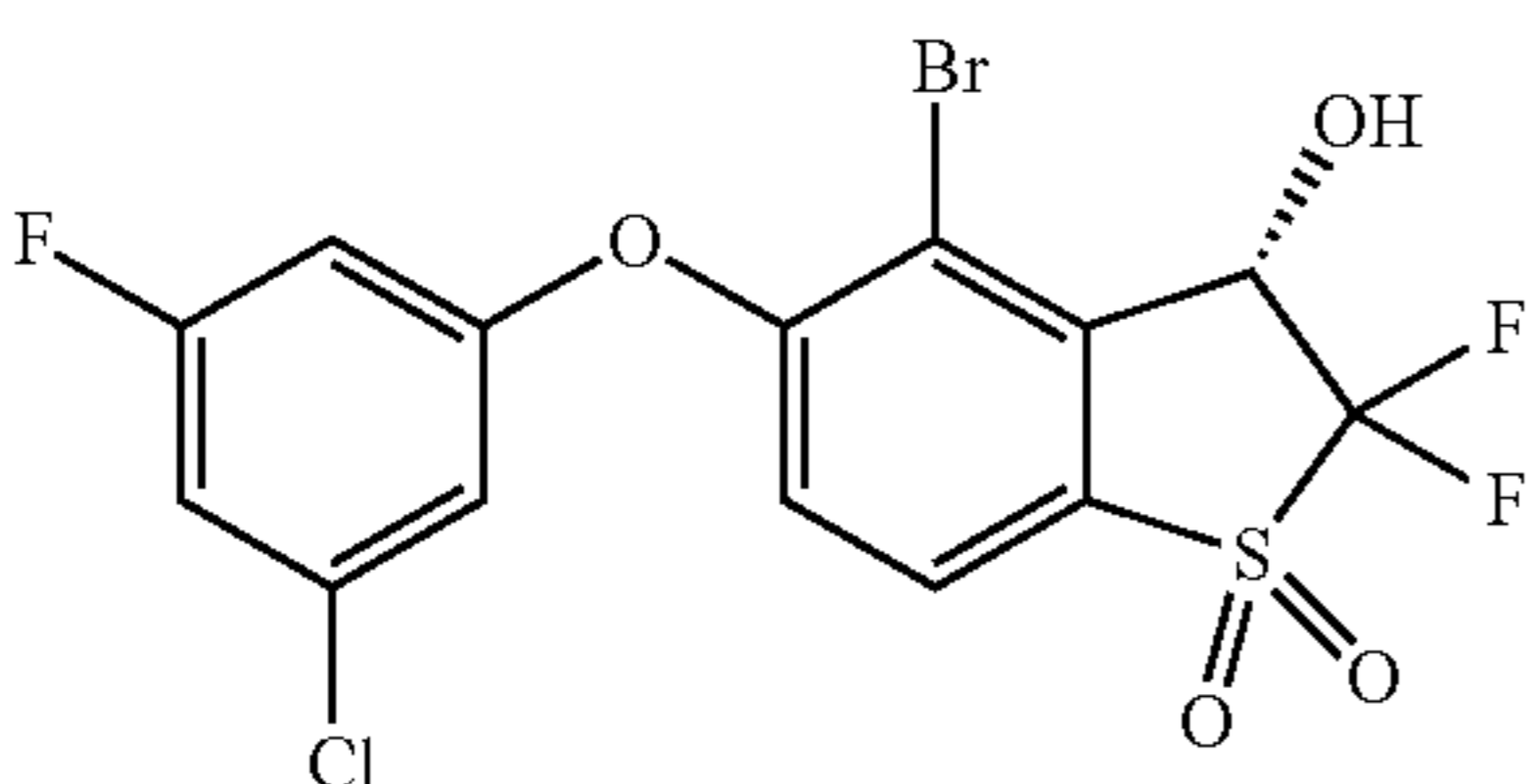
(3S)-4-Bromo-5-(3-chloro-5-fluoro-phenoxy)-2,2-difluoro-1,1-dioxo-3H-benzothiophen-3-ol (Compound 59)
