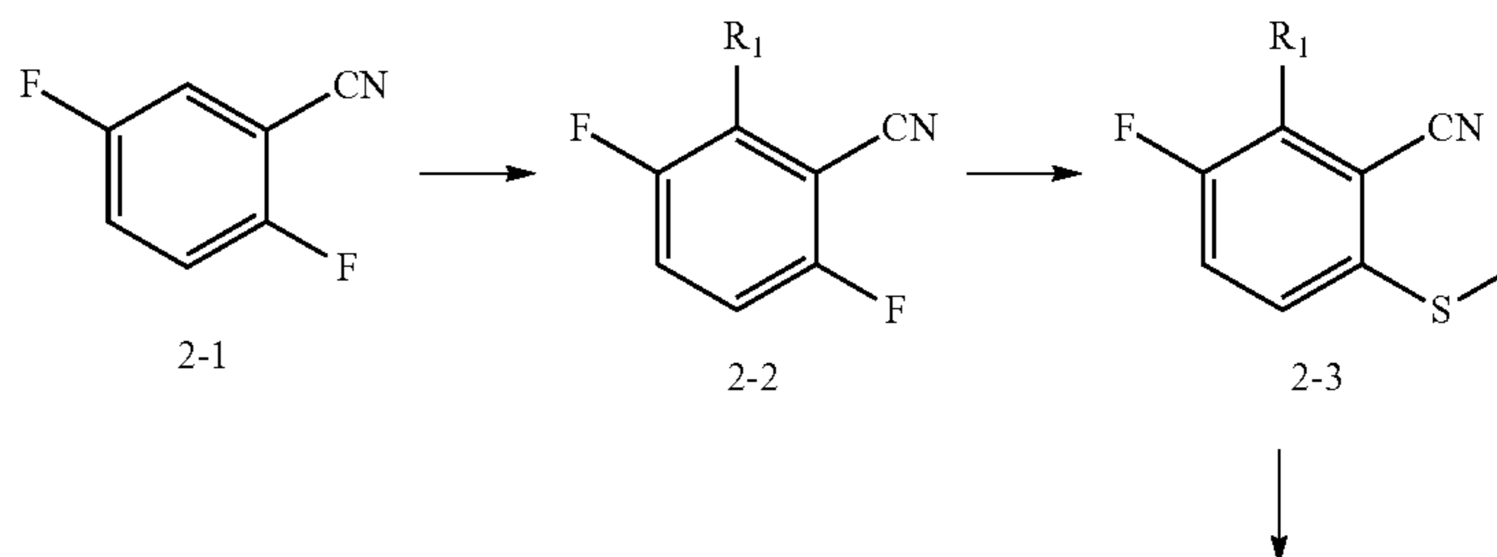
Scheme 2
