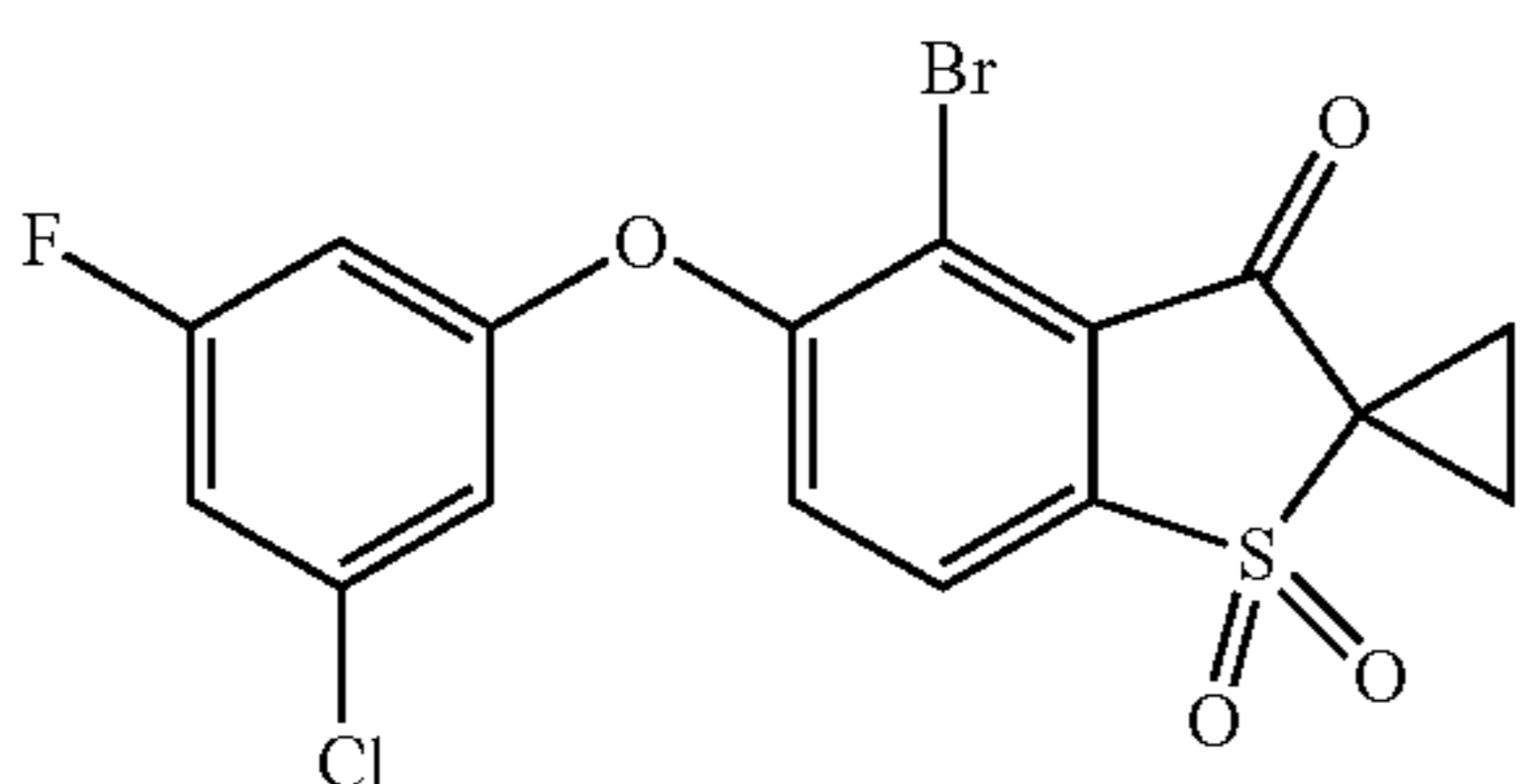
4-Bromo-5-(3-chloro-5-fluoro-phenoxy)-1,1-dioxo-spiro[benzothiophene-2,1'-cyclopropane]-3-one (Compound 58)
