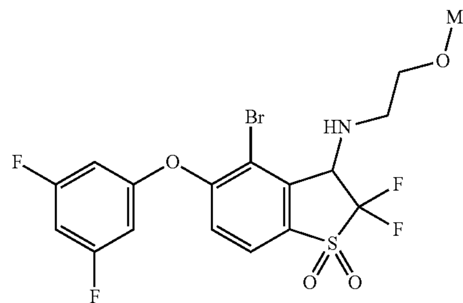
4-Bromo-5-(3,5-difluorophenoxy)-2,2-difluoro-3-((2-methoxyethyl)amino)-2,3-dihydrobenzo[b]thiophene 1,1-dioxide (Compound 33)
