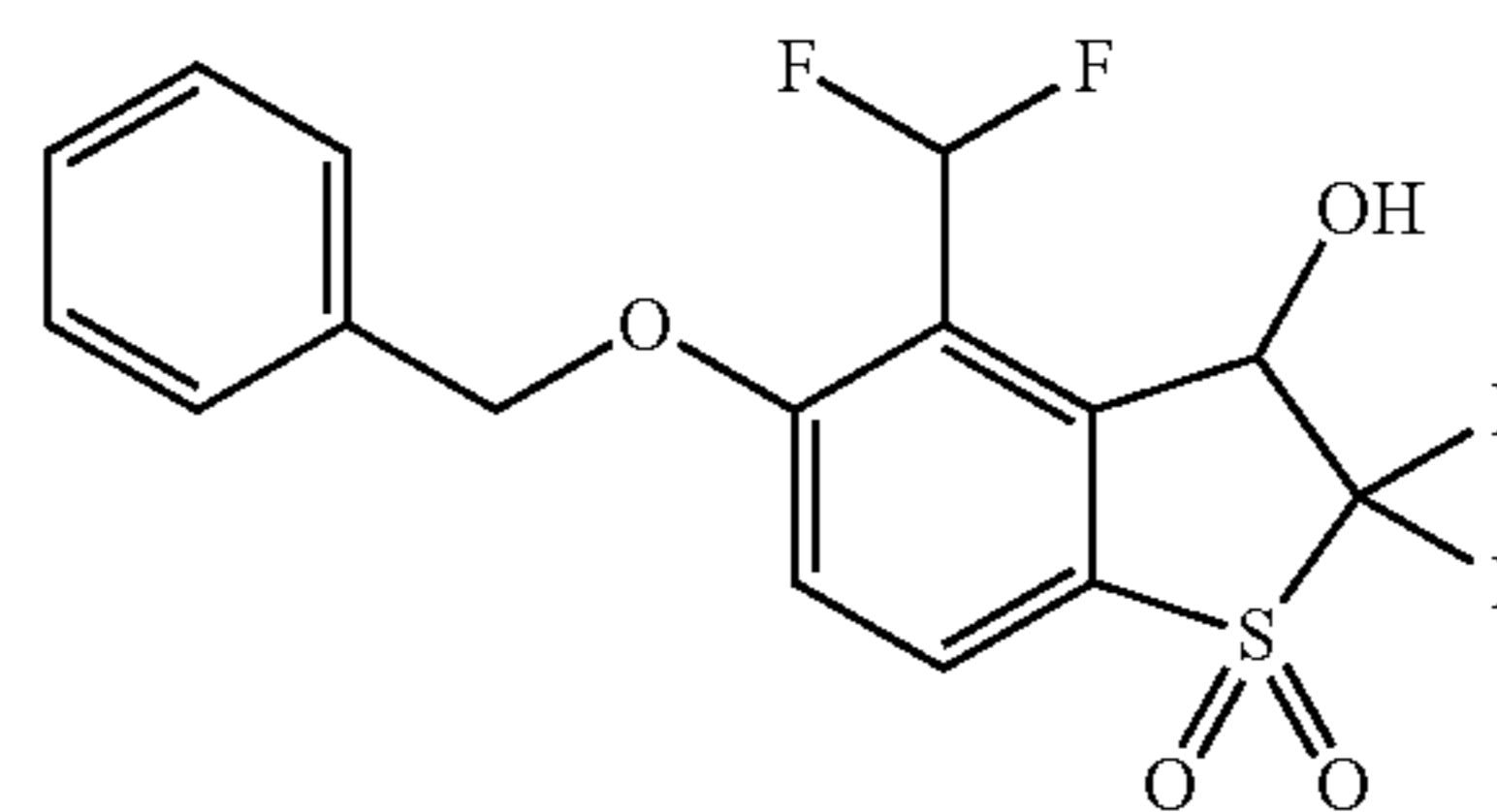
5-Benzyloxy-4-(difluoromethyl)-2,2-difluoro-1,1-dioxo-3H-benzothiophen-3-ol (Compound 65)
