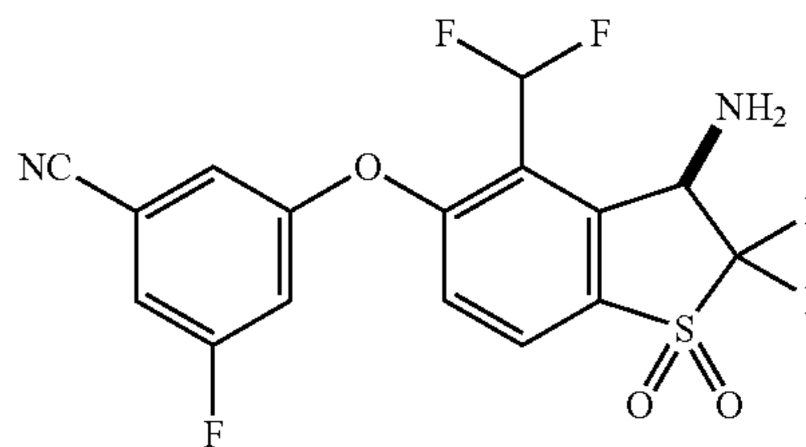
(R)-3-((3-Amino-4-(difluoromethyl)-2,2-difluoro-1,1-dioxido-2,3-dihydrobenzo[b]thiophen-5-yl)oxy)-5-fluorobenzonitrile (Compound 41)
