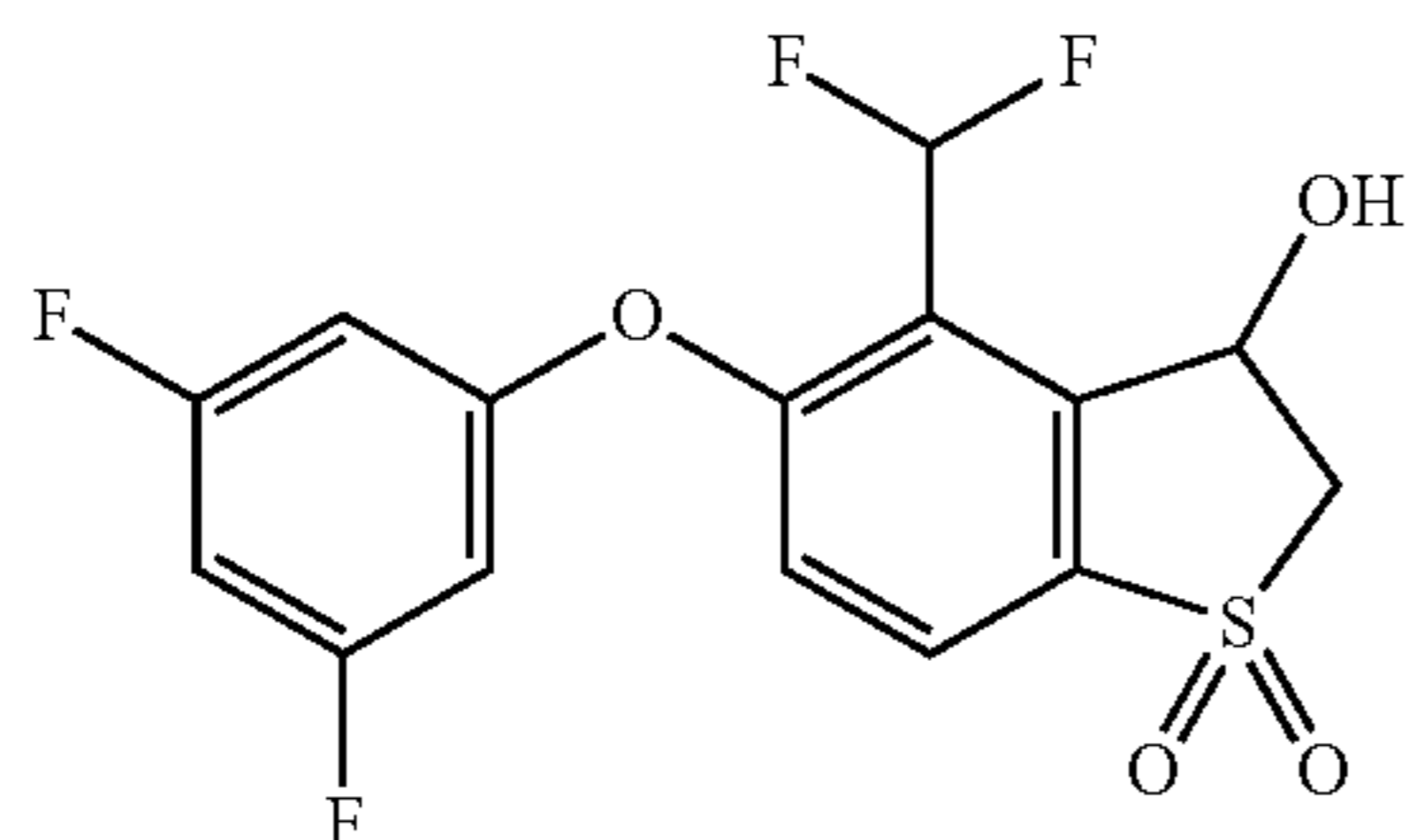
4-(Difluoromethyl)-5-(3,5-difluorophenoxy)-3-hydroxy-2,3-dihydrobenzo[b]thiophene 1,1-dioxide (Compound 24)
