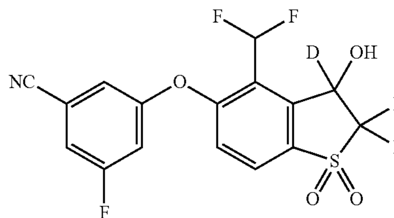
3-((4-(Difluoromethyl)-2,2-difluoro-3-hydroxy-1,1-dioxido-2,3-dihydrobenzo[b]thiophen-5-yl-3-d)oxy)-5-fluorobenzonitrile (Compound 40)
