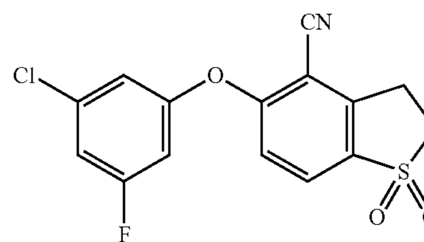
5-(3-Chloro-5-fluorophenoxy)-2,3-dihydrobenzo[b]thiophene-4-carbonitrile 1,1-dioxide (Compound 5)
