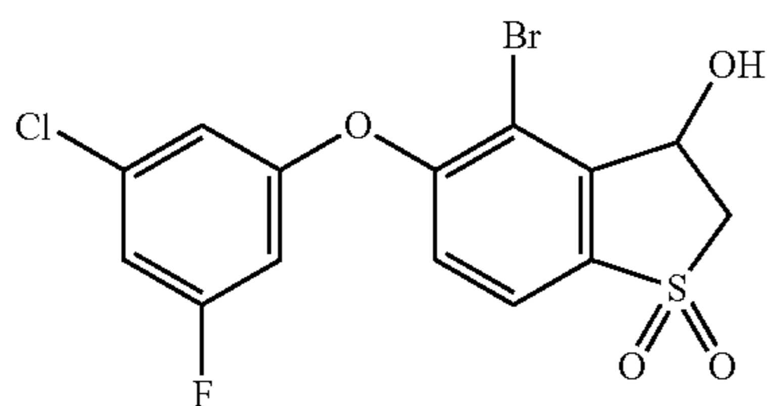
4-Bromo-5-(3-chloro-5-fluorophenoxy)-3-hydroxy-2,3-dihydrobenzo[b]thiophene 1,1-dioxide (Compound 6)
