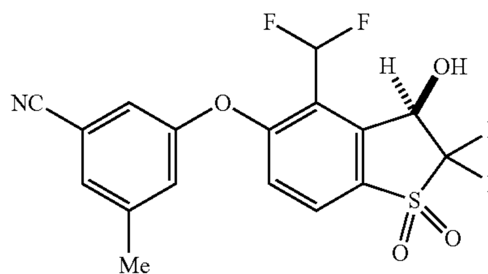
(R)-3-((4-(Difluoromethyl)-2,2-difluoro-3-hydroxy-1,1-dioxido-2,3-dihydrobenzo[b]thiophen-5-yl)oxy)-5-methylbenzonitrile (Compound 46)
