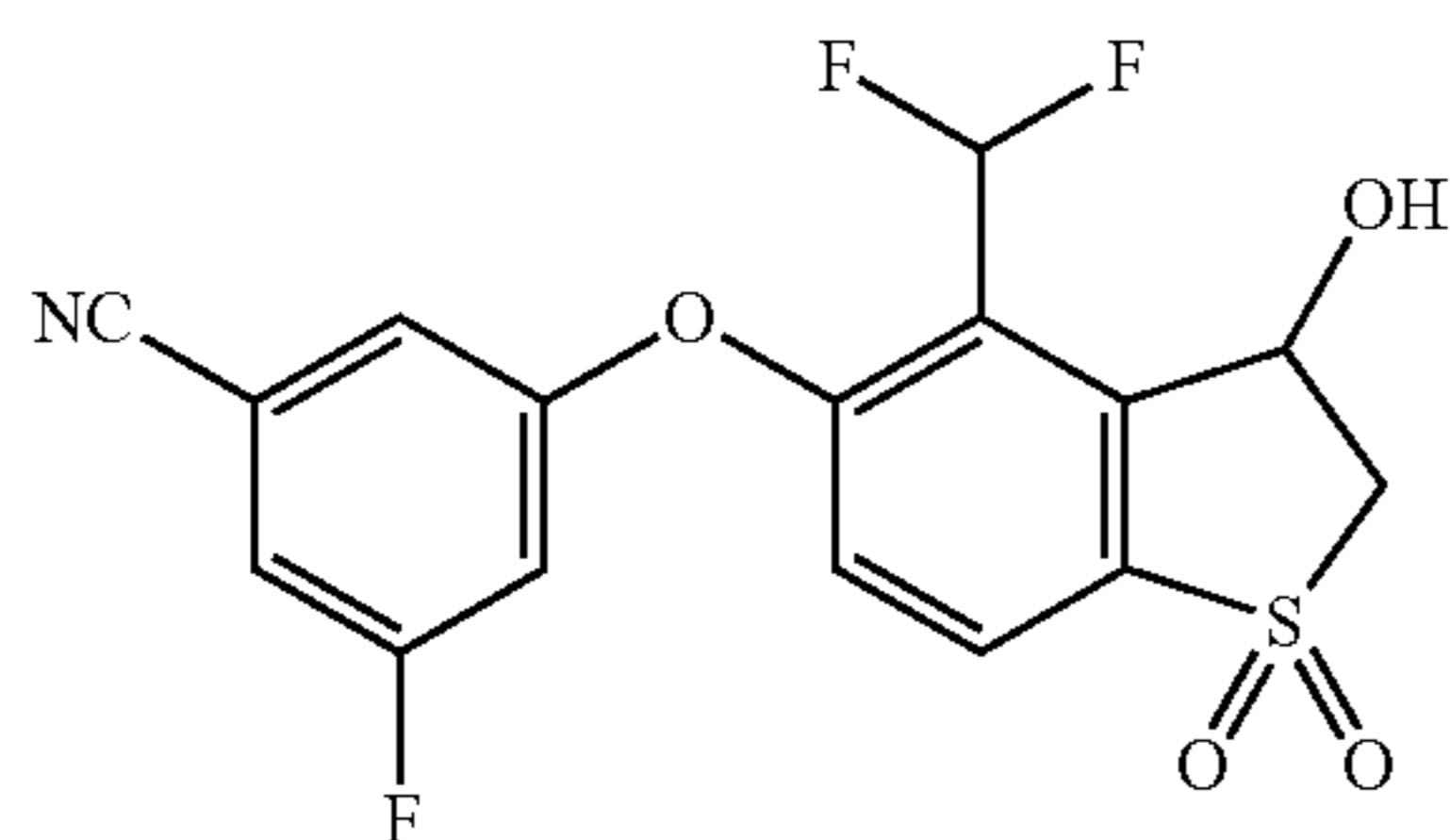
3-((4-(Difluoromethyl)-3-hydroxy-1,1-dioxido-2,3-dihydrobenzo[b]thiophen-5-yl)oxy)-5-fluorobenzonitrile (Compound 28)
