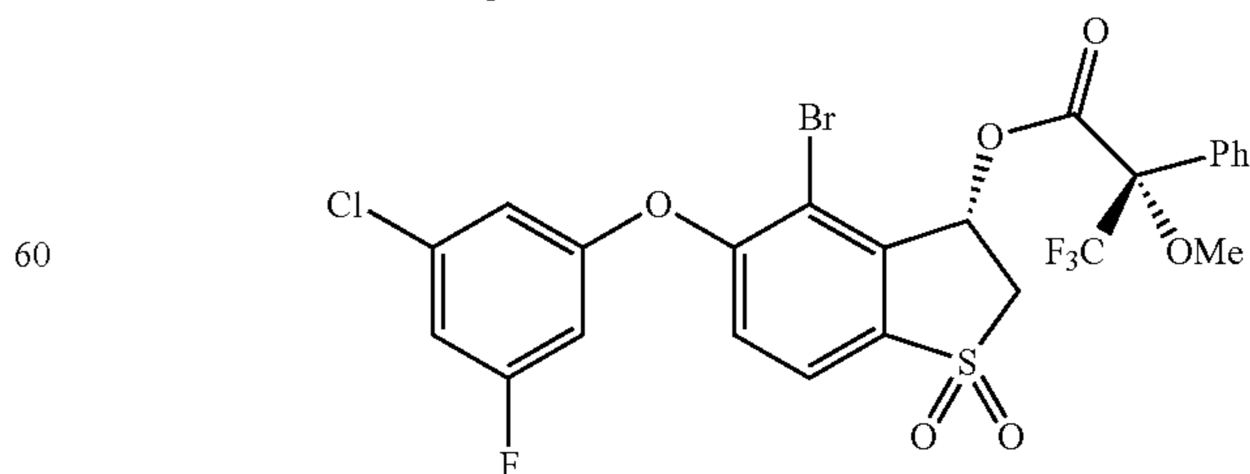
Compound 119B
