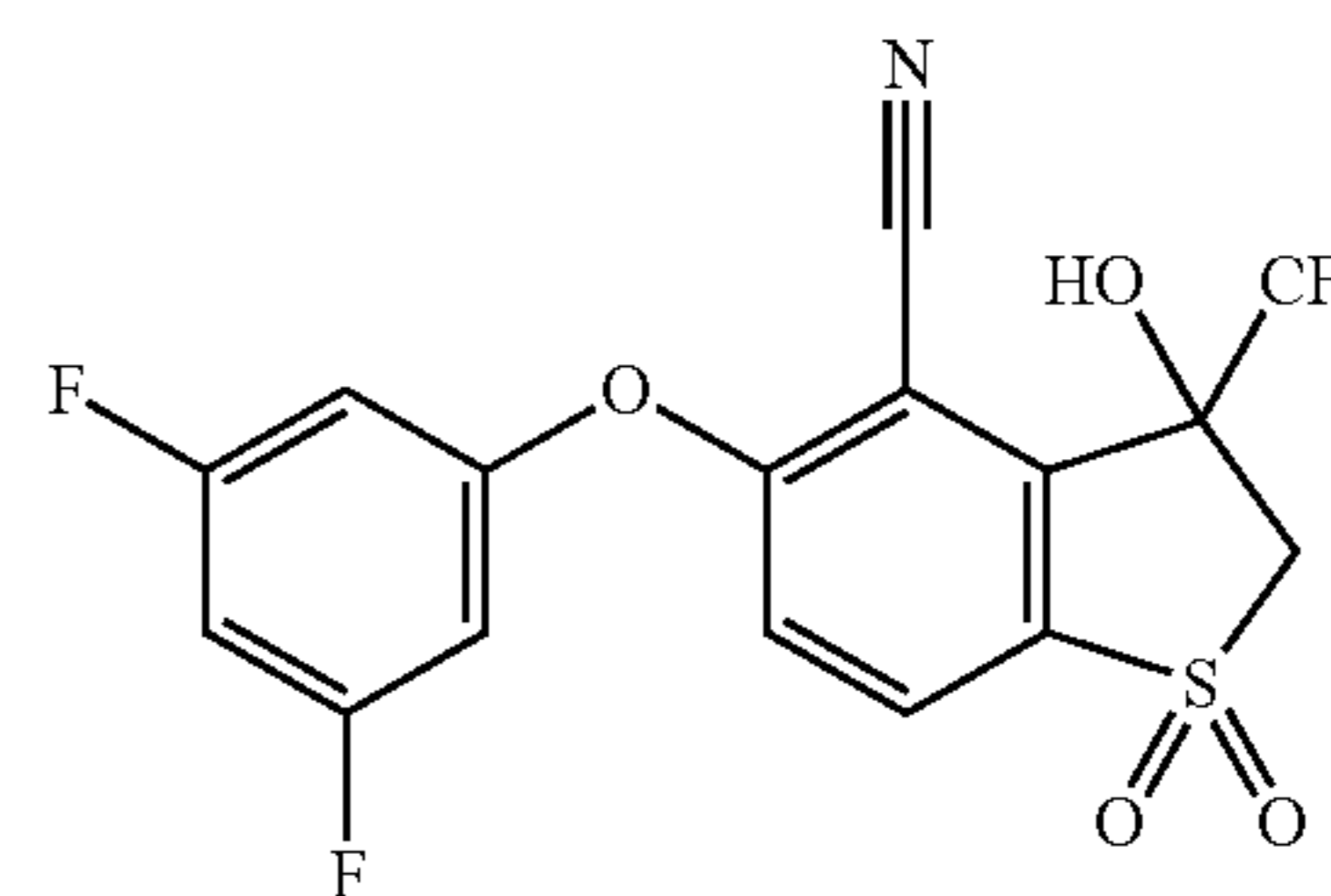
5-(3,5-Difluorophenoxy)-3-hydroxy-3-(trifluoromethyl)-2,3-dihydrobenzo[b]thiophene-4-carbonitrile 1,1-dioxide (Compound 102)
