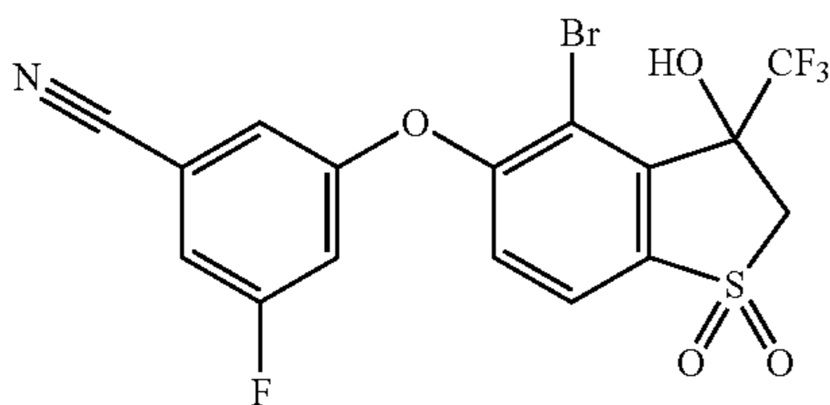
3-((4-Bromo-3-hydroxy-1,1-dioxido-3-(trifluoromethyl)-2,3-dihydrobenzo[b]thiophen-5-yl)oxy)-5-fluorobenzonitrile (Compound 103)
