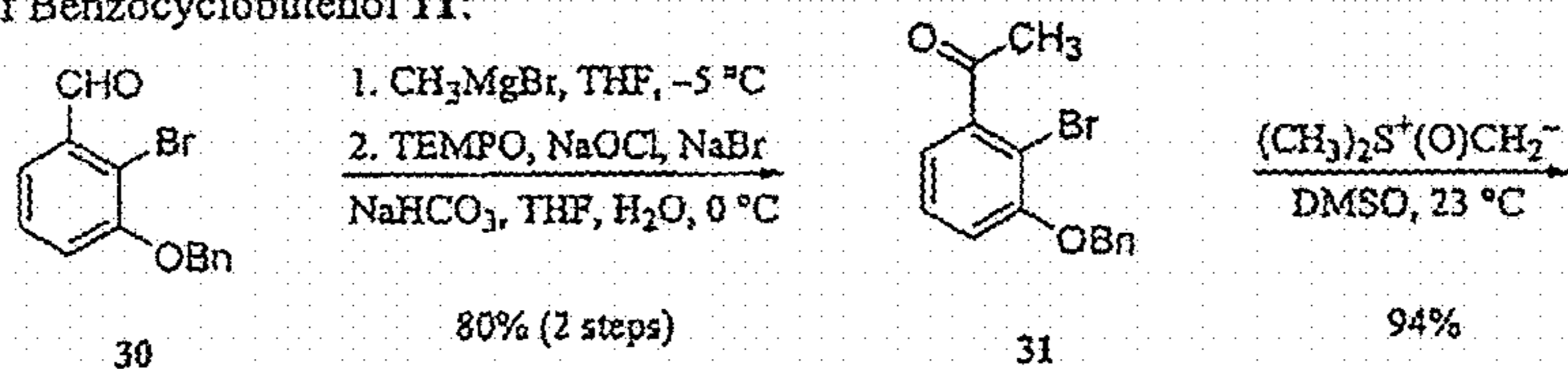
Figure 5 Synthesis of Benzocyclobutenol 11:
