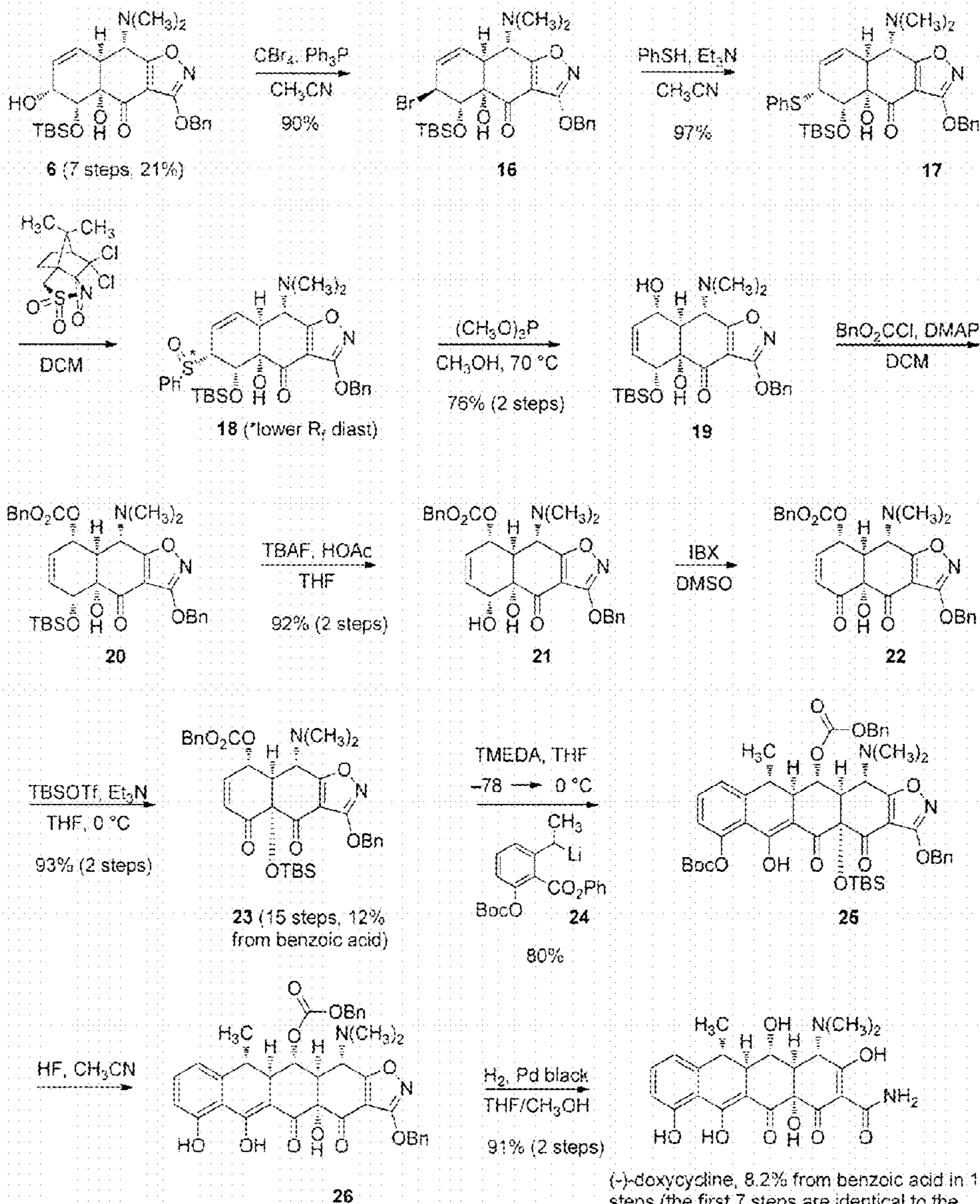
Figure 3 Total Synthesis of Doxycycline
