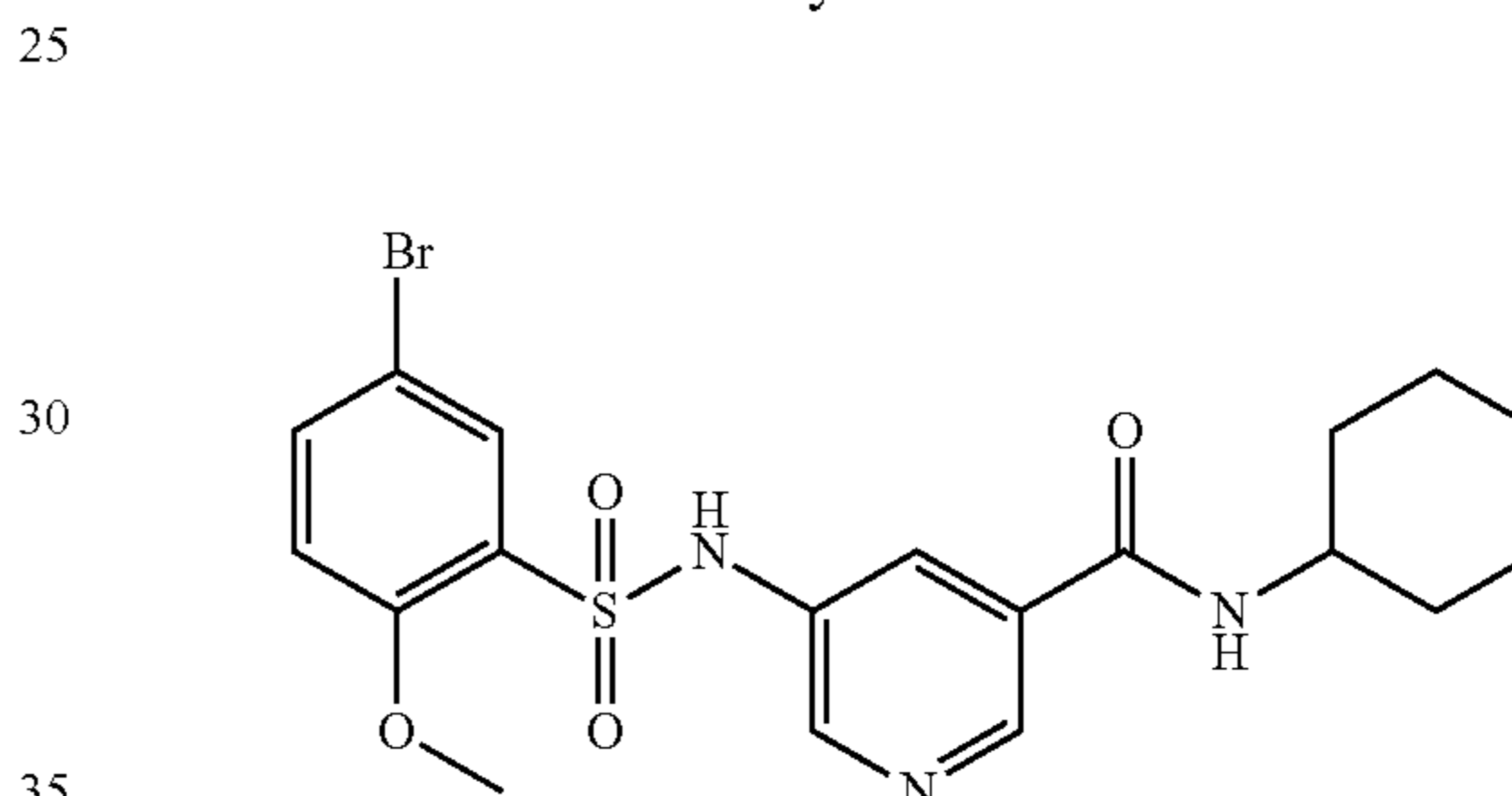
5-(5-Bromo-2-methoxyphenylsulfonamido)-N-cy- clohexylnicotinamide
