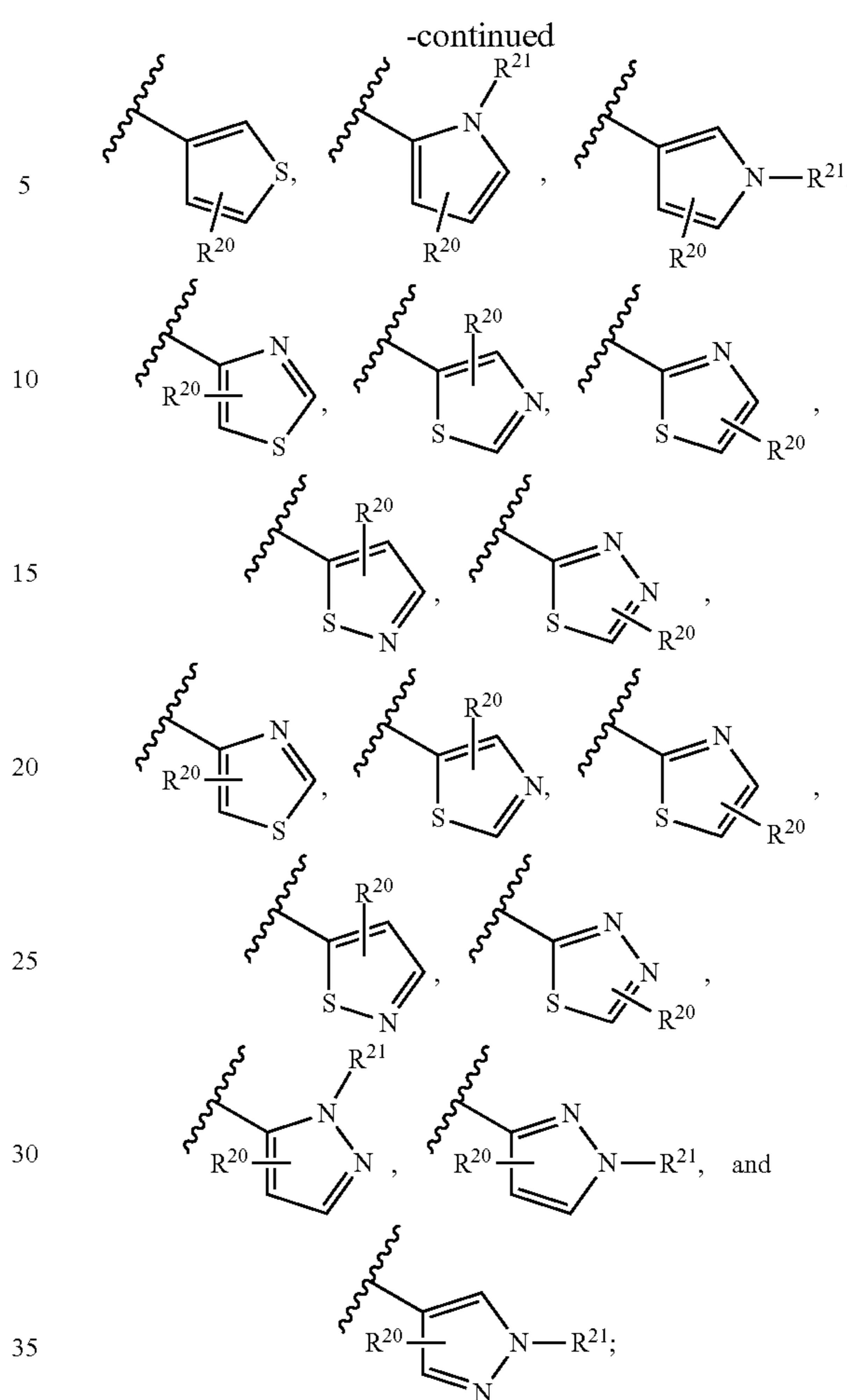
(Formula IVe)
