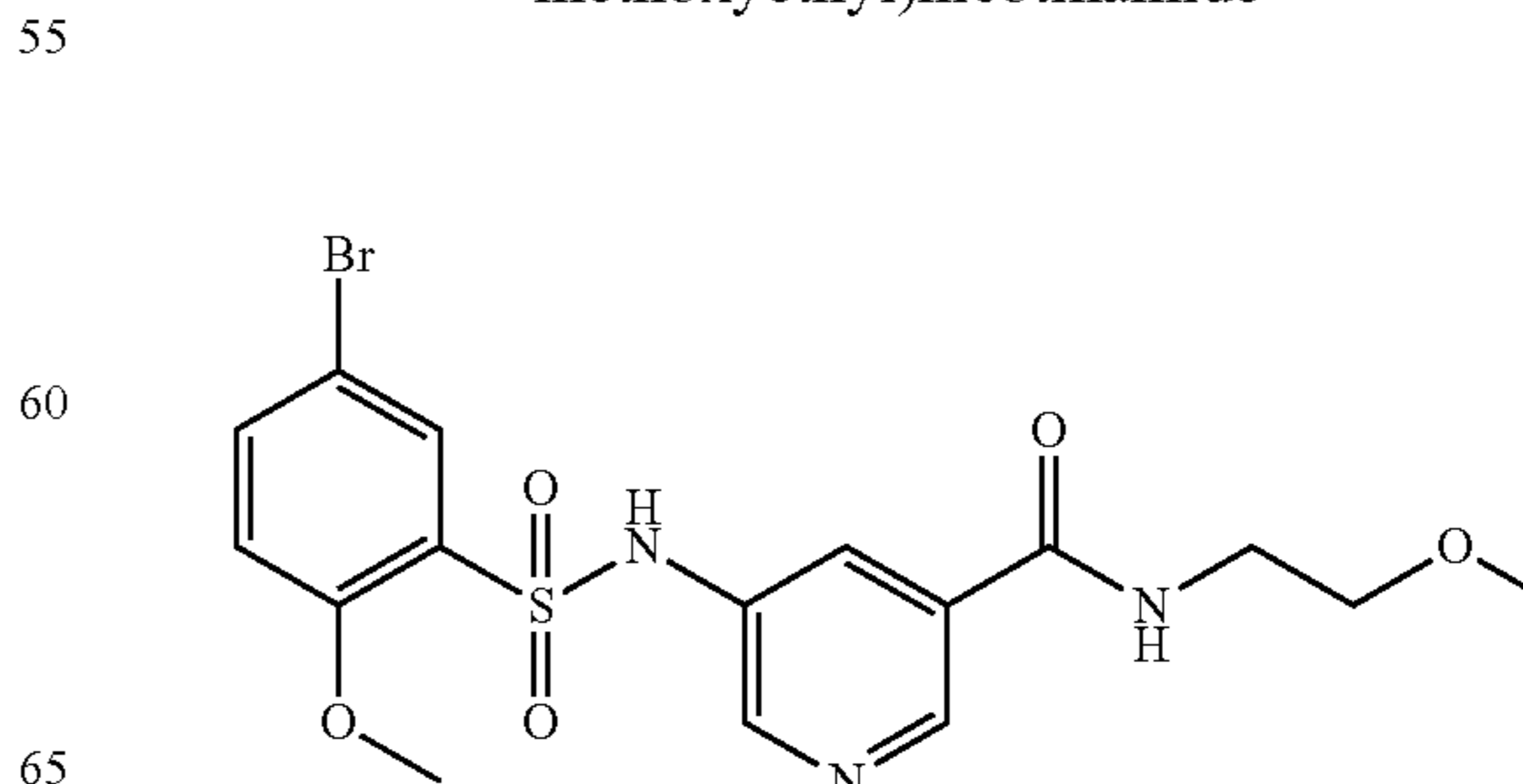
5-(5-Bromo-2-methoxyphenylsulfonamido)-N-(2- methoxyethyl)nicotinamide
