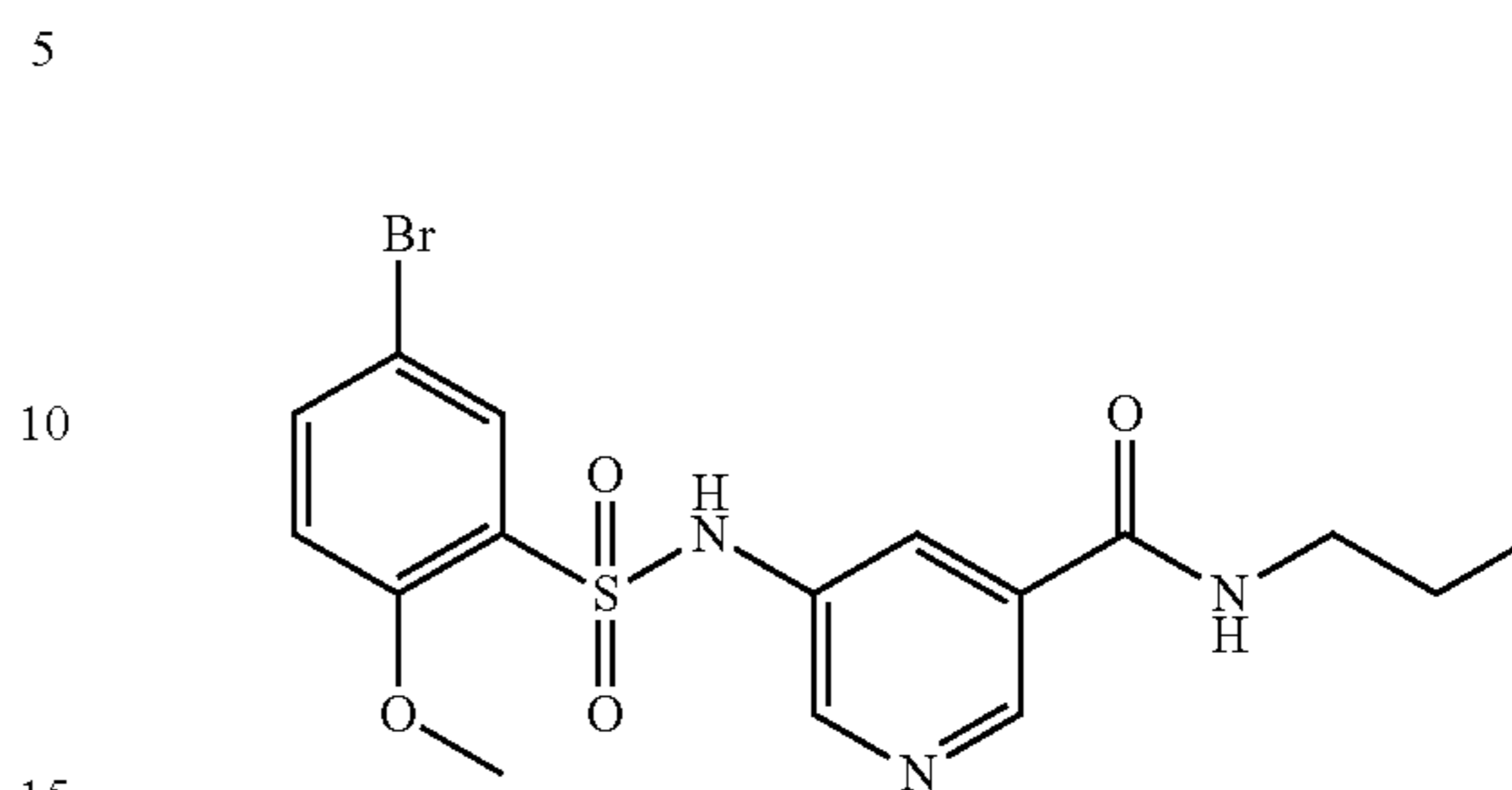
5-(5-Bromo-2-methoxyphenylsulfonamido)-N-pro- pylnicotinamide
