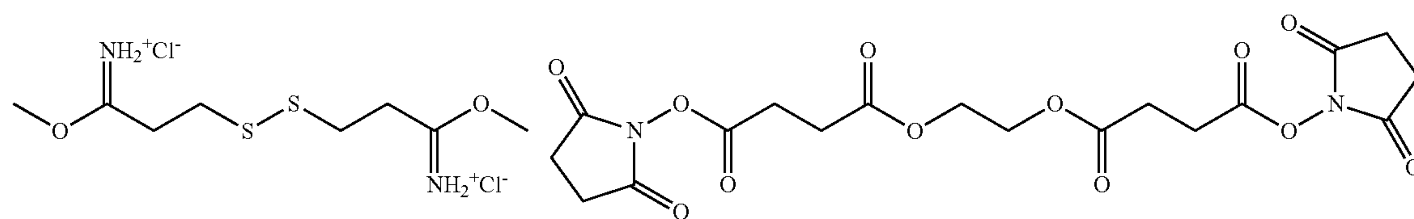
dimethyl-3,3'-dithiobispropionimidate
