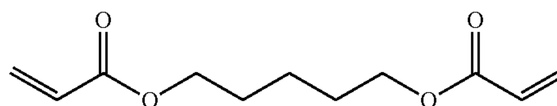
1,5-pentanediol diacrylate
