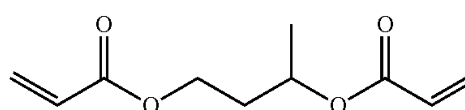
1,3-butanediol diacrylate
