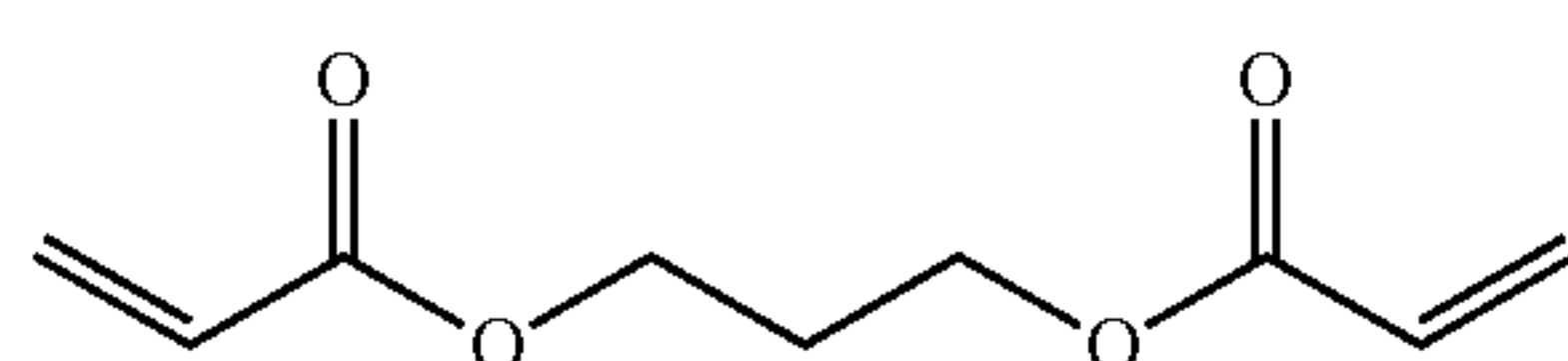
1,3-propanediol diacrylate
