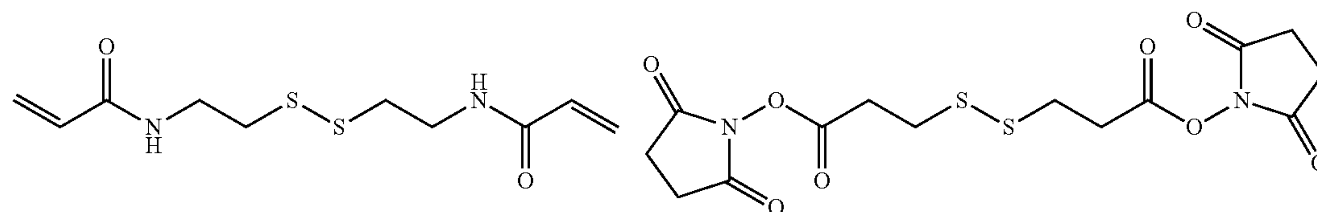
N,N'-bis(acrylyl)cystamine
