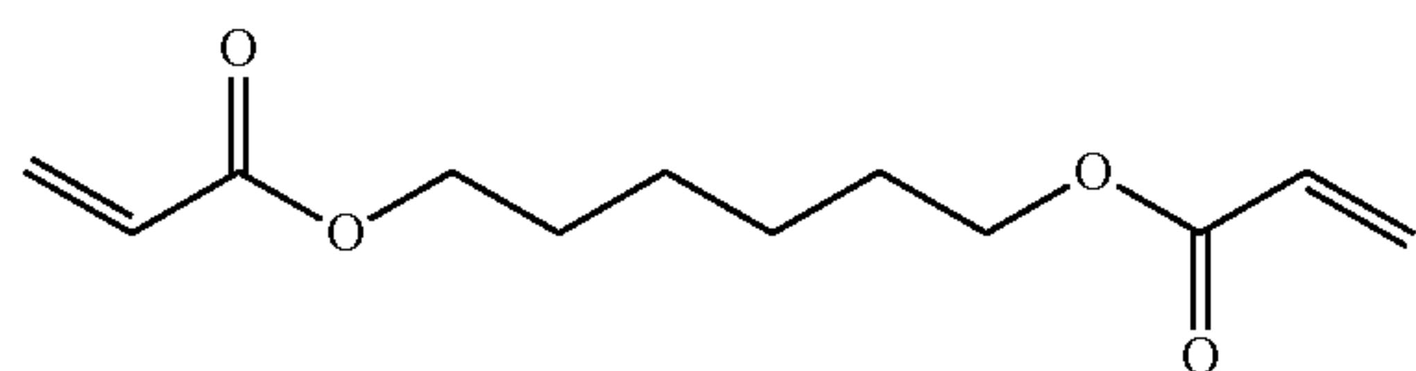
1,6-hexanediol diacrylate
