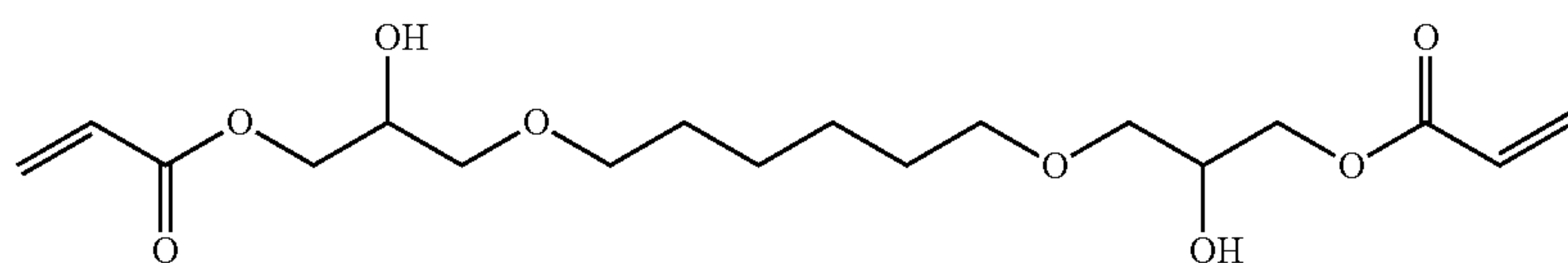
1,6-(hexanediylbis[oxy(2-hydroxy-3,1-propanediyl)] bisacrylate
