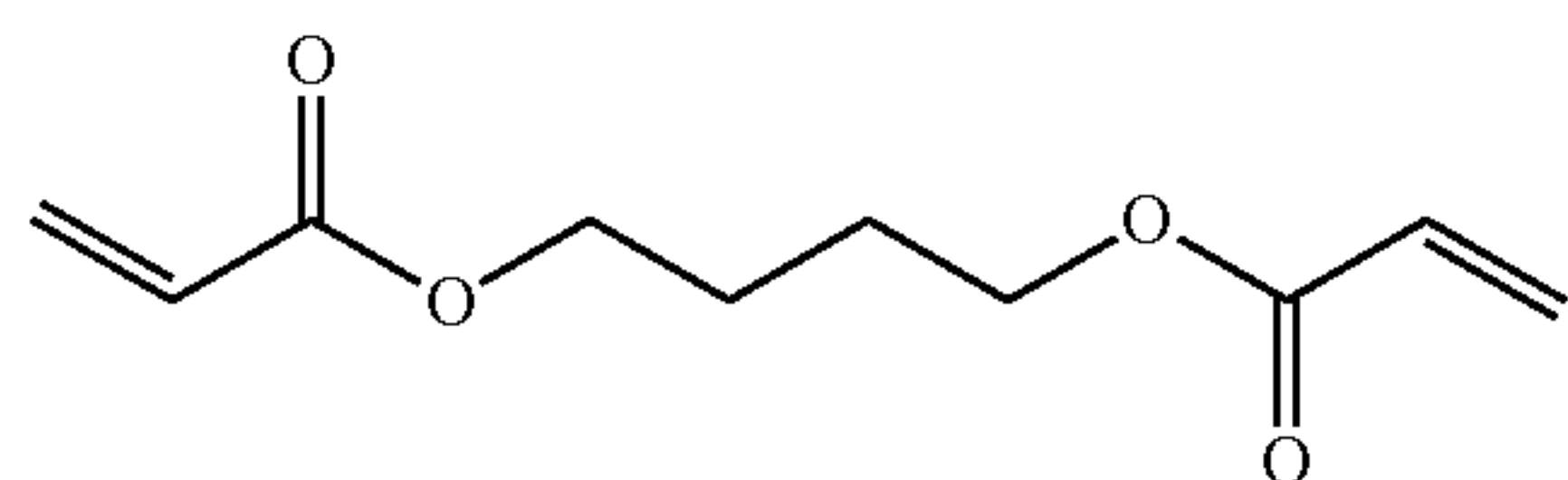
1,4-butanediol diacrylate
