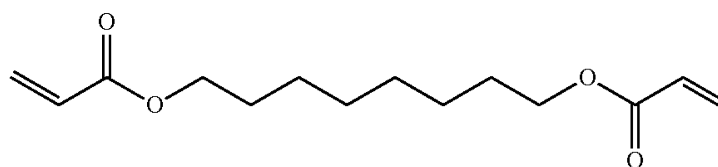
1,8-octanediol diacrylate
