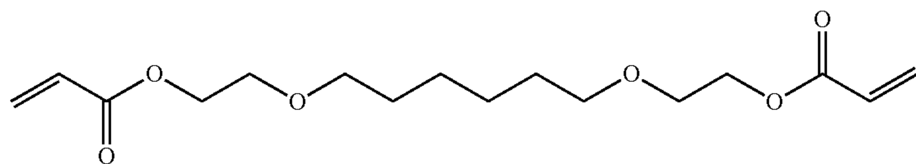
2,2'-(hexane-1,6-diylbis(oxy))bis(ethane-2,1-diyl) diacrylate
