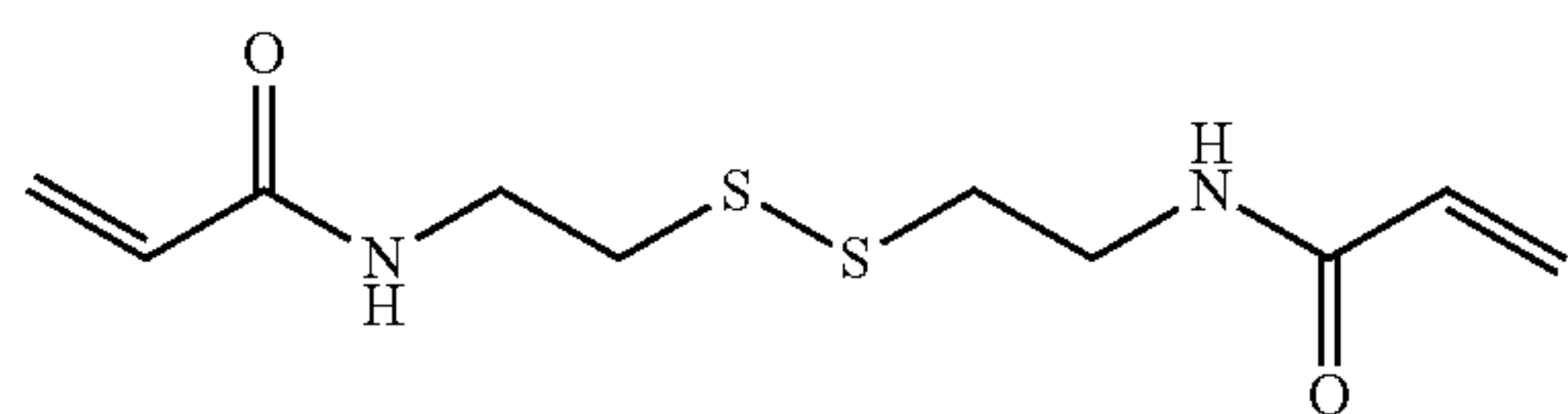
N,N'-bis(acrylyl)cystamine
