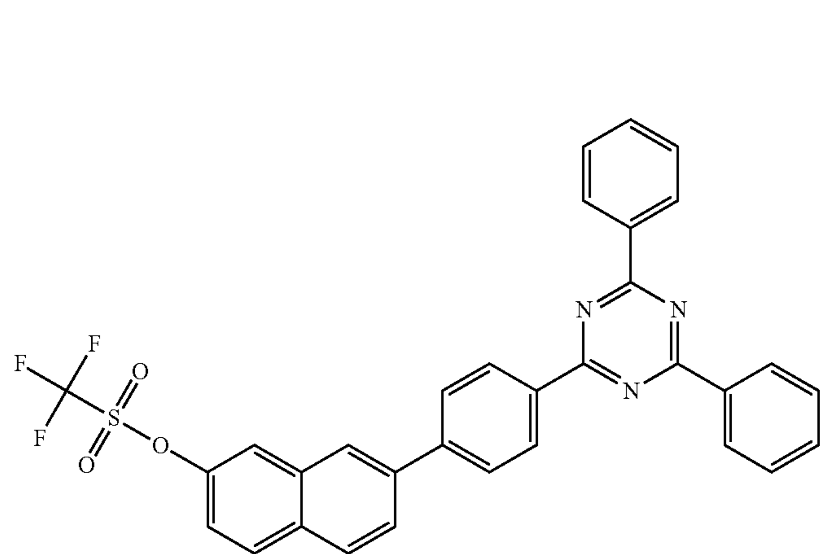
[Compound 1-D]
