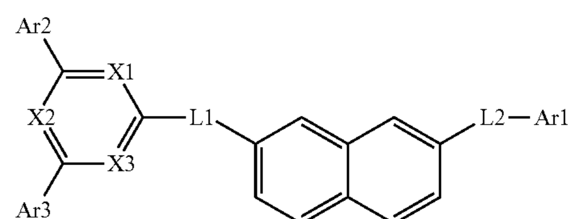
[Chemical Formula 1-2]
