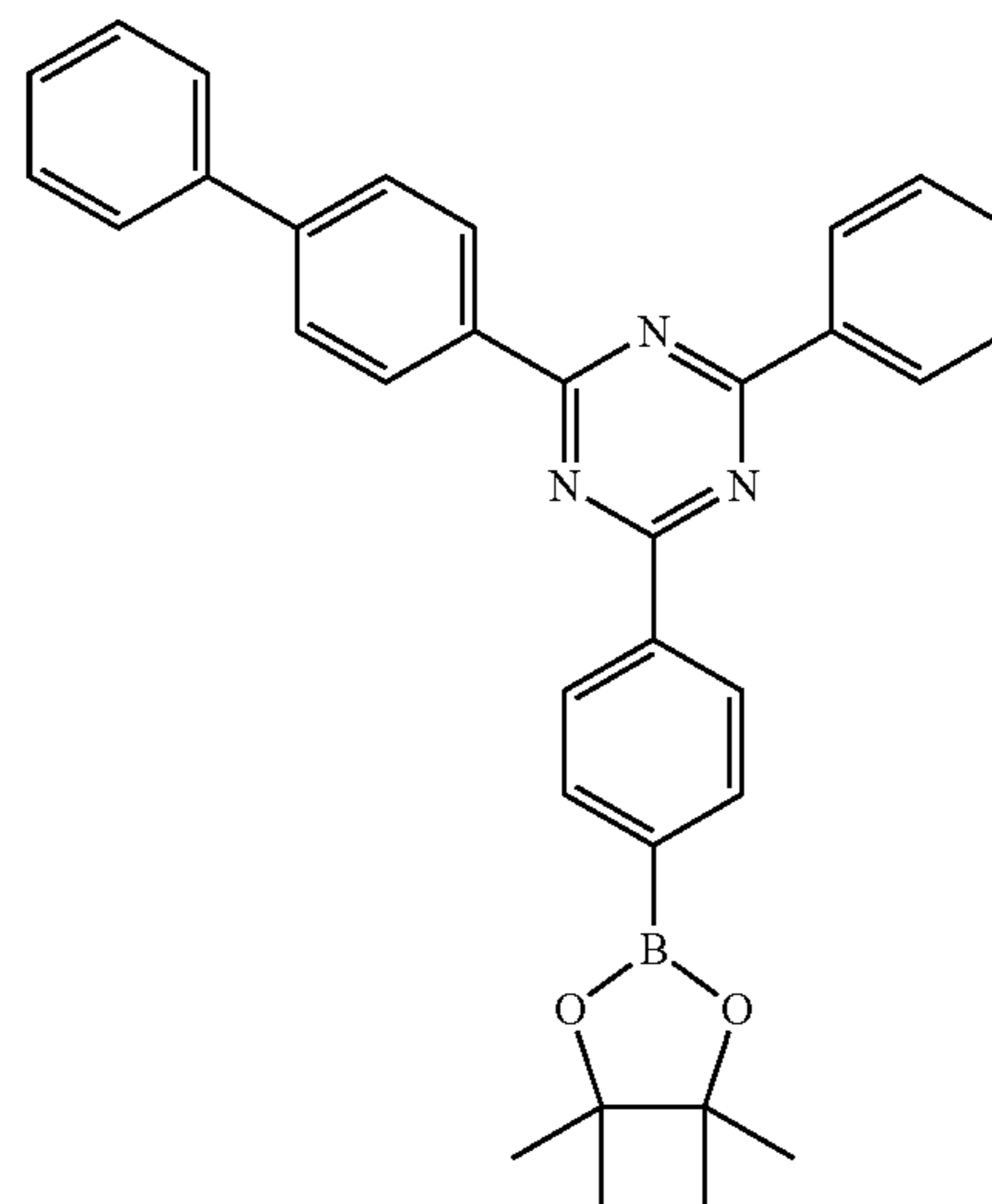
[Compound 4-B]
