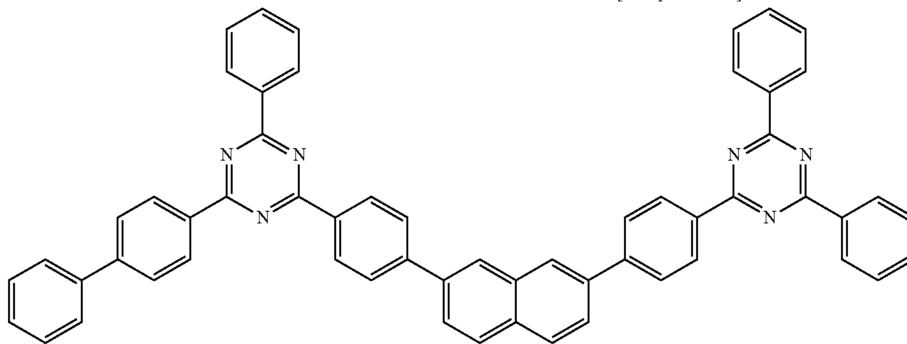
[Compound 4-B]
