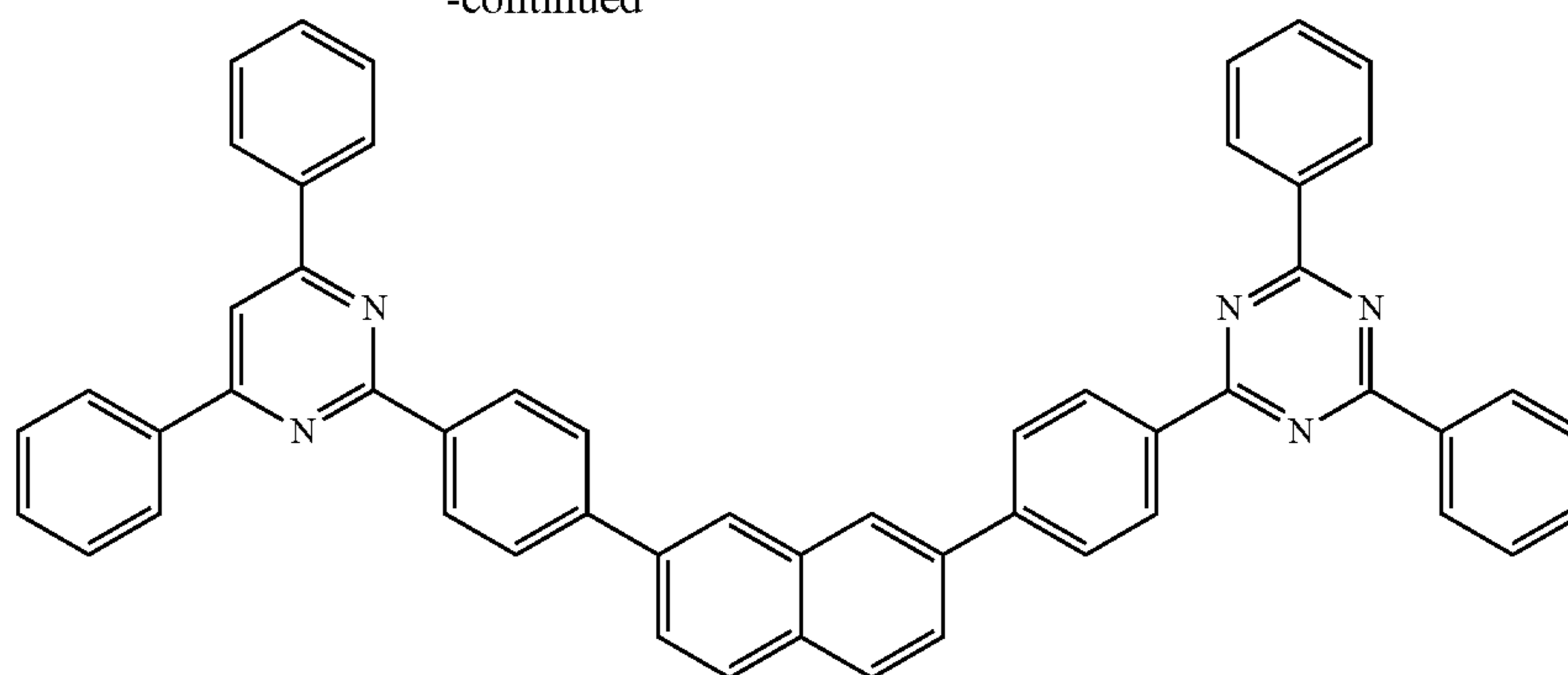
[Compound 1-a-2]
