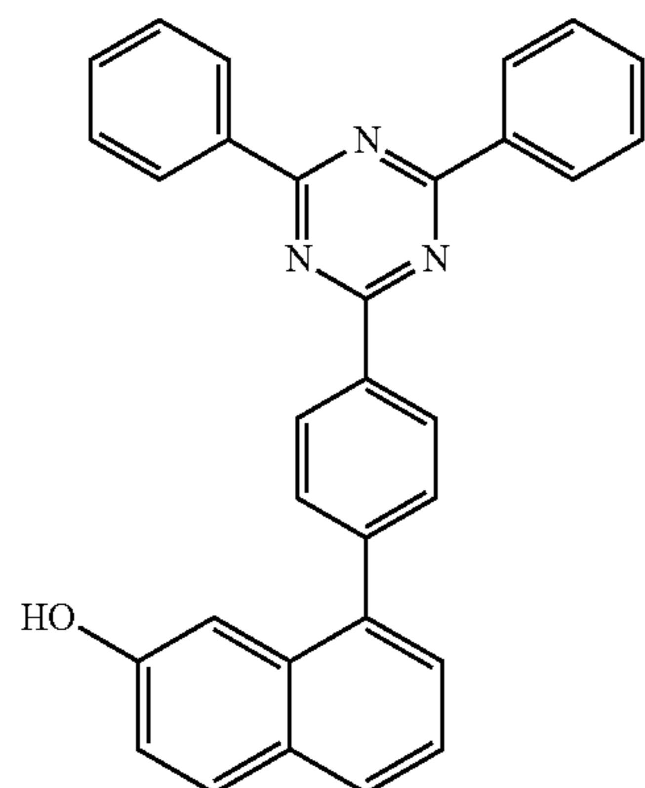
[Compound 5-A]
