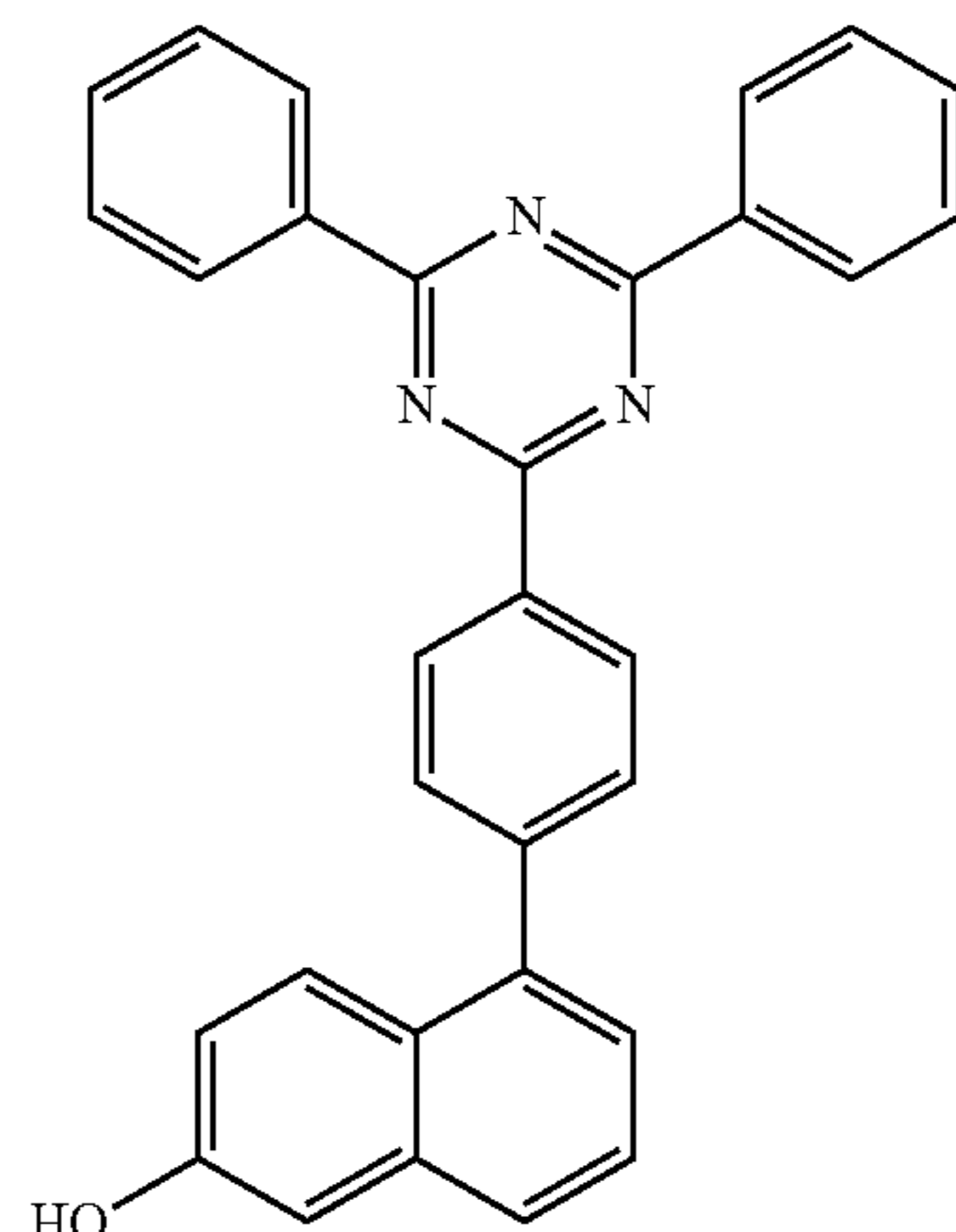
[Compound 6-A]
