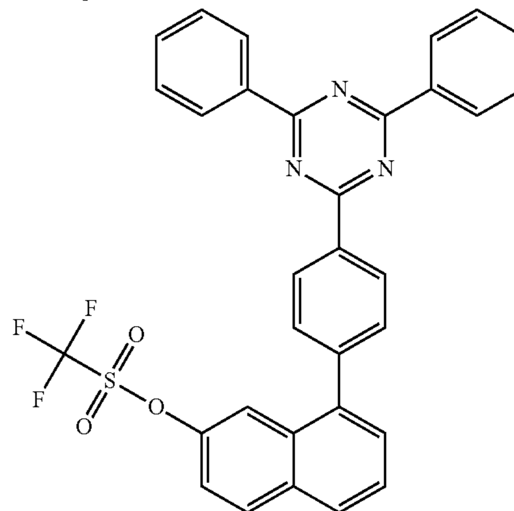
[Compound 5-B]
