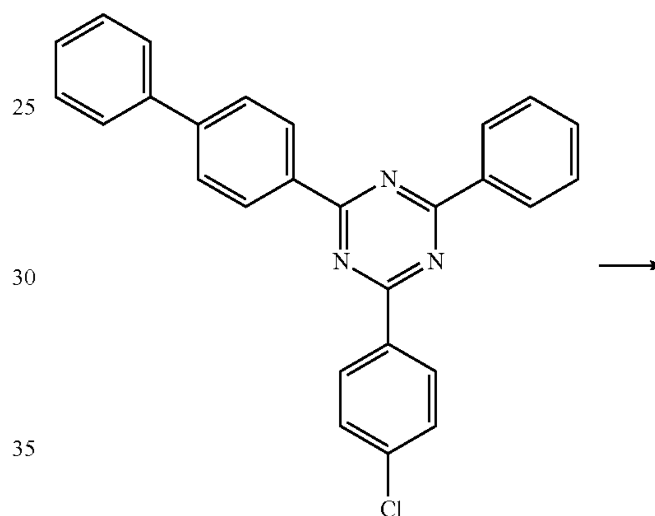
[Compound 4-A]
