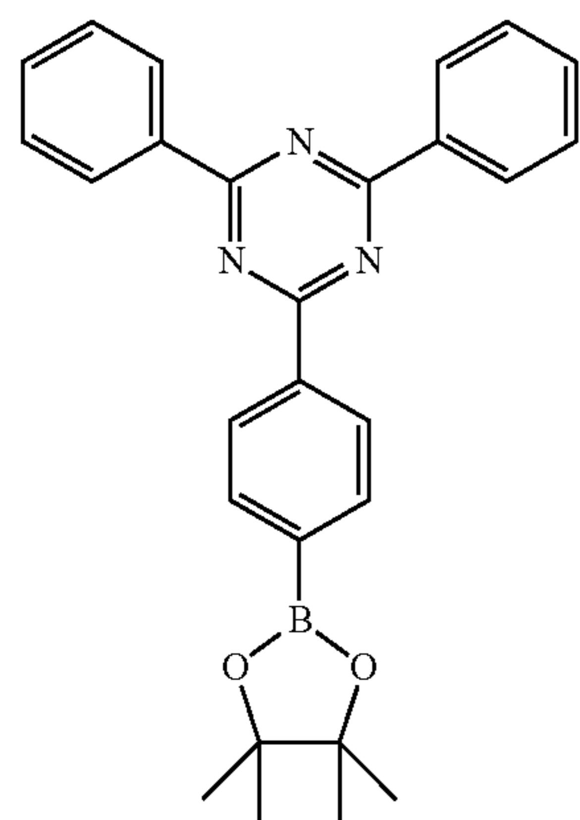
[Compound 1-B]
