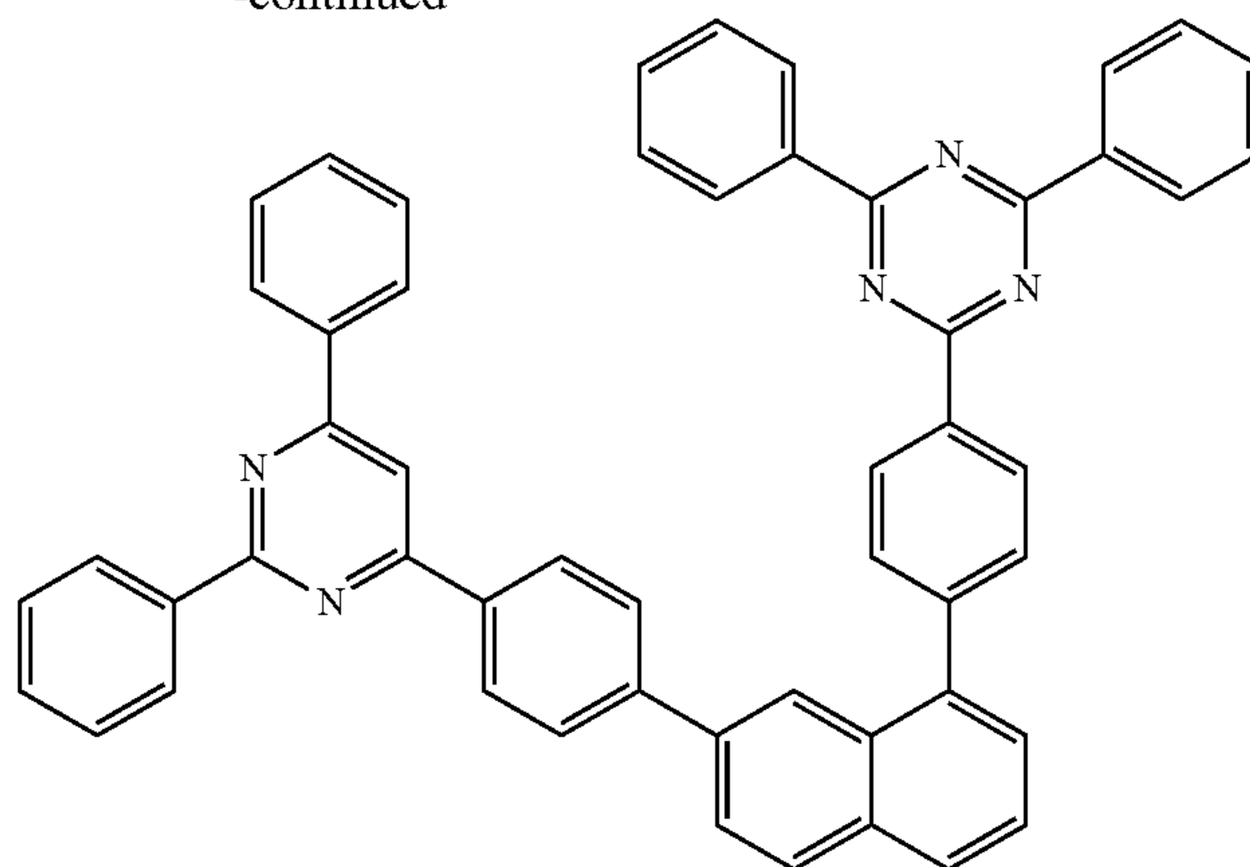
[Compound 2-a-1]
