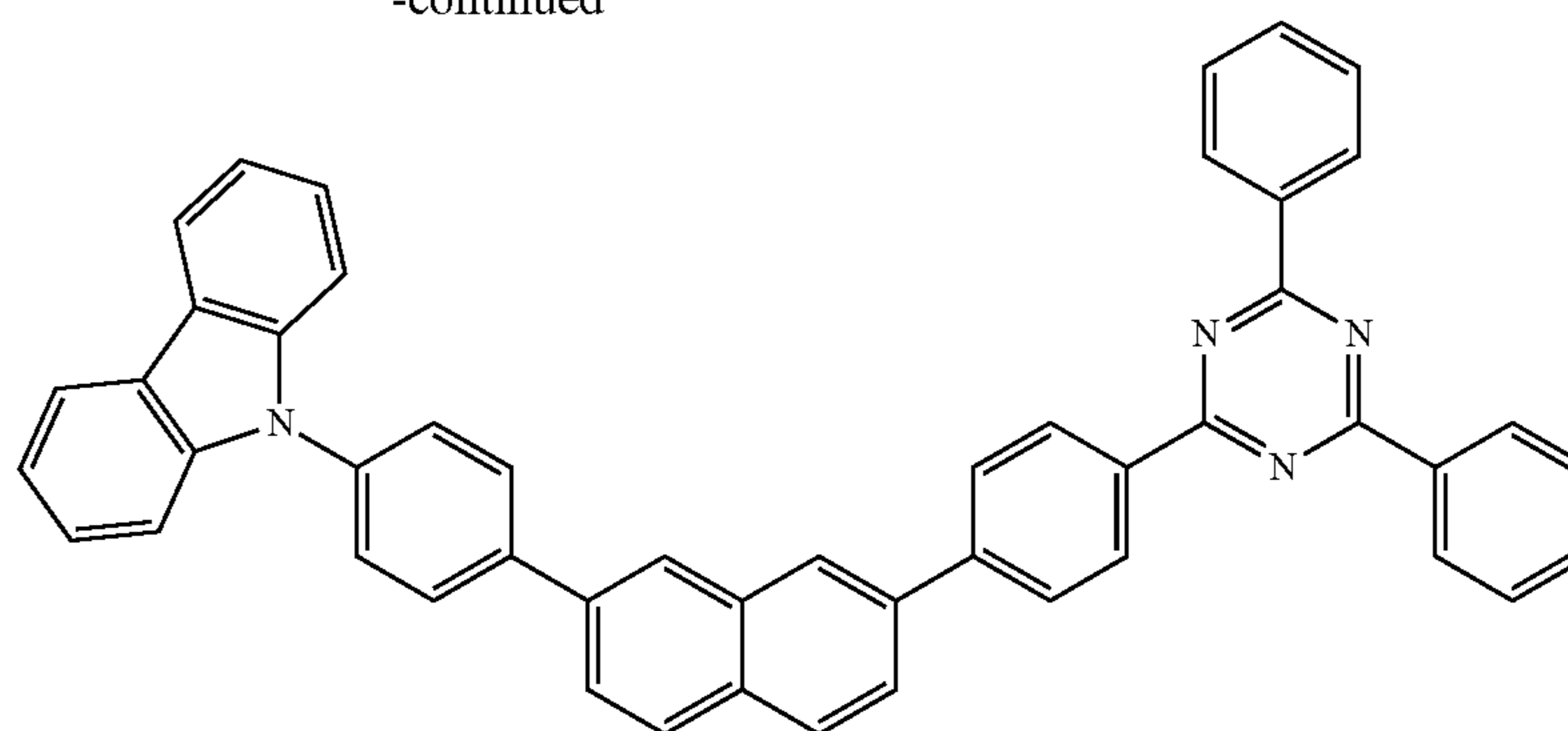
[Compound 1-b-1]
