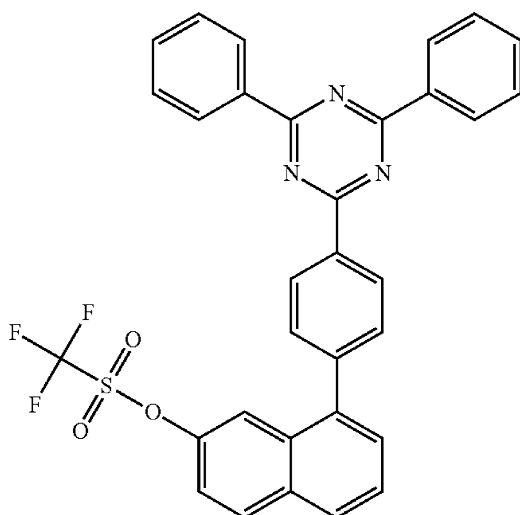
[Compound 5-B]
