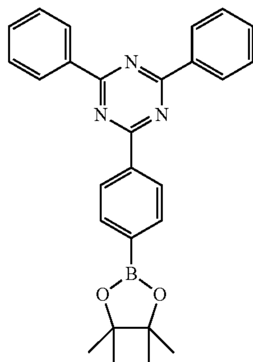
[Compound 1-B]
