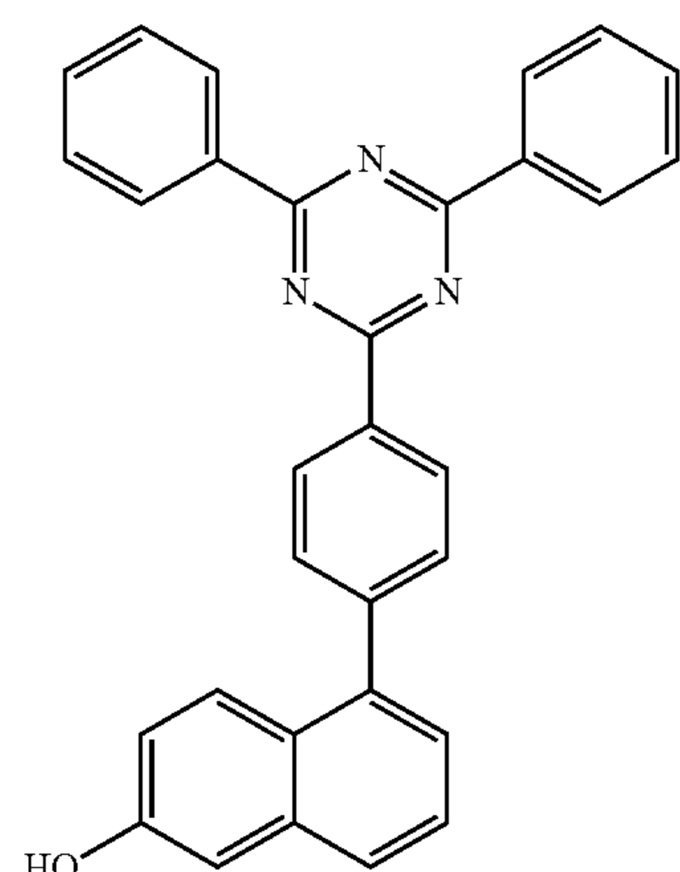
[Compound 6-A]
