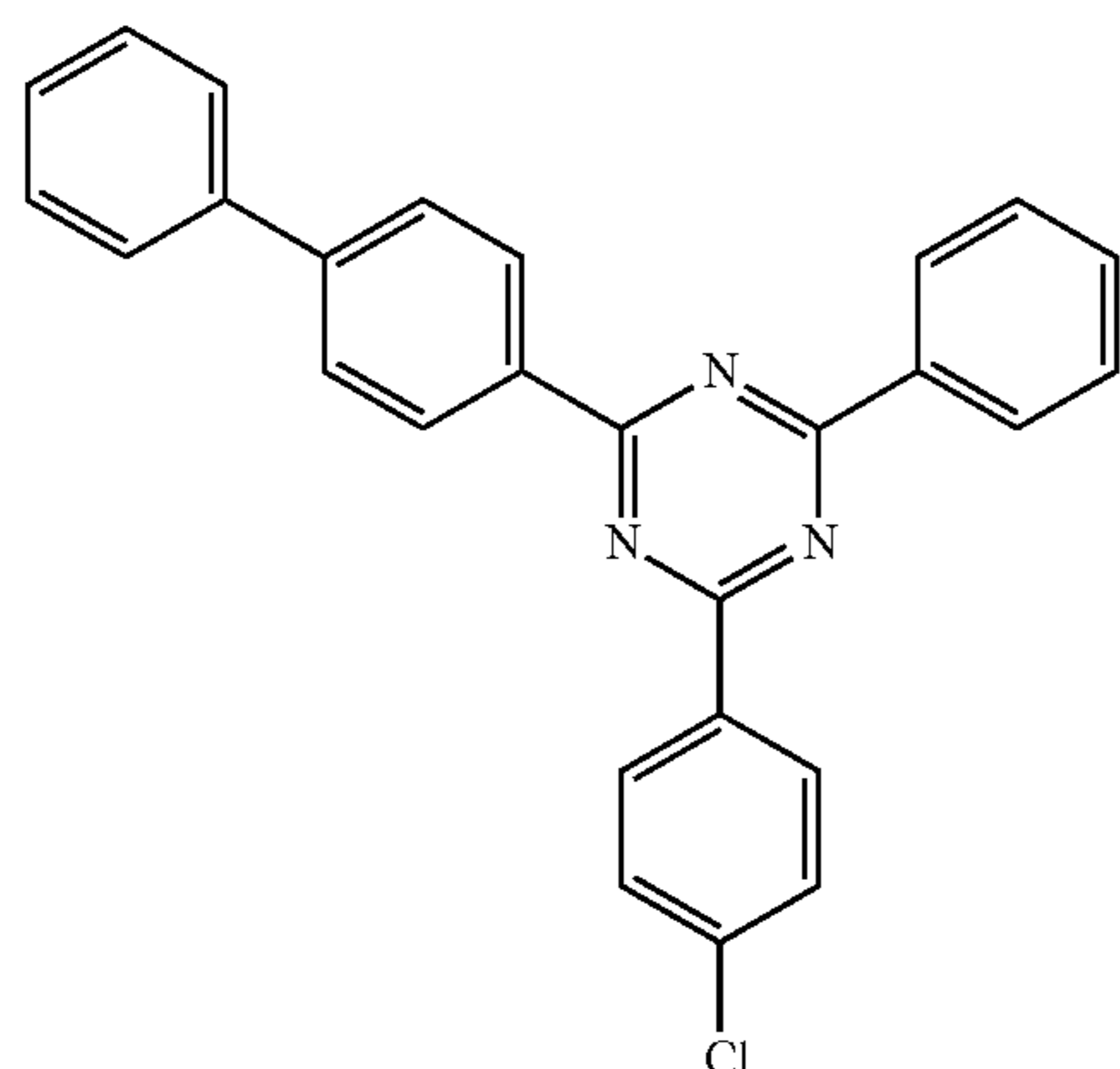
[Compound 4-A]
