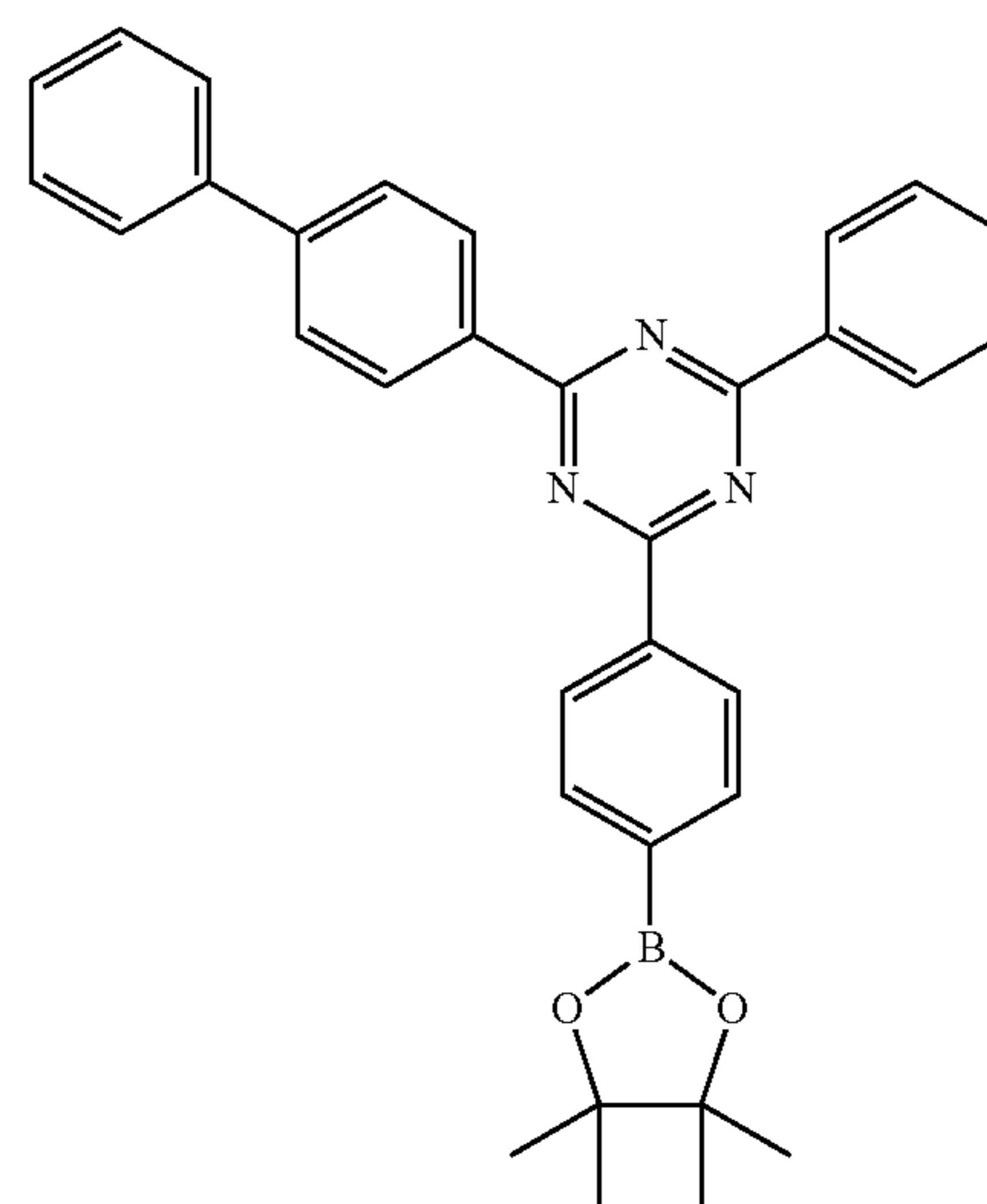
[Compound 4-B]
