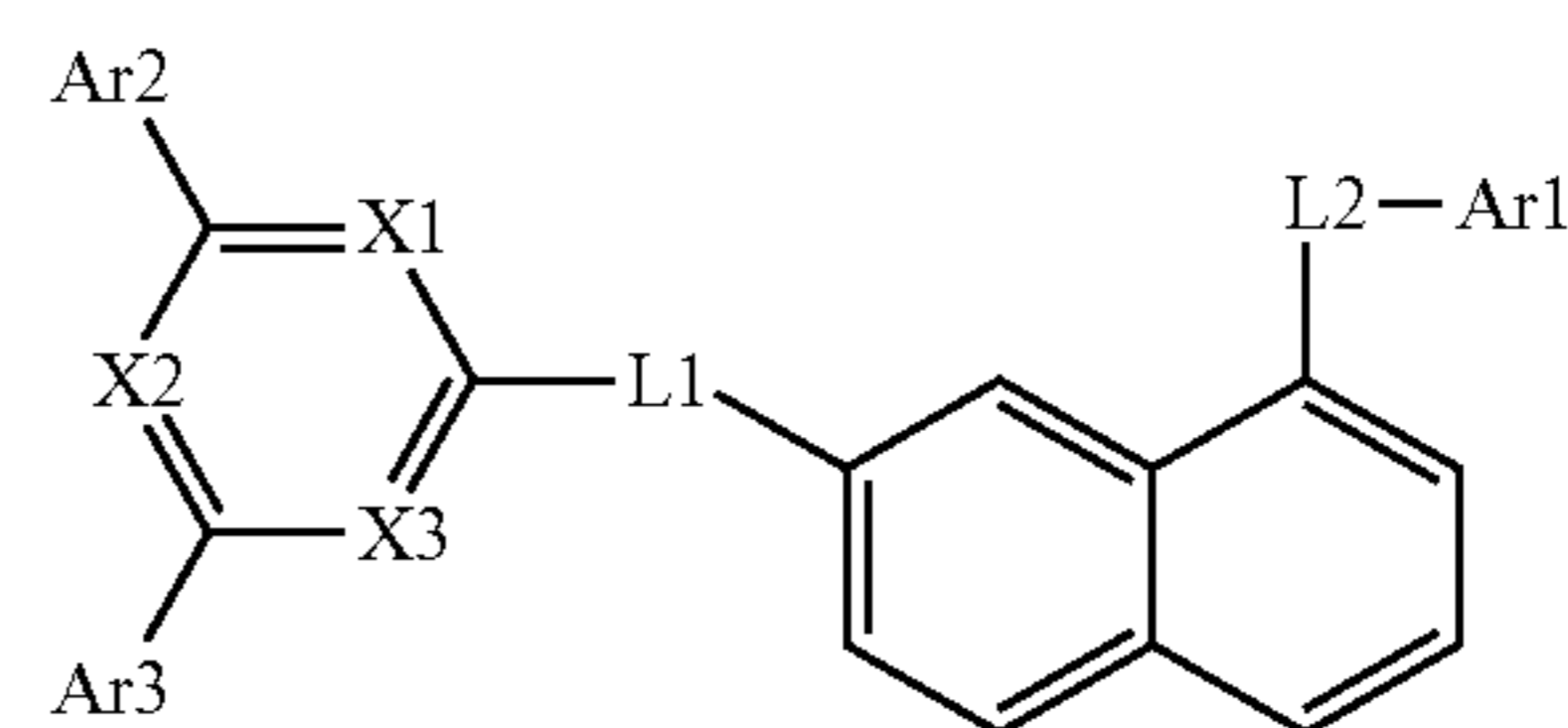
[Chemical Formula 1-3]
