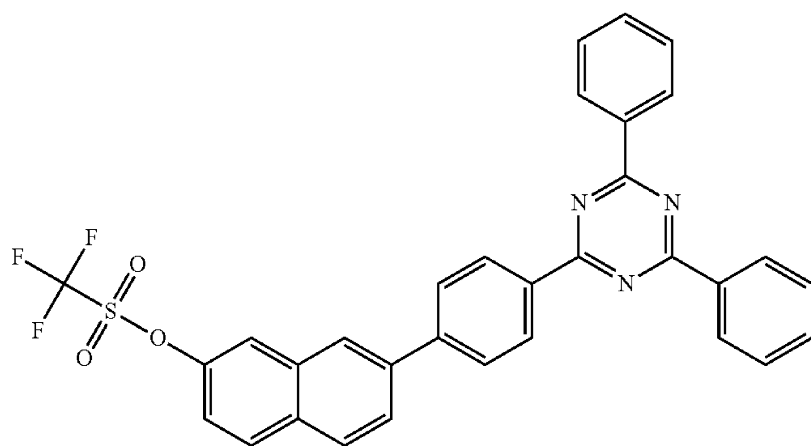
[Compound 1-D]
