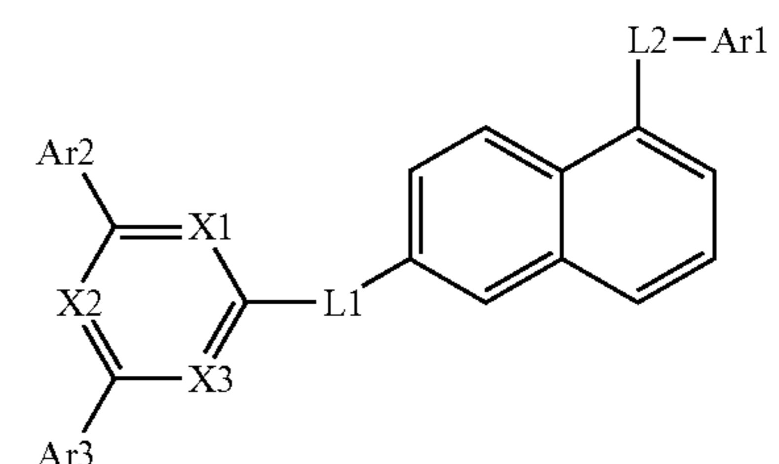
[Chemical Formula 1-3]
