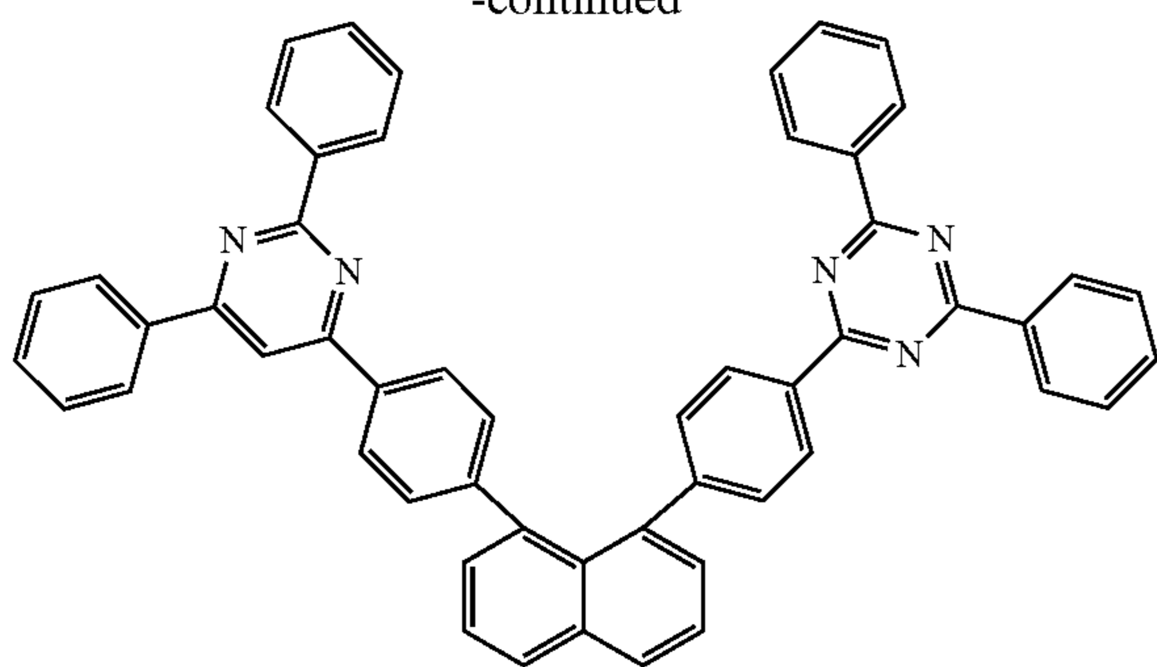
[Compound 4-a-1]
