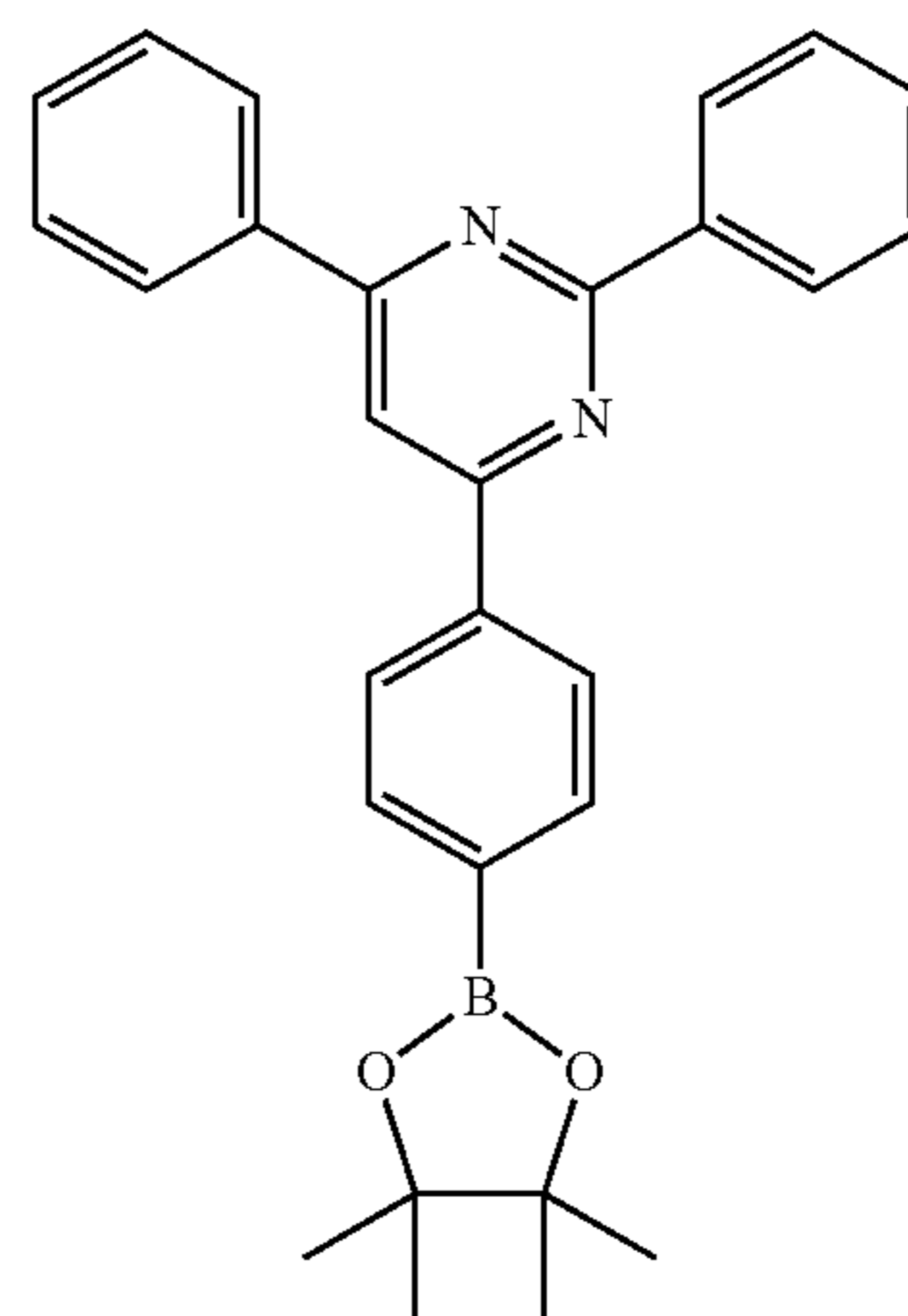
[Compound 2-B]
