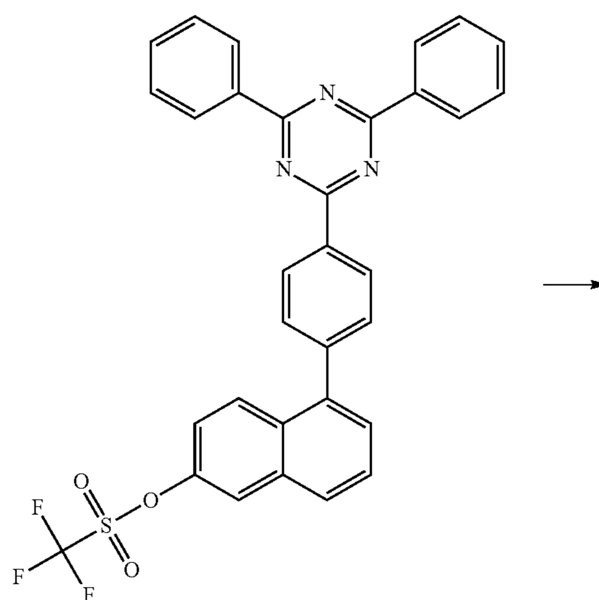
[Compound 6-B]
