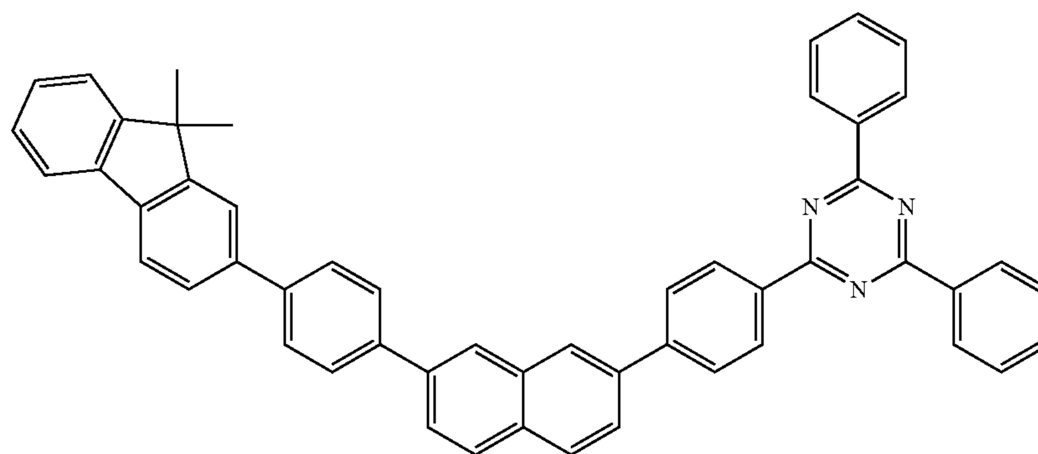
[Compound 1-b-2]
