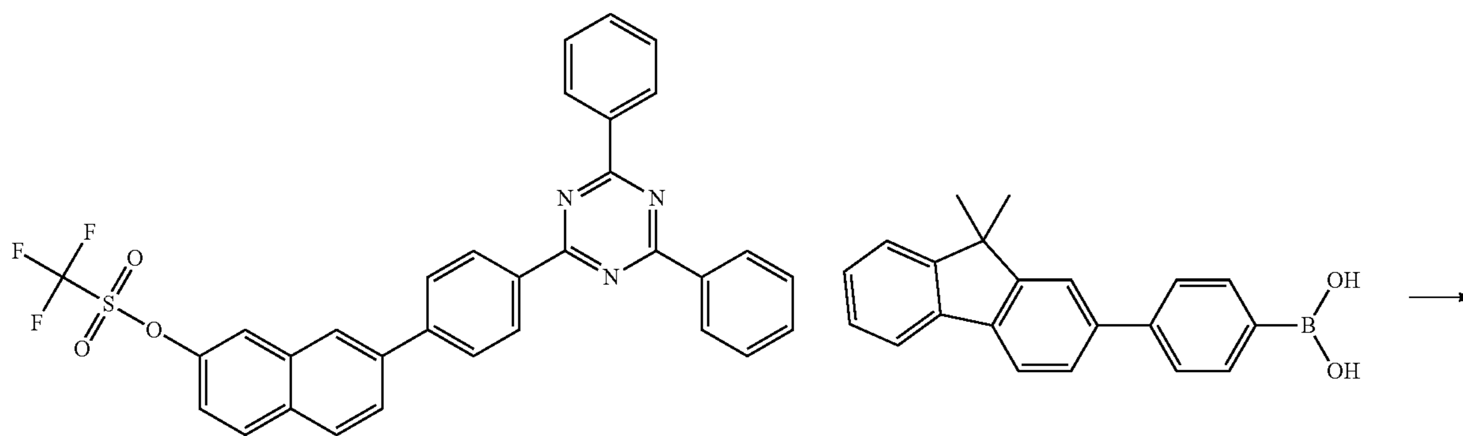
[Compound 1-D]
