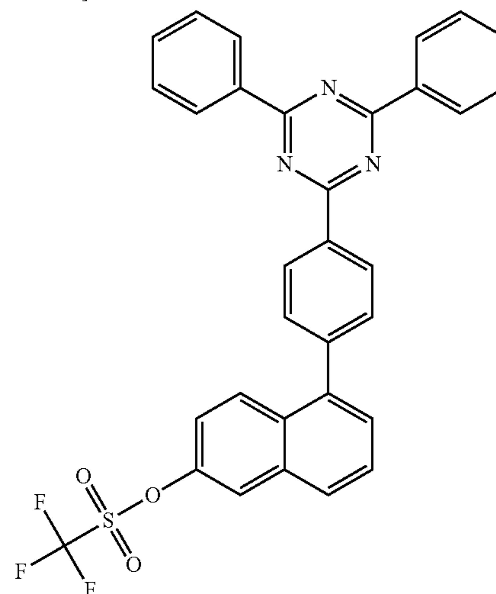
[Compound 6-A]
