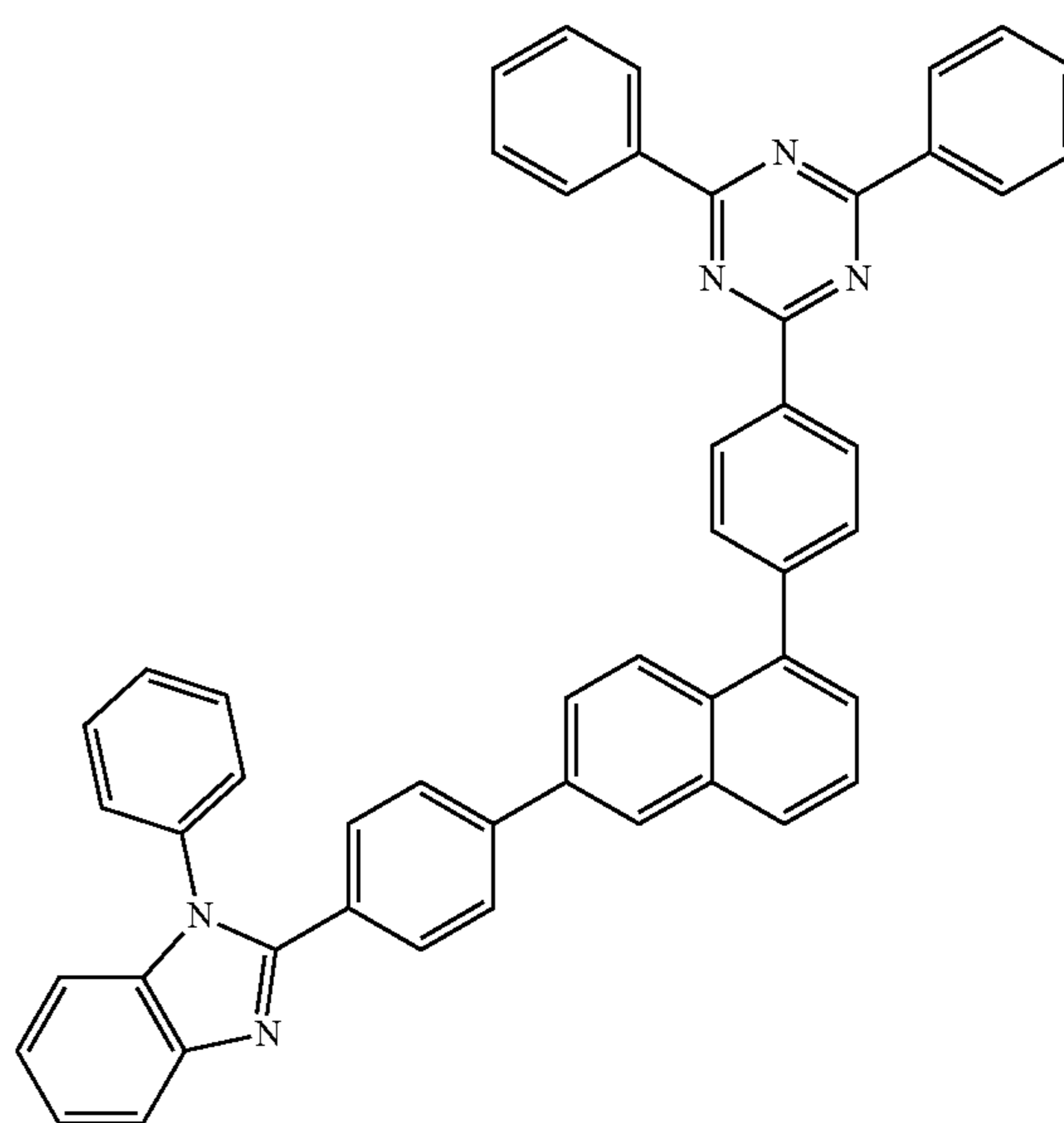
[Compound 6-B]
