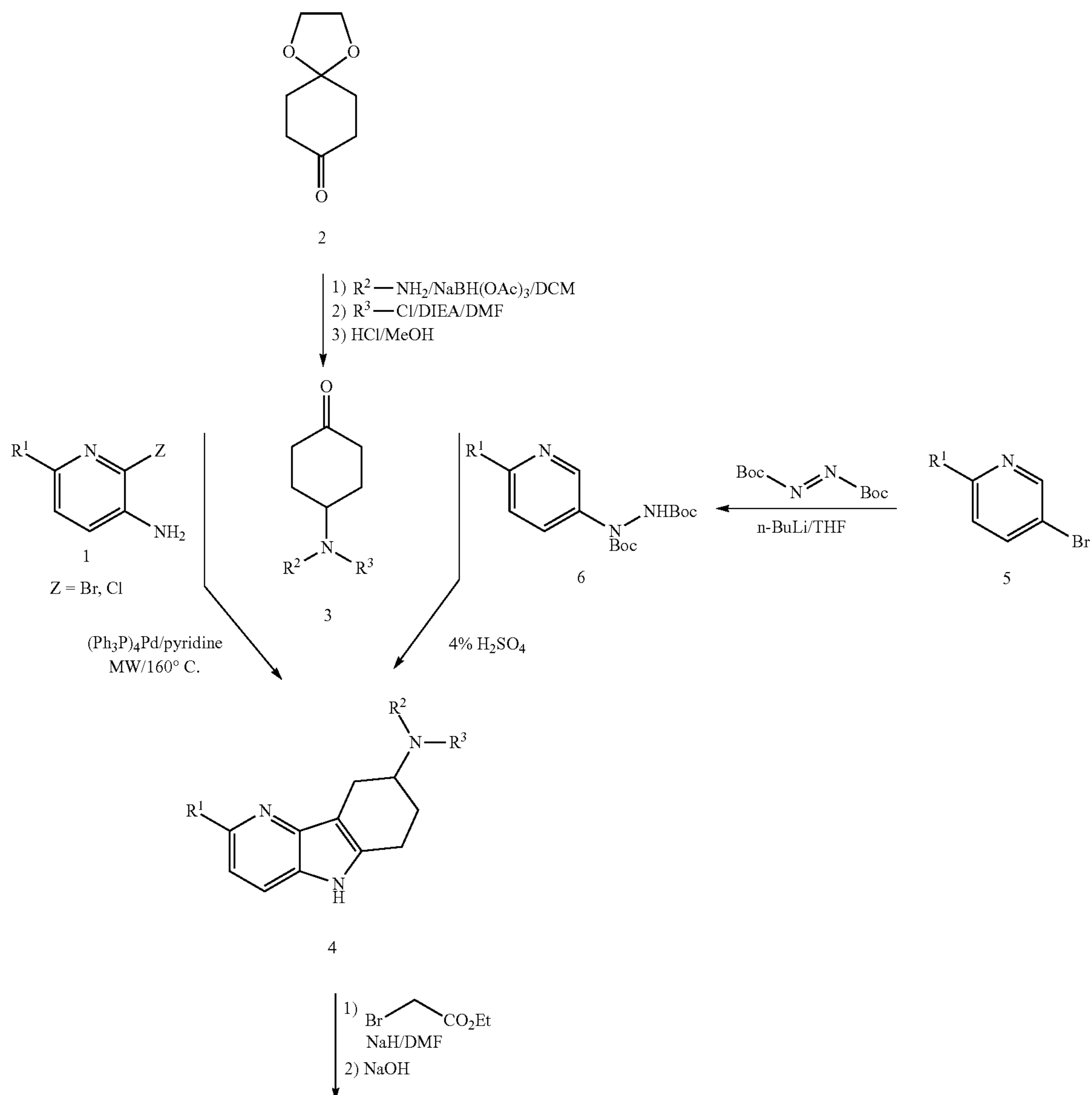
Scheme 1: General synthetic route for the preparation of compounds of formula (I) ( \text{R}^3 represents 5-chloro-pyrimidin-2-yl)
