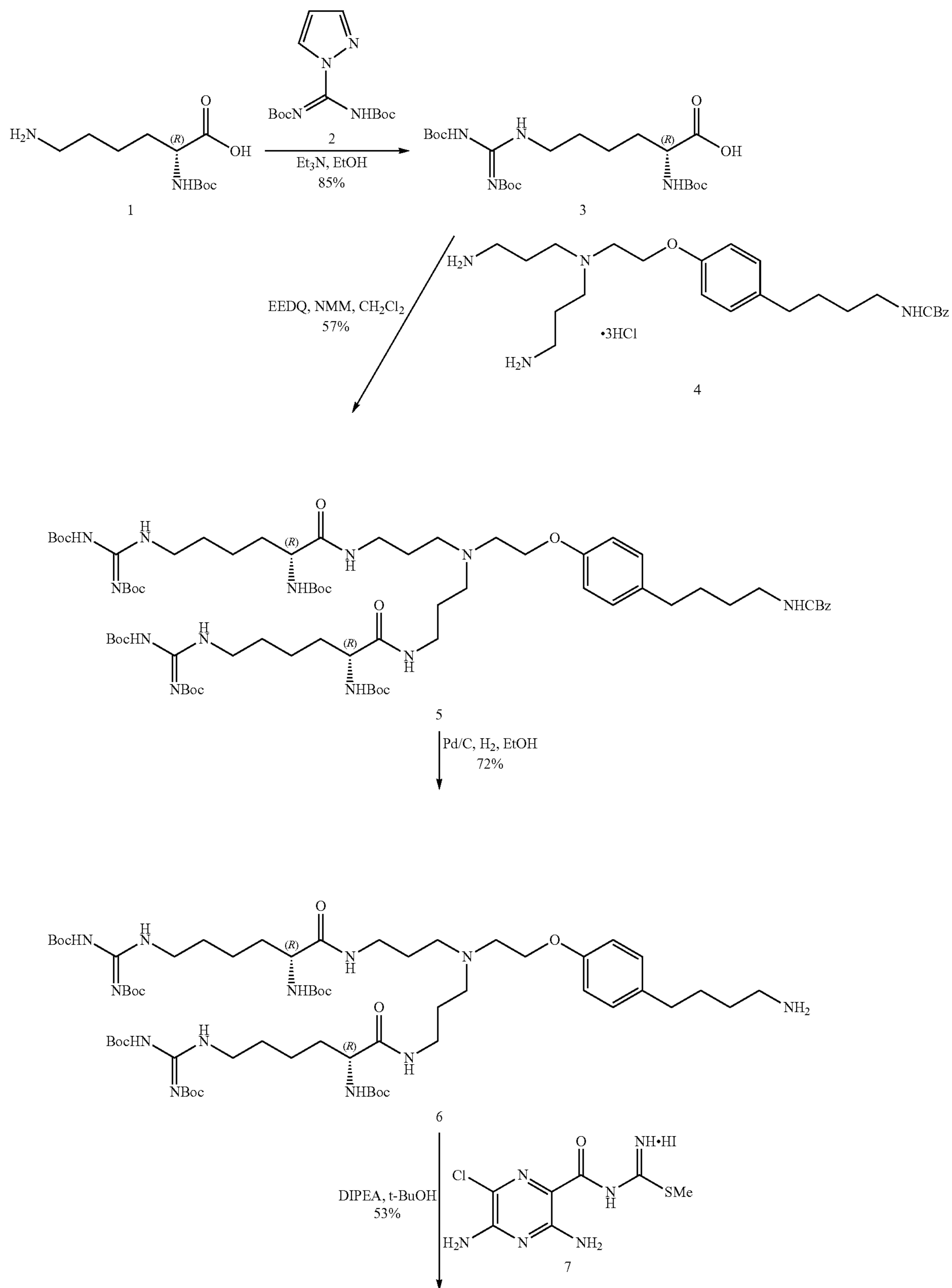
Scheme 1. Preparation of the hydrochloride salt of (2R,2'R)-N,N'-(3,3'-(2-(4-(4-(3-(3,5-diamino-6-chloropyrazine-2-carbonyl)guanidino)butyl)phenoxy)ethylazanediy)bis(propane-3,1-diyl))bis(2-amino-6-guanidinohexanamide) (9).
