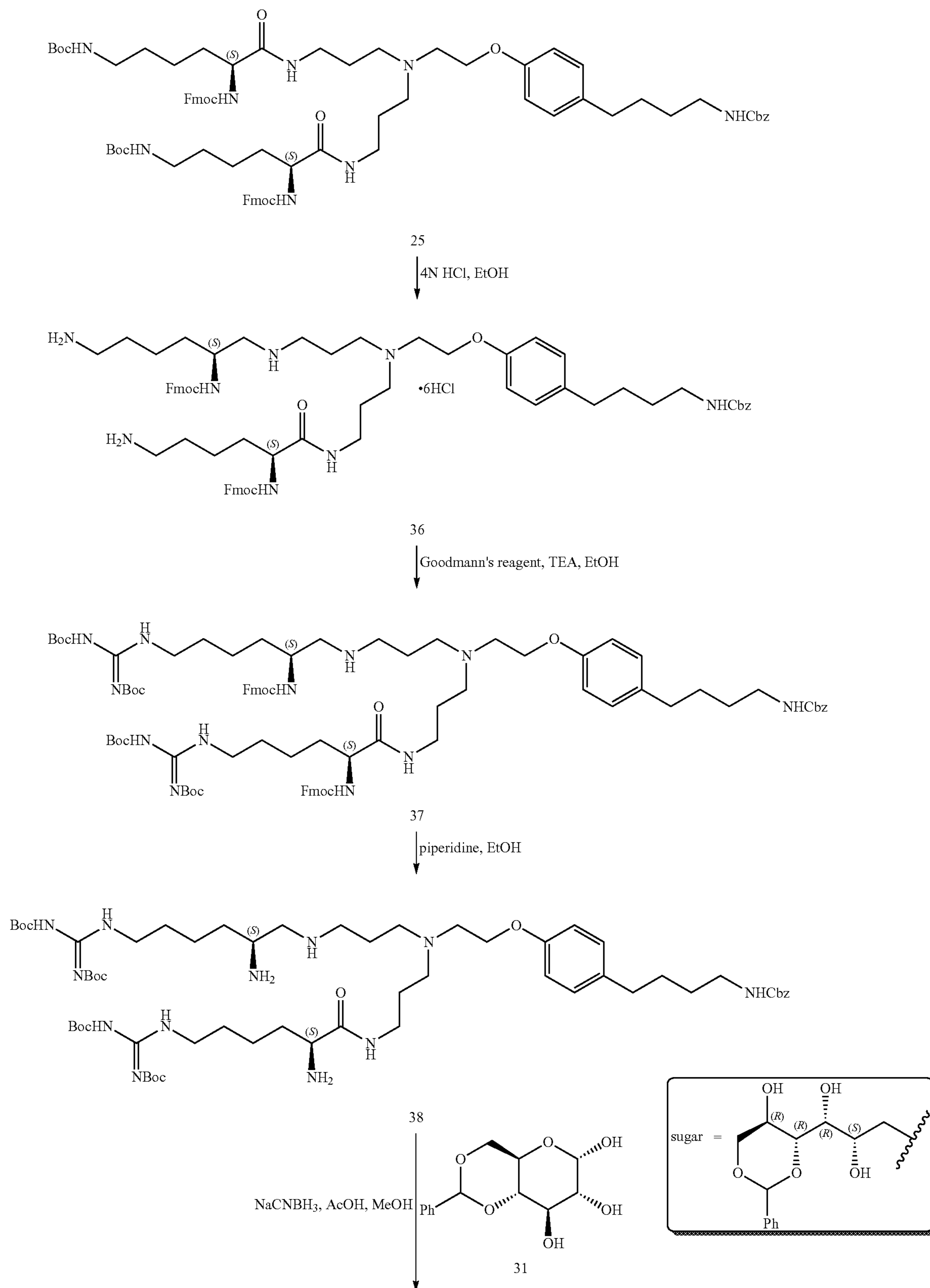
Scheme 6. Preparation of the Hydrochloride Salt of (S,R,R,R,2S,2'S)-N,N'-(3,3'-(2-(4-(4-(3-(3,5-diamino-6-chloropyrazine-2-carbonyl)guanidino)butyl)phenoxy)ethylazanediy)bis(propane-3,1-diyl))bis(6-guanidino-2-((2S,3R,4R,5R)-2,3,4,5,6-pentahydroxyhexylamino)hexanamide)-Compound 42
