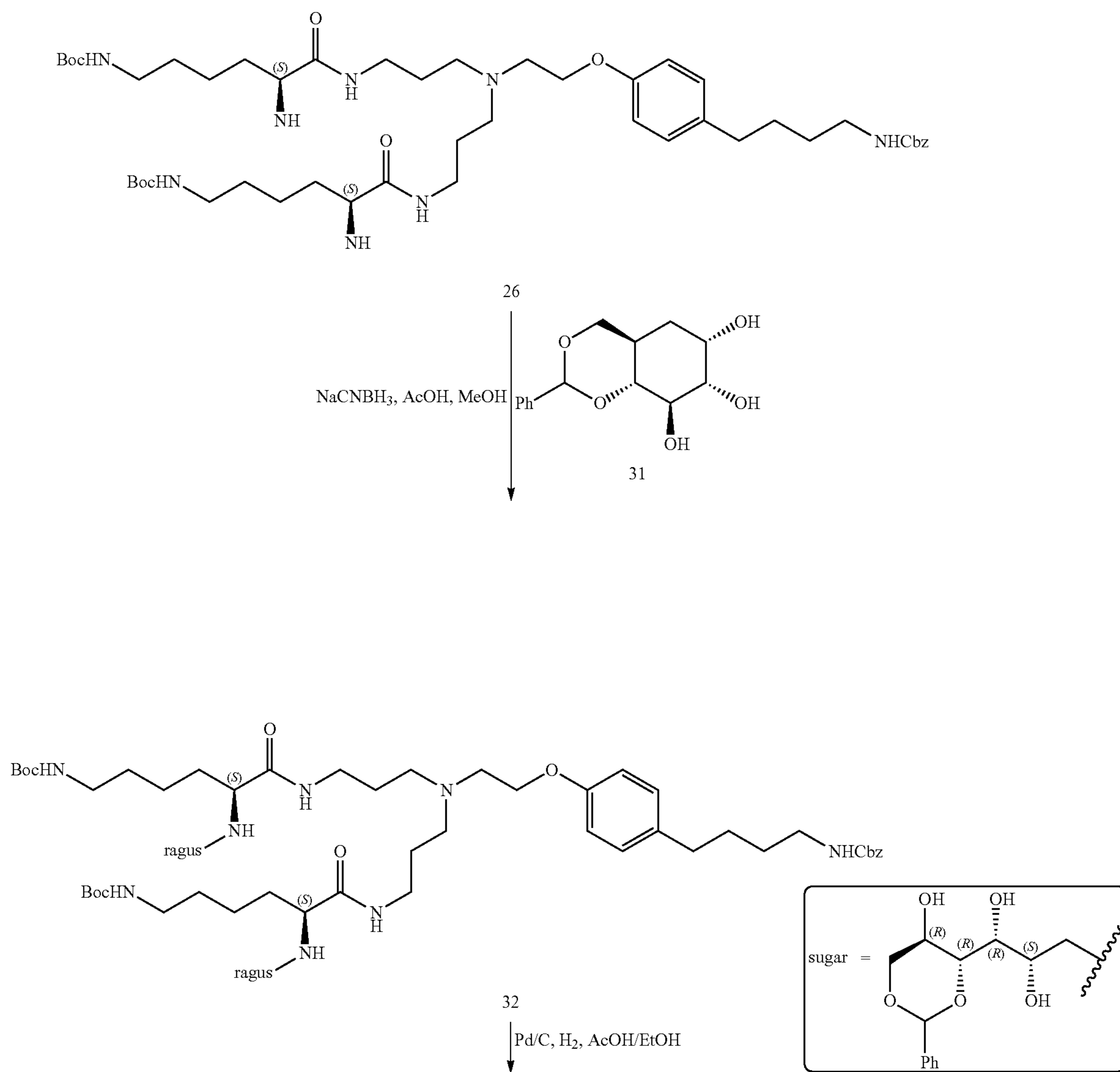
Scheme 5. Preparation of (S,R,R,R,2S,2'S)-N,N'-(3,3'-(2-(4-(4-(3-(3,5-diamino-6-chloropyrazine-2-carboxyl)guanidino)butyl)phenoxy)ethylazanediy)bis(propane-3,1-diyl))bis(6-amino-2-((2S,3R,4R,5R)-2,3,4,5,6-pentahydroxyhexylamino)hexanamide)-35
