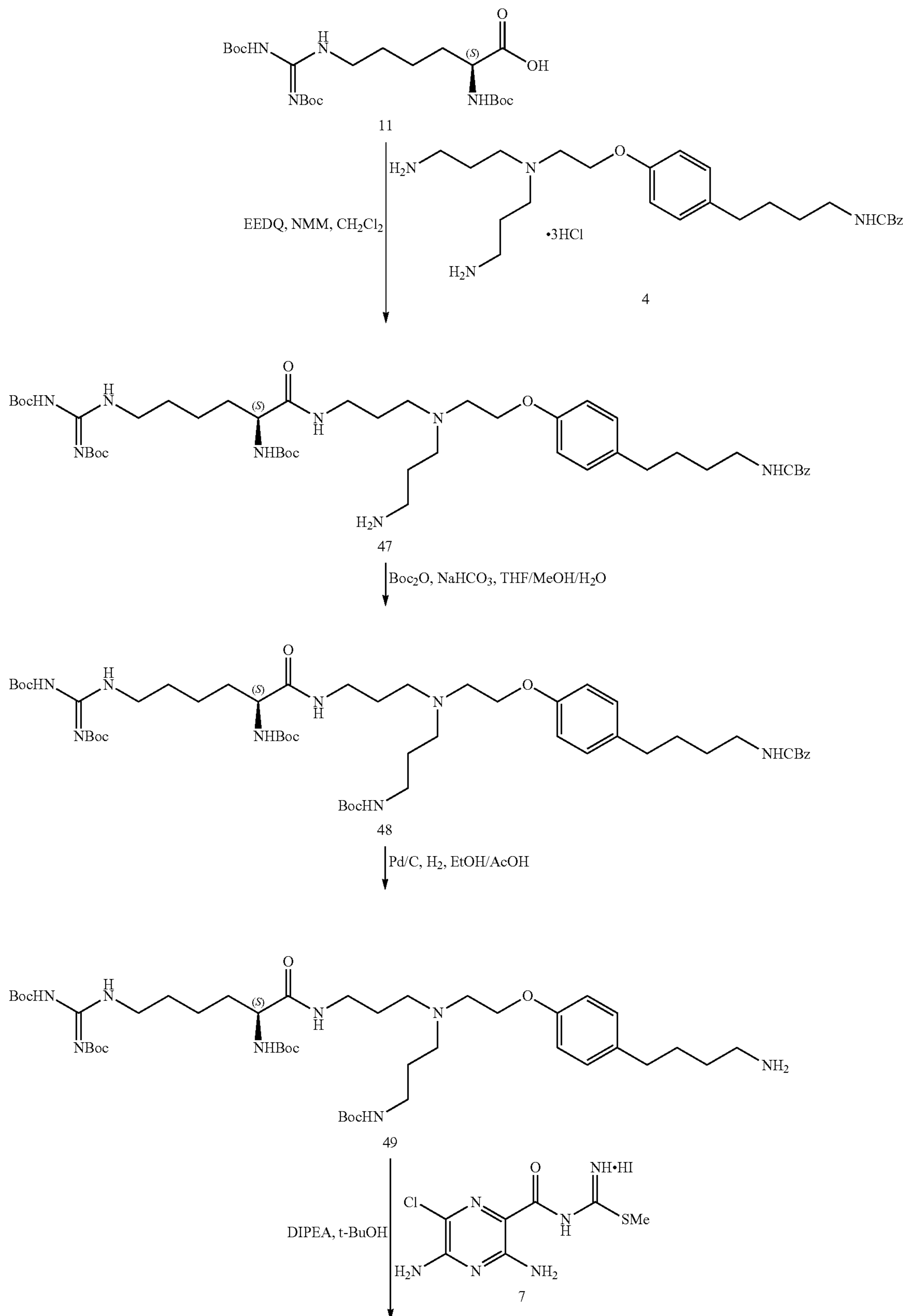
Scheme 8. The Preparation of the Hydrochloride Salt of (S)-3,5-diamino-N-(N-(4-(4-(2-((3-(2-amino-6-guanidinohexanamido)propyl)(3-aminopropyl)amino)ethoxy)phenyl)butyl)-carbamimidoyl)-6-chloropyrazine-2-carboxamide- Compound 51
