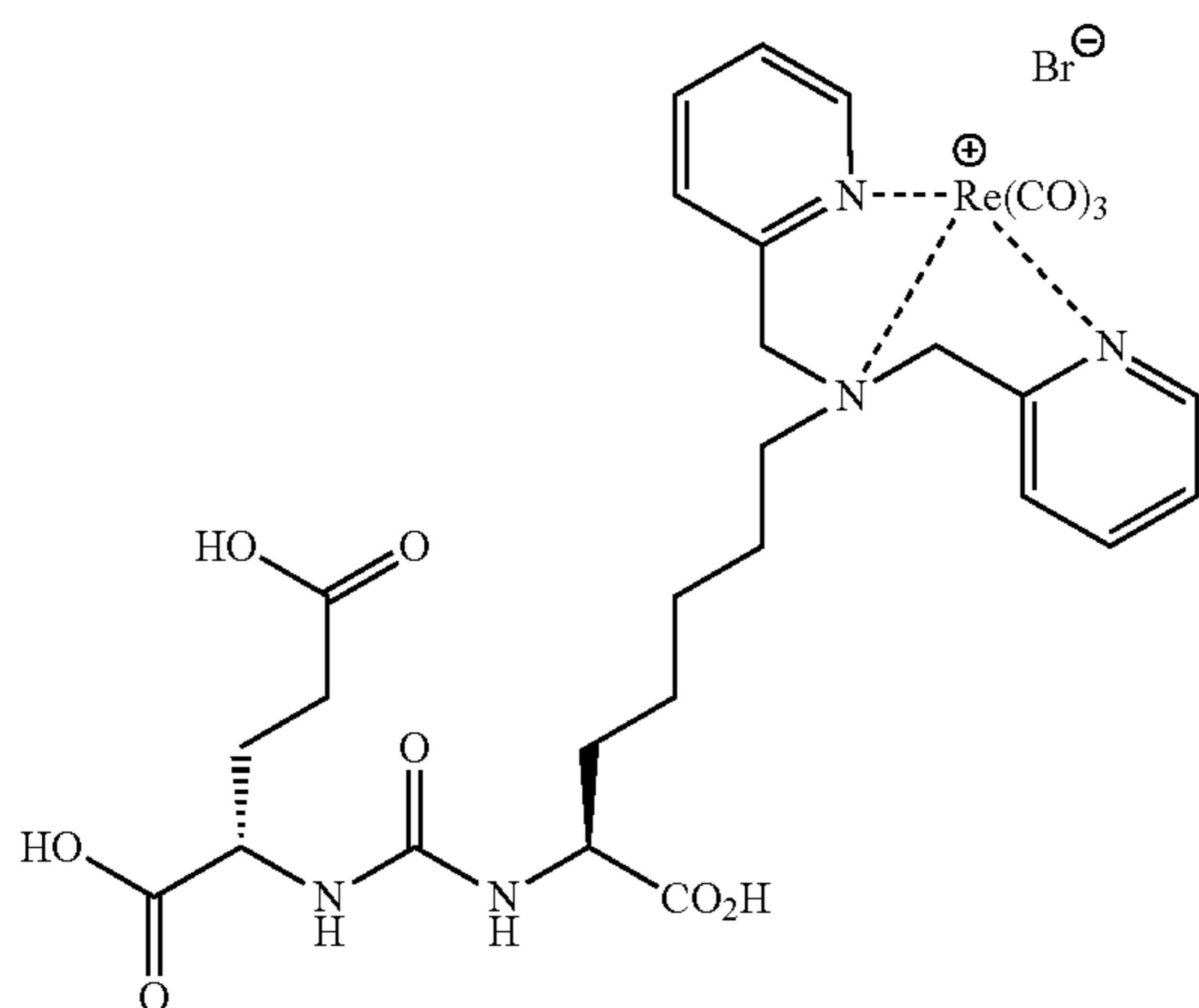
2-{3-[1-Carboxy-5-(carboxymethyl-pyridin-2-ylmethyl-amino)-pentyl]-ureido}-pentanedioic acid (26)
