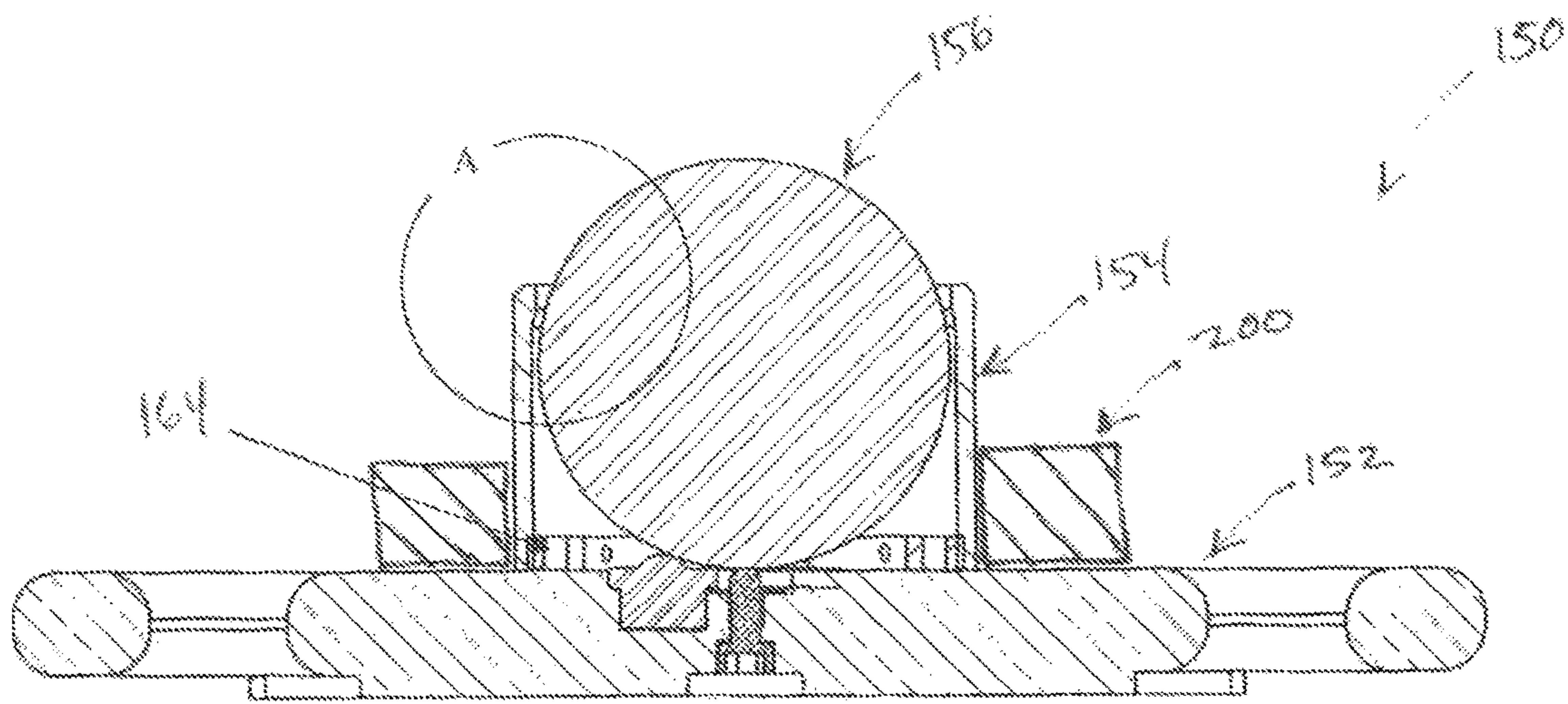
Section view
