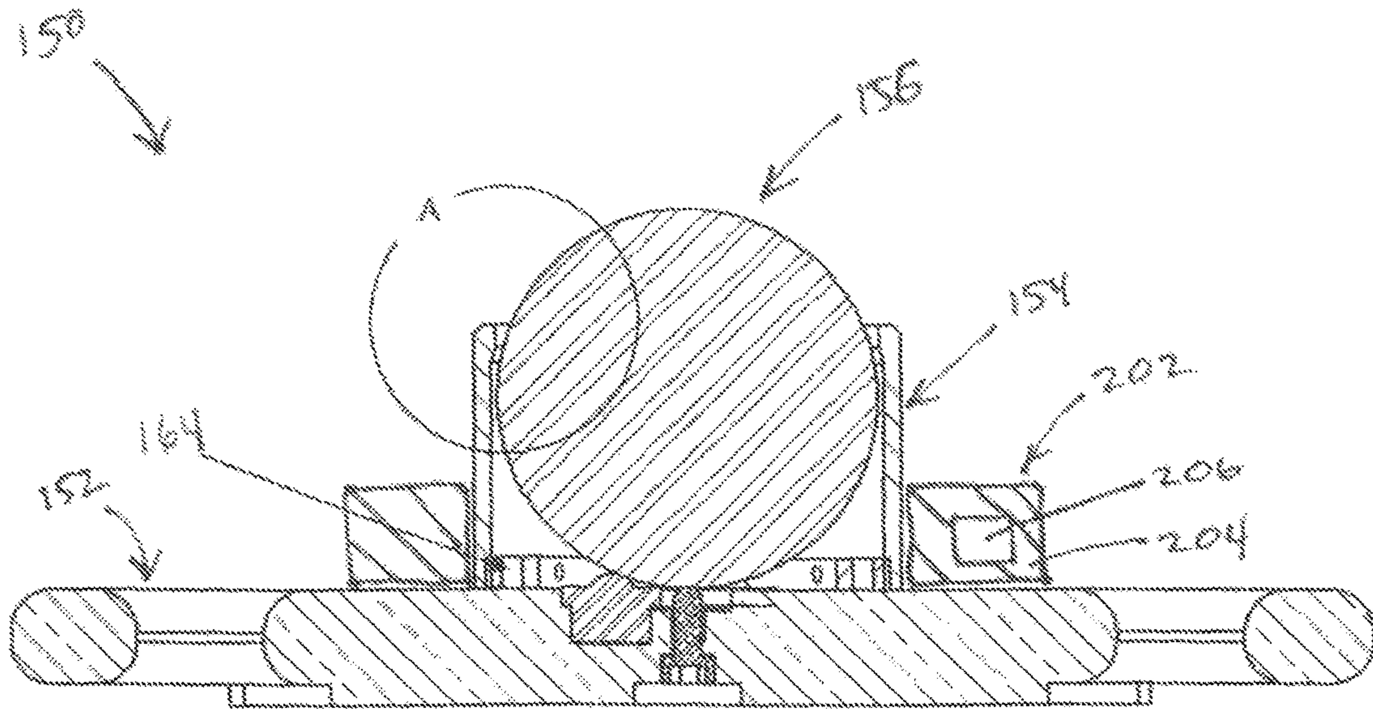
Section view
