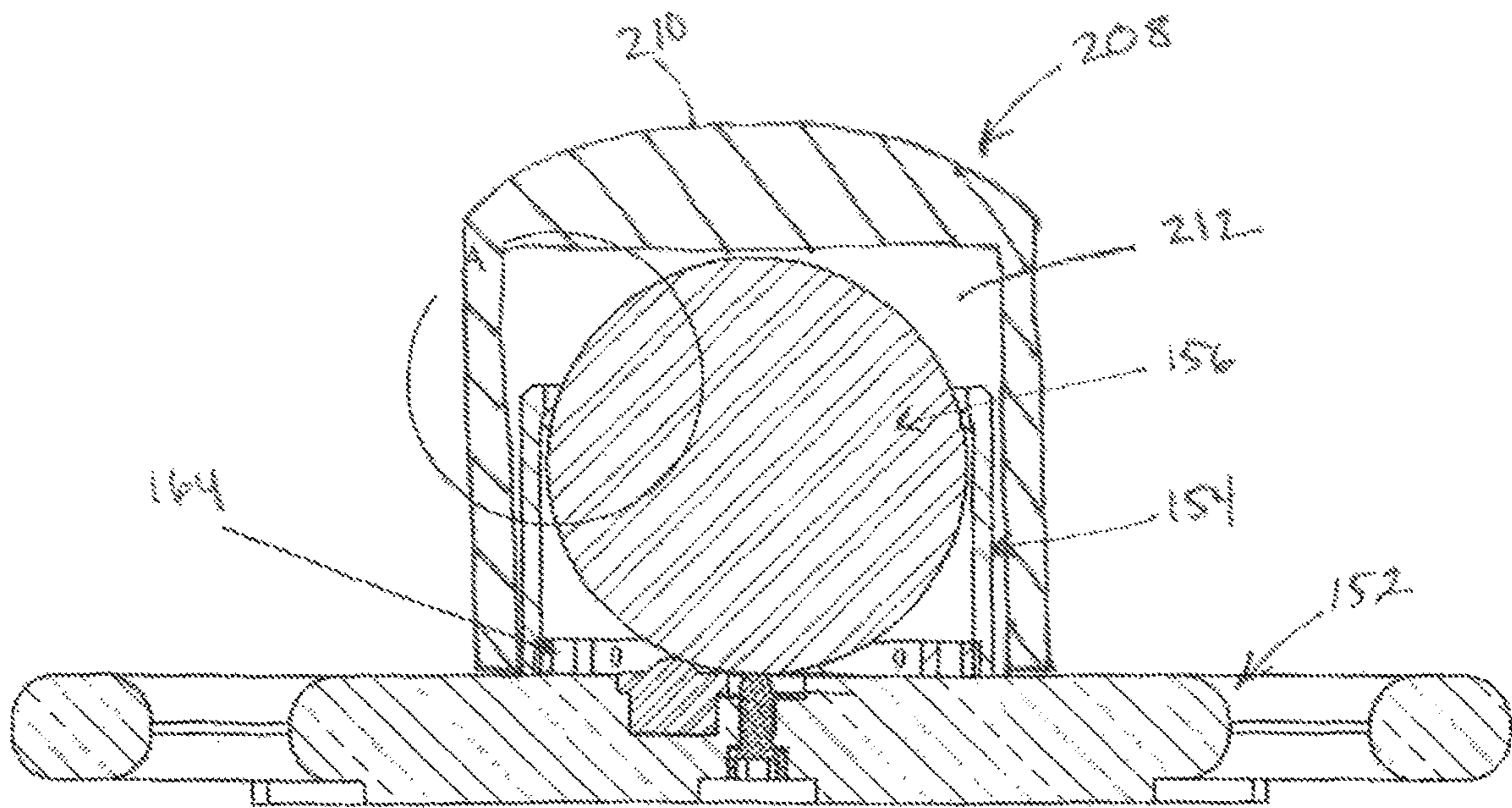
Section view
