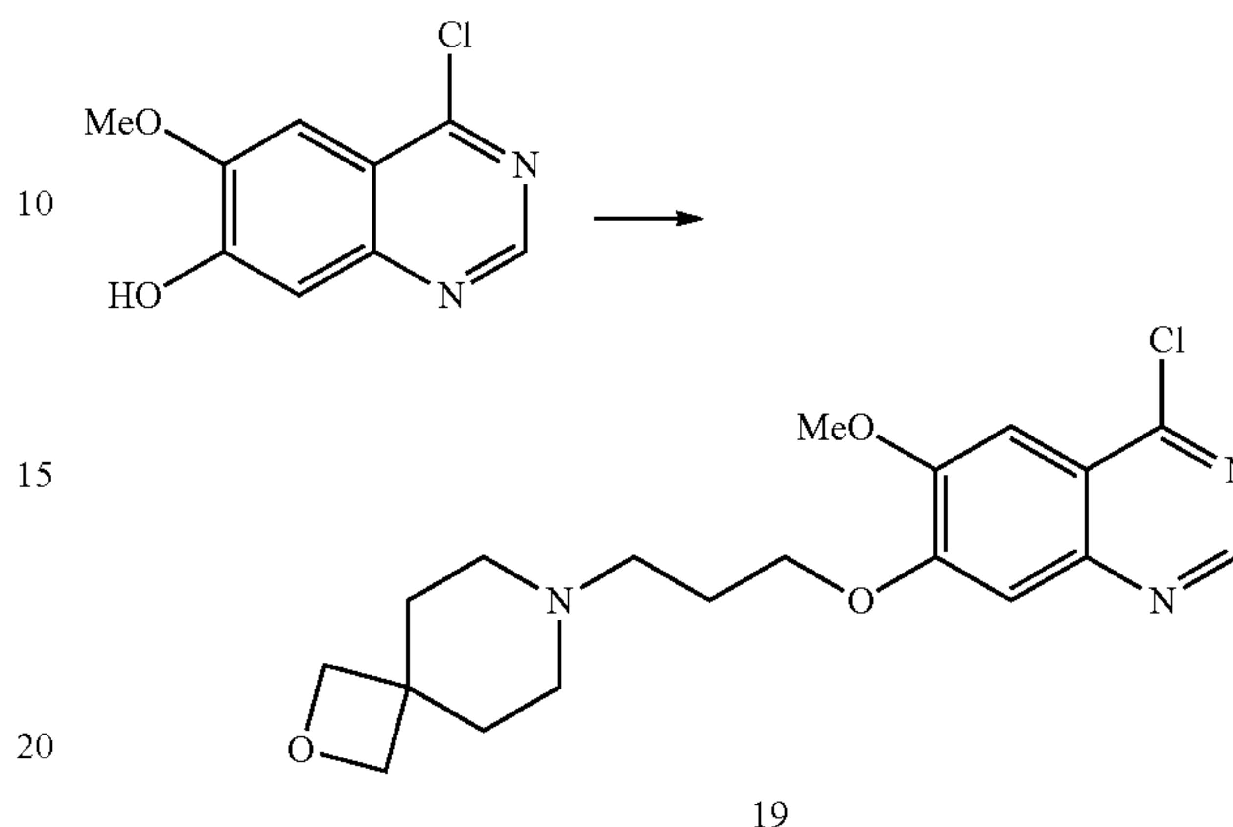
Compound 19
