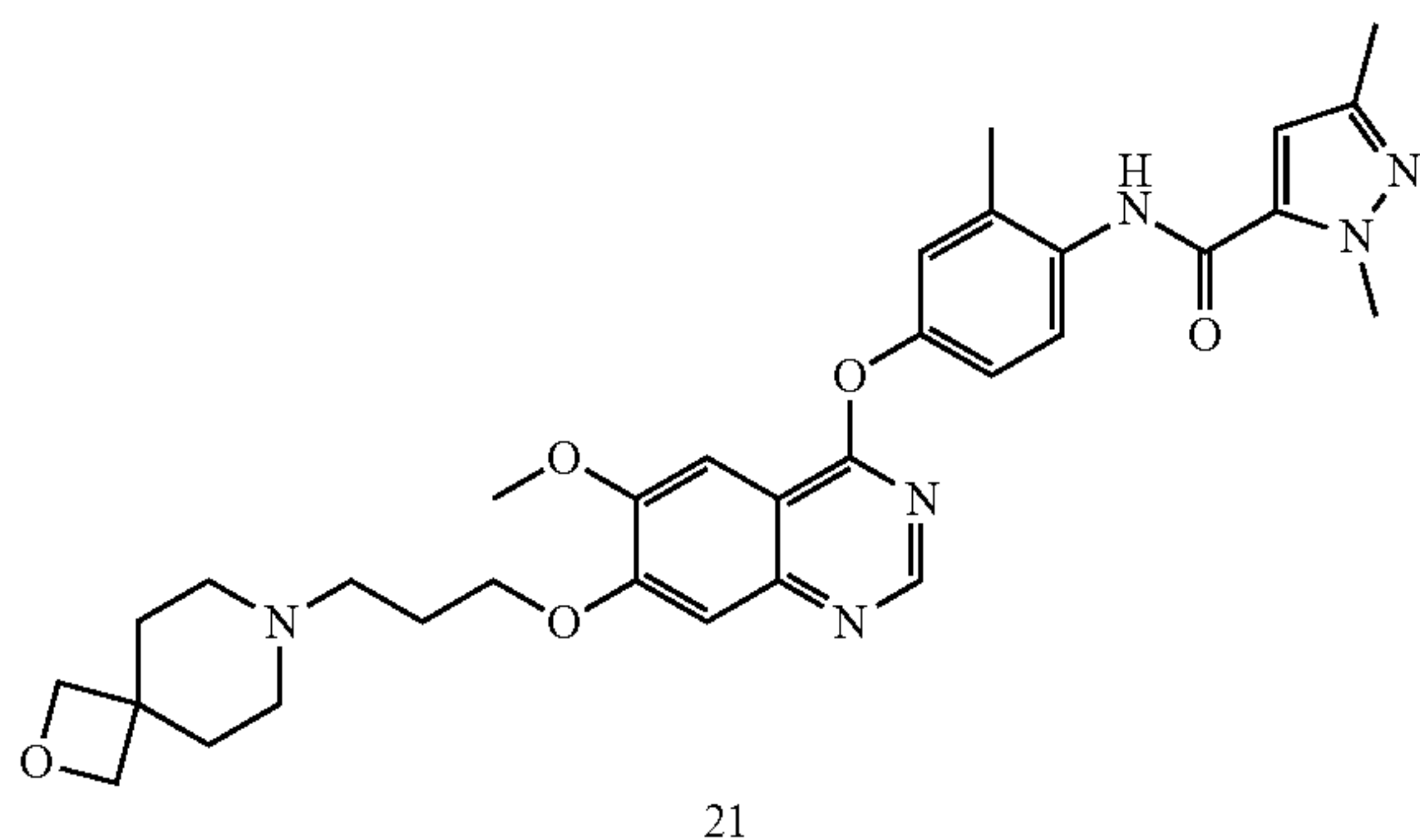
Compound 21
