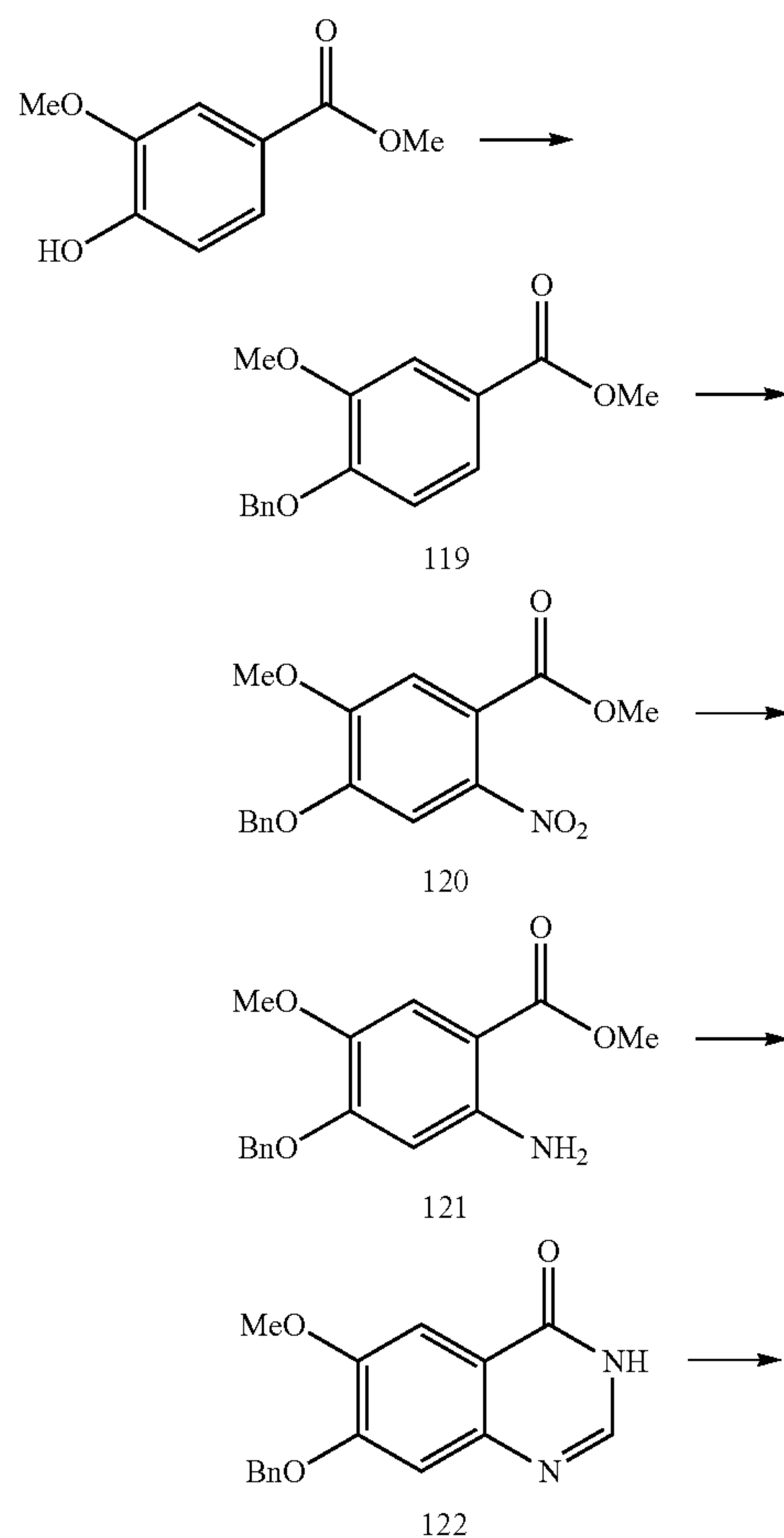
Scheme 3
