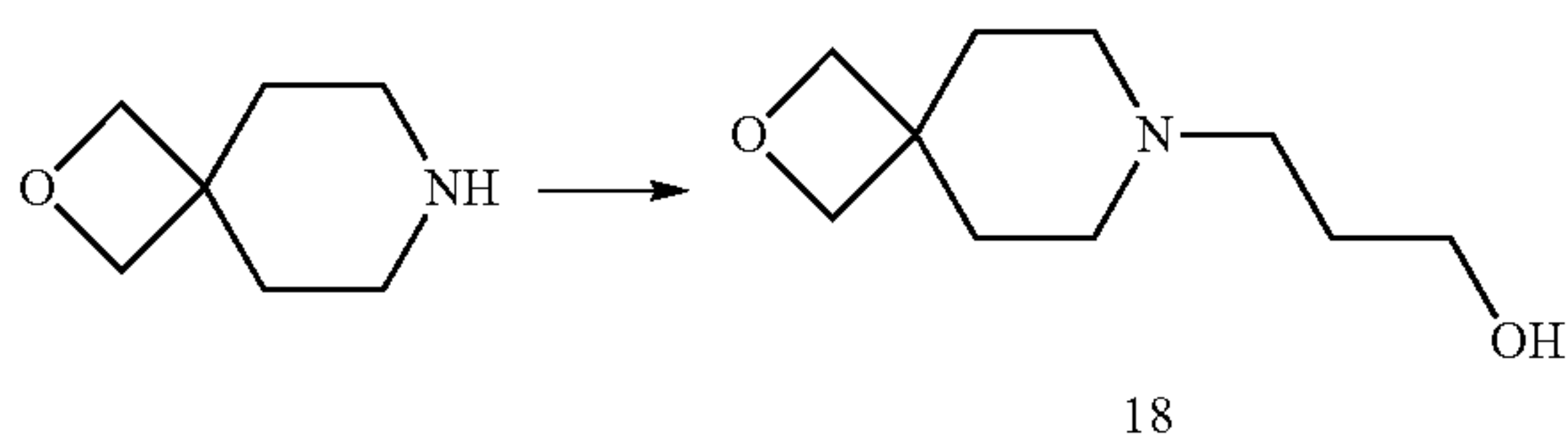
Compound 18
