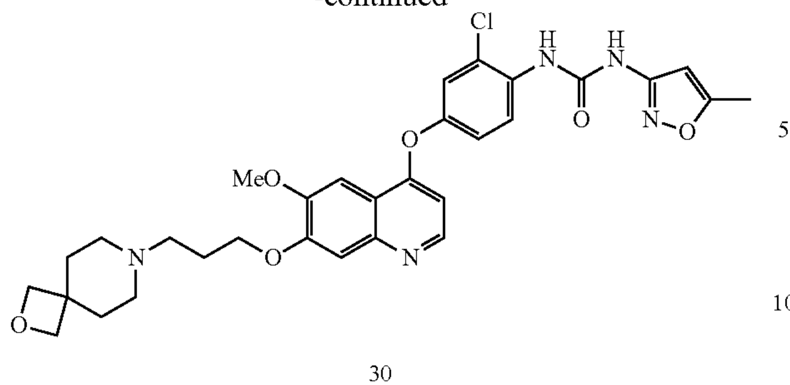
Compound 30
