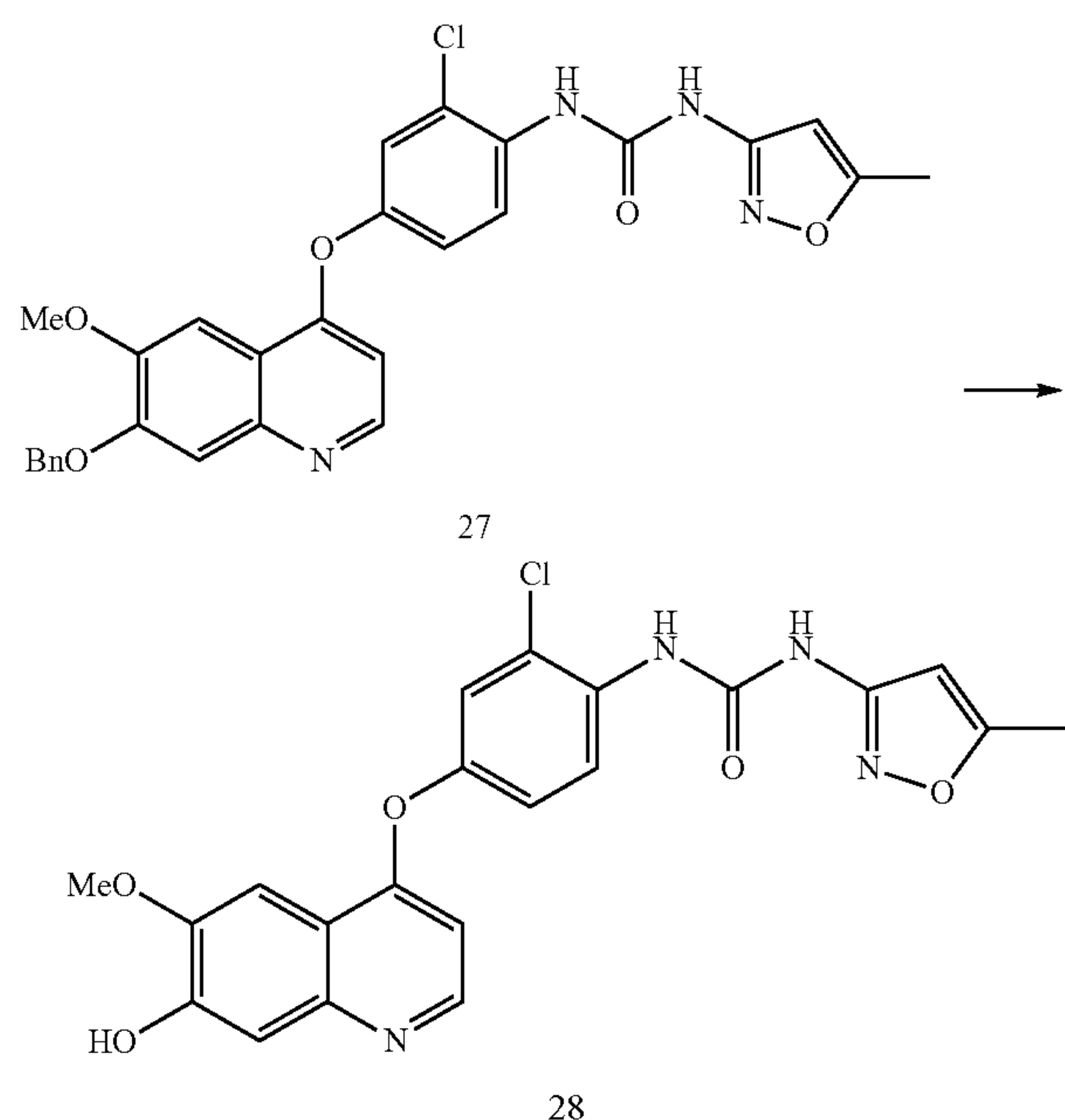
Compound 28
