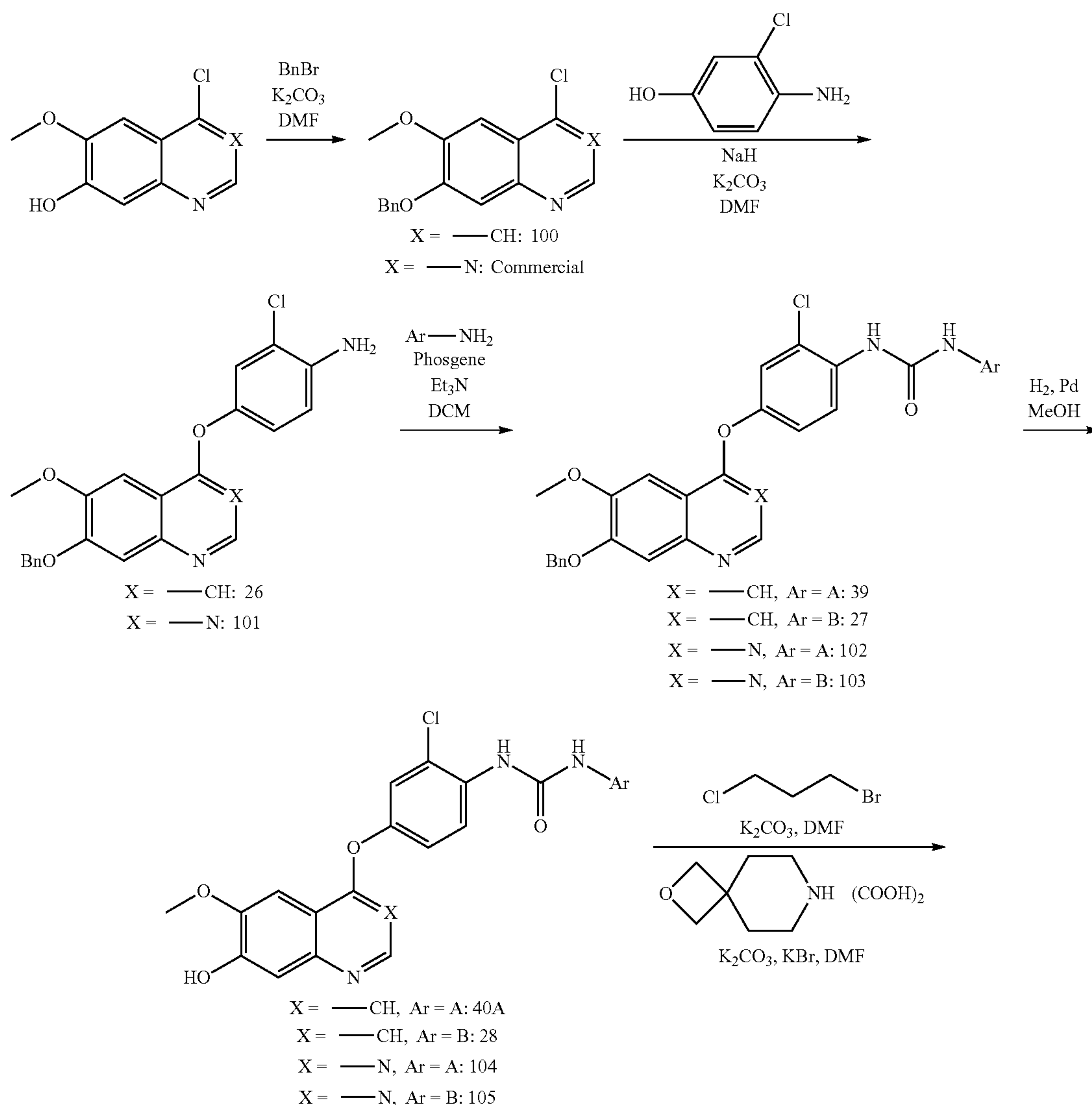
Scheme 1
