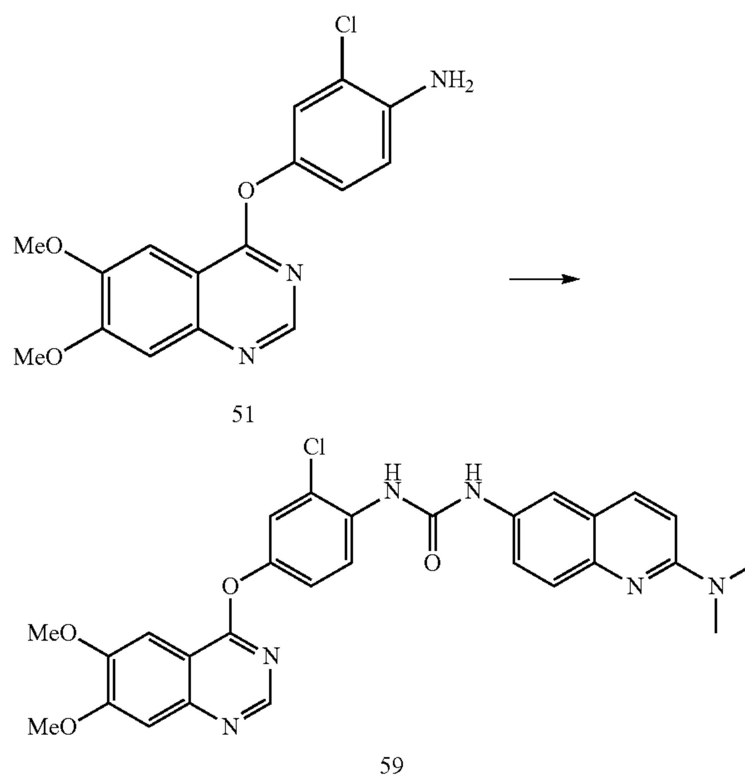
Compound 59
