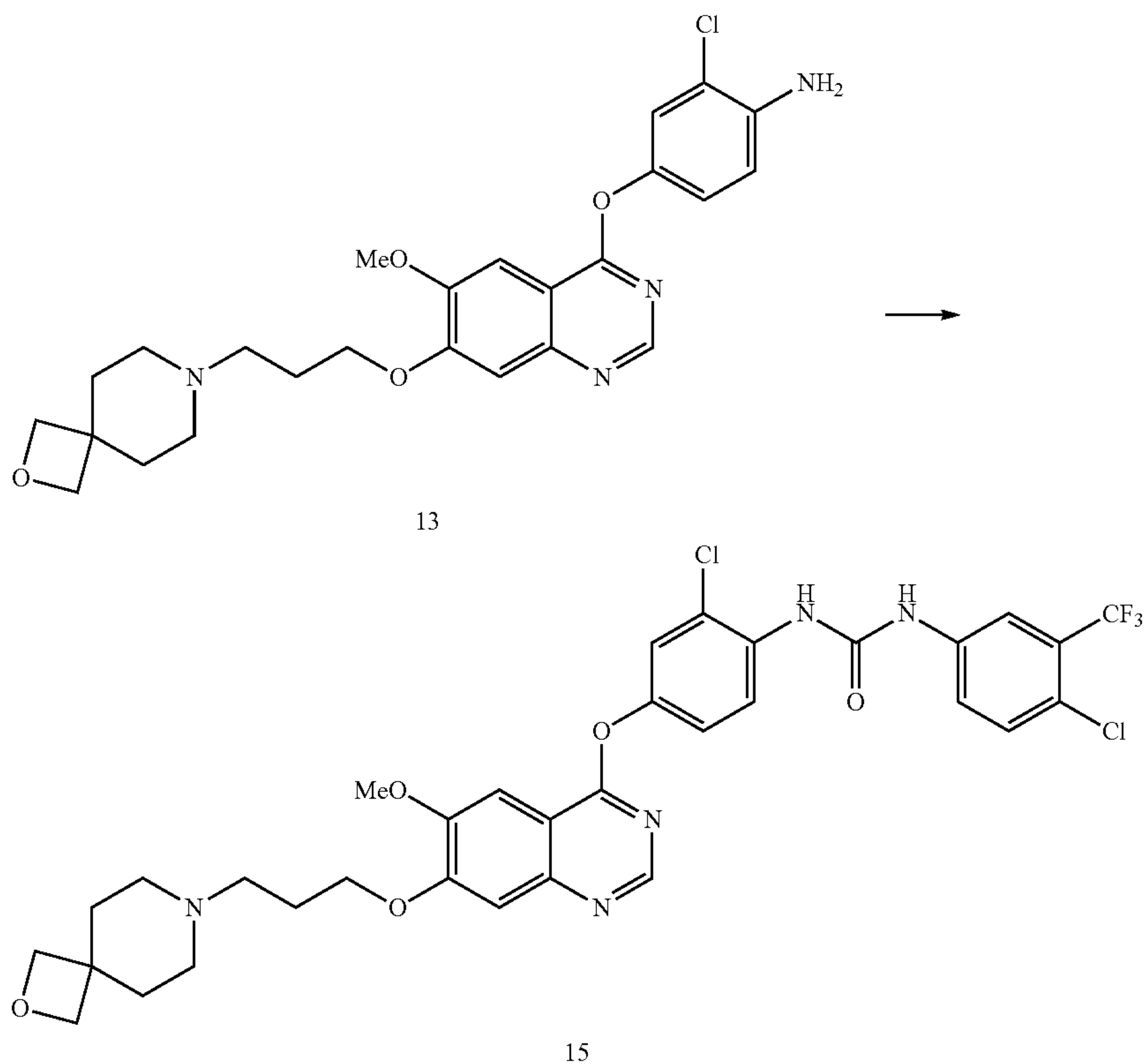
Compound 15
