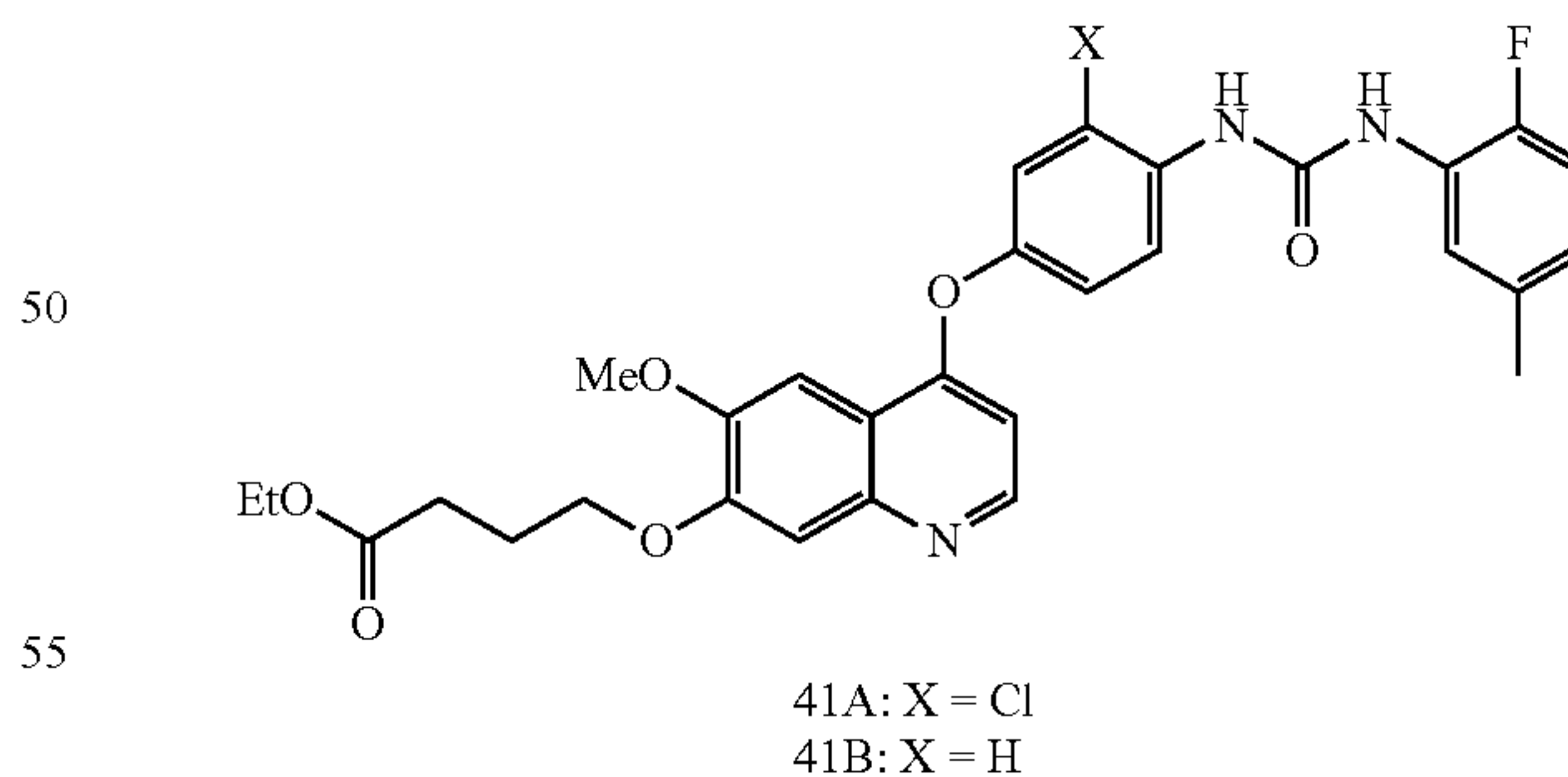
Compound 41
