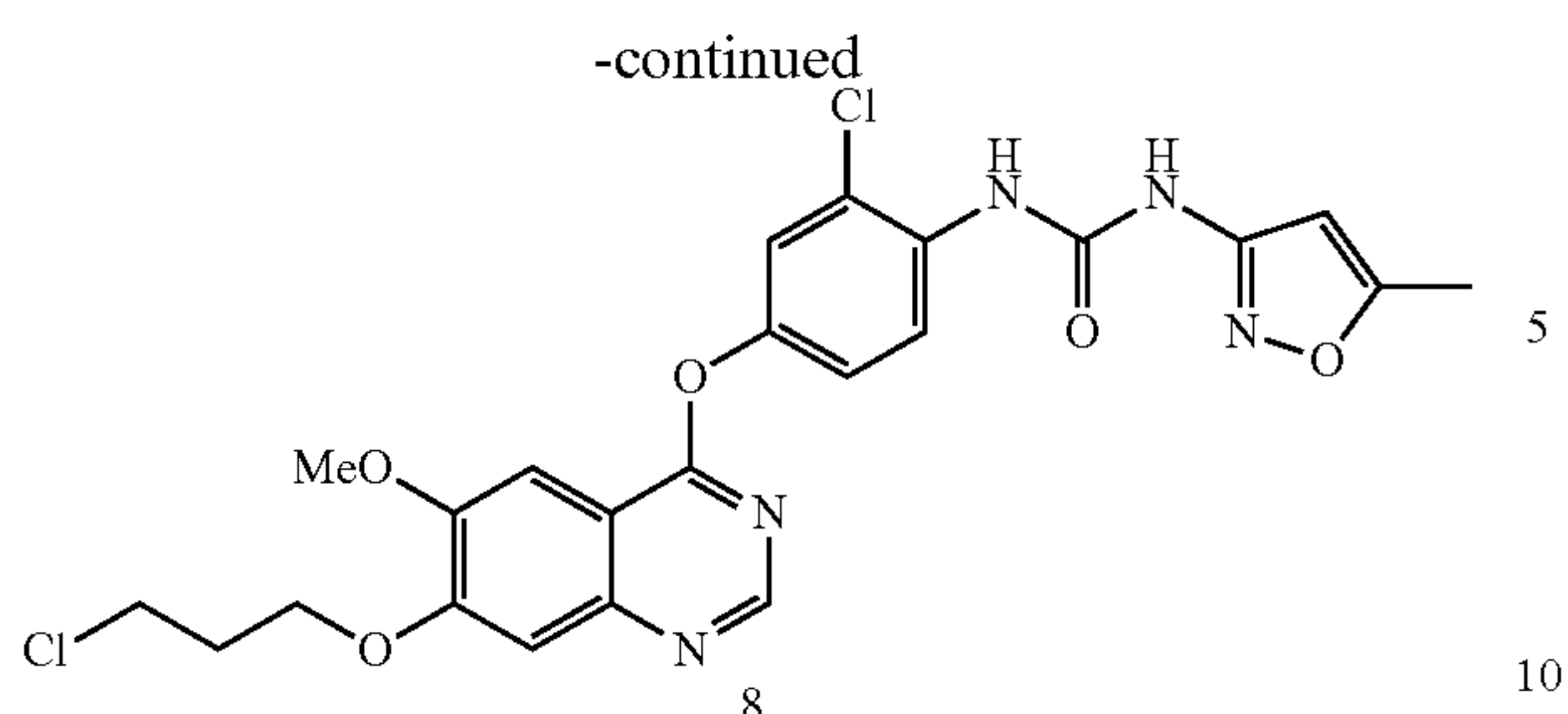
Compound 8
