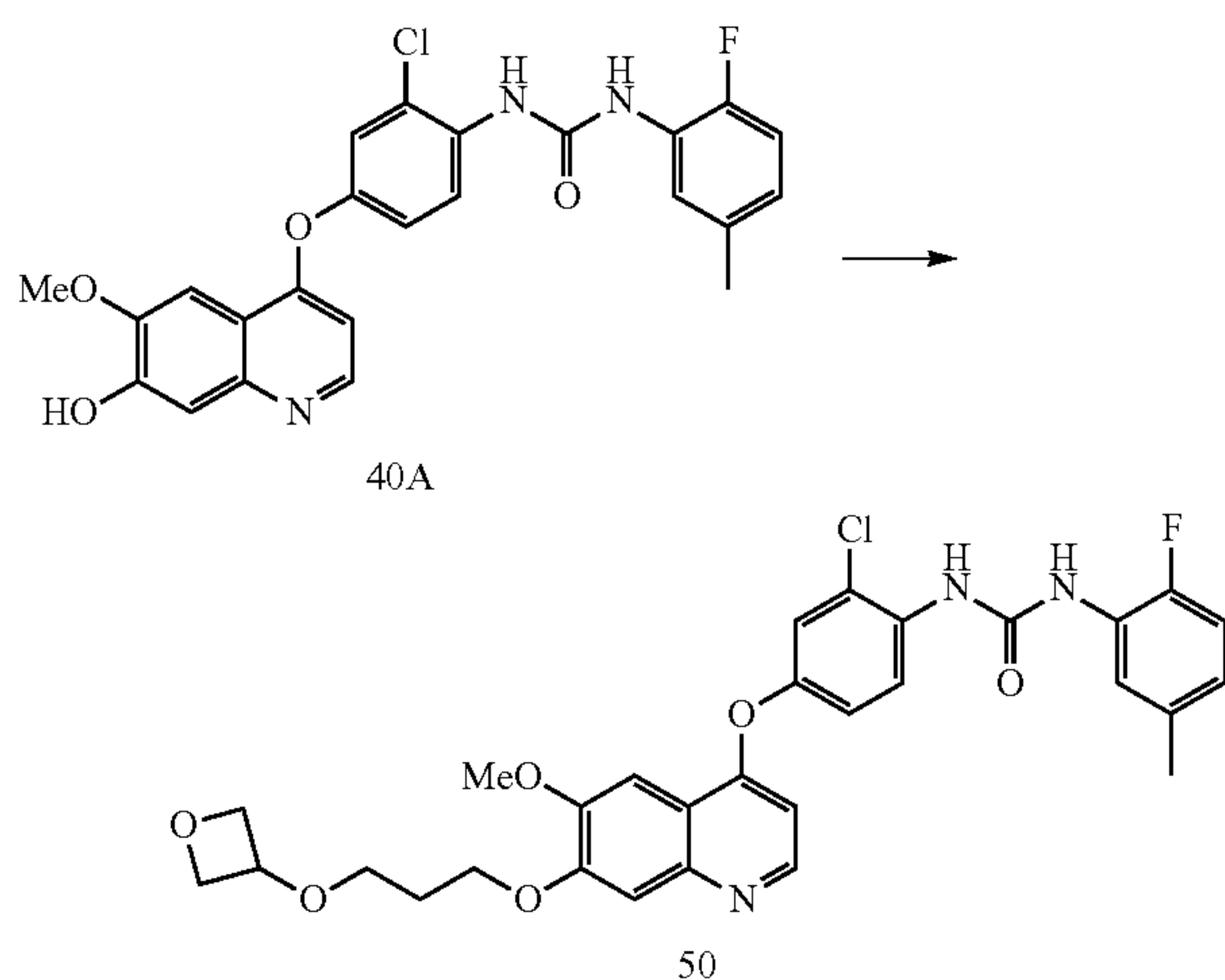
Compound 50
