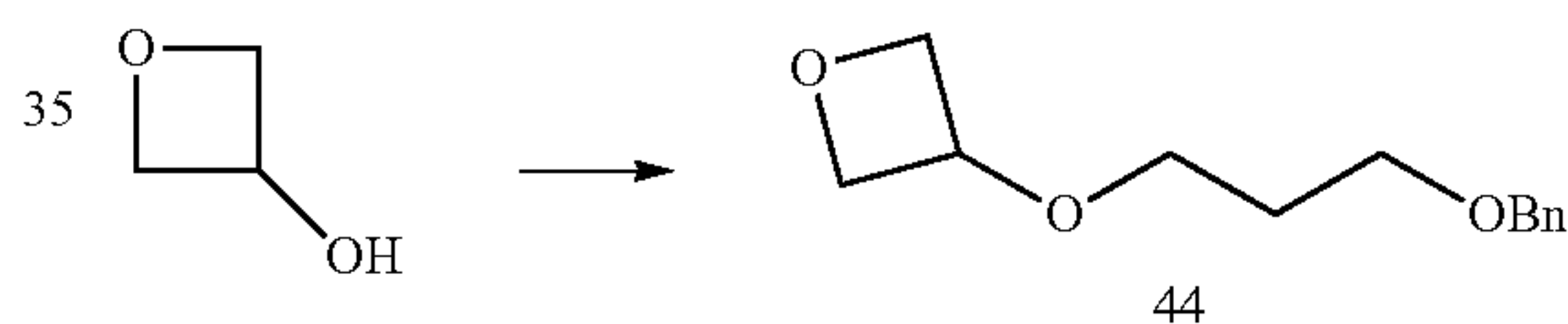
Compound 44
