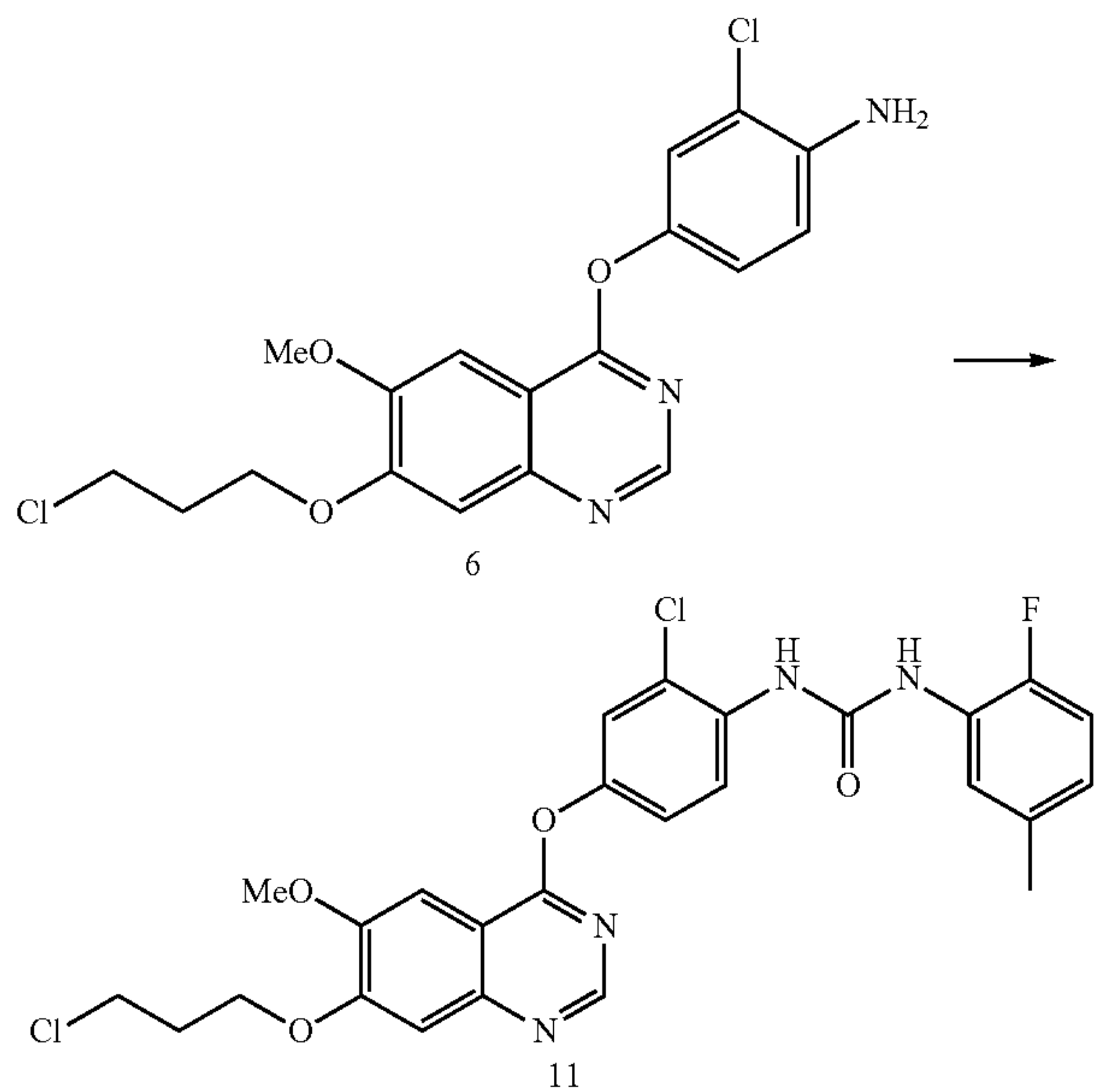
Compound 11
