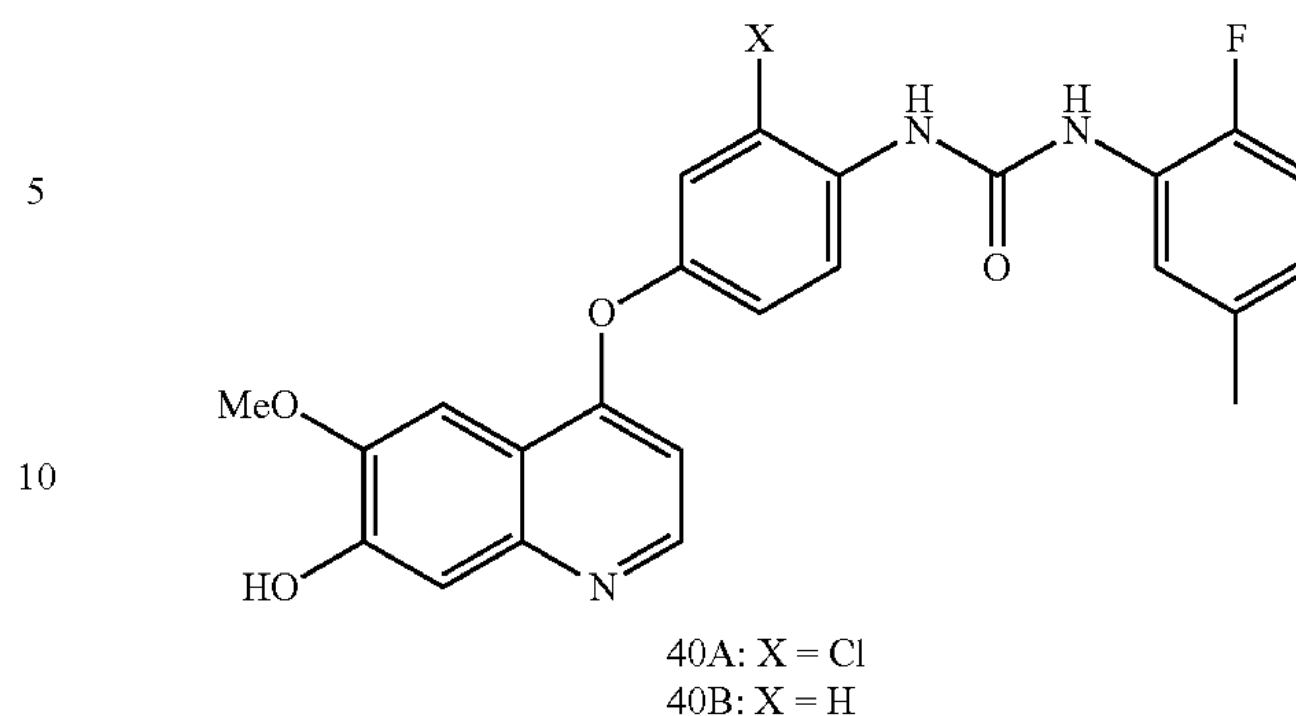
Compound 40
