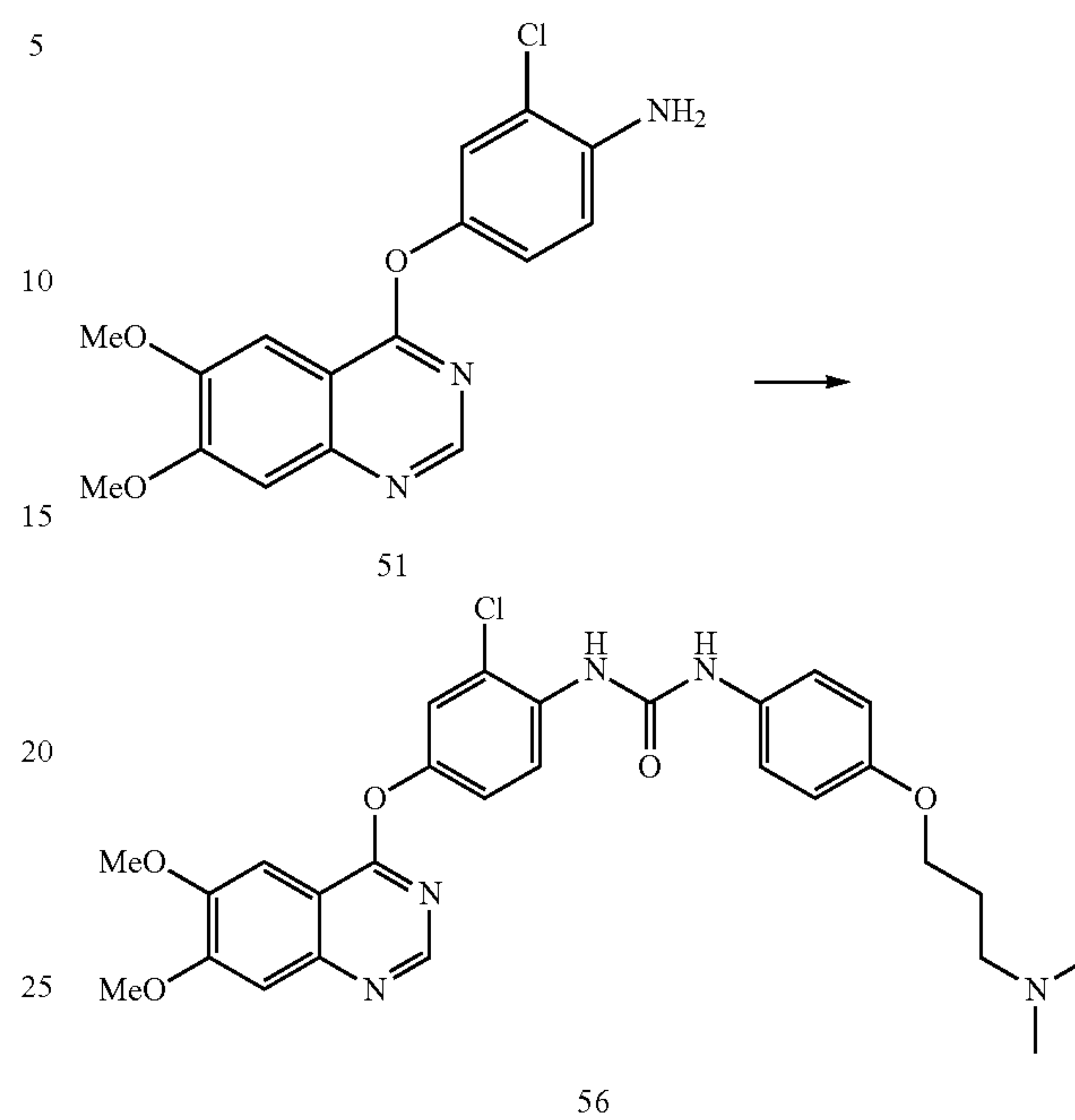
Compound 56
