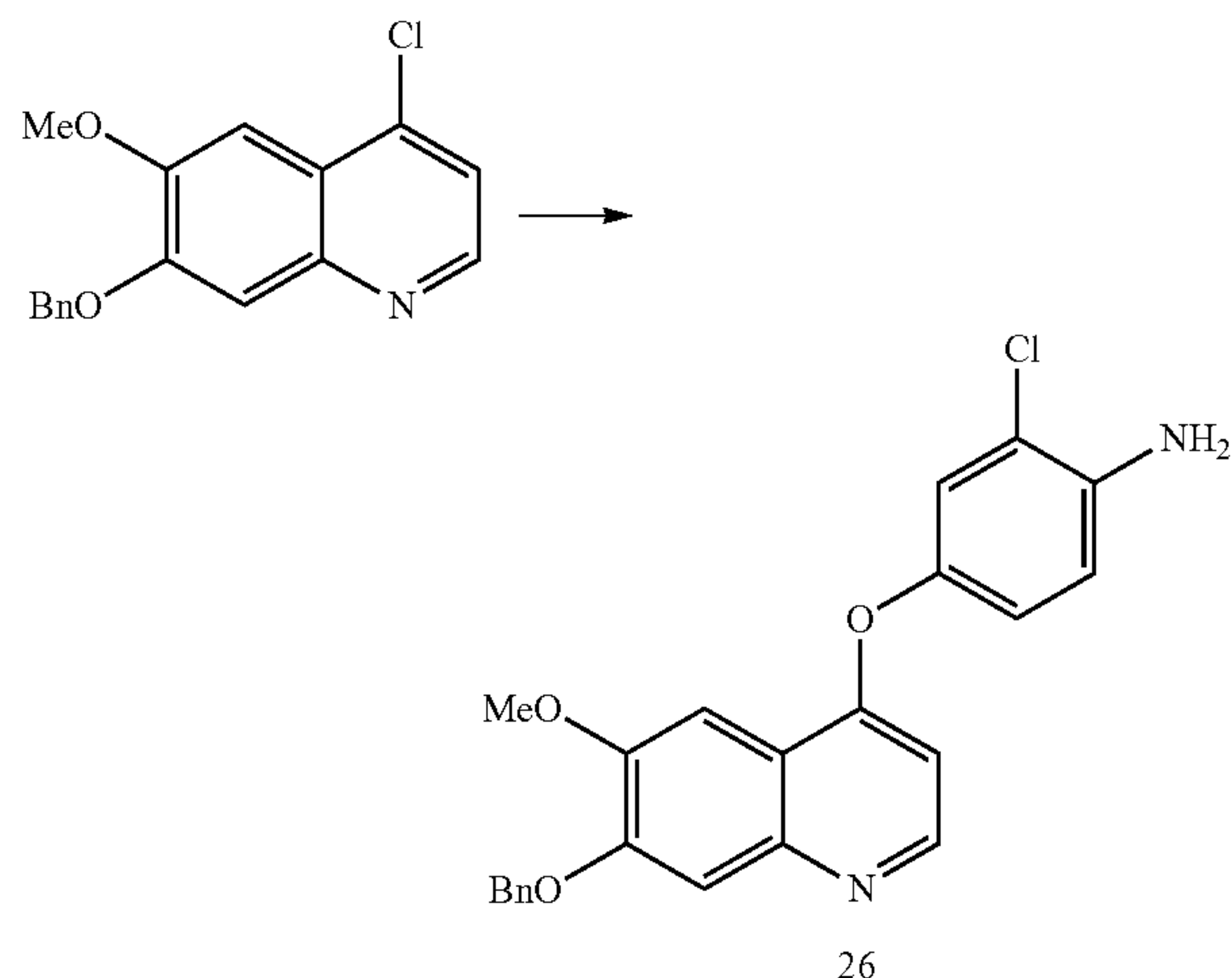
Compound 26
