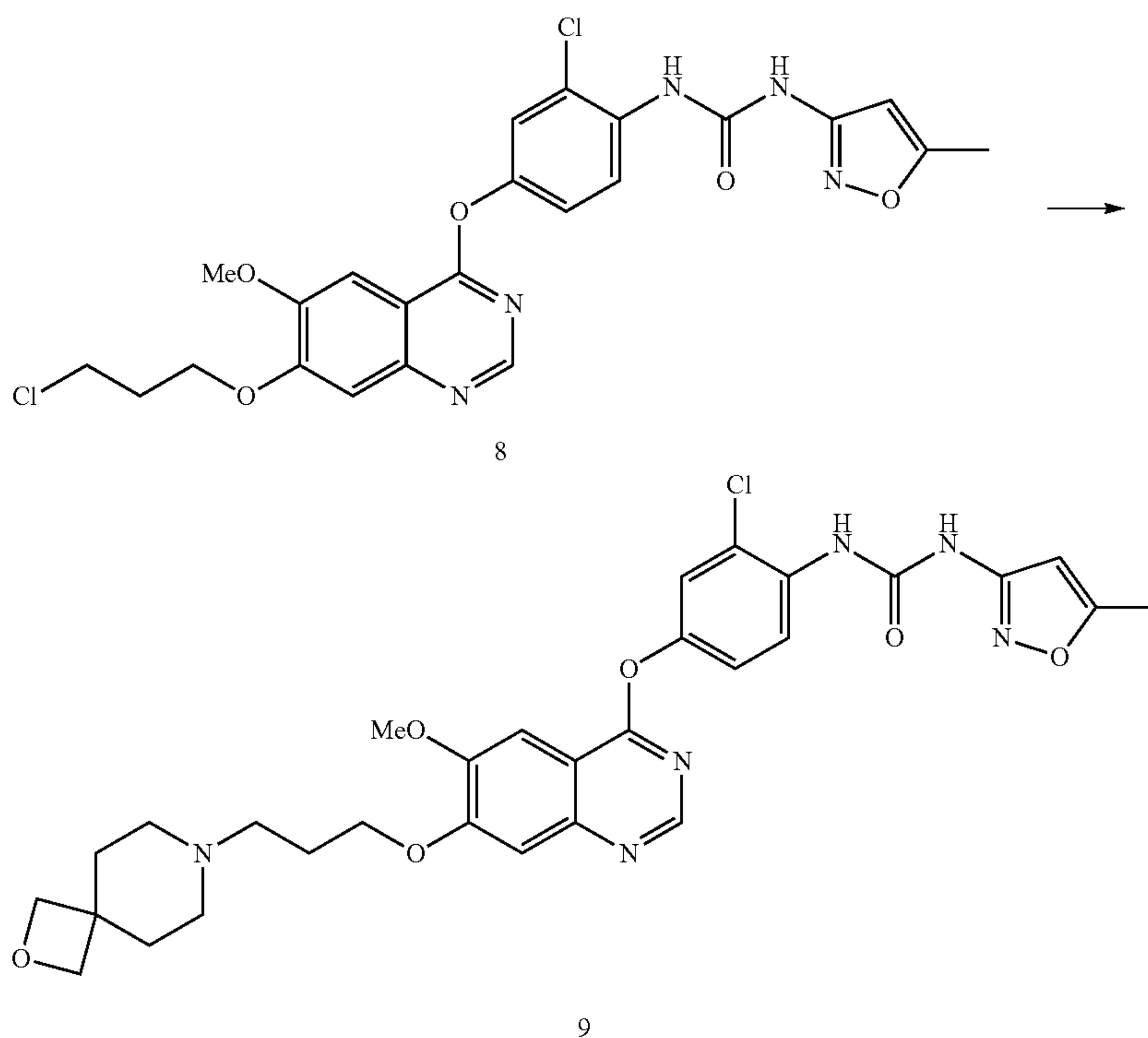
Compound 9
