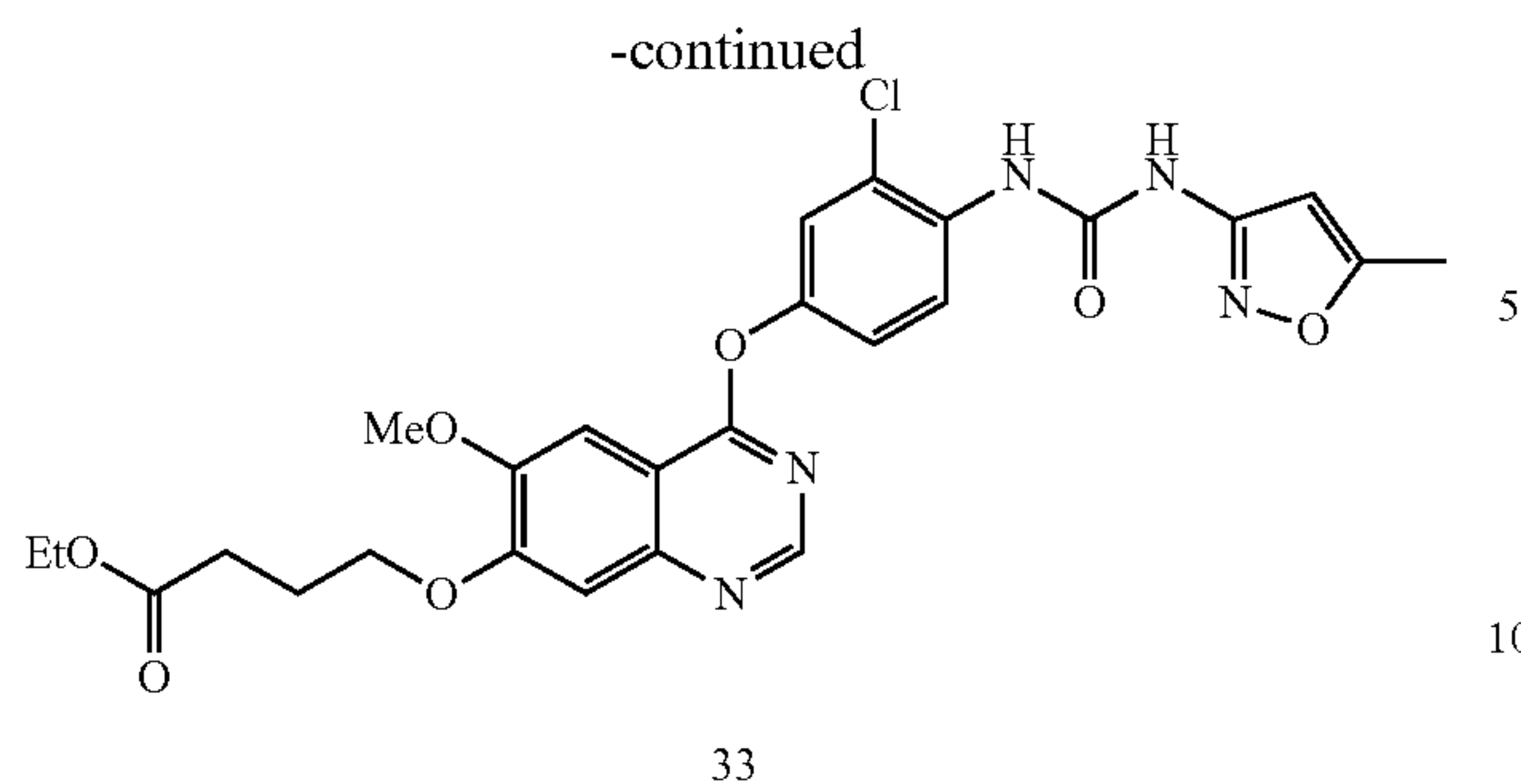
Compound 33
