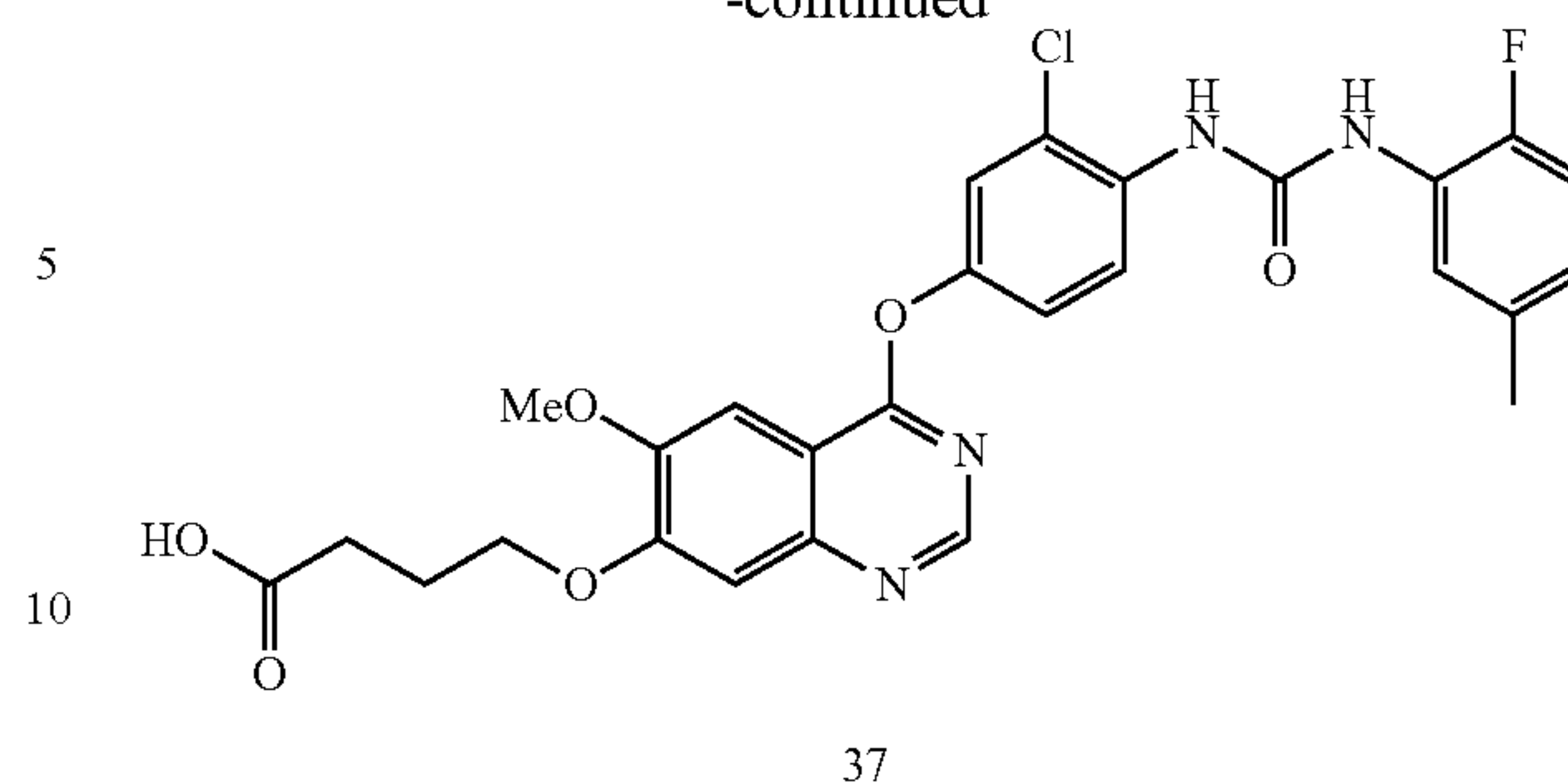
Compound 37
