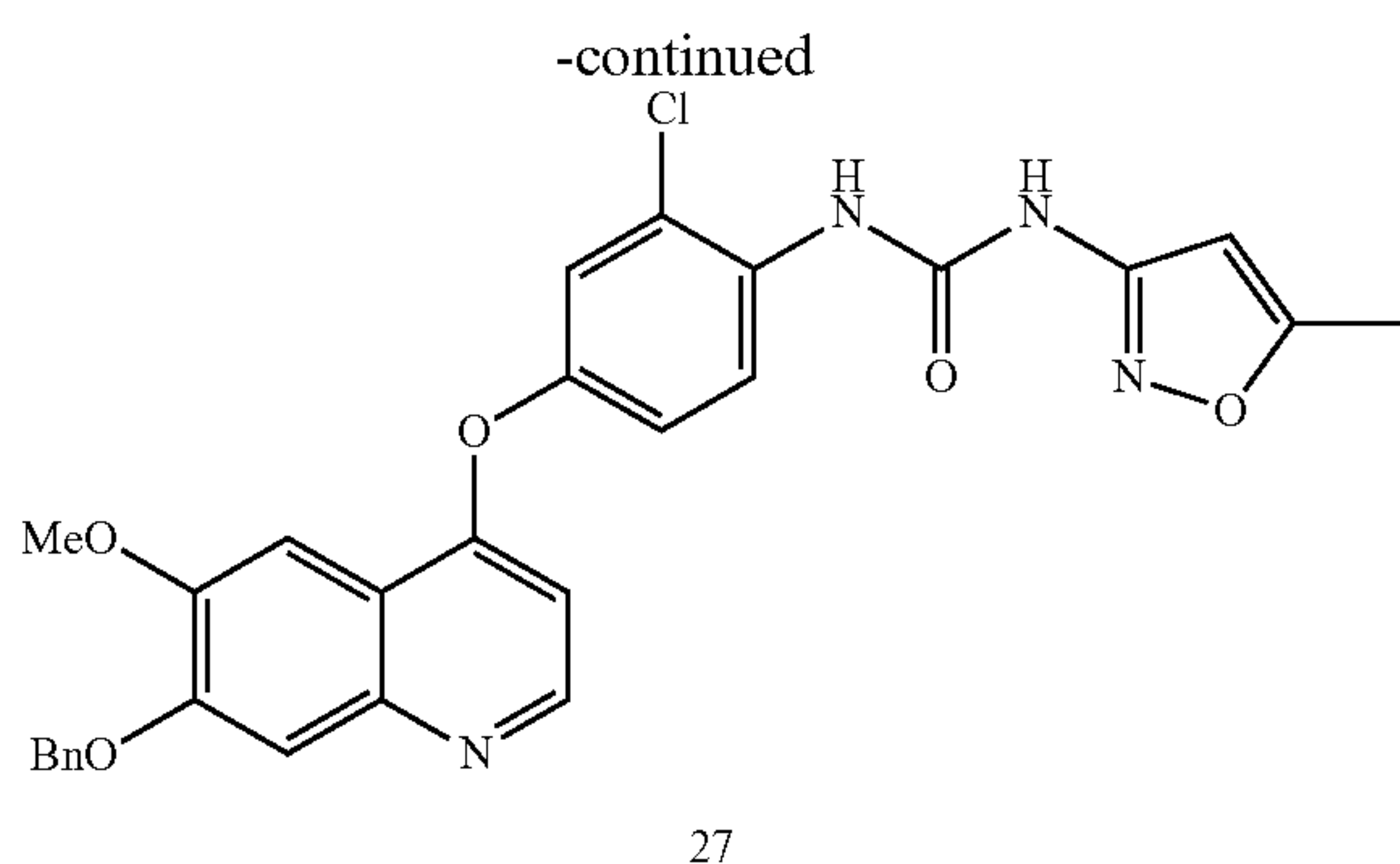
Compound 27
