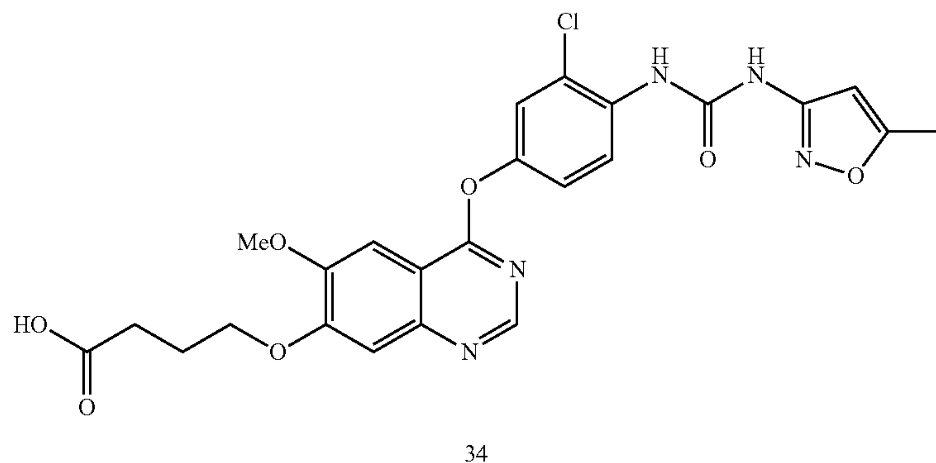
Compound 34
