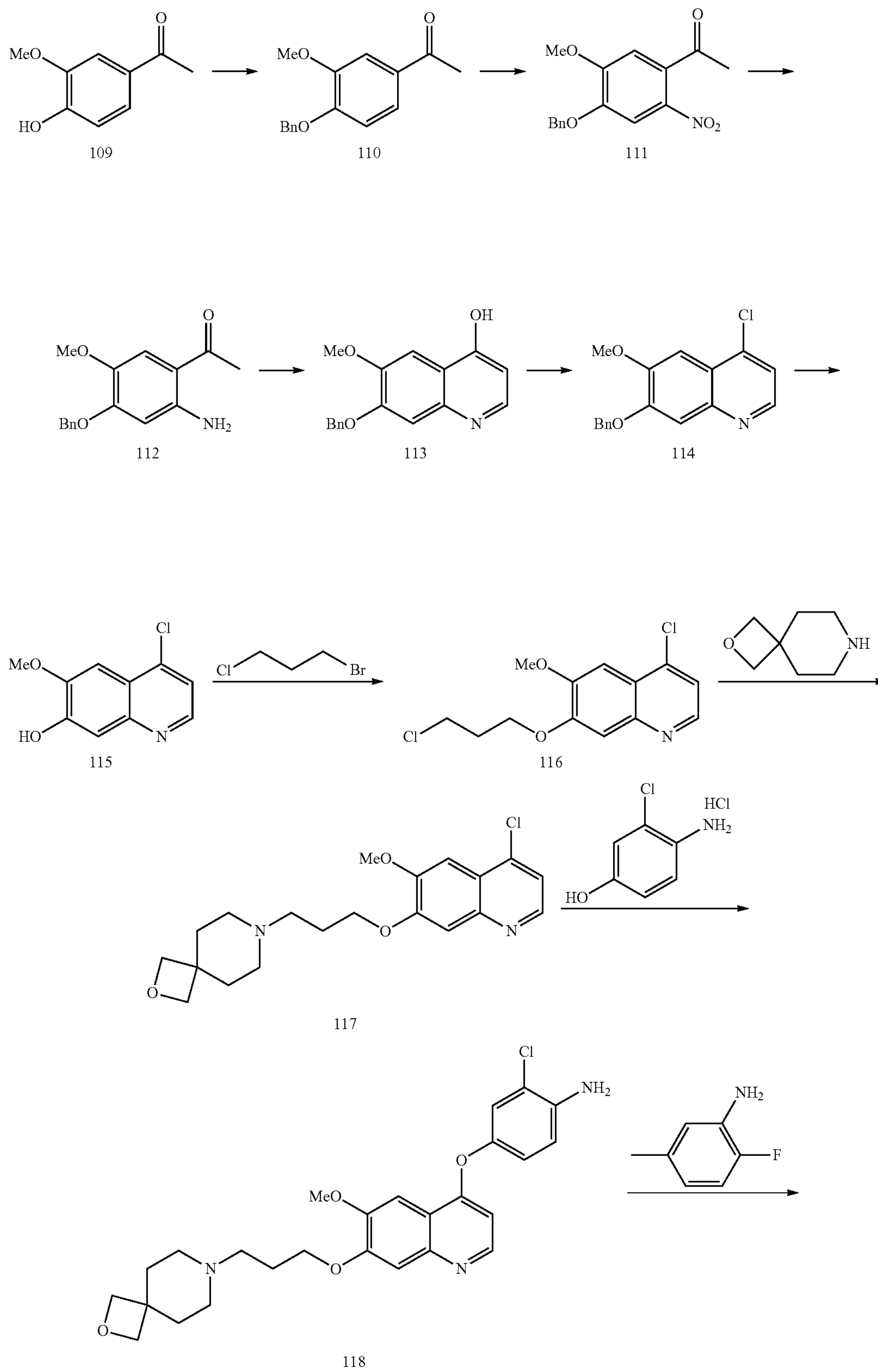
Scheme 2
