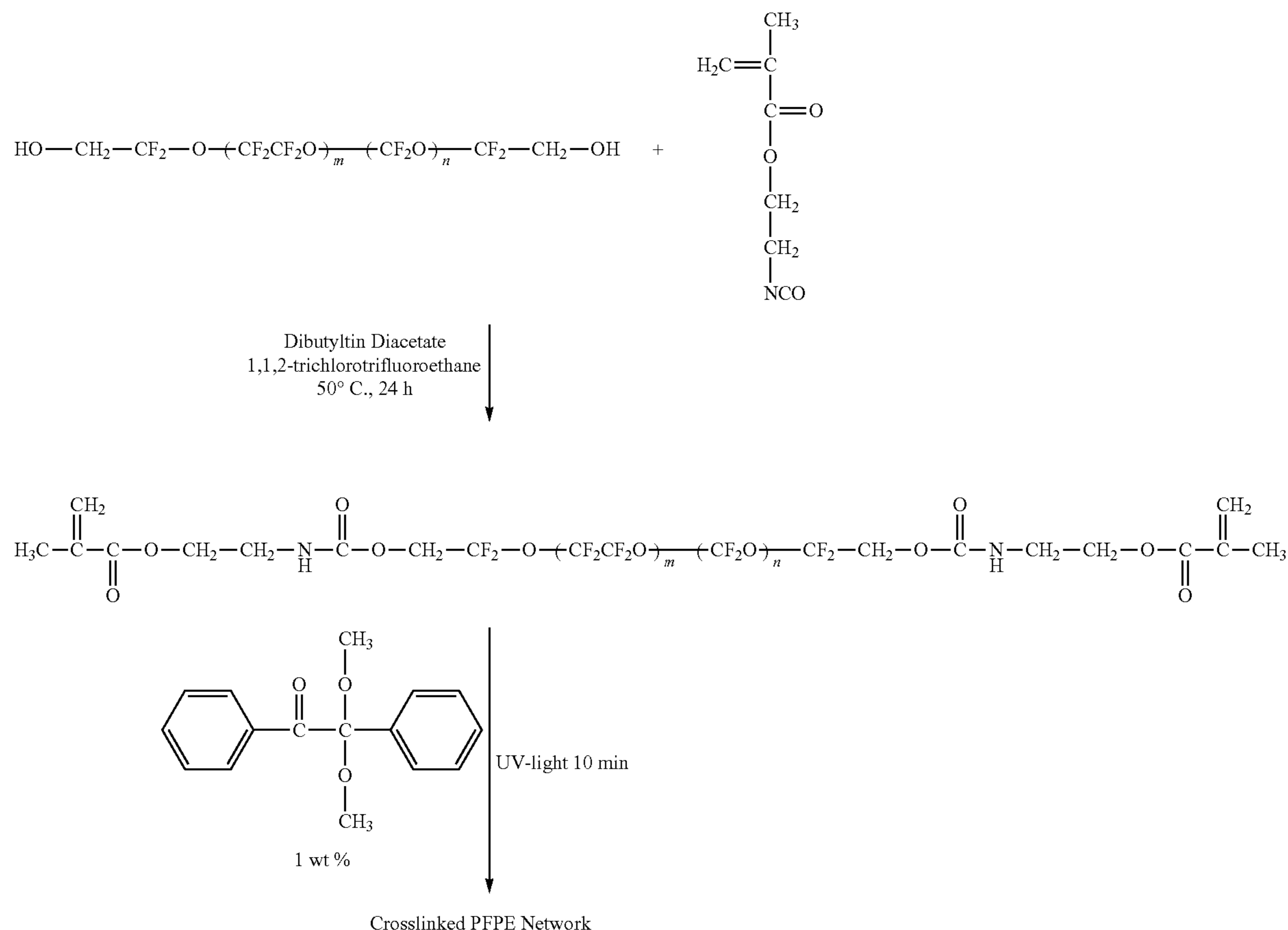
Scheme 1. Synthesis and Photocuring of Functional Perfluoropolyethers.
