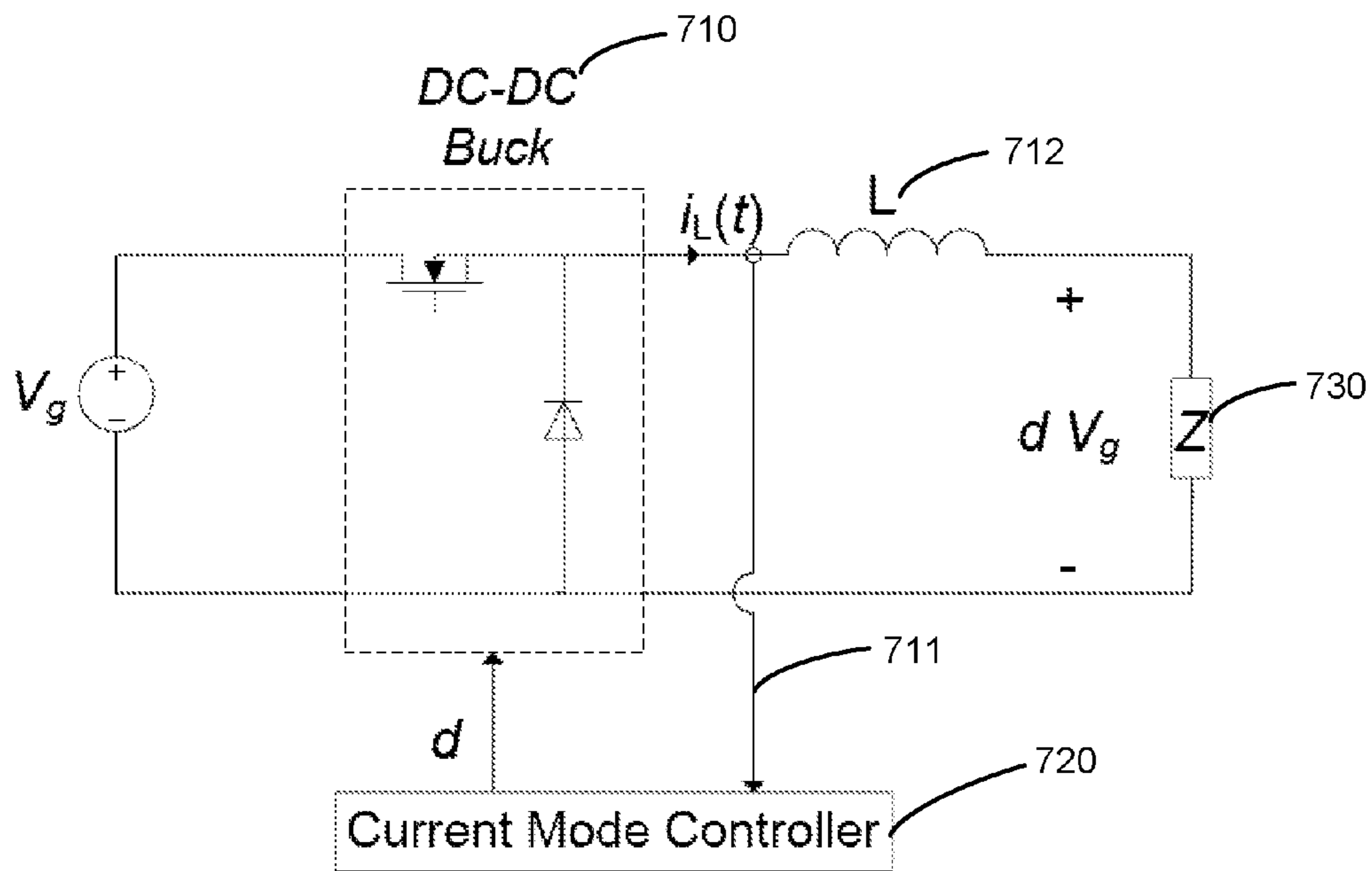
CPM-controlled buck converter
