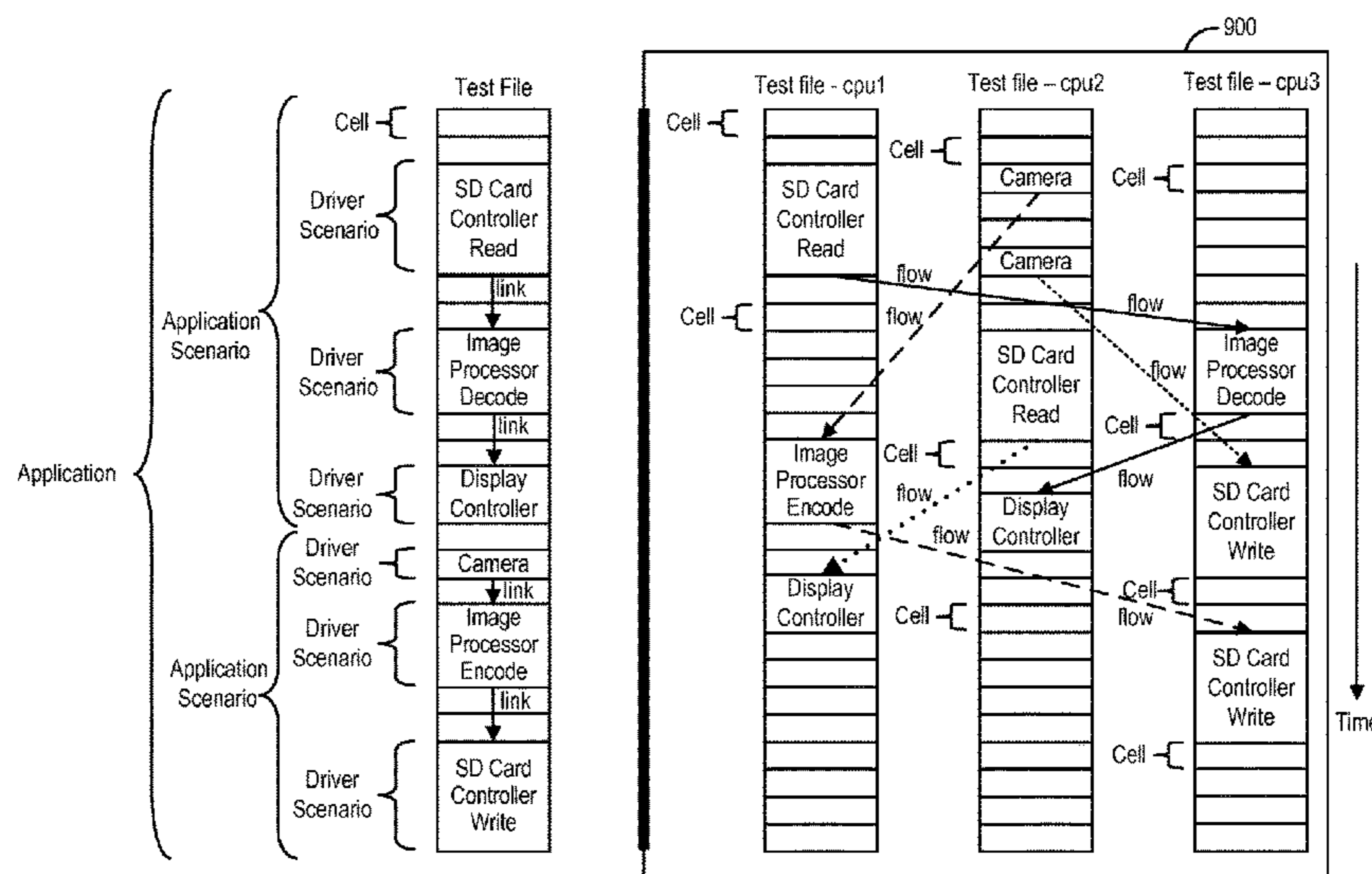
(Generated Test Case Multi-processor Flow)
