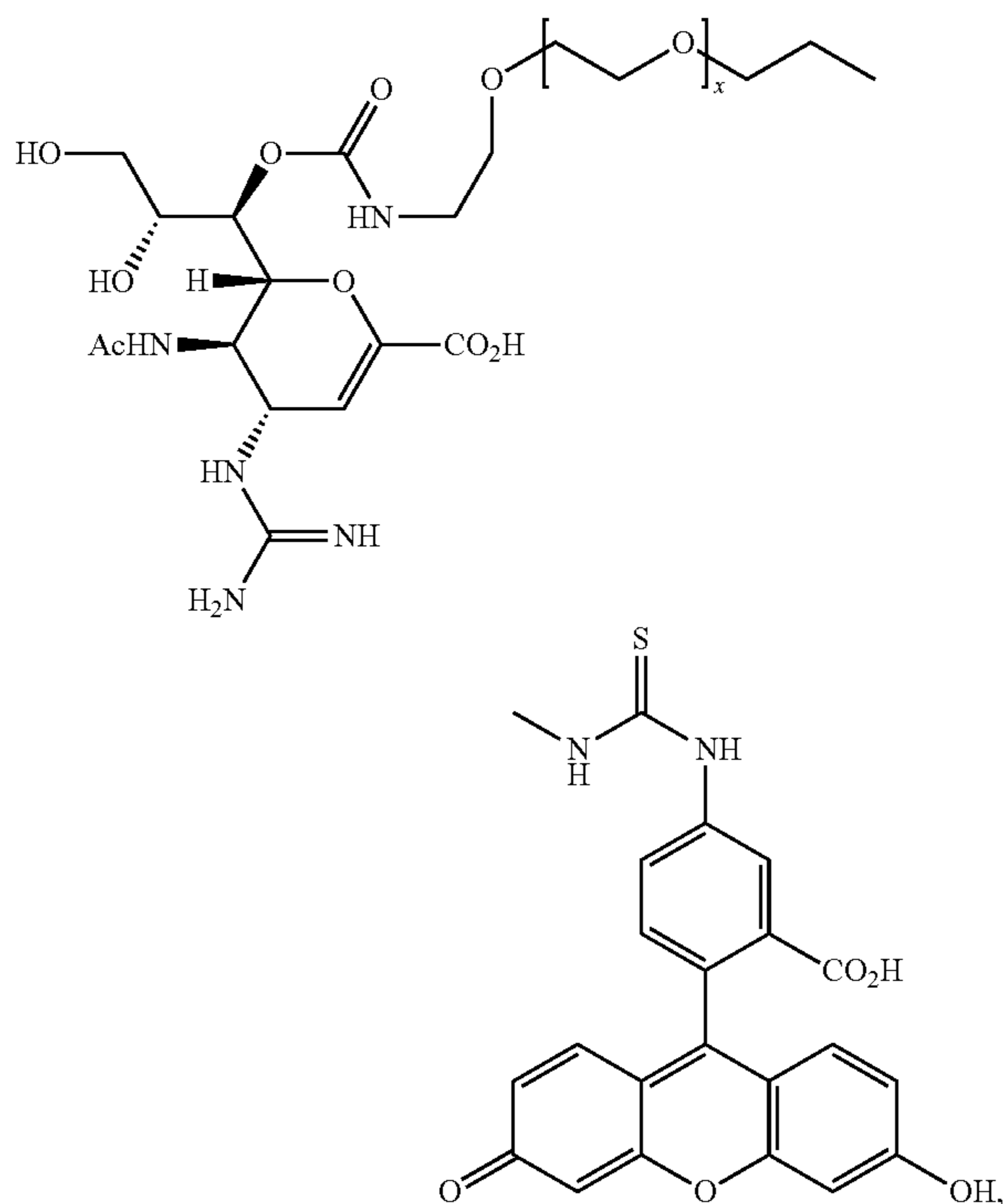
BM 6: (Tamiphosphor Guanidine)-(Ethylene Glycol Linker)-Fluorescein
