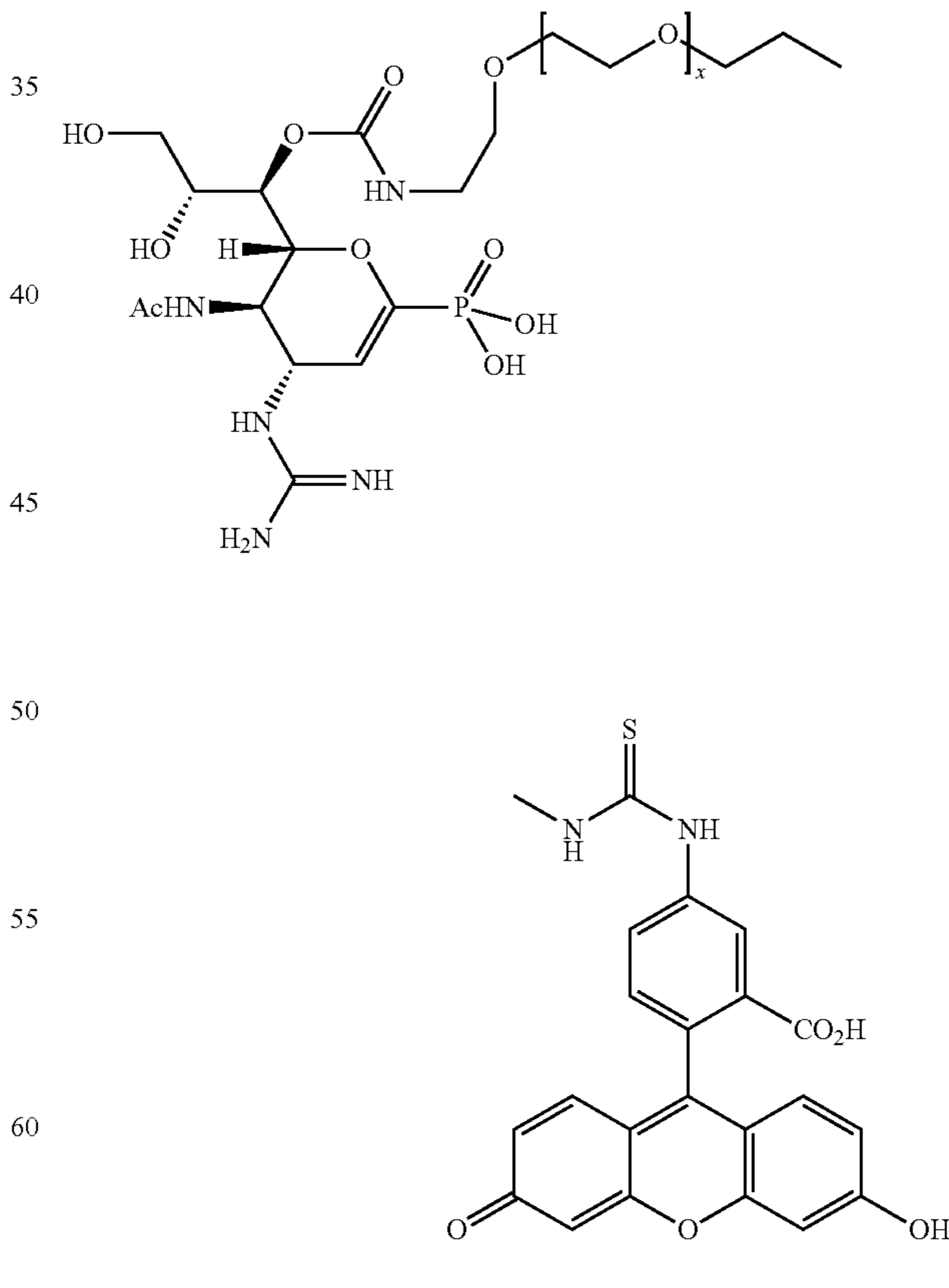
BM 10: (PhosphaZanamivir Monoester)-(Ethylene Glycol Linker)-Fluorescein
