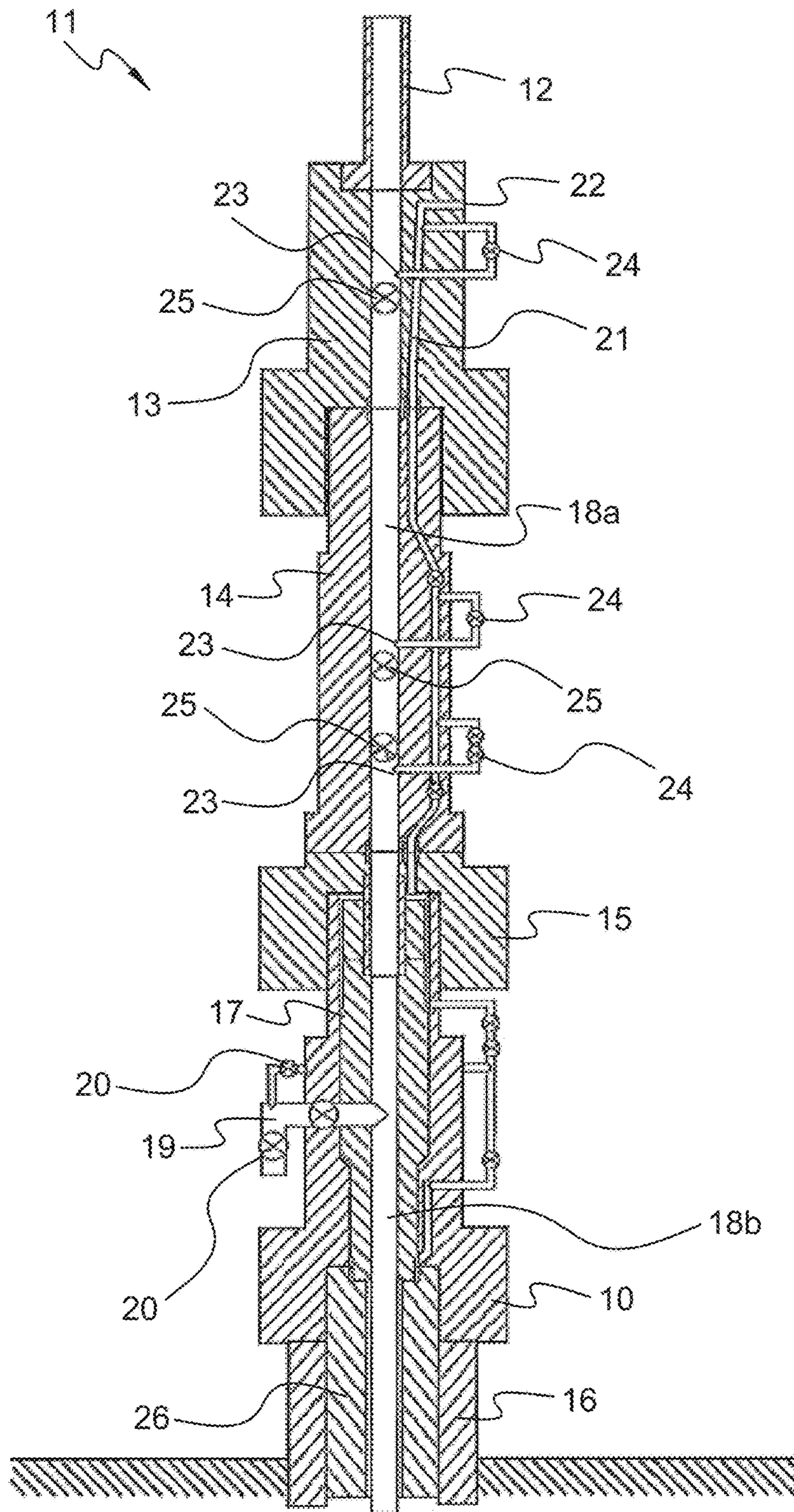
Fig. 2 (Prior Art)
