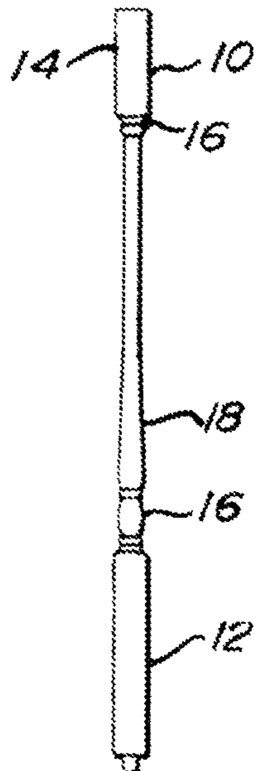
Fig. 1F (PRIOR ART)
