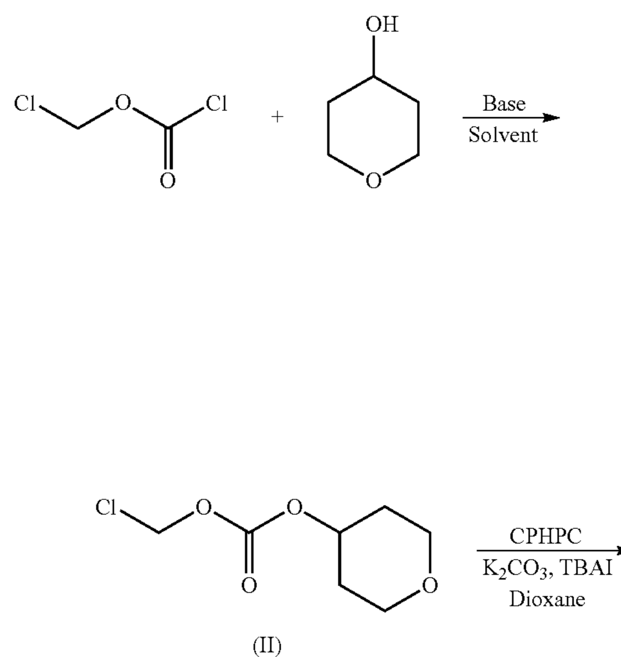
Reaction Scheme 1
