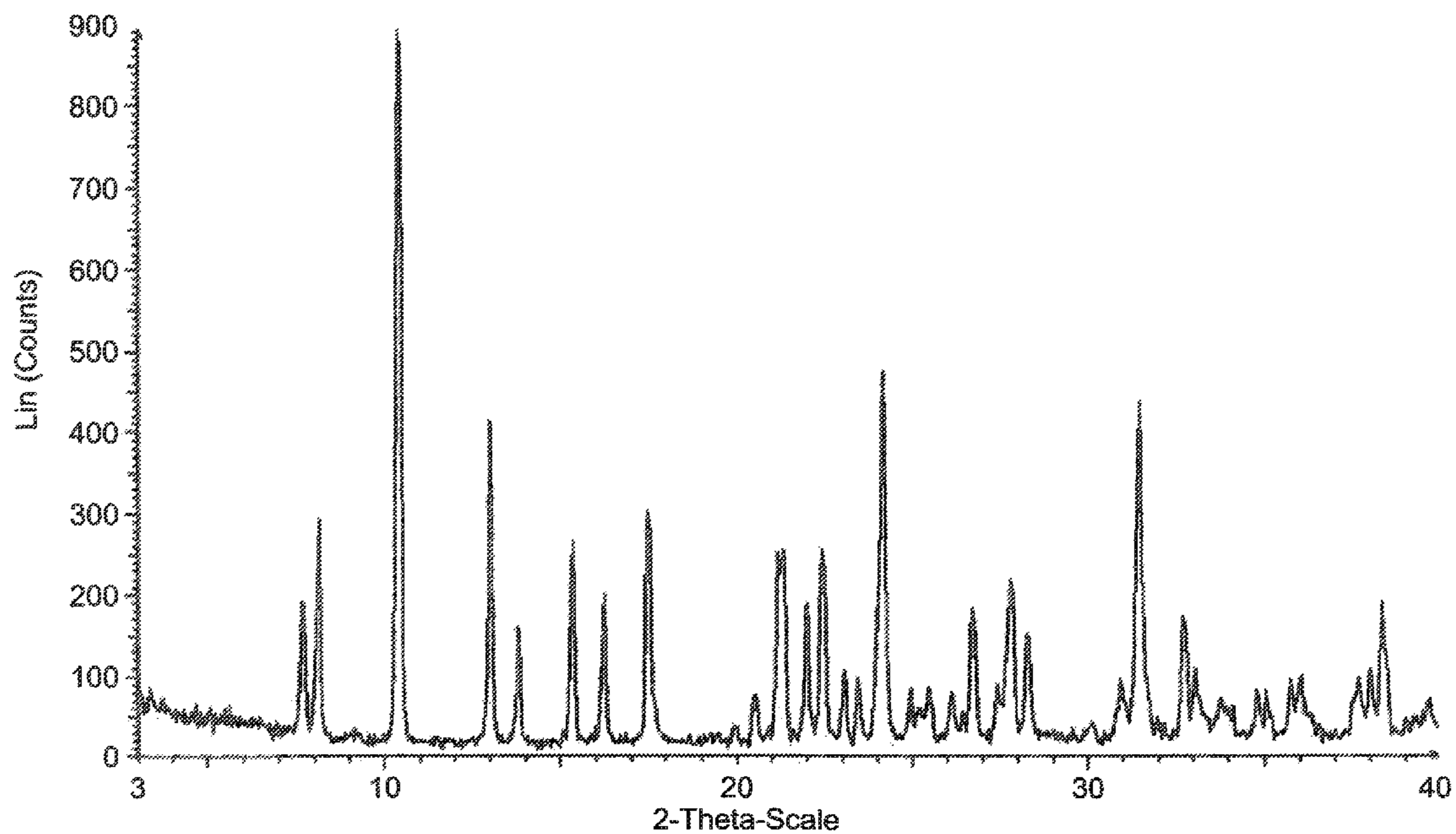
X-Ray Powder Diffraction Pattern For Example 2
