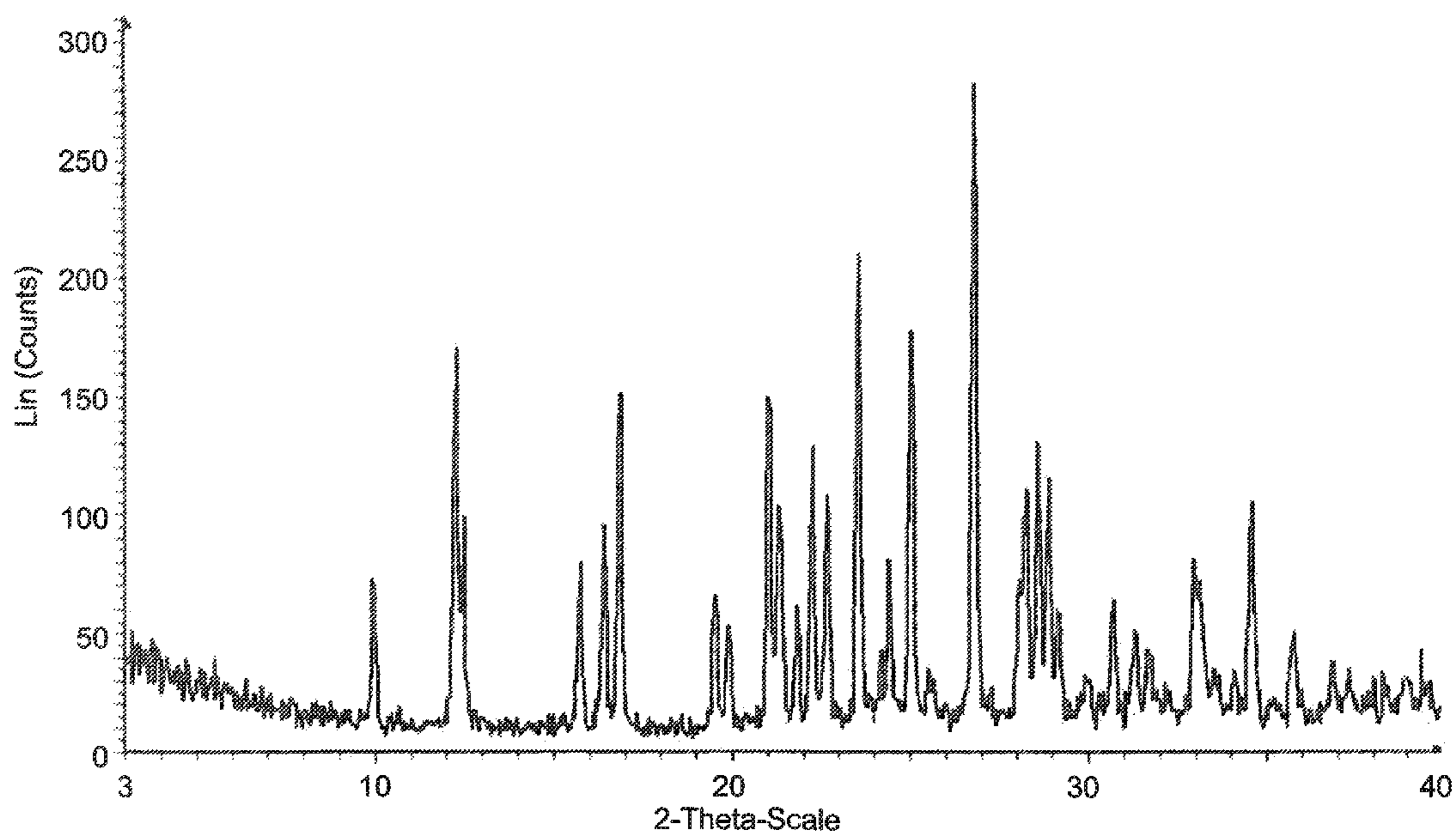
X-Ray Powder Diffraction Pattern For Example 1
