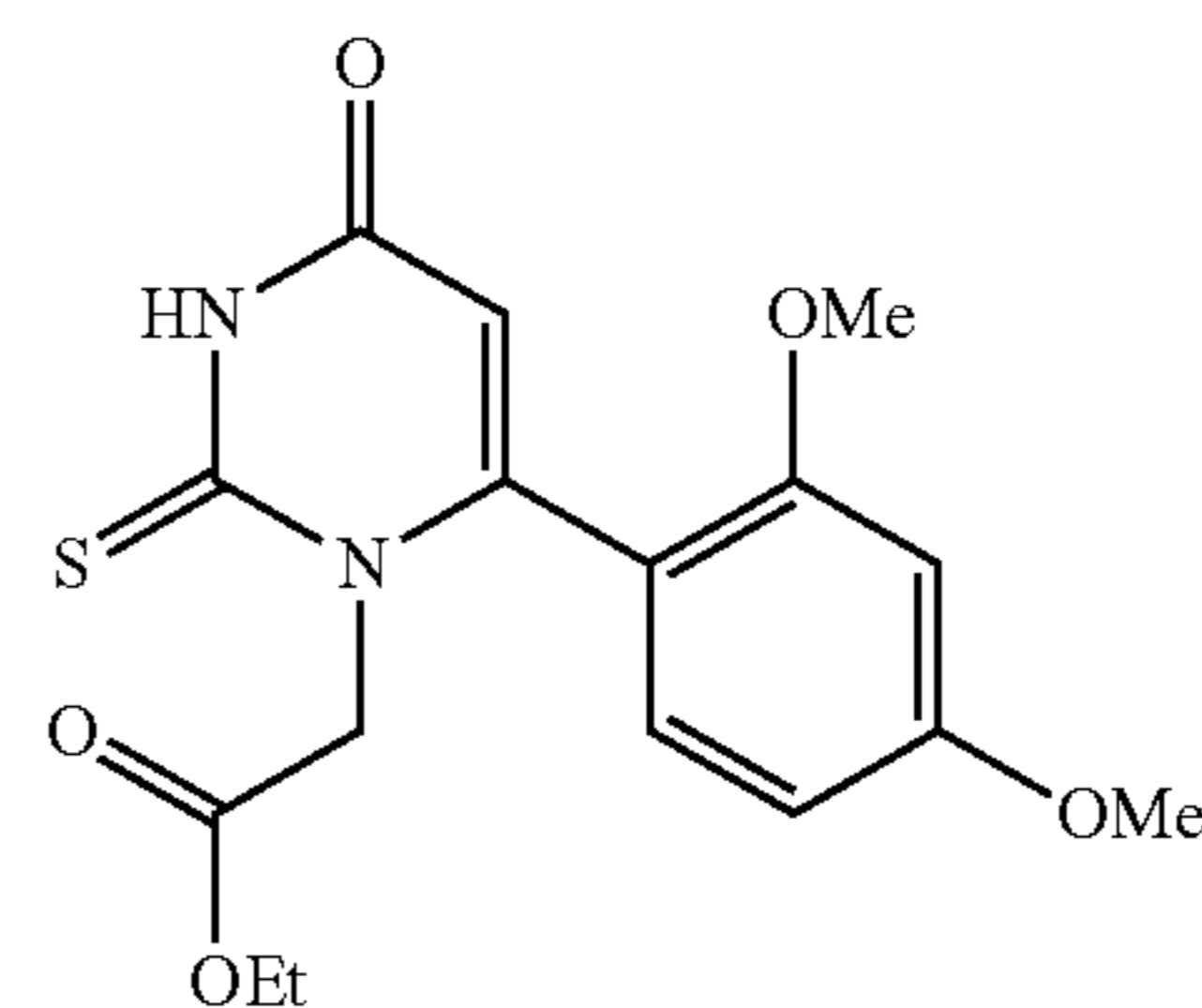
Ethyl 2-(6-(2,4-dimethoxyphenyl)-4-oxo-2-thioxo-3,4-dihydropyrimidin-1(2H)-yl)acetate
