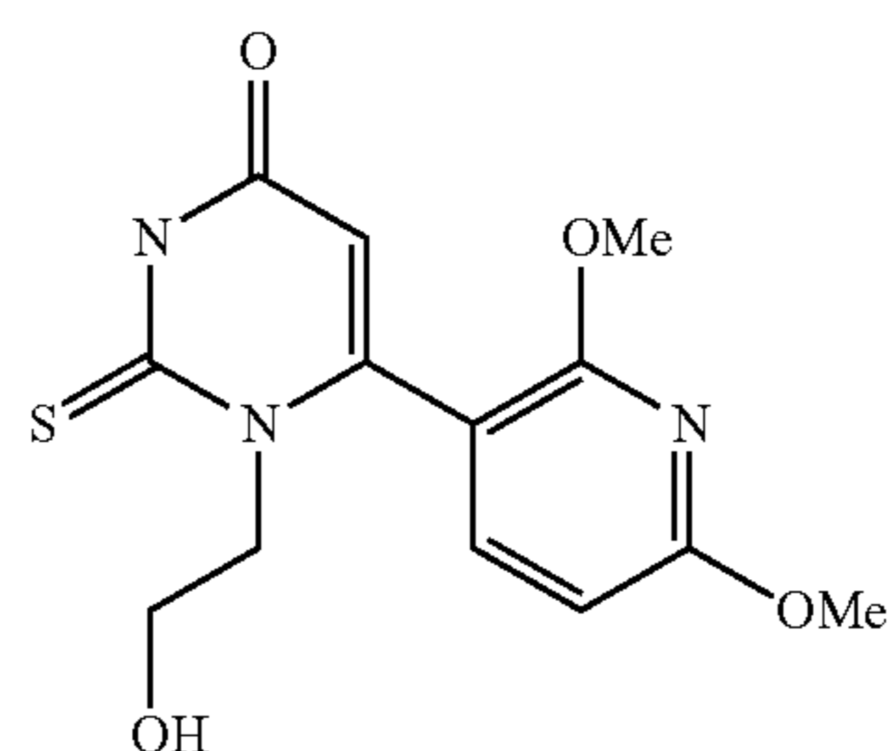
6-(2,6-Dimethoxy-pyridin-3-yl)-1-(2-hydroxyethyl)-2-thioxo-2,3-dihydropyrimidin-4(1H)-one
