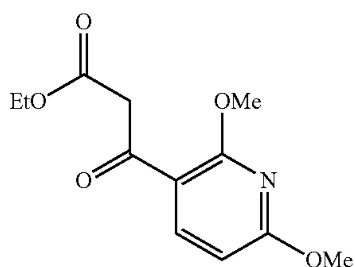
Ethyl 3-(2,6-dimethoxy-pyridin-3-yl)-3-oxopropanoate
