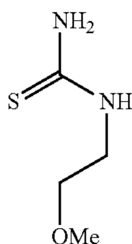
1-(2-Methoxyethyl)thiourea
