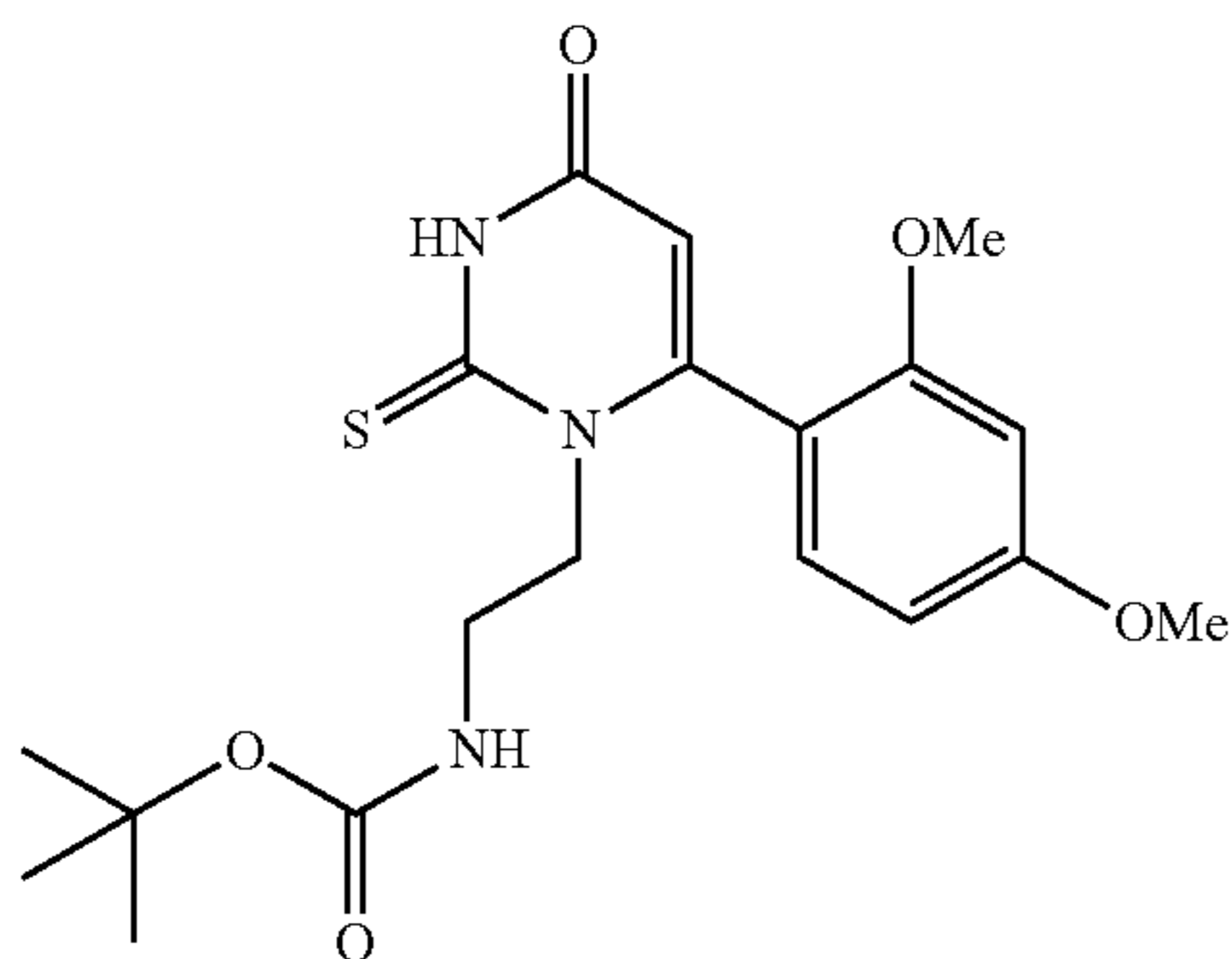
tert-butyl 2-(6-(2,4-dimethoxyphenyl)-4-oxo-2-thioxo-3,4-dihydropyrimidin-1(2H)-yl)ethylcarbamate
