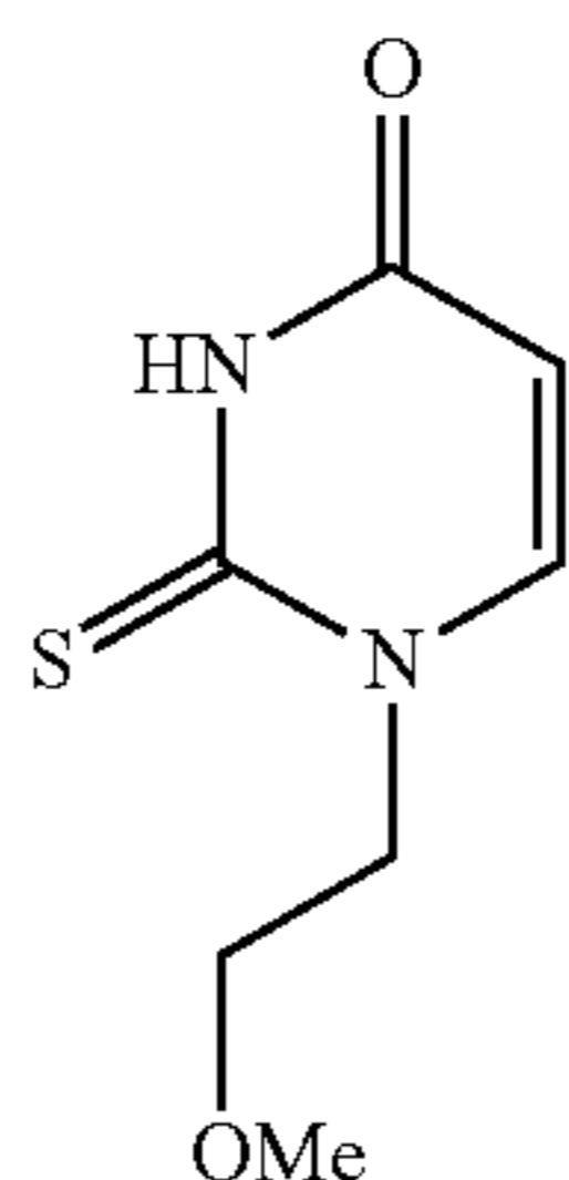
1-(2-Methoxyethyl)-2-thioxo-2,3-dihydropyrimidin-4(1H)-one
