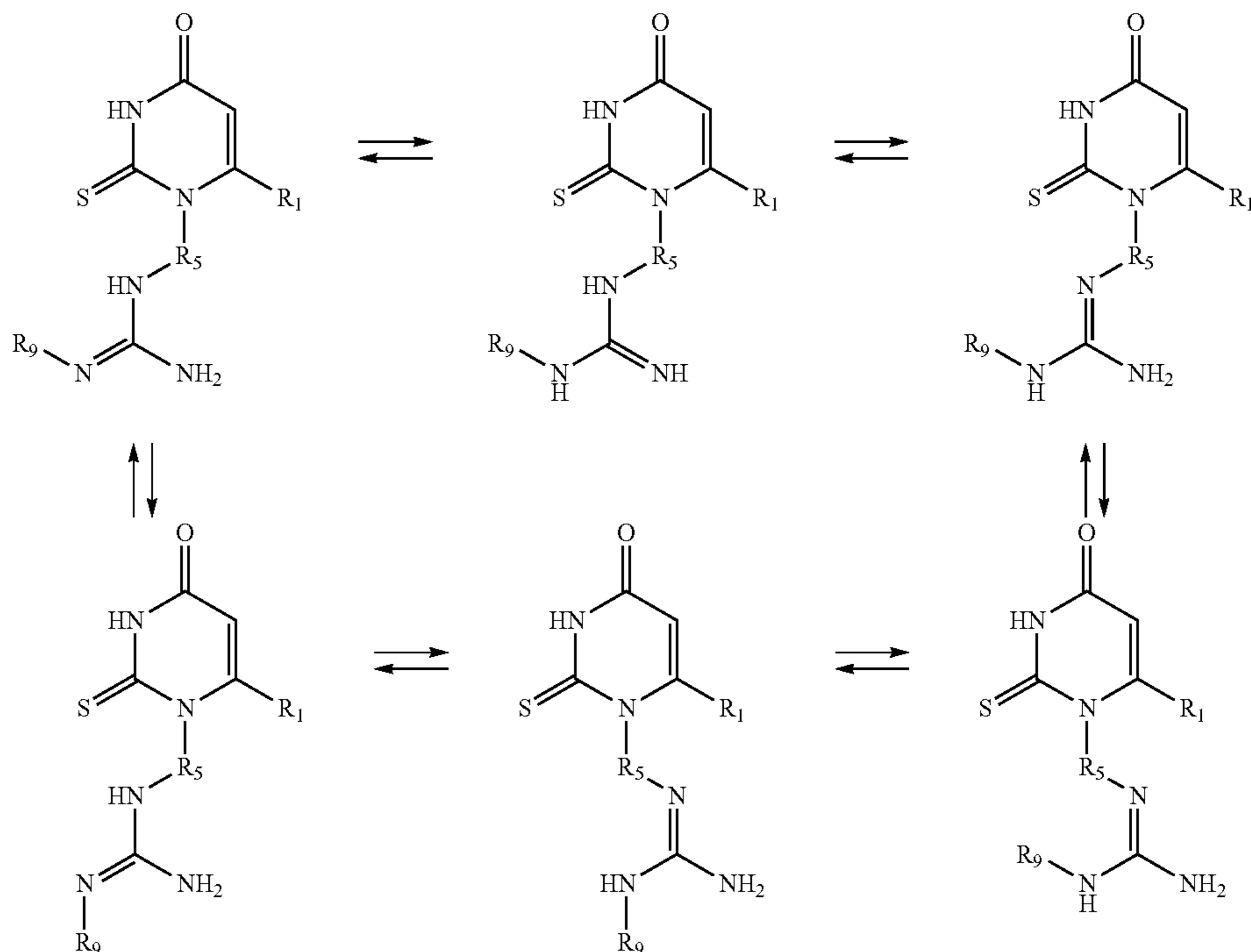
Example of Guanidine Tautomers and Geometric Isomers
