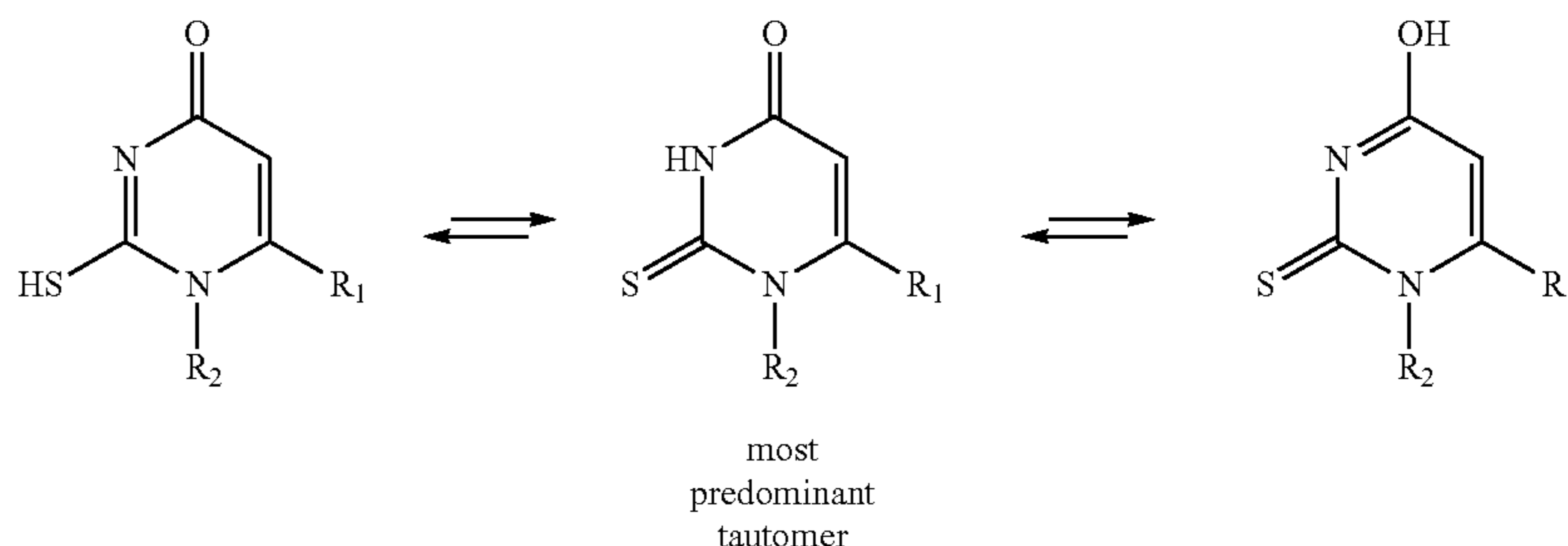
Thiouracil Tautomers
