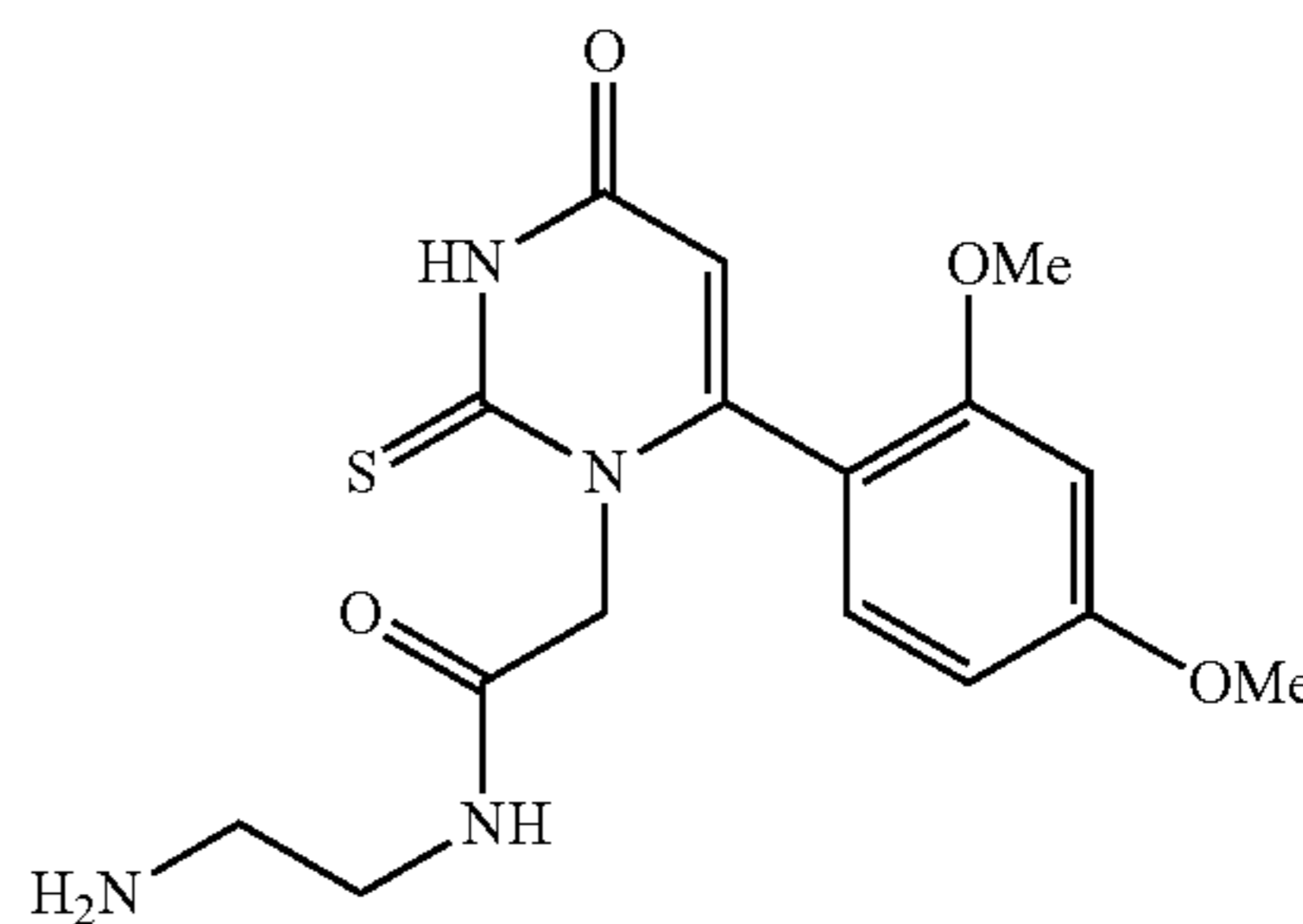
N-(2-aminoethyl)-2-(6-(2,4-dimethoxyphenyl)-4-oxo-2-thioxo-3,4-dihydropyrimidin-1(2H)-yl)acetamide hydrochloride
