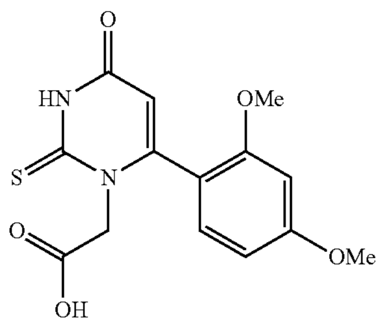
2-(6-(2,4-dimethoxyphenyl)-4-oxo-2-thioxo-3,4-dihydropyrimidin-1(2H)-yl)acetic acid
