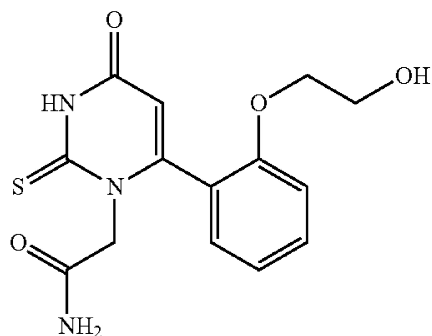
2-(6-(2-(2-Hydroxyethoxy)phenyl)-4-oxo-2-thioxo-3,4-dihydropyrimidin-1(2H)-acetamide
