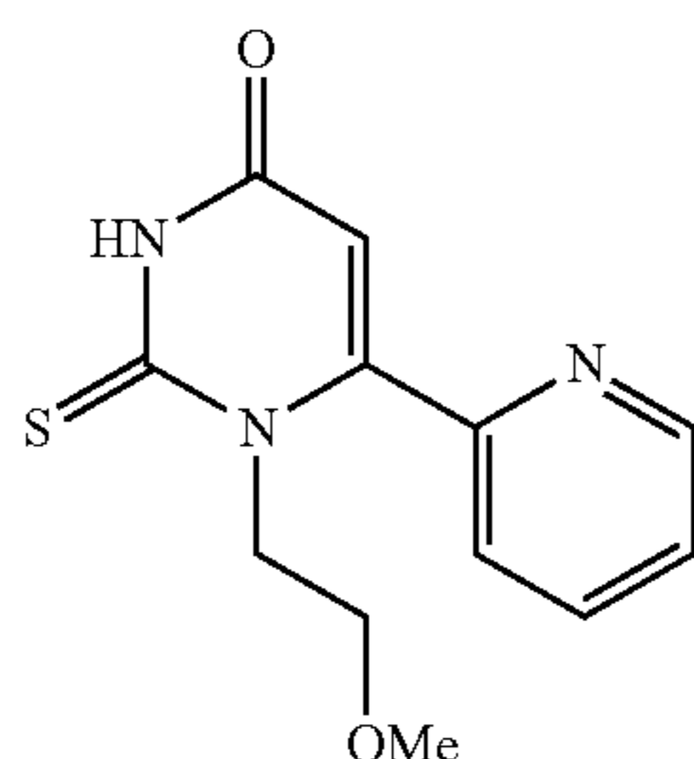
1-(2-Methoxyethyl)-6-(pyridin-2-yl)-2-thioxo-2,3-dihydropyrimidin-4(1H)-one
