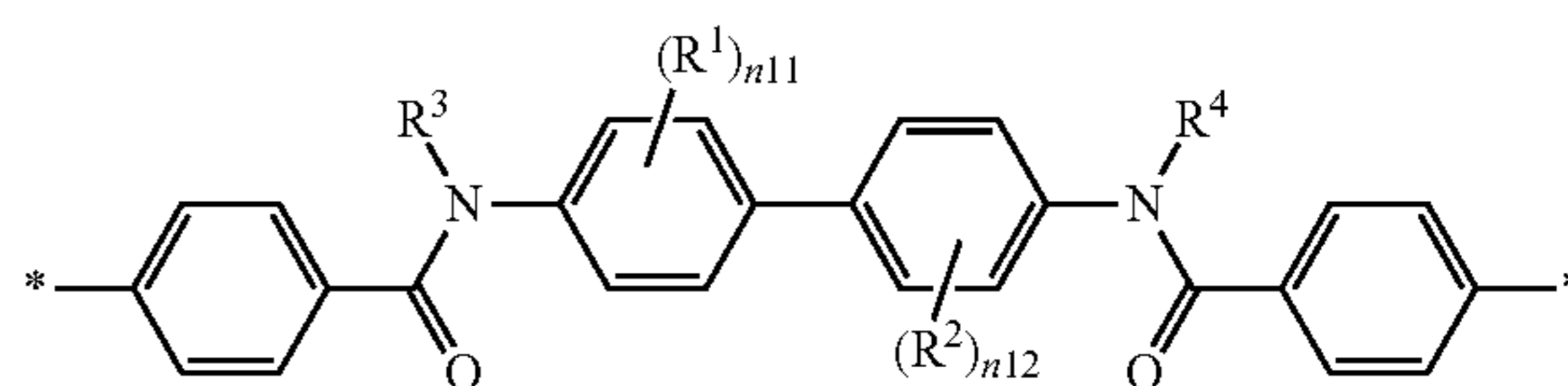
Chemical Formula 9
