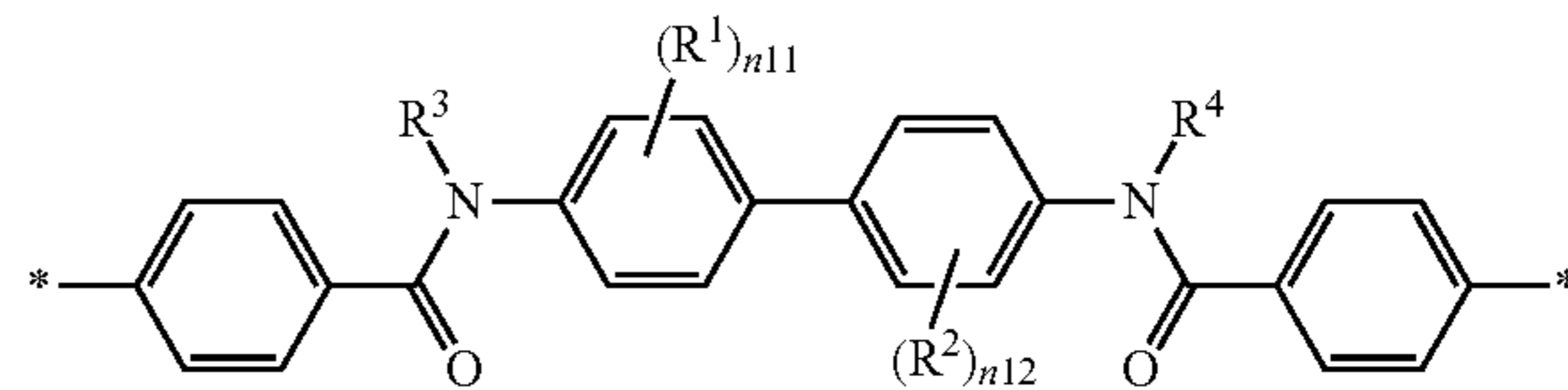
Chemical Formula 9
