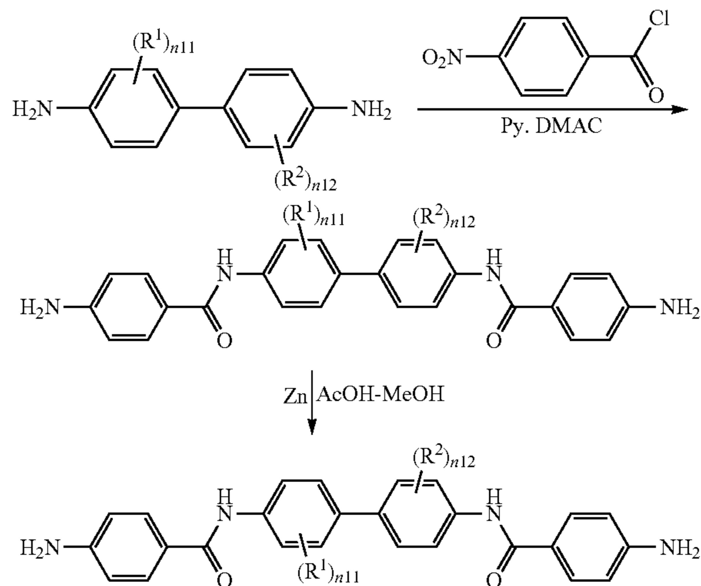
Reaction Scheme 1
