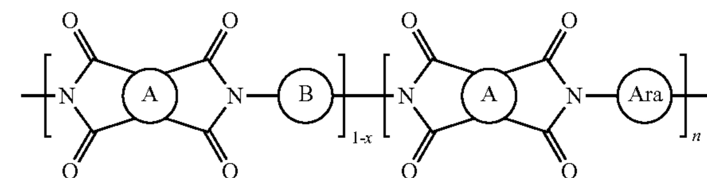
Chemical Formula 8
