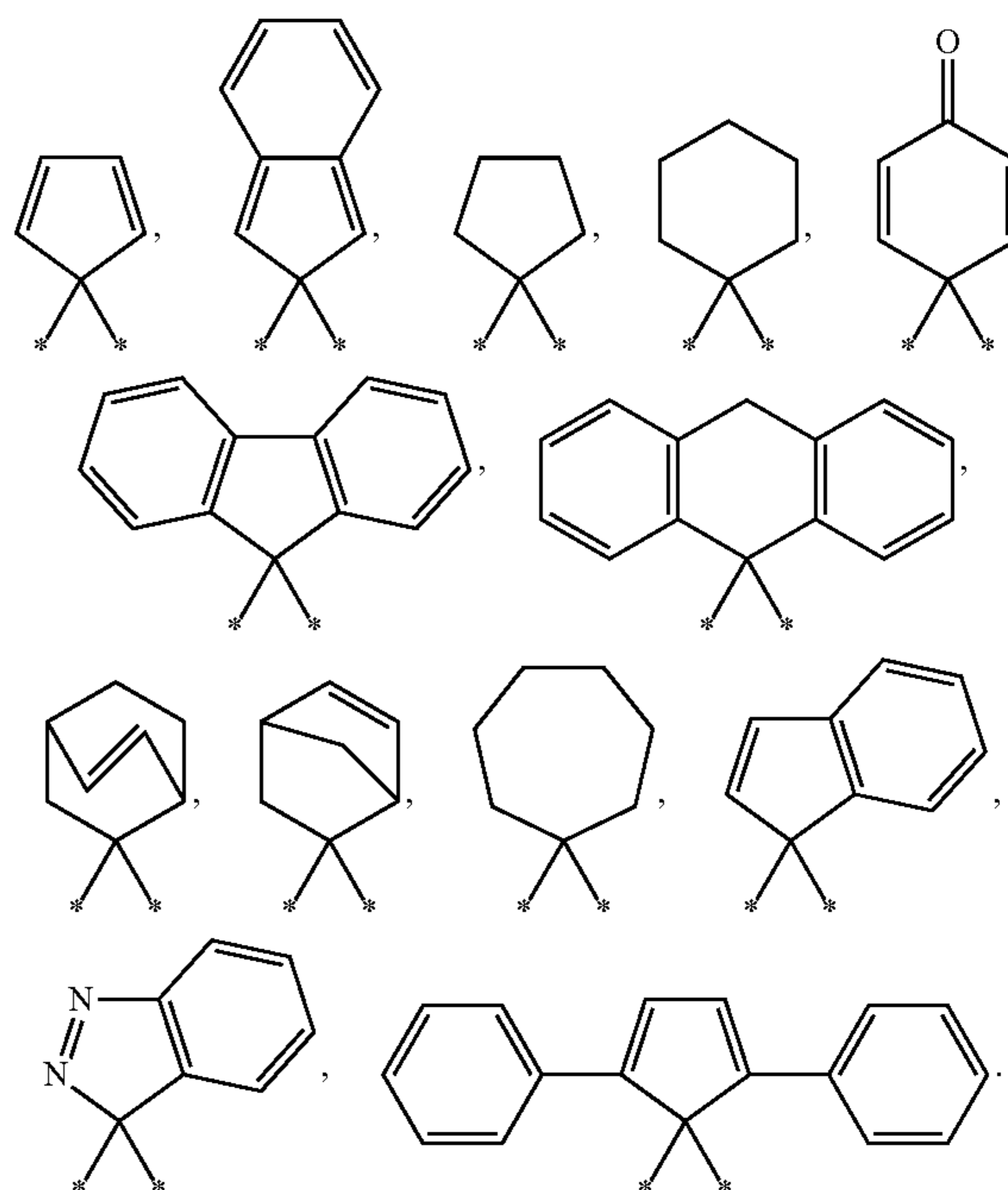
Chemical Formula 3
