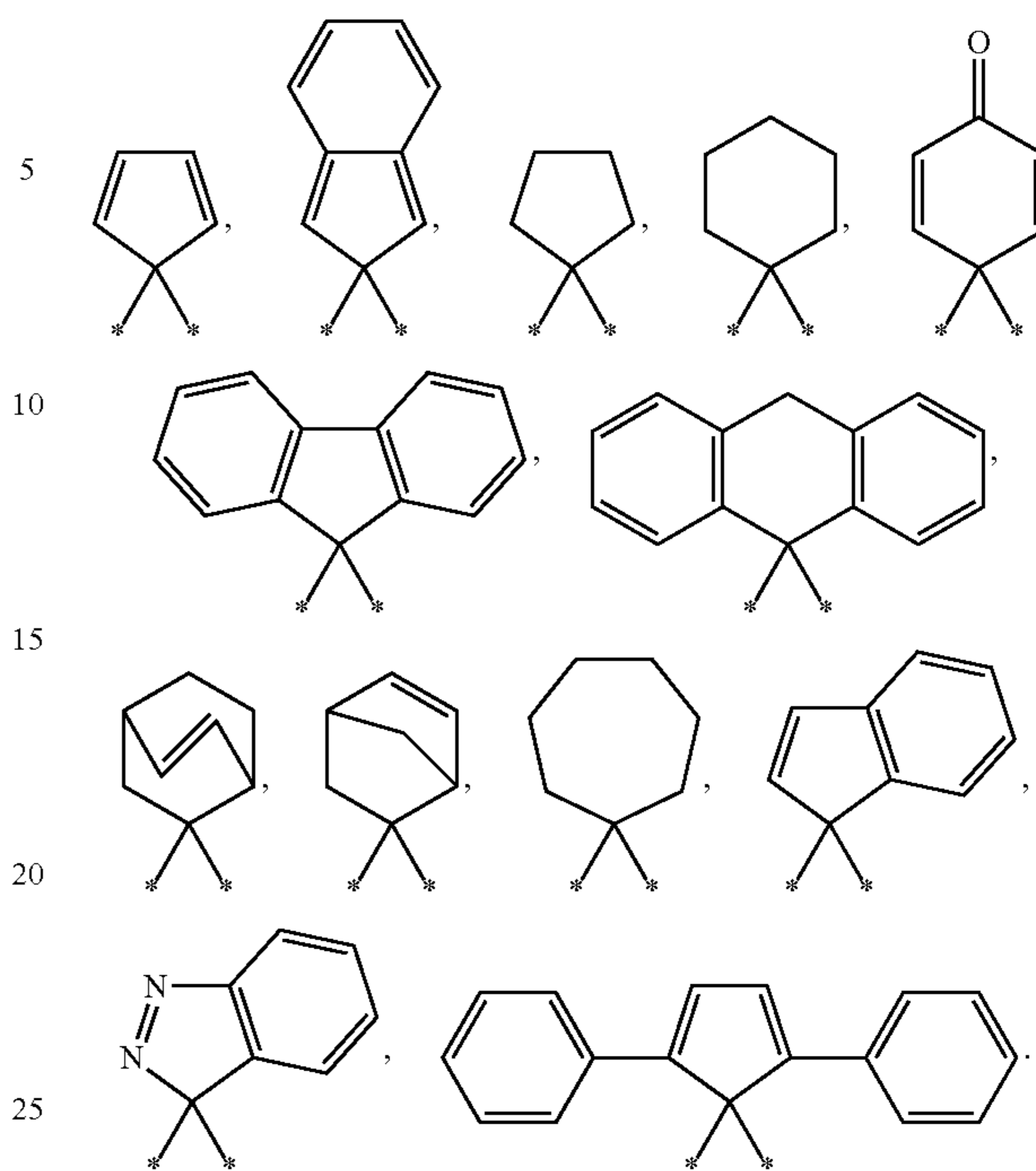
Chemical Formula 6-1
