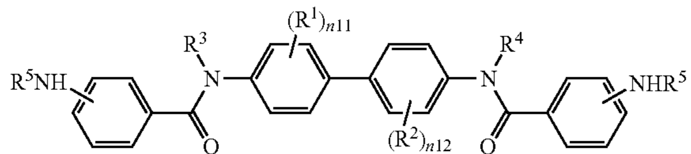
Chemical Formula 1
