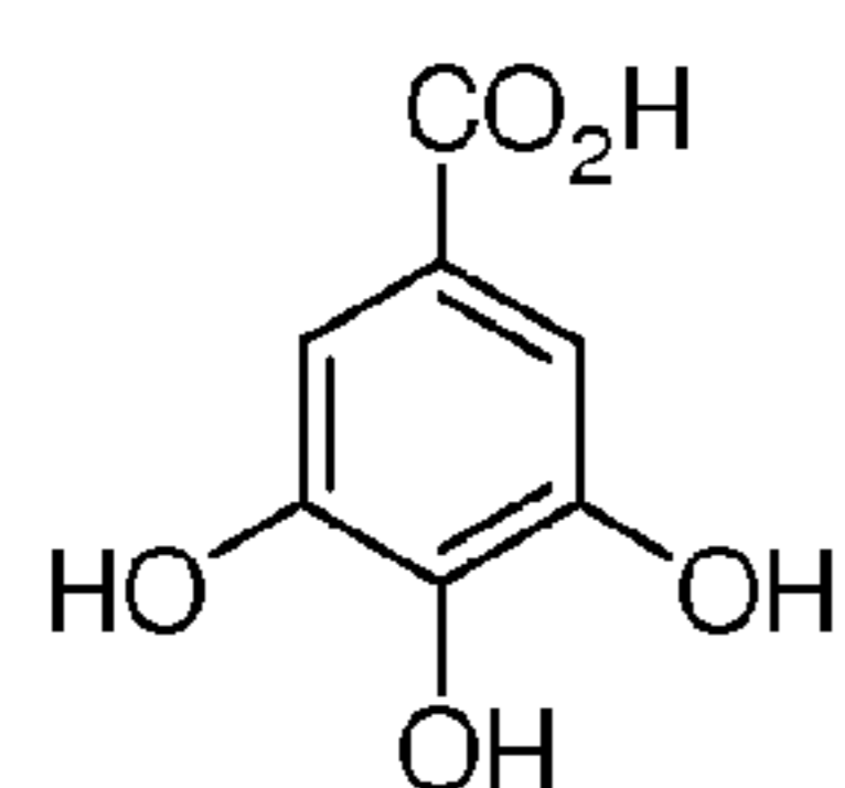
gallic acid
