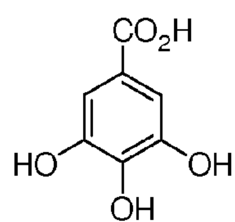
gallic acid
