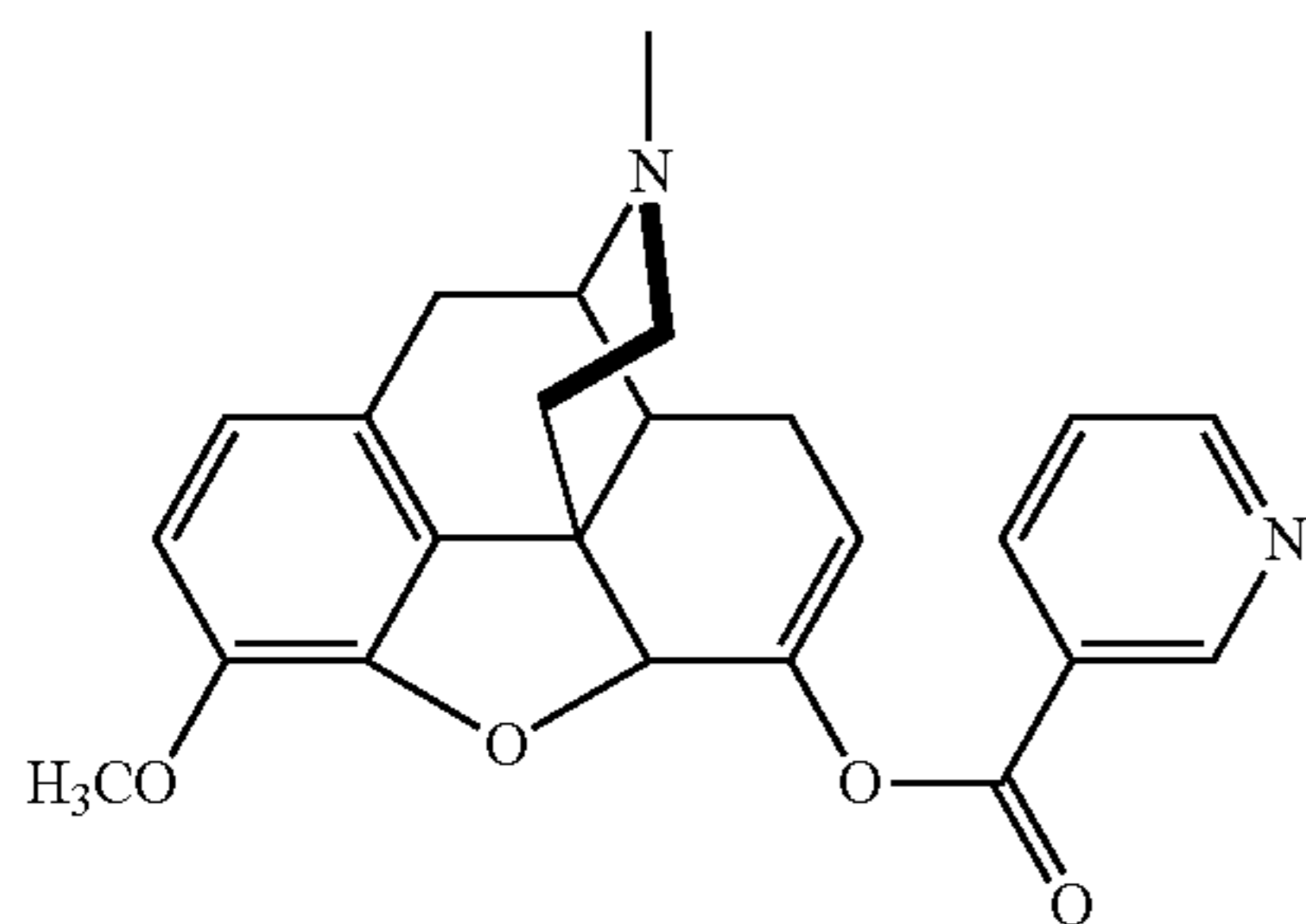
nicotinate-hydrocodone (Nicotinate-HC)
