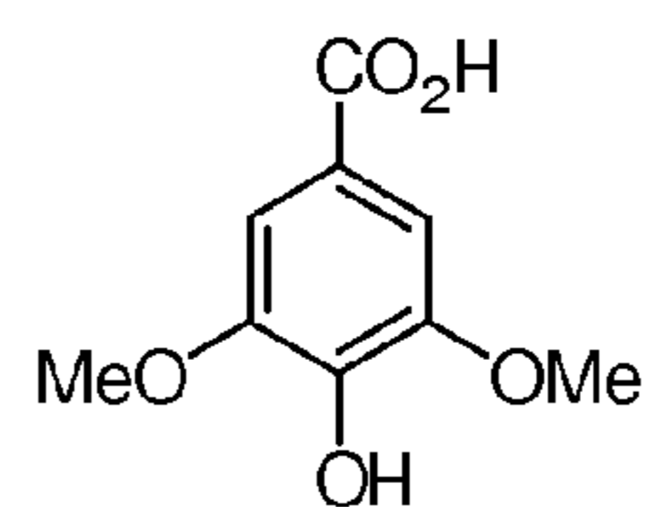
syringic acid
