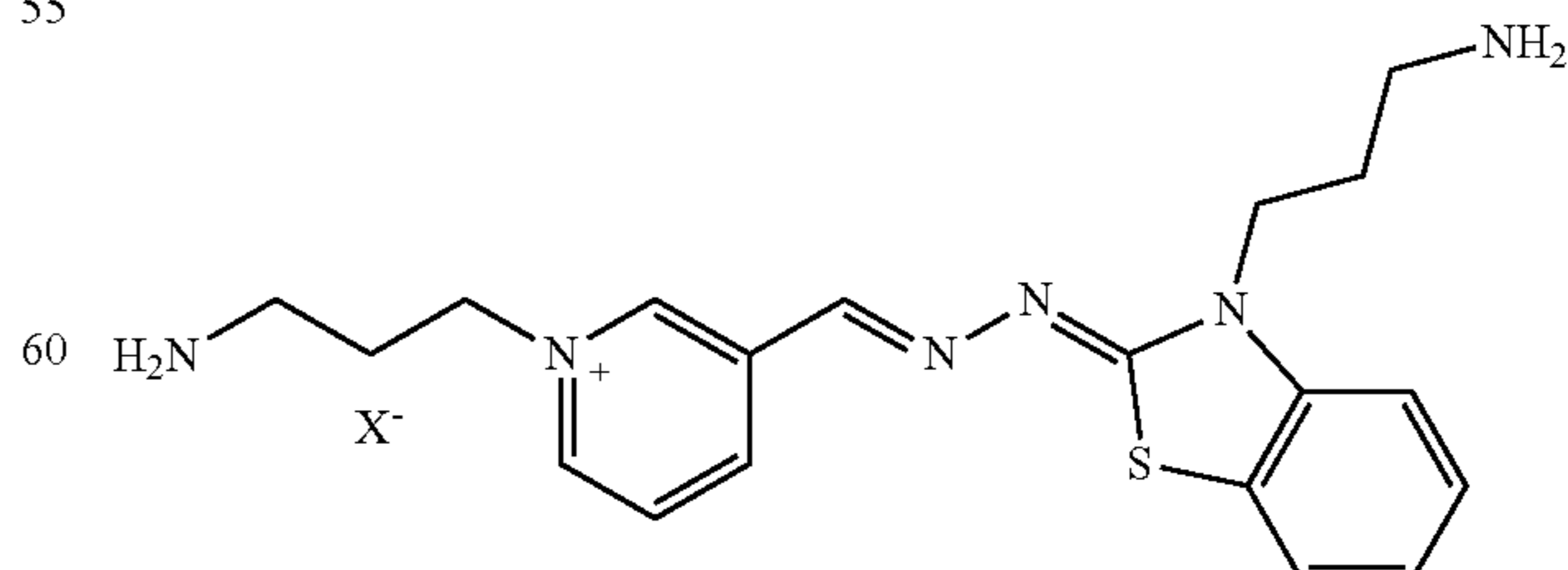
Formula XXIX
