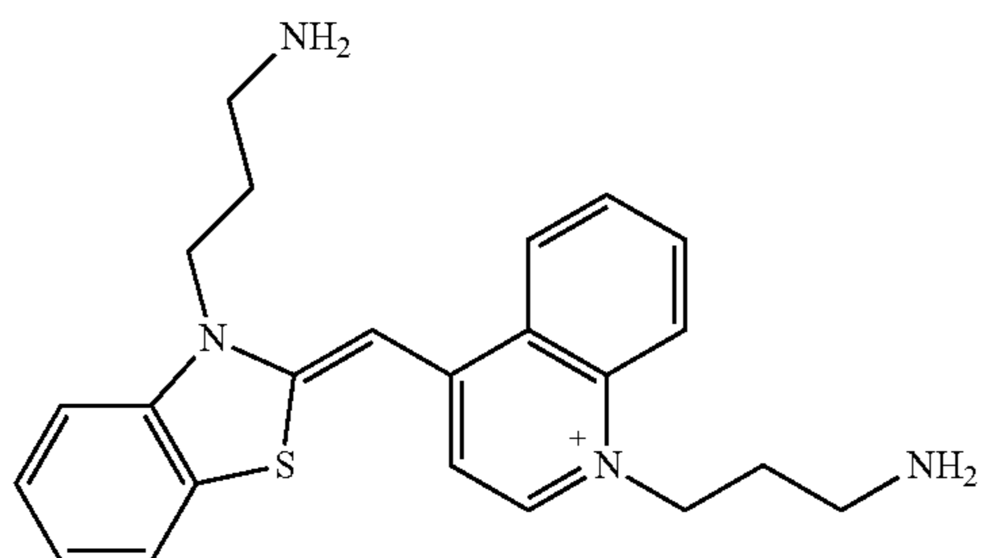
Formula XIII
