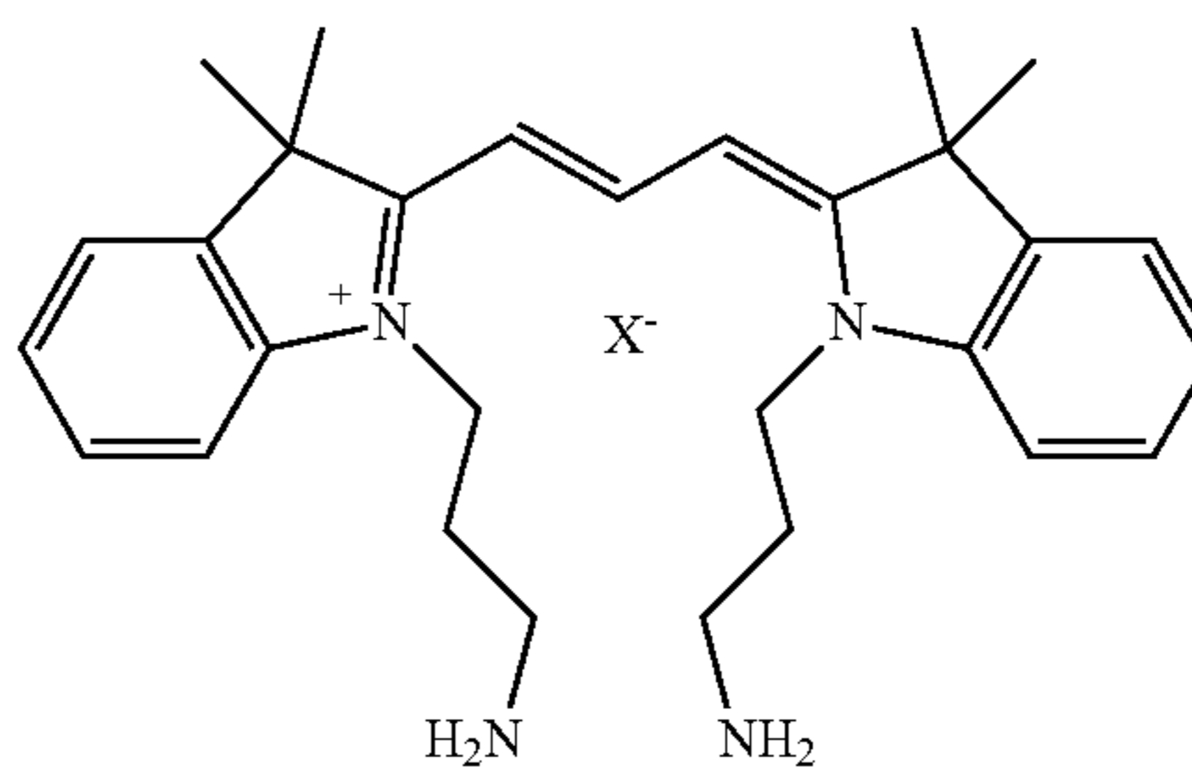
Formula XXVIII
