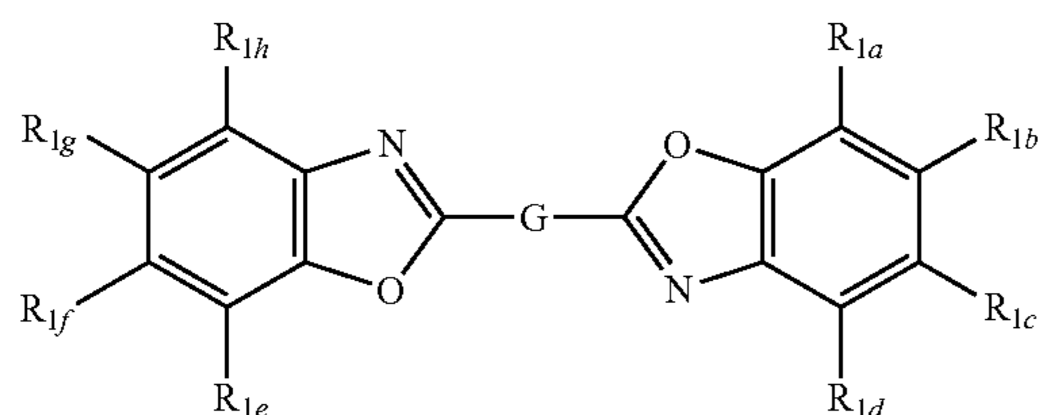
(XXVIa)
