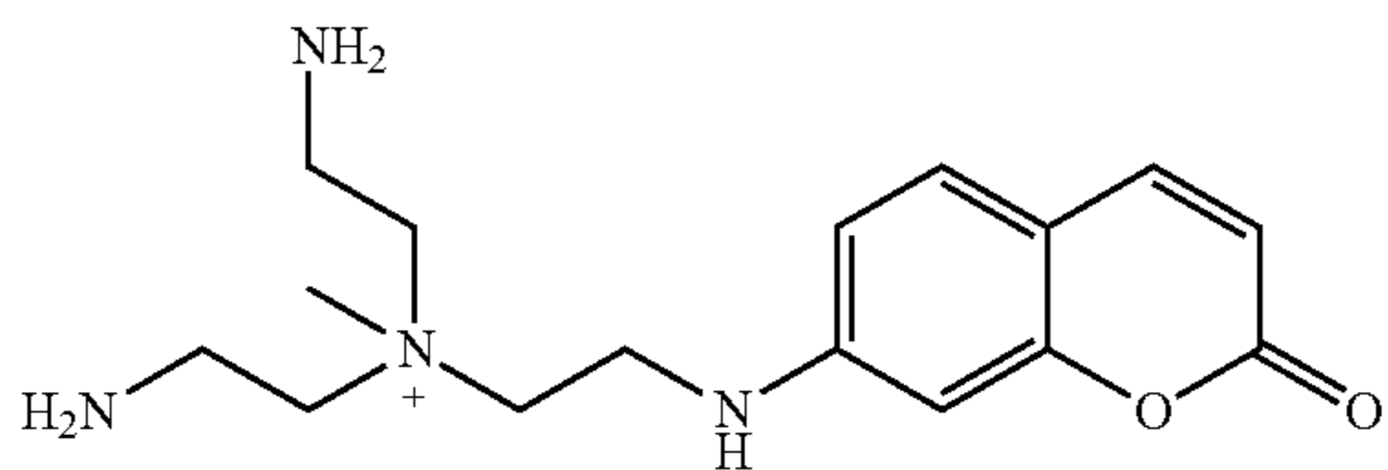
Formula V
