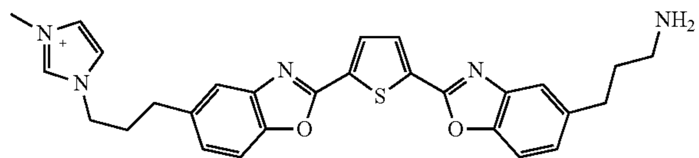
Formula XI
