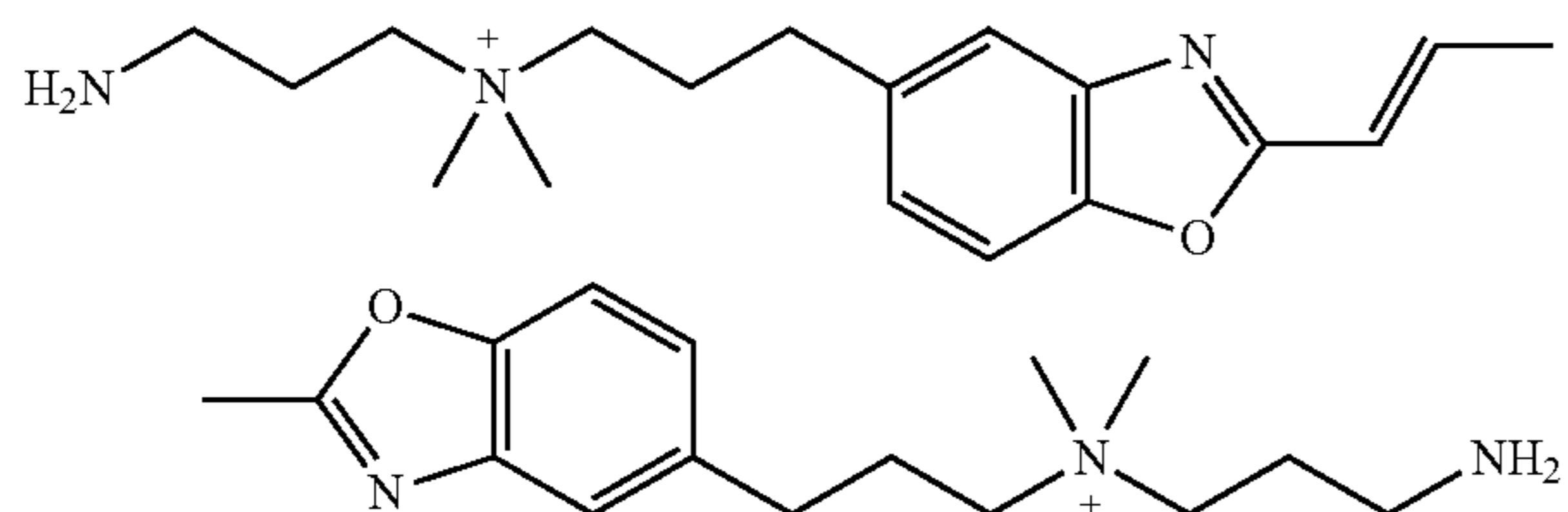
Formula VIII
