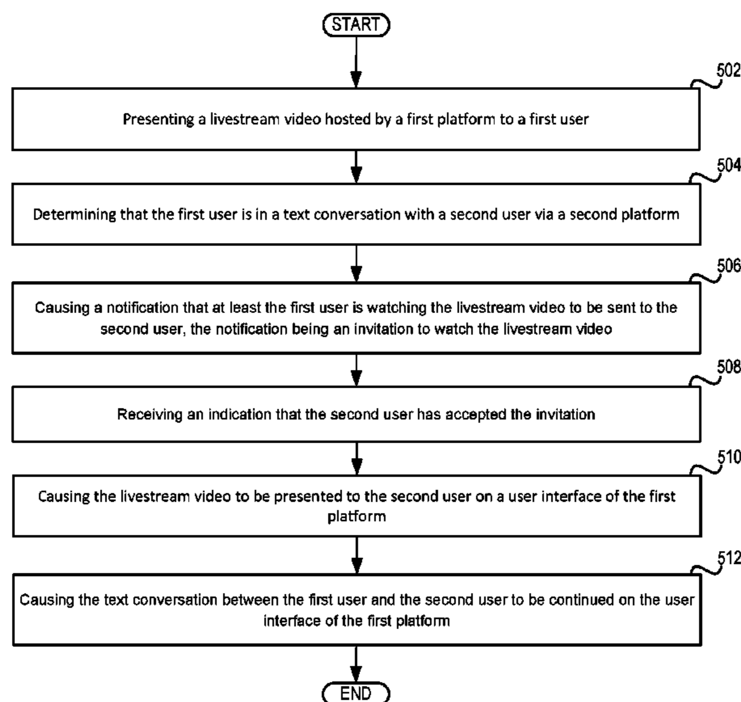
Method 500
