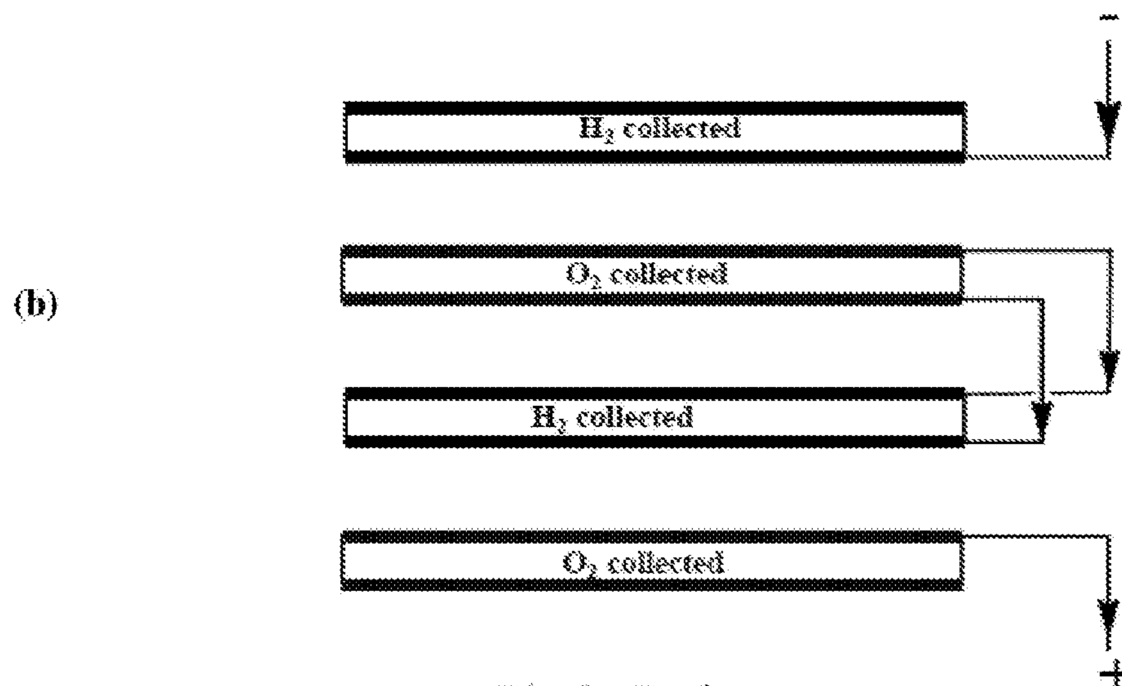
Bipolar Design (cells in series)
