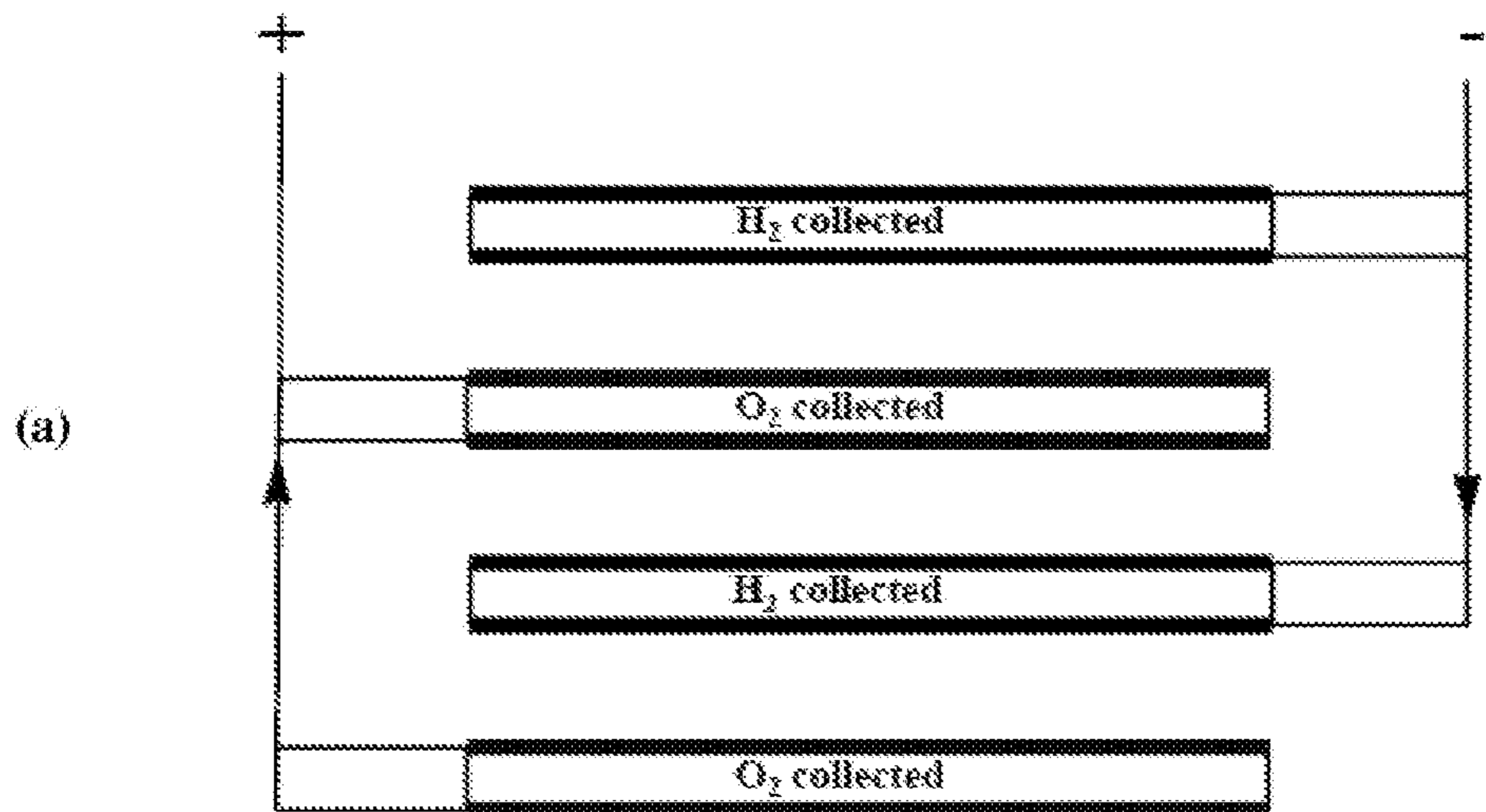
Unipolar Design (cells in parallel)
