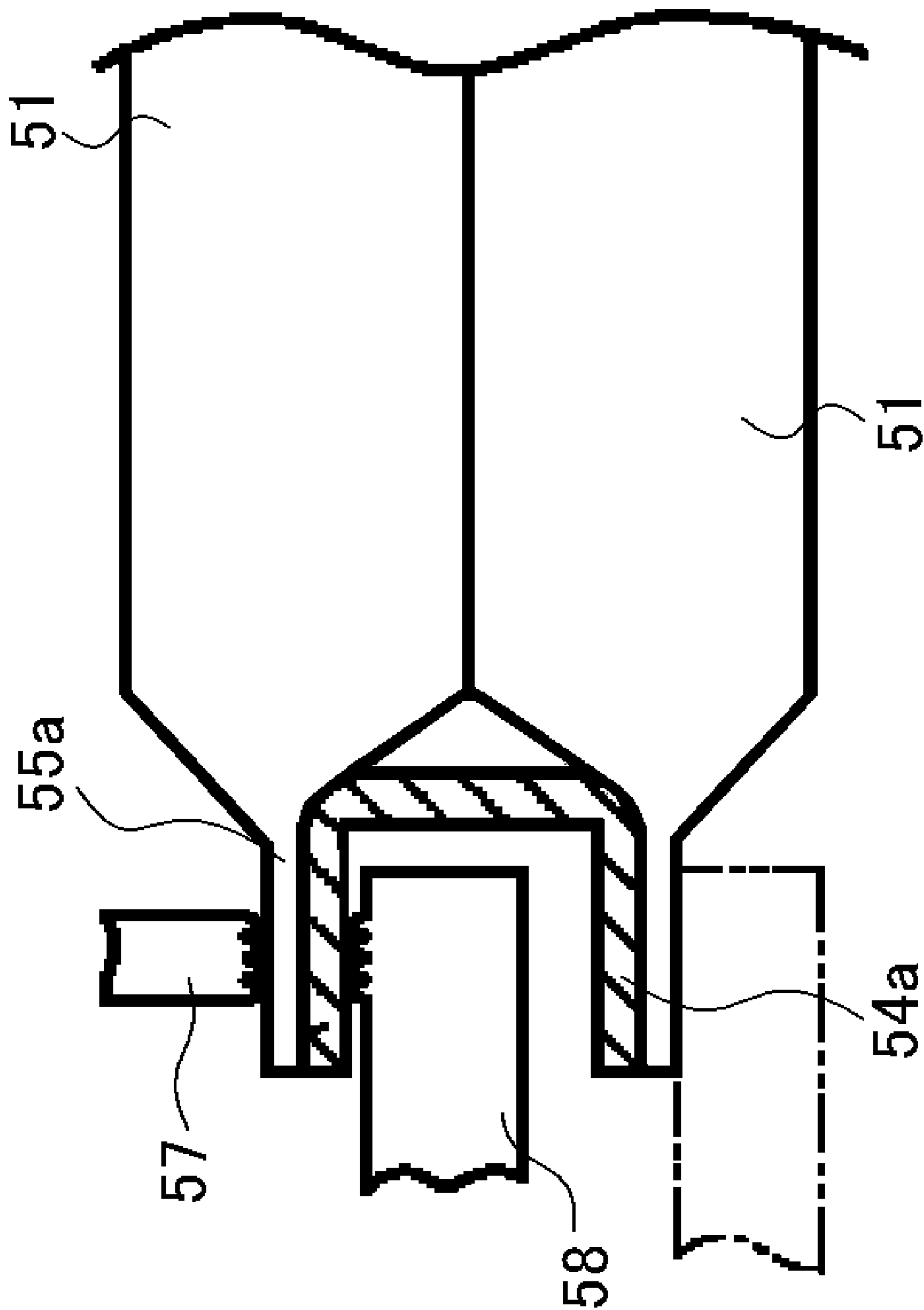
FIG.10 (PRIOR ART)
