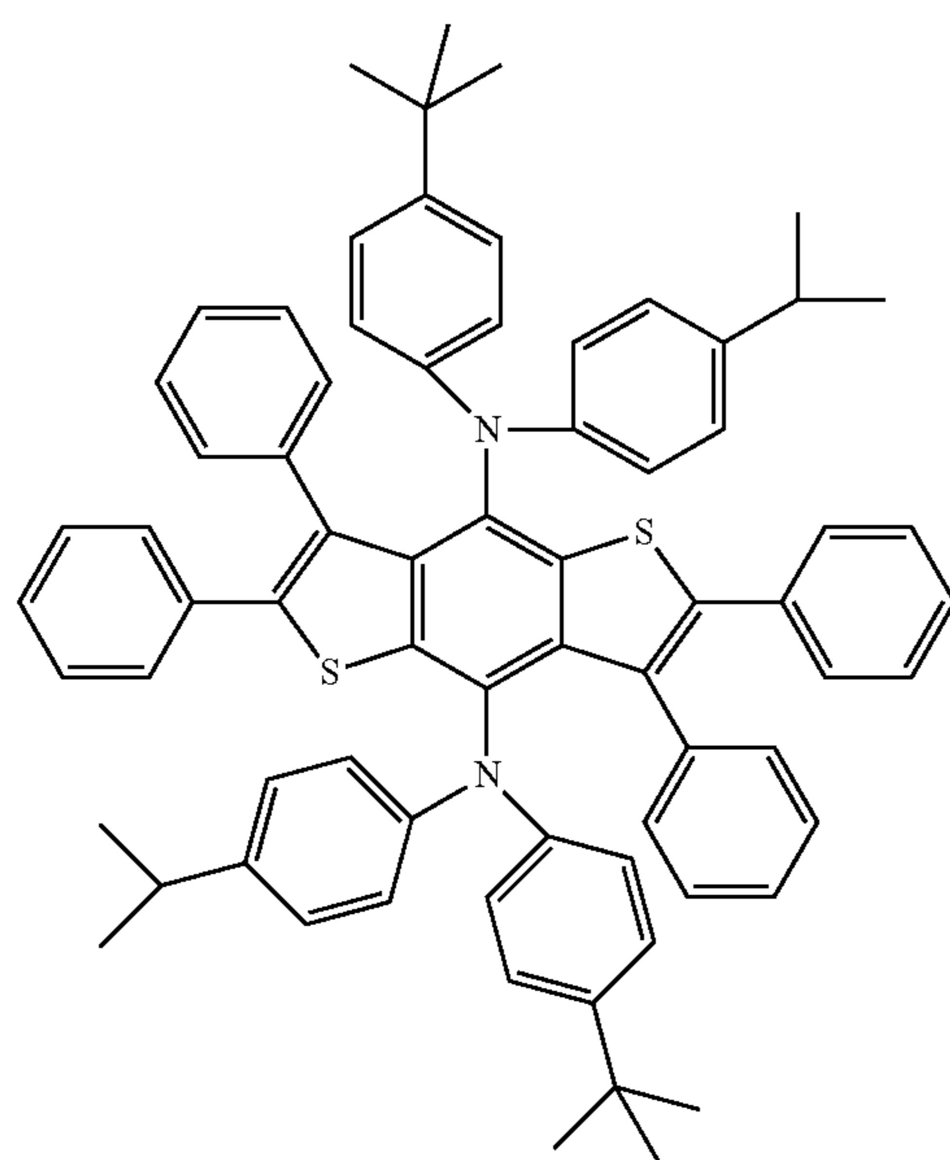
Compound 22
