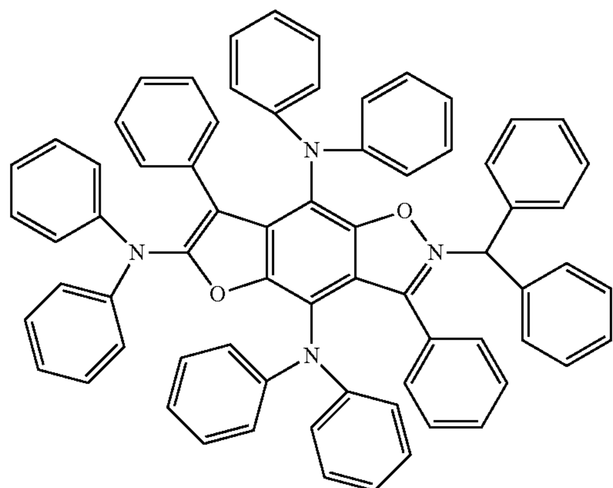
Compound 20
