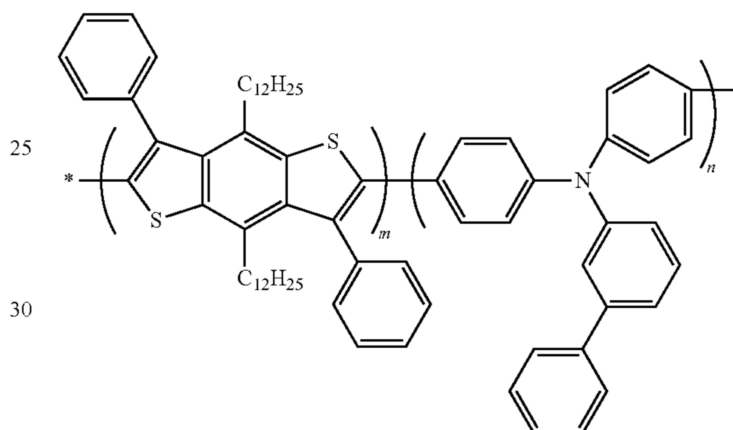
Compound 34
