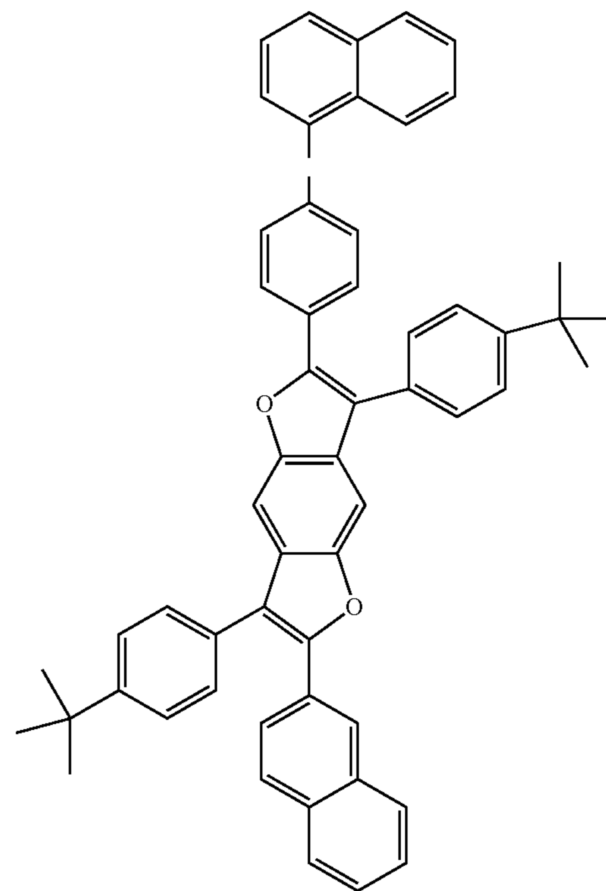
Compound 13
