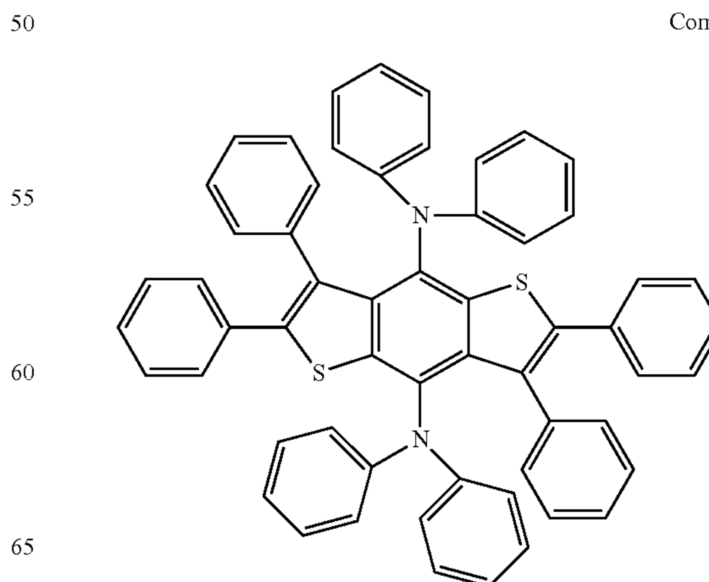
Compound 16
