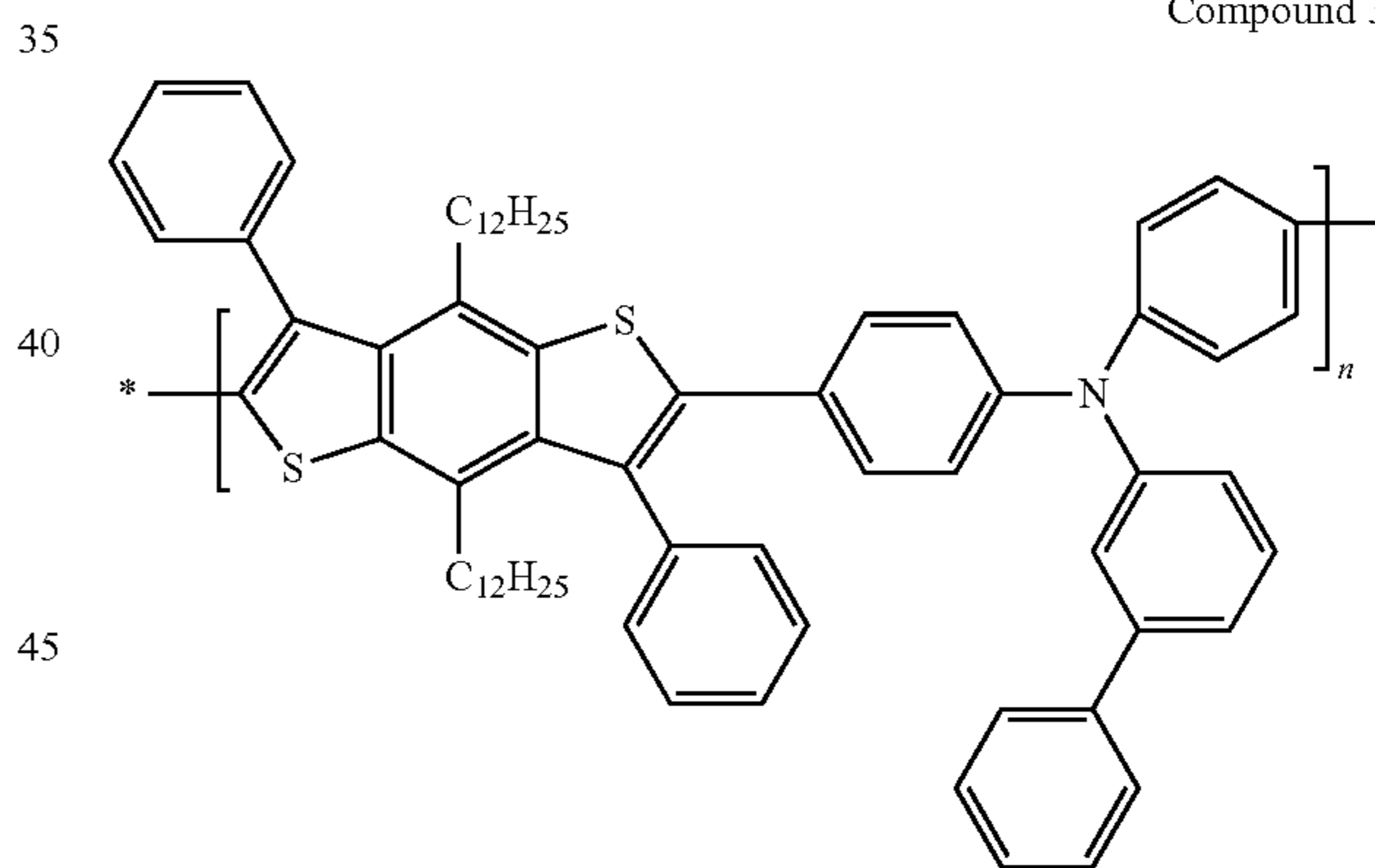
Compound 34
