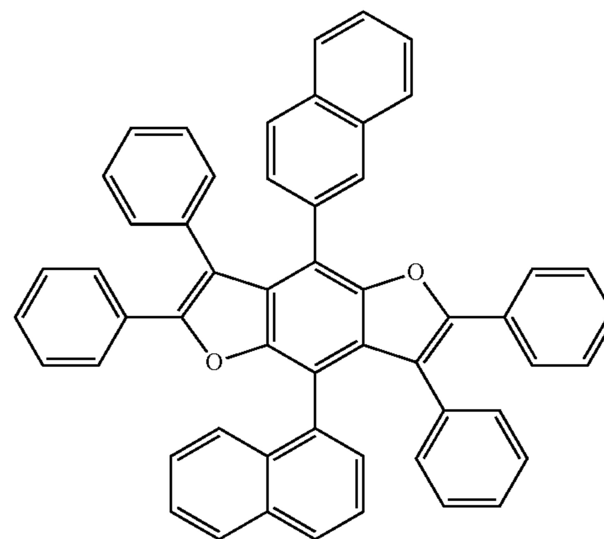
Compound 24
