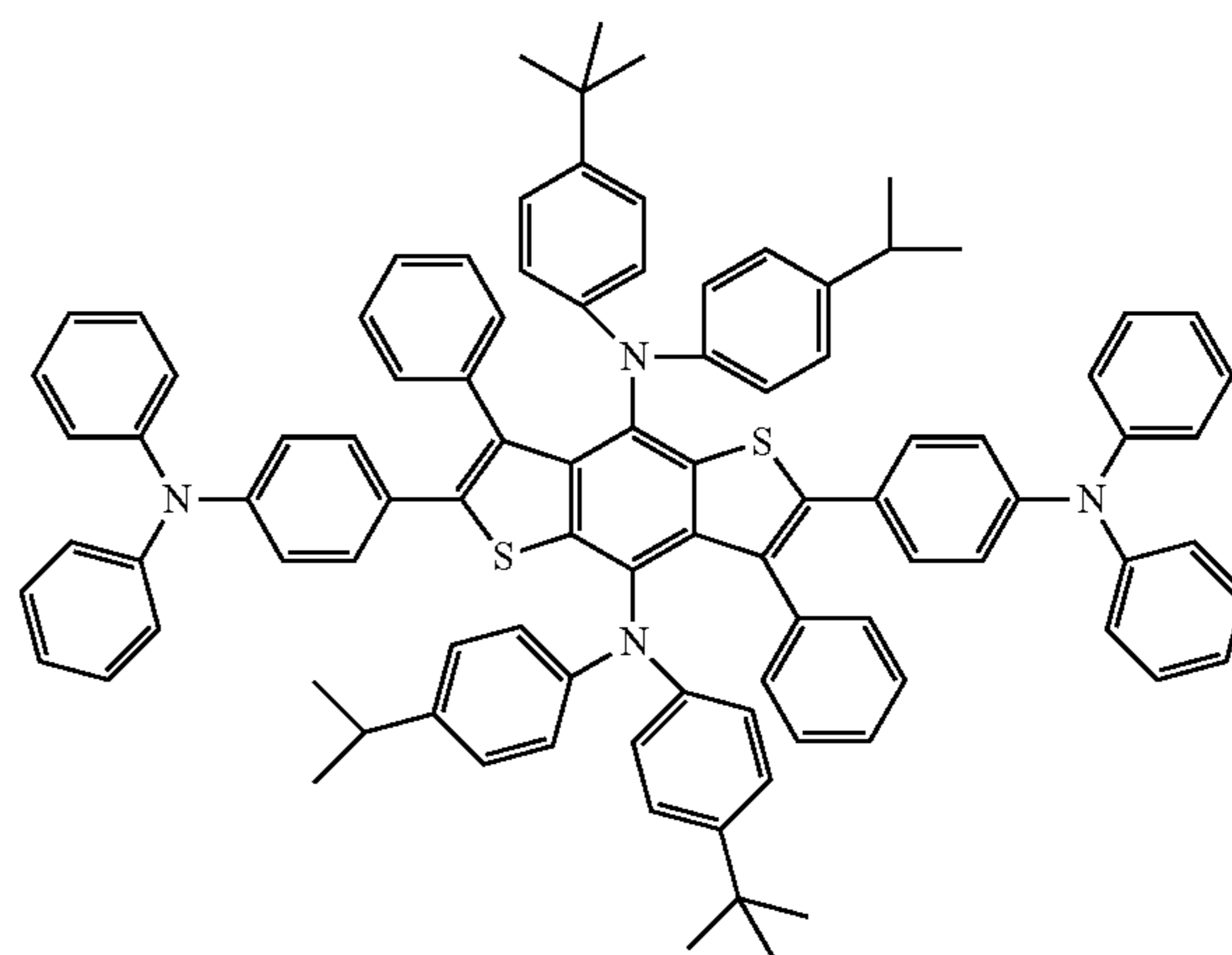
Compound 23
