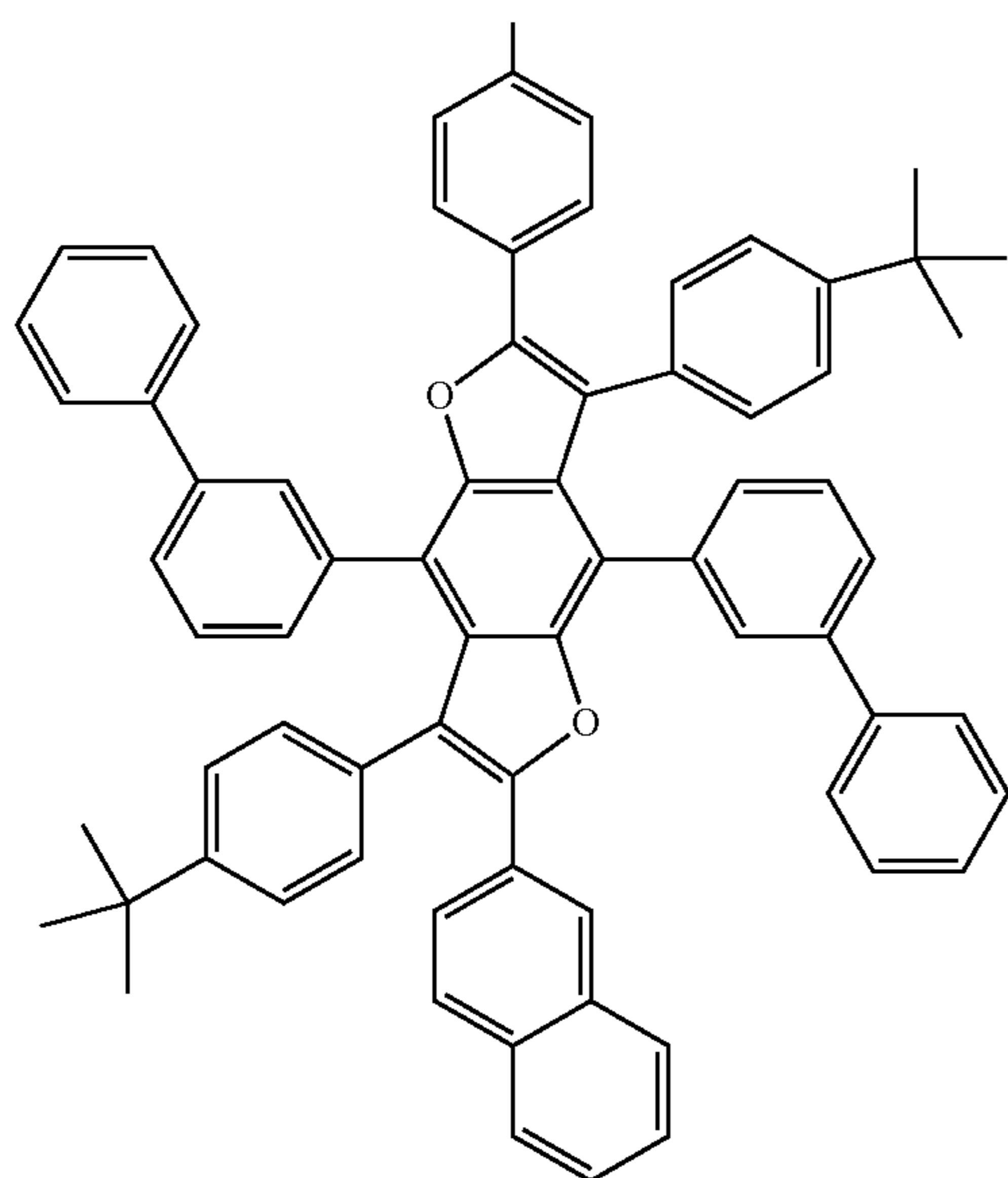
Compound 15
