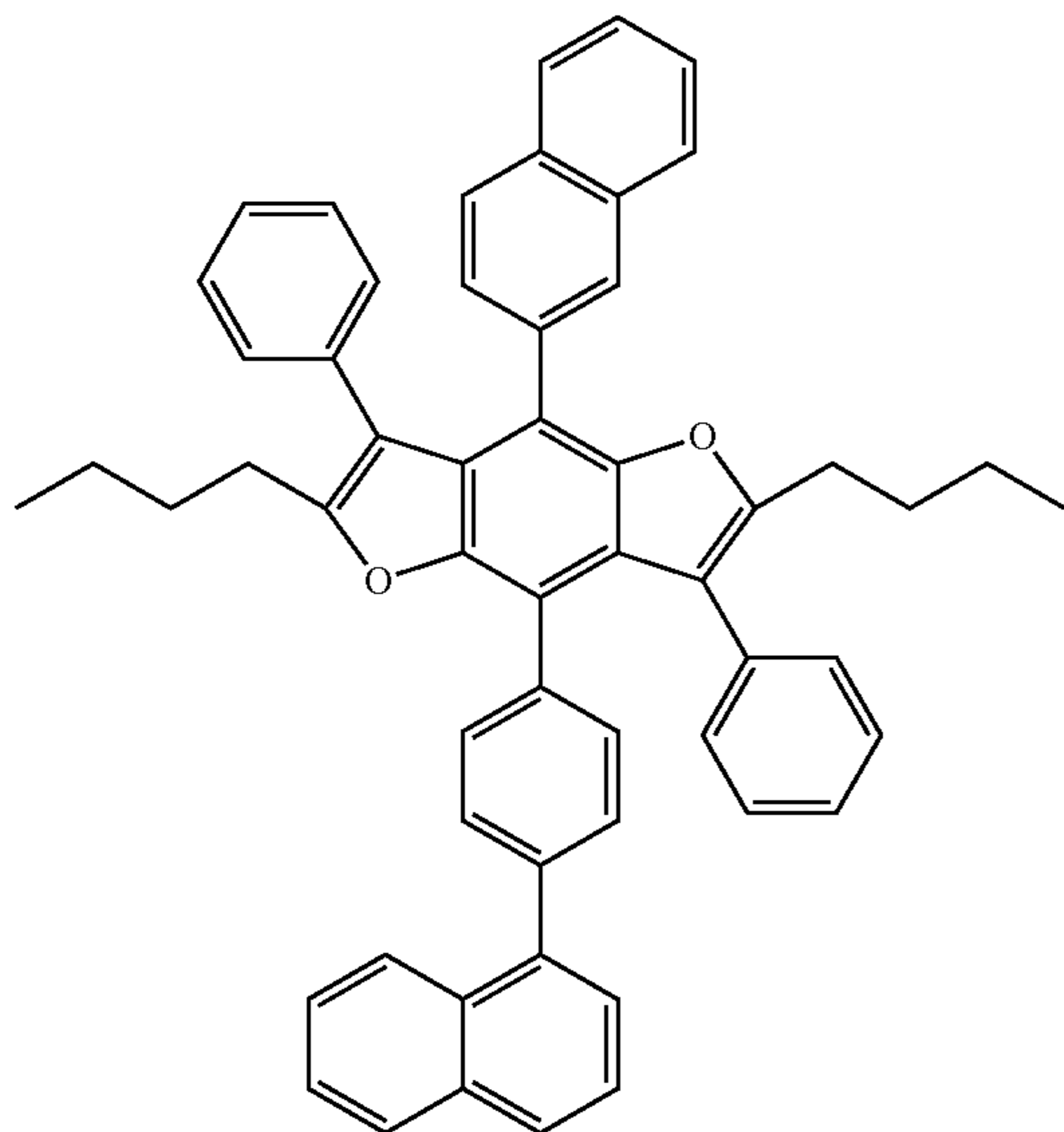
Compound 10
