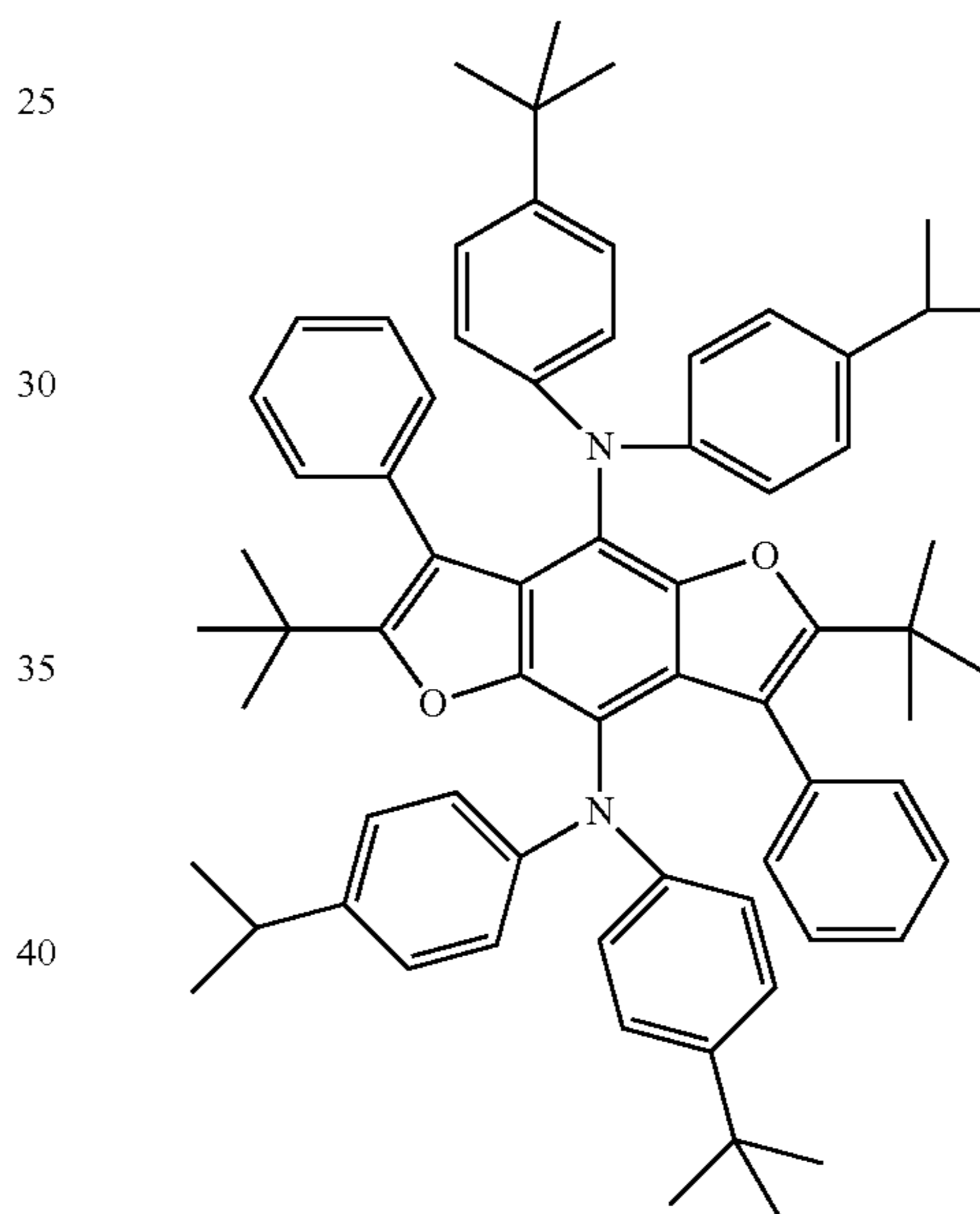
Compound 15
