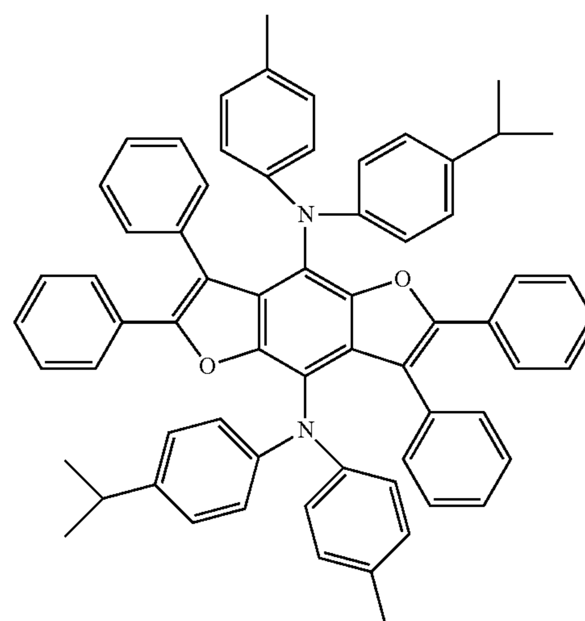
Compound 25
