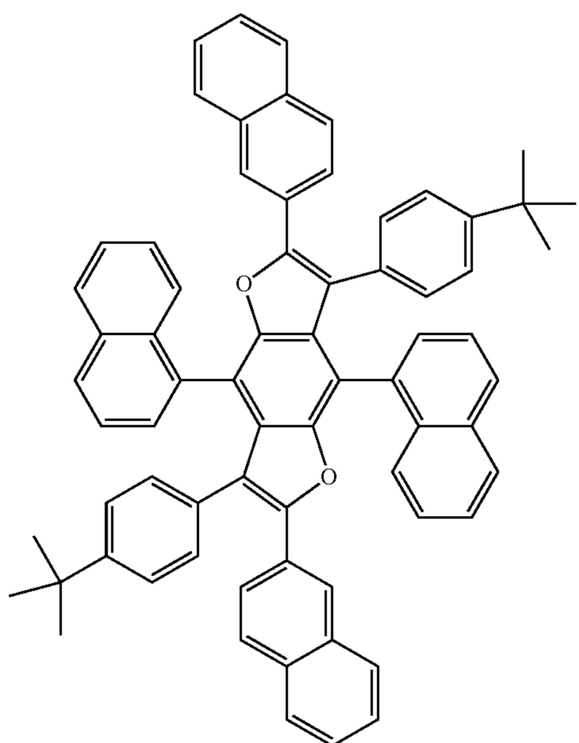
Compound 15
