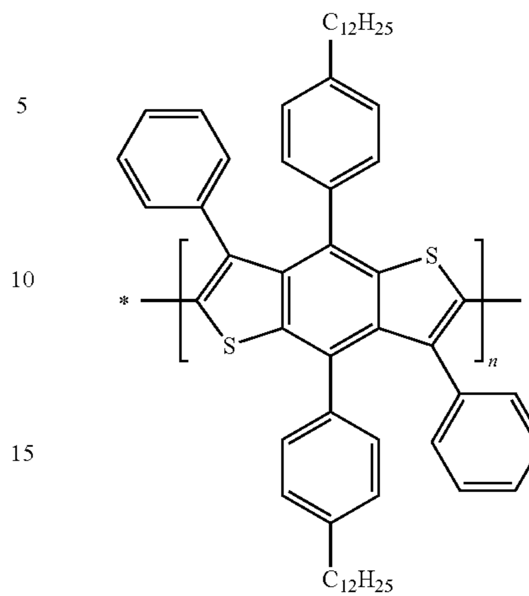
Compound 33
