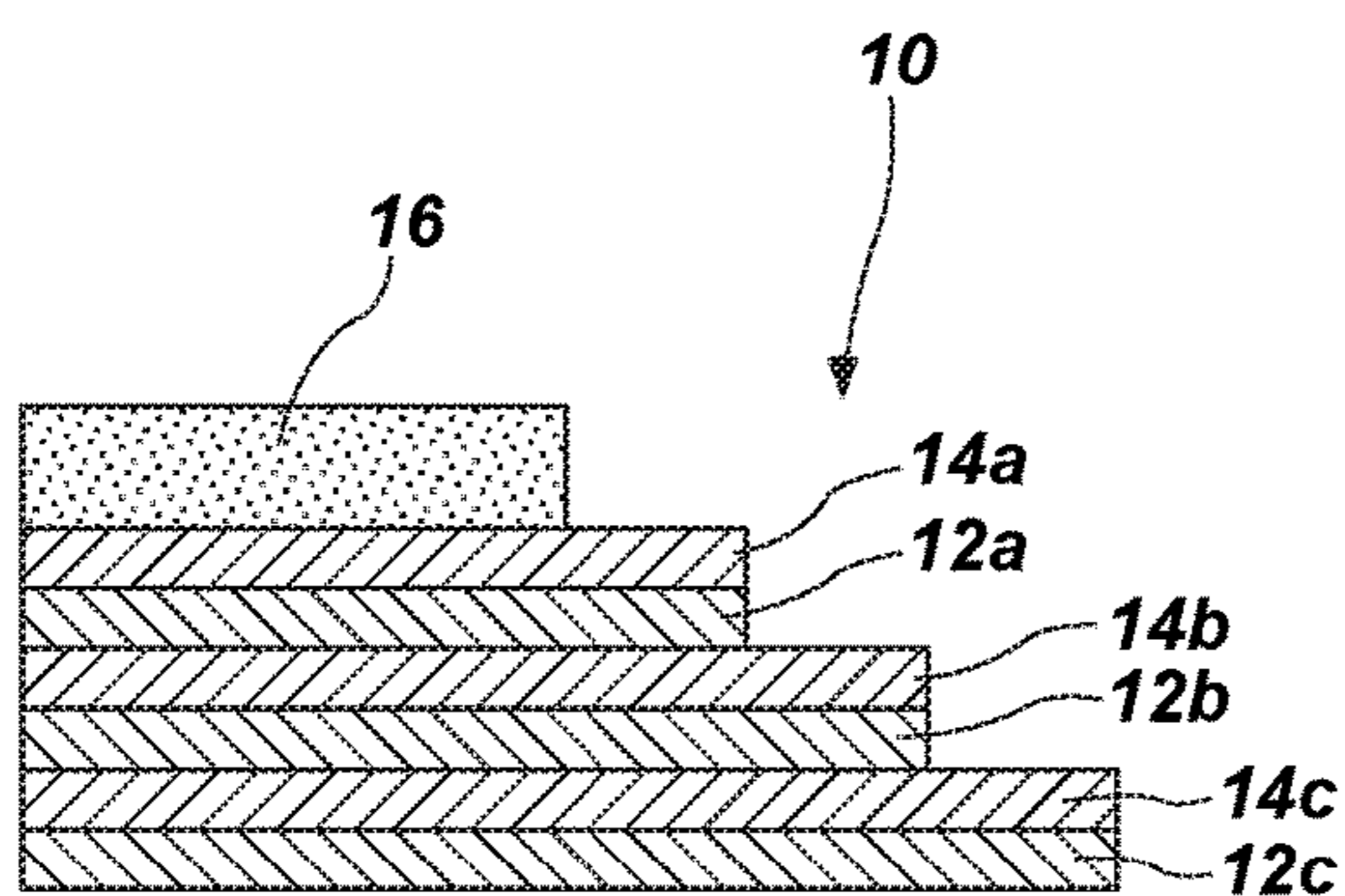
FIG. 1C (PRIOR ART)
