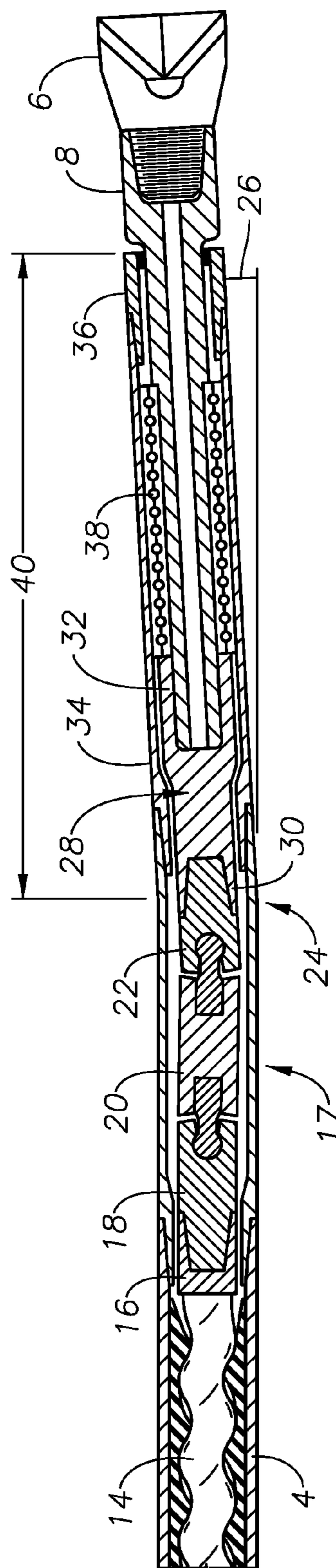
FIG. 2 (Prior Art)
