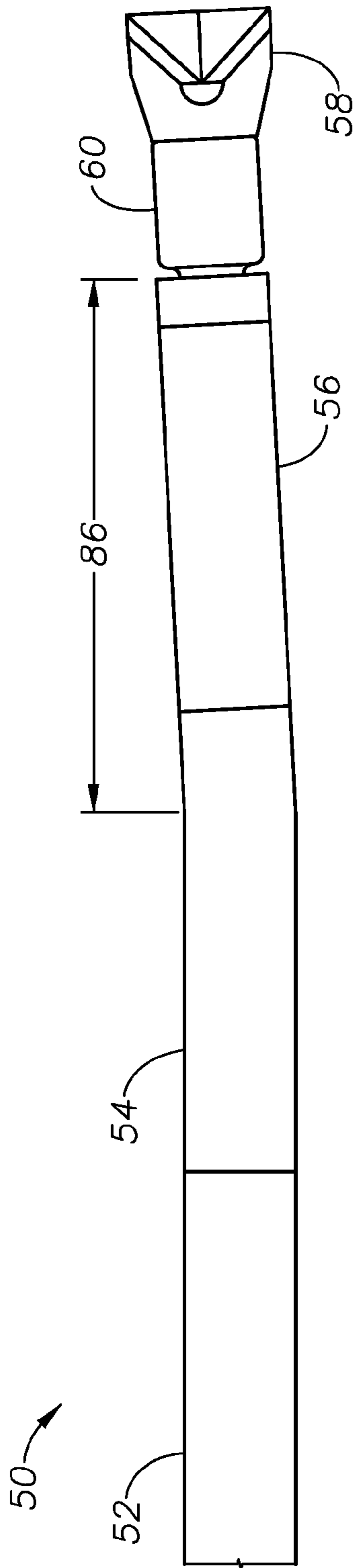
FIG. 3 (Prior Art)
