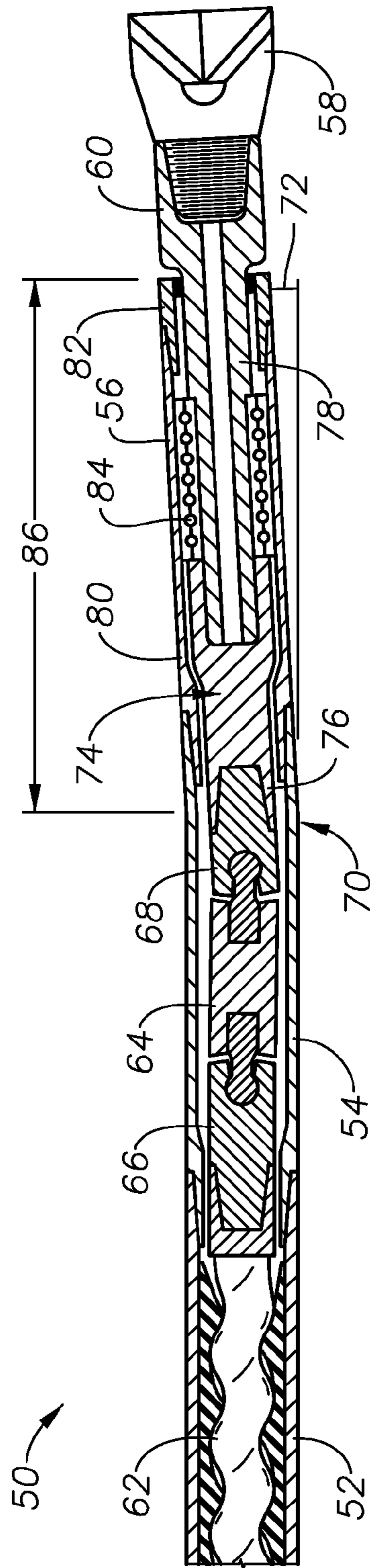
FIG. 4 (Prior Art)
