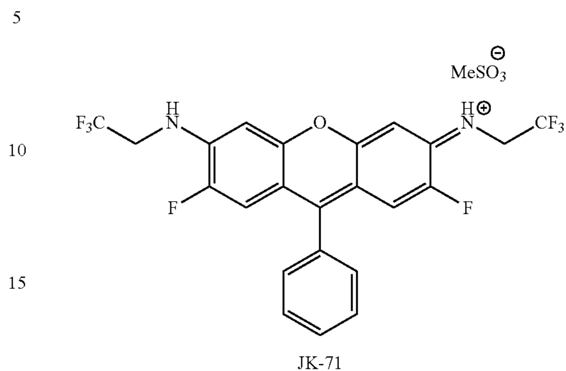
(Z)-N-(2,7-difluoro-9-phenyl-6-((2,2,2-trifluoroethyl)amino)-3H-xanthene-3-ylidene)-2,2,2-trifluoroethan-1-aminium methanesulfonate
