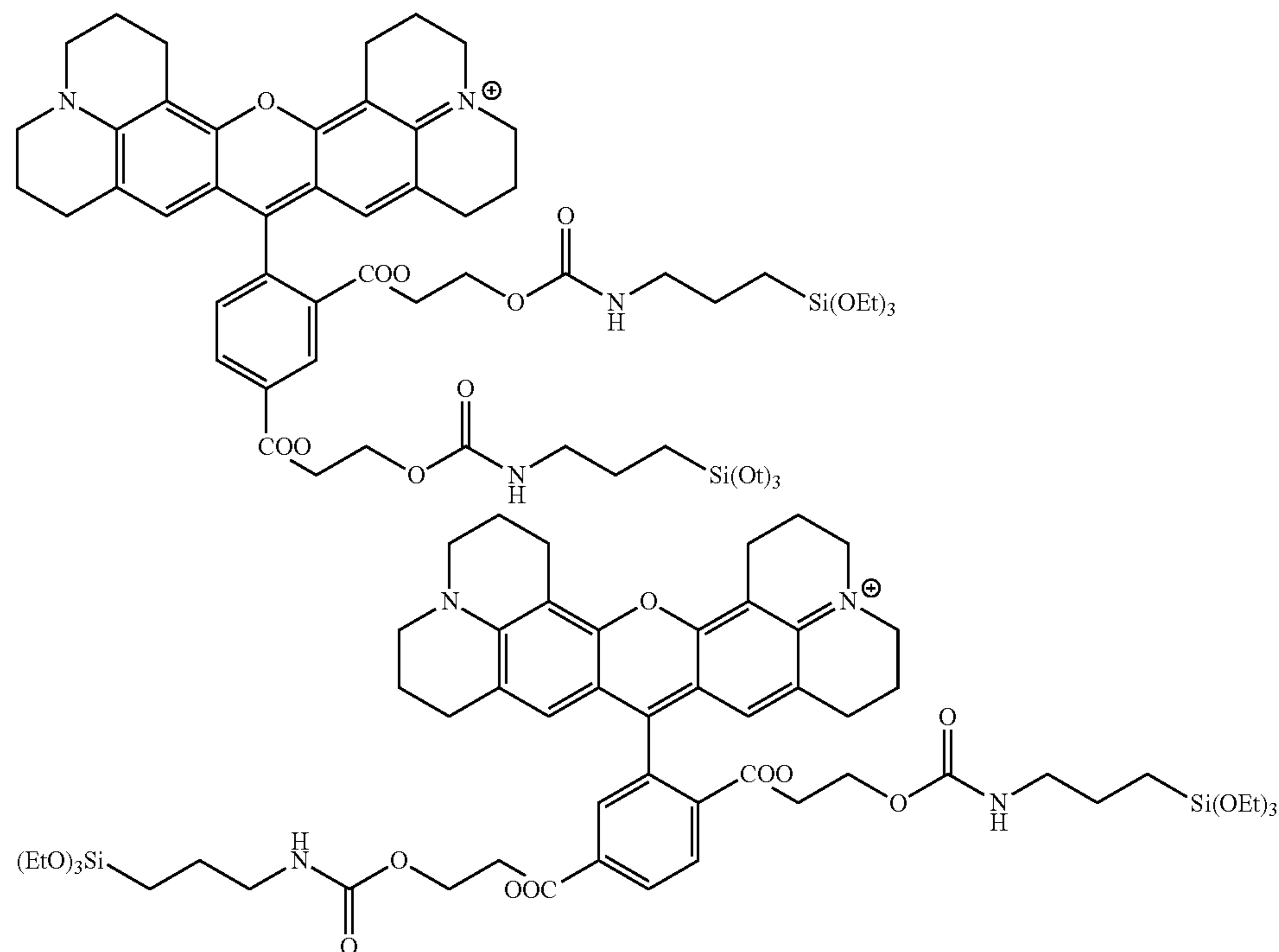
5- and 6-Carboxy X-rhodamine-Silylated
