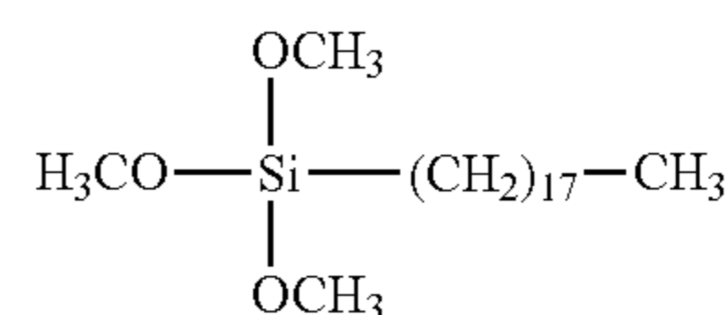
Octadecyltrimethoxysilane
