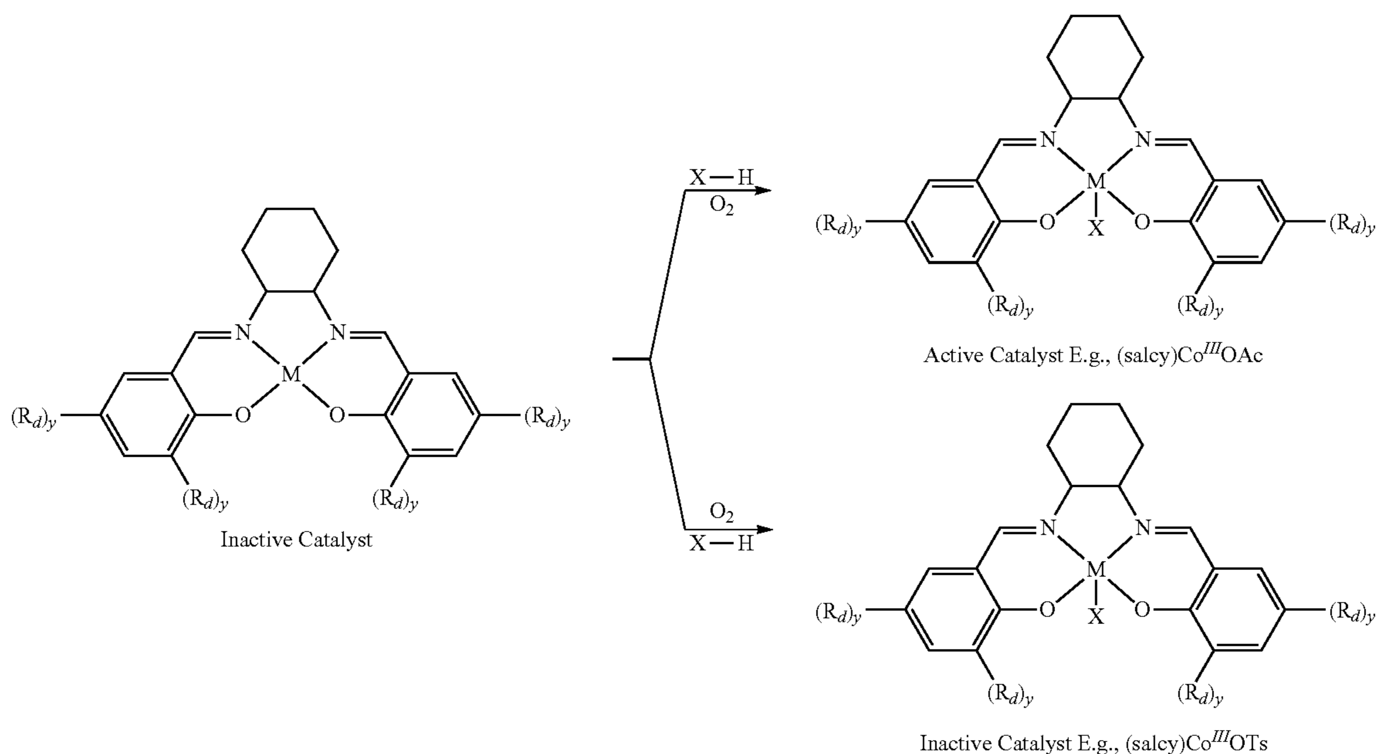
Scheme I-Exemplary Catalyst Synthesis
