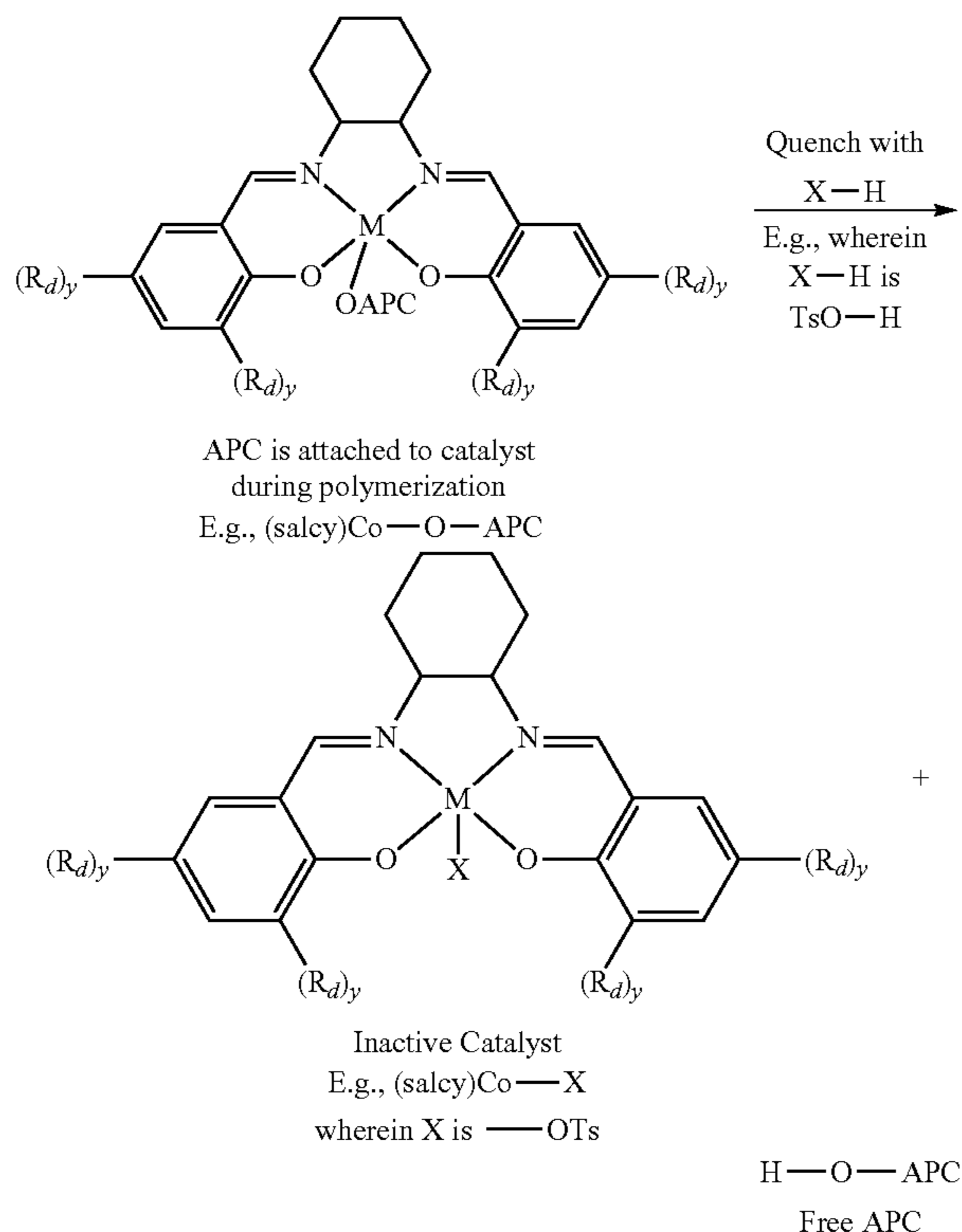
Scheme II-Exemplary Polymerization Quench
