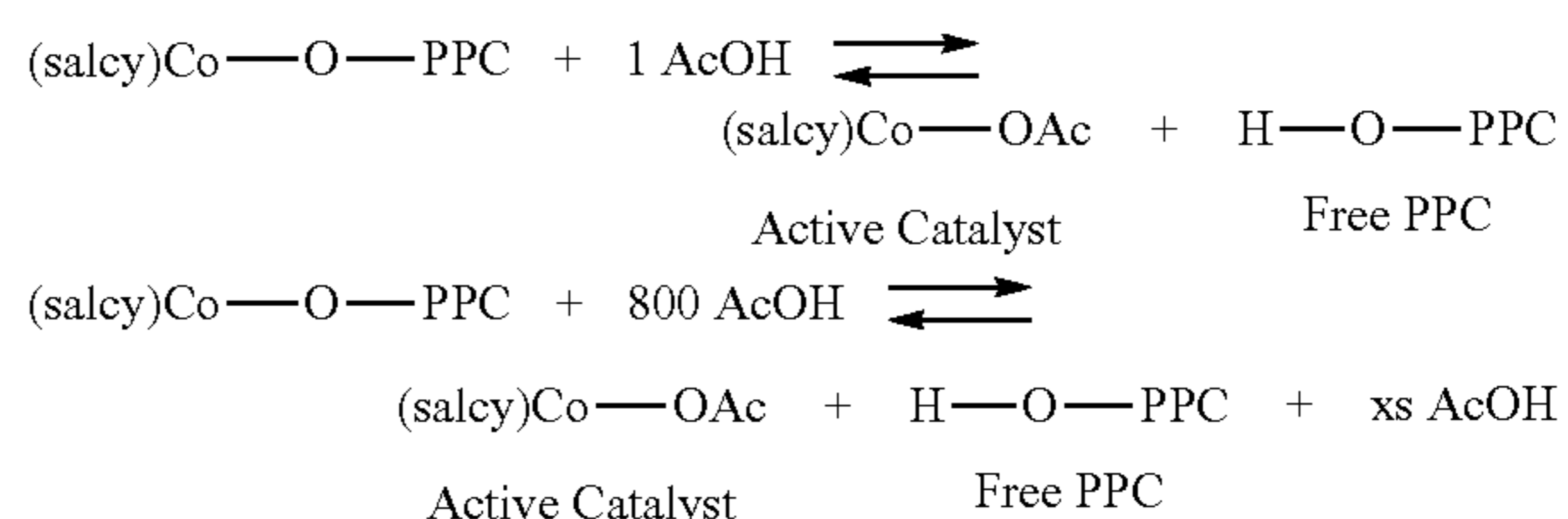
Scheme III - Exemplary Acetic Acid Quench
