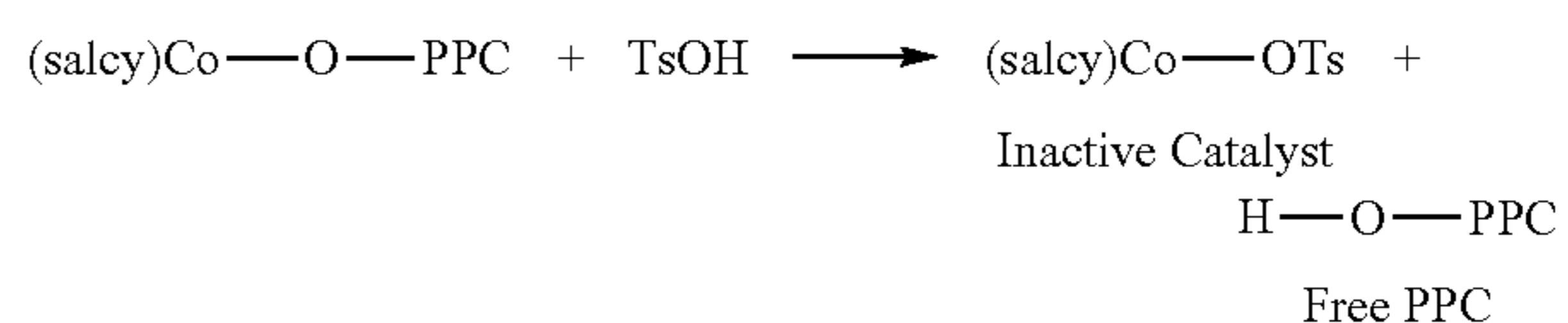
Scheme IV-Exemplary p-Toluene sulfonic acid (TsOH) Quench
