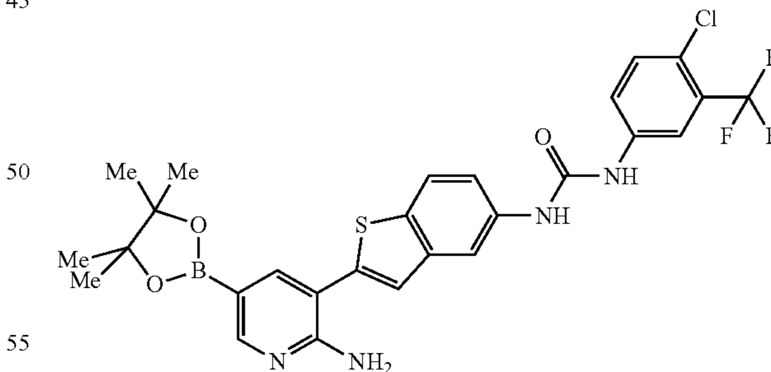
1-{2-[2-amino-5-(4,4,5,5-tetramethyl-1,3,2-dioxaborolan-2-yl)pyridin-3-yl]-1-benzothien-5-yl}-3-[4-chloro-3-(trifluoromethyl)phenyl]urea
