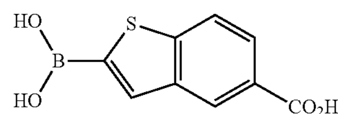
2-(dihydroxyboryl)-1-benzothiophene-5-carboxylic acid
