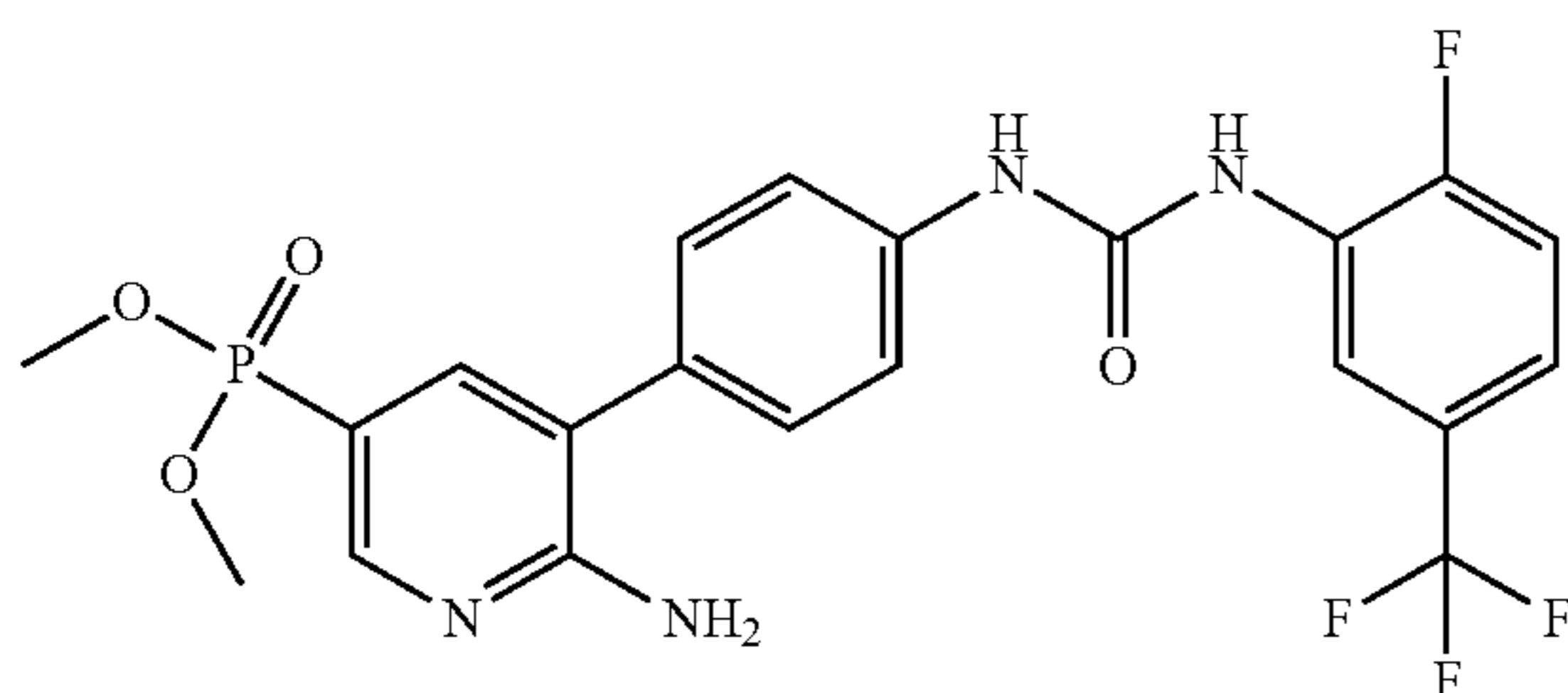
dimethyl {6-amino-5-[4-({[2-fluoro-5-(trifluoromethyl)phenyl]carbamoyl}amino)phenyl]pyridin-3-yl}phosphonate
