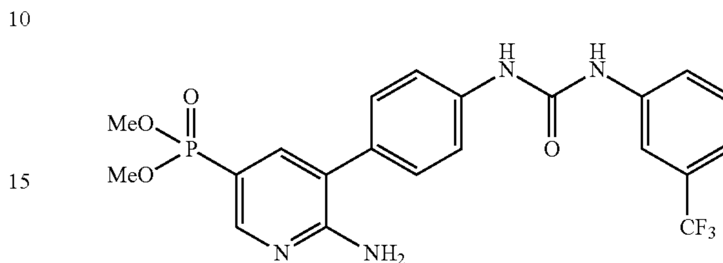
dimethyl (6-amino-5-(4-(3-(3-(trifluoromethyl)phenyl)ureido)phenyl)pyridin-3-yl)phosphonate
