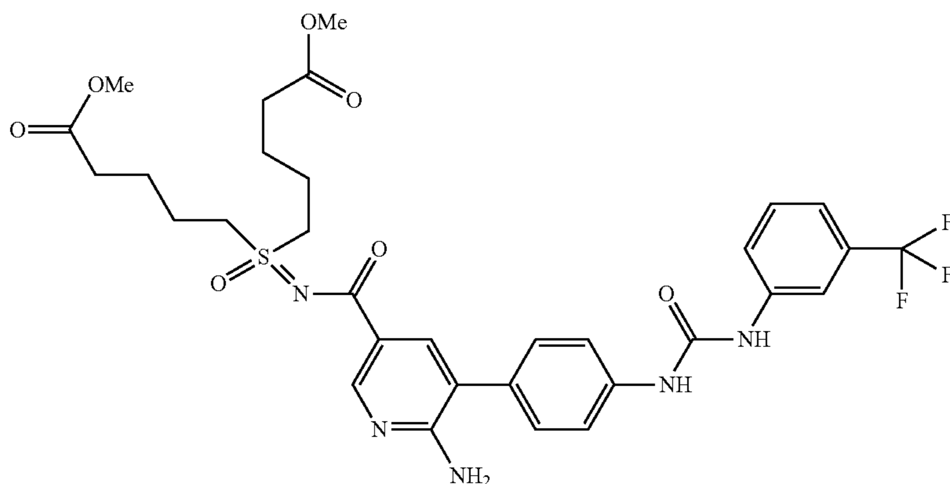
dimethyl 5,5'-(N-([6-amino-5-(4-([3-(trifluoromethyl)phenyl]carbamoyl)amino)phenyl]pyridin-3-yl)carbonyl)sulfonimidoyl)dipentanoate
