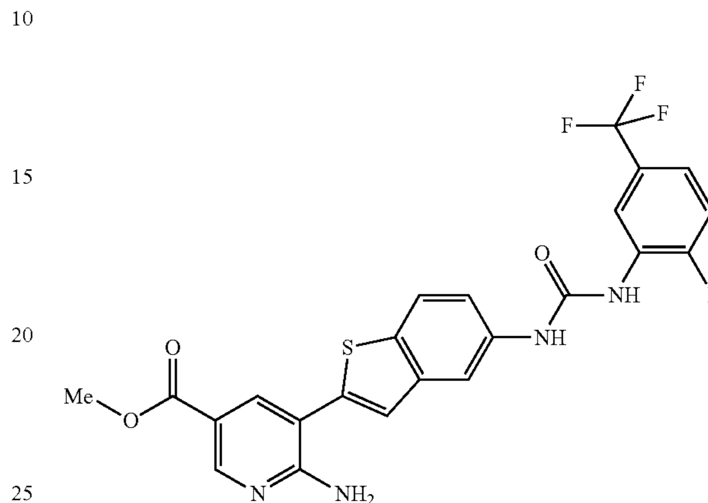
methyl 6-amino-5-{5-[[[2-fluoro-5-(trifluoromethyl)phenyl]amino]carbonyl]amino]-1-benzothien-2-yl}nicotinate
