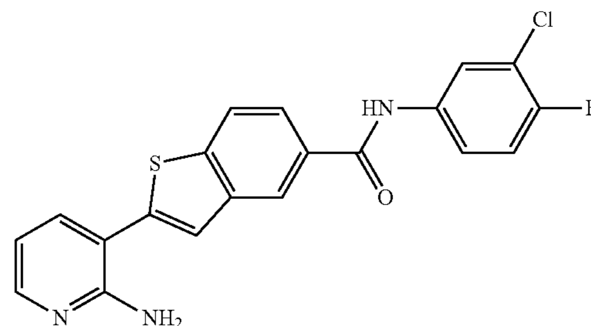
2-(2-aminopyridin-3-yl)-N-(3-chloro-4-fluorophenyl)-1-benzothiophene-5-carboxamide
