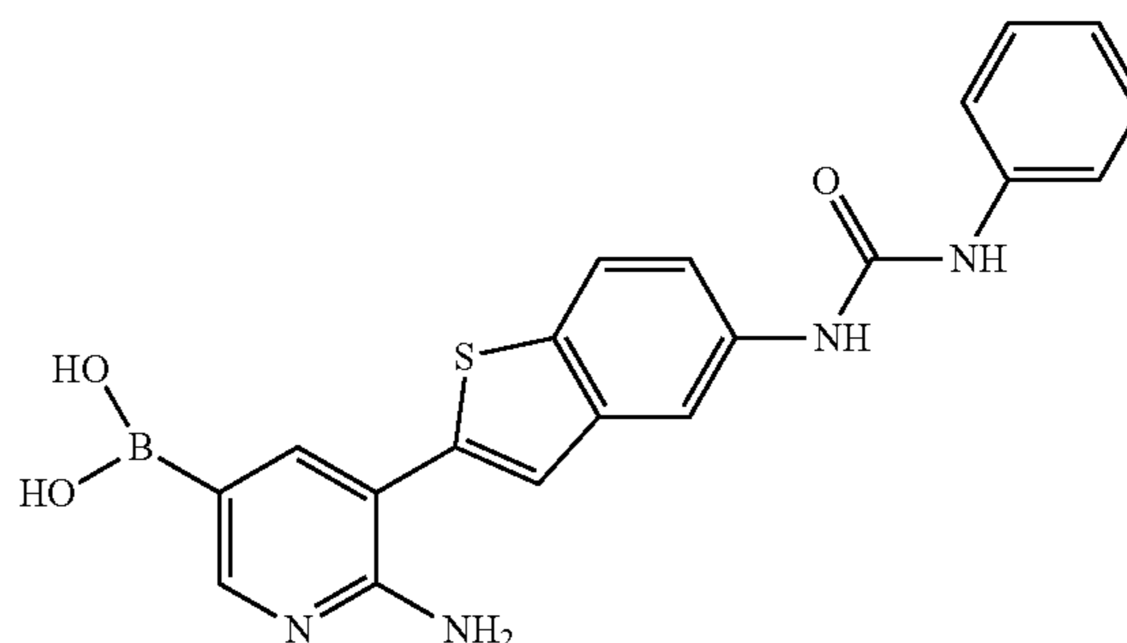
(6-amino-5-[5-((anilino)carbonyl)amino]-1-benzothien-2-yl)pyridin-3-ylboronic acid
