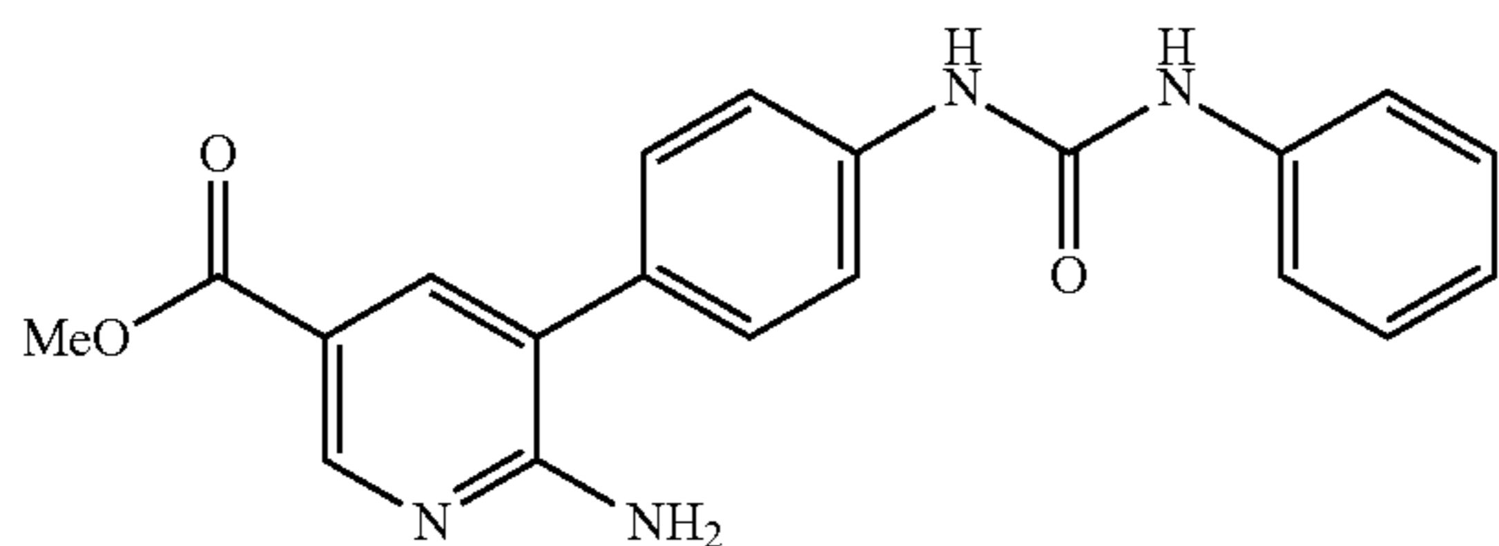
methyl 6-amino-5-[4-((phenylcarbamoyl)amino)phenyl]pyridine-3-carboxylate
