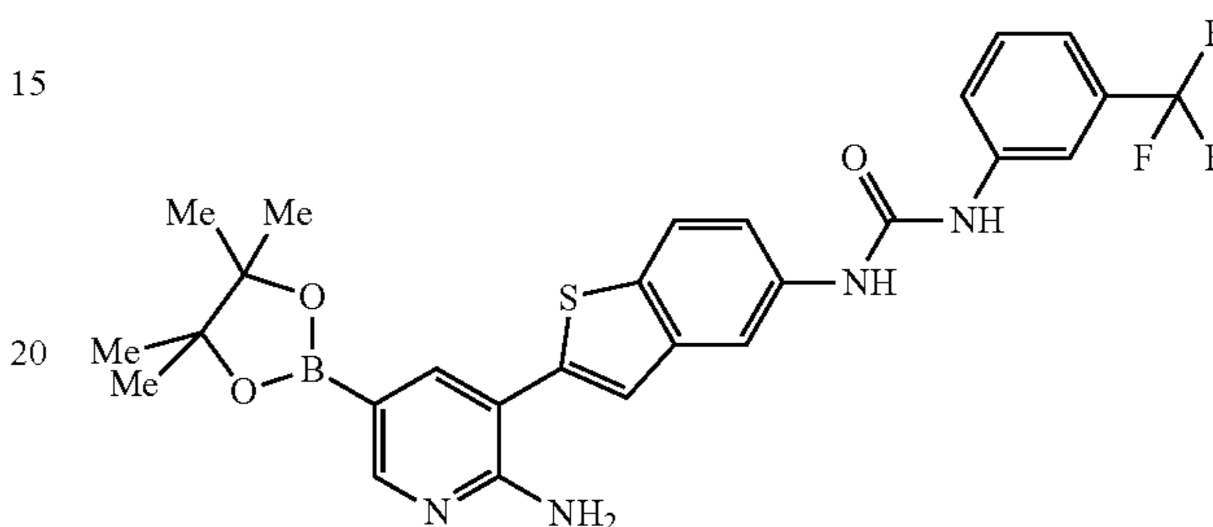
1-{2-[2-amino-5-(4,4,5,5-tetramethyl-1,3,2-dioxaborolan-2-yl)pyridin-3-yl]-1-benzothien-5-yl}-3-[3-(trifluoromethyl)phenyl]urea
