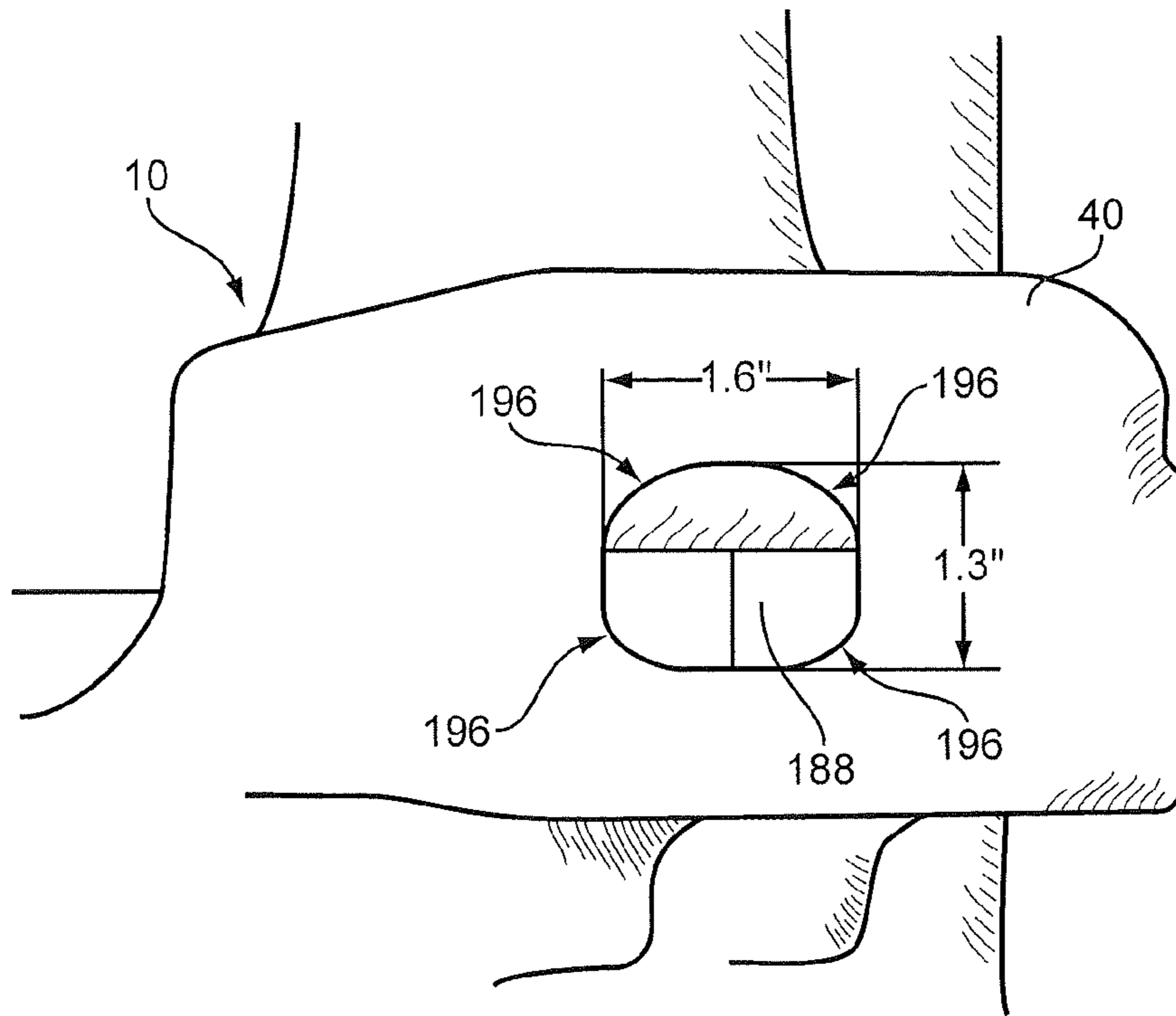
FIG. 30 PRIOR ART
