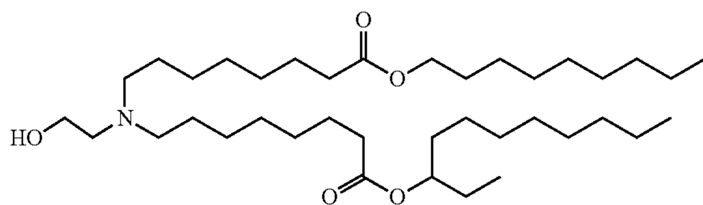
Chemical Formula: C_{38}H_{75}NO_5 Molecular Weight: 626.02
