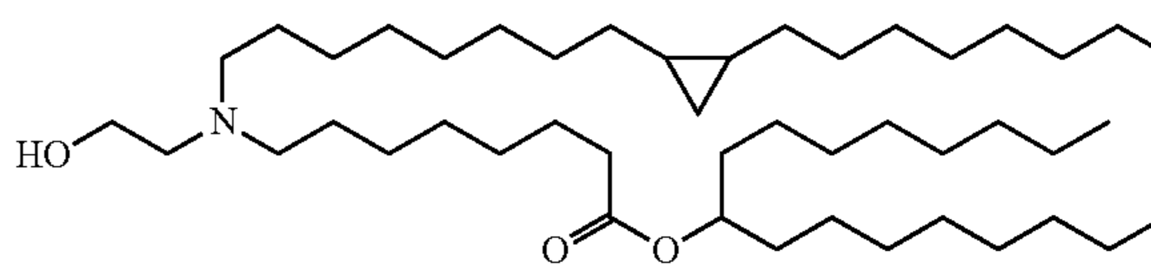
Chemical Formula: C_{46}H_{91}NO_3 Molecular Weight: 706.24
