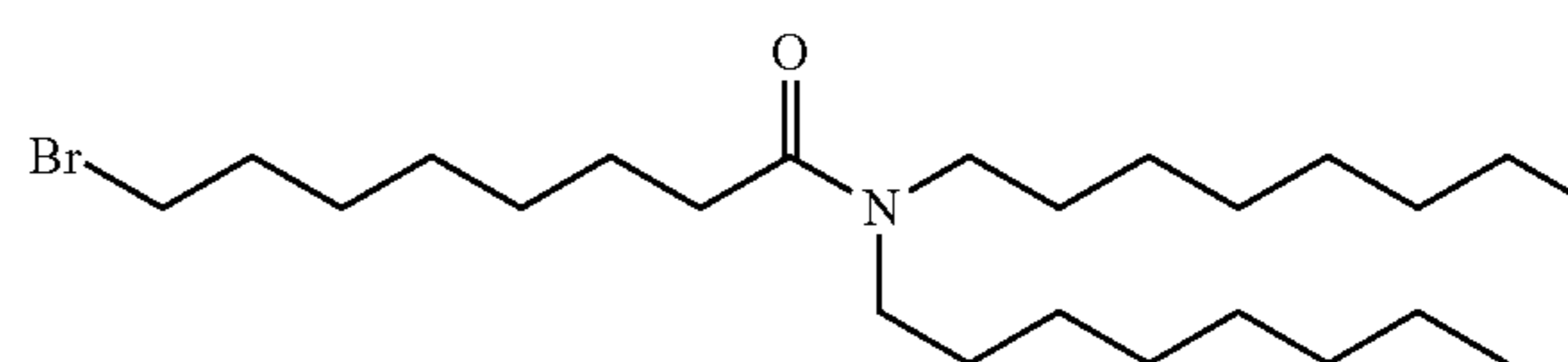
BI. Compound 144: Nonyl 8-((8-(diocetyl)amino)-8-oxooctyl)(2-hydroxyethyl)amino)octanoate 8-Bromo-N,N-diocetyl octanamide
