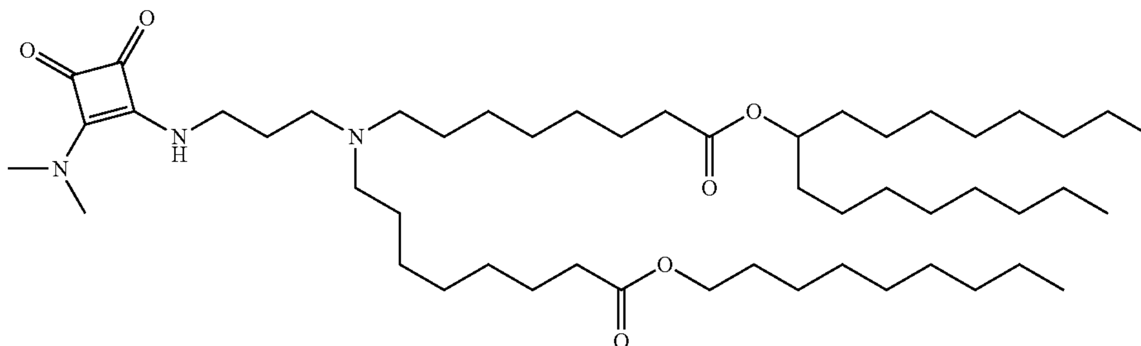
Chemical Formula: C 51 H 95 N 3 O 6 Molecular Weight: 846.34
