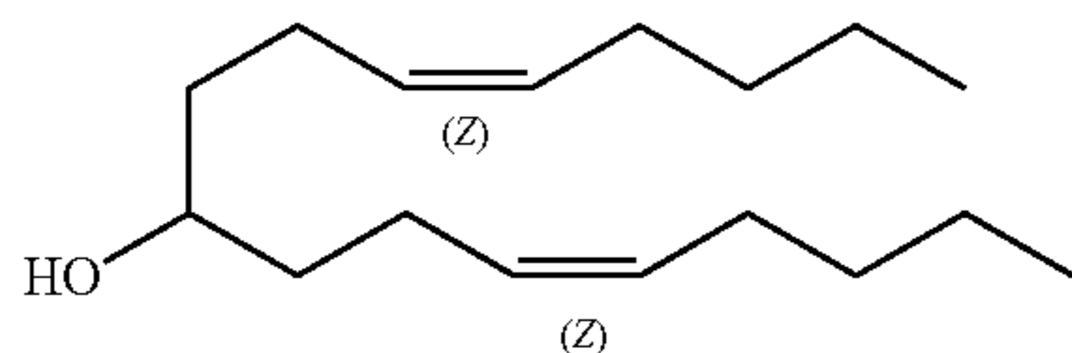
Chemical Formula: C 17 H 32 O Molecular Weight: 252.44
