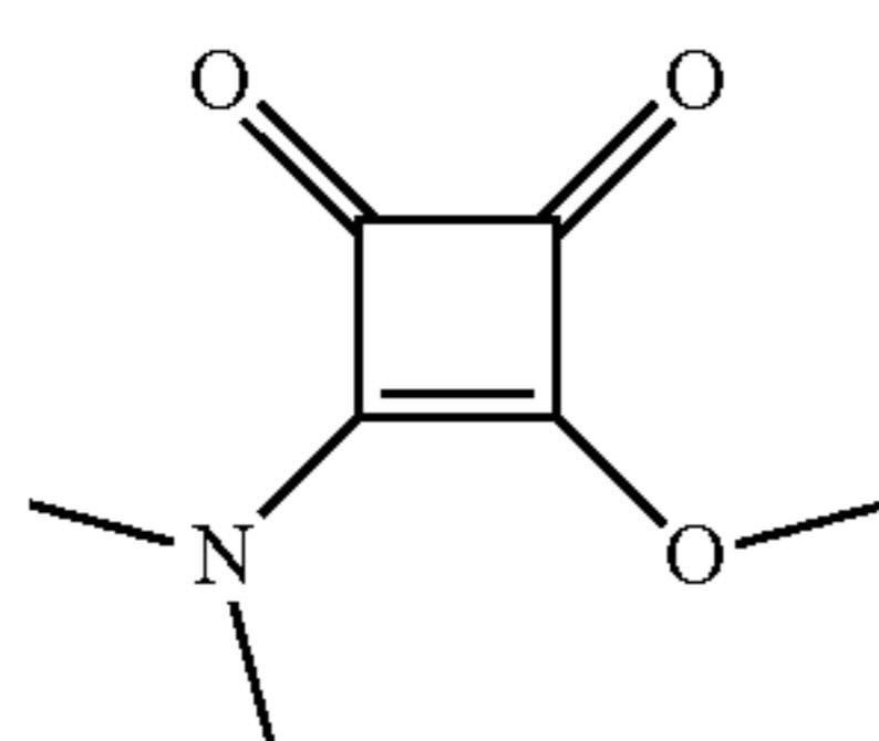
Chemical Formula: C 7 H 9 NO 3 Molecular Weight: 155.15
