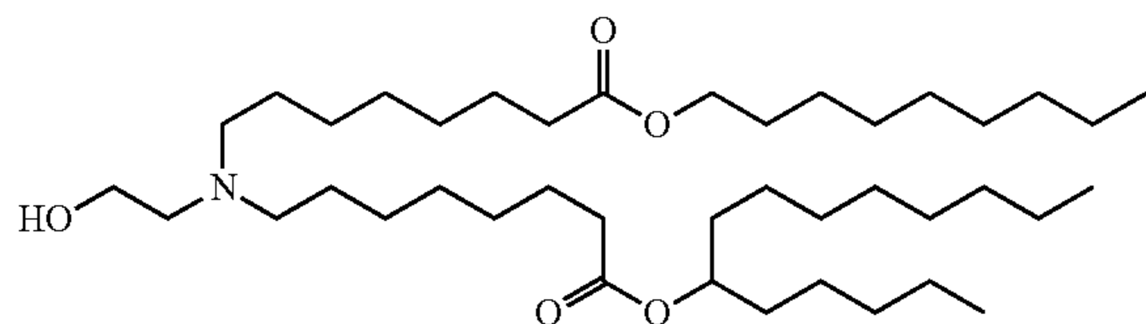
Chemical Formula: C_{41}H_{81}NO_5 Molecular Weight: 668.10
