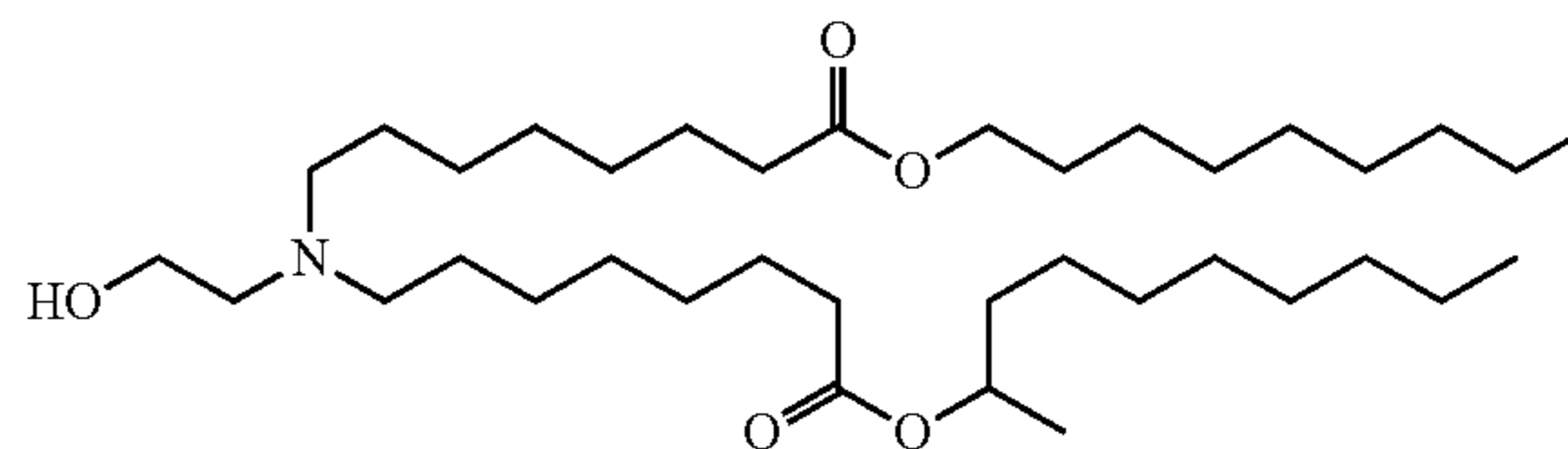
Chemical Formula: C_{37}H_{73}NO_5 Molecular Weight: 611.99
