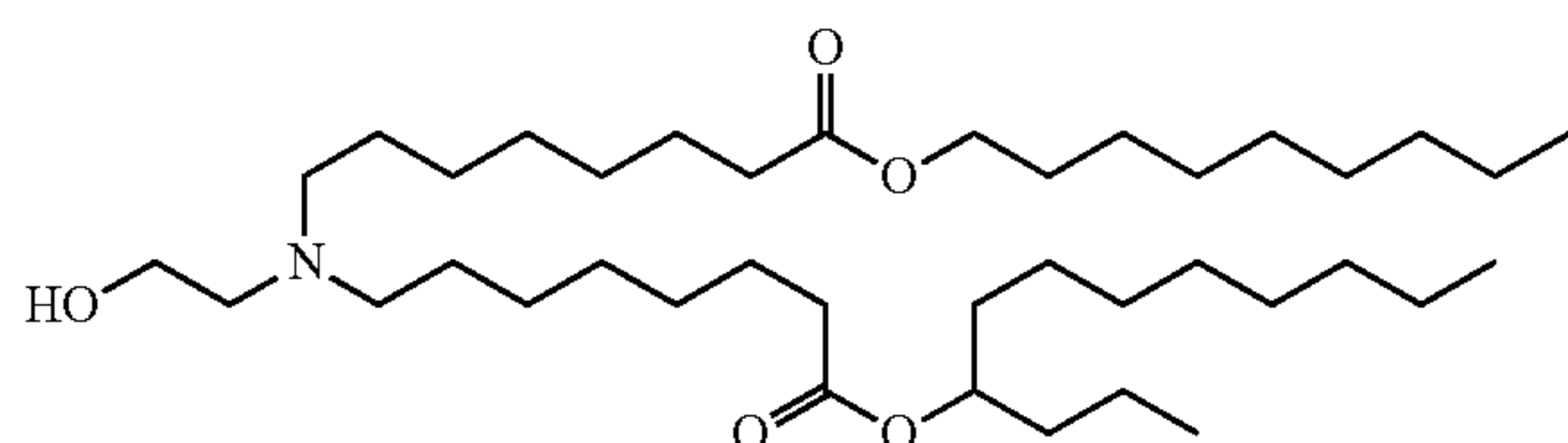
Chemical Formula: C_{39}H_{77}NO_5 Molecular Weight: 640.05
