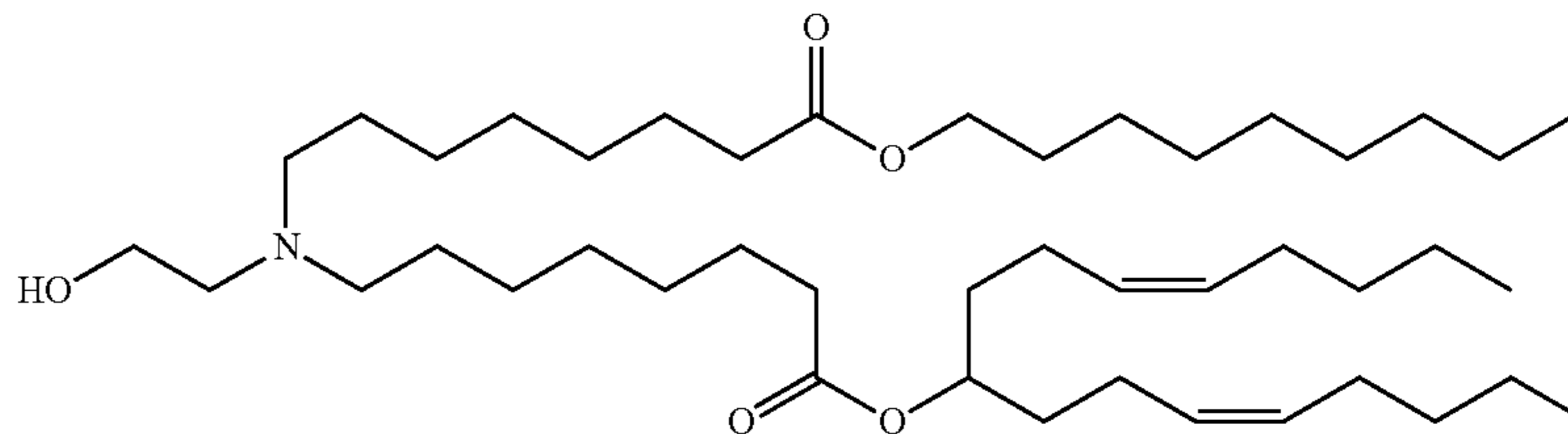
Chemical Formula: C 44 H 83 NO 5 Molecular Weight: 706.15
