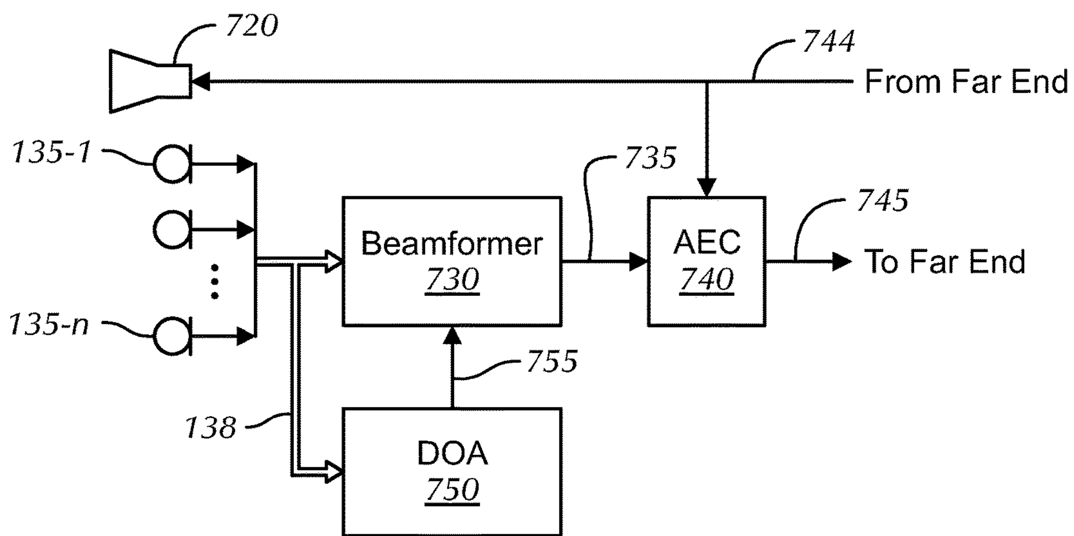
FIG. 7 (Prior Art)
