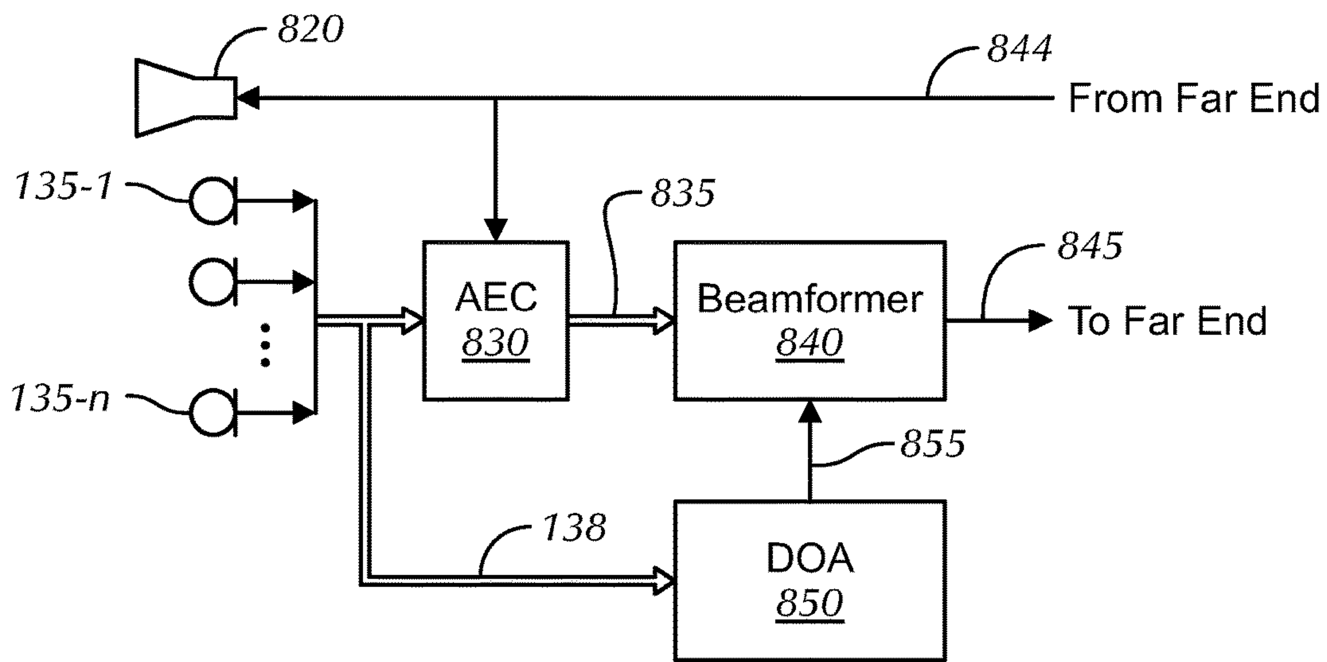
FIG. 8 (Prior Art)
