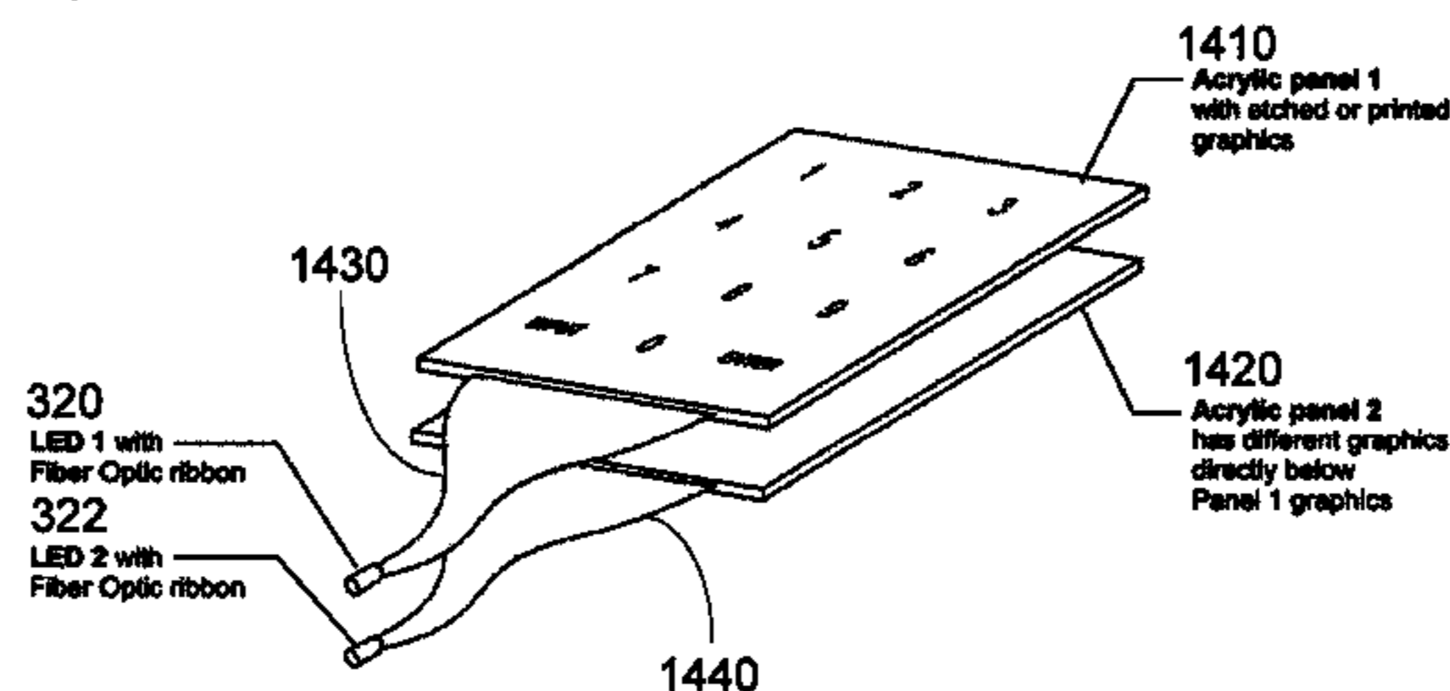
Exploded View
